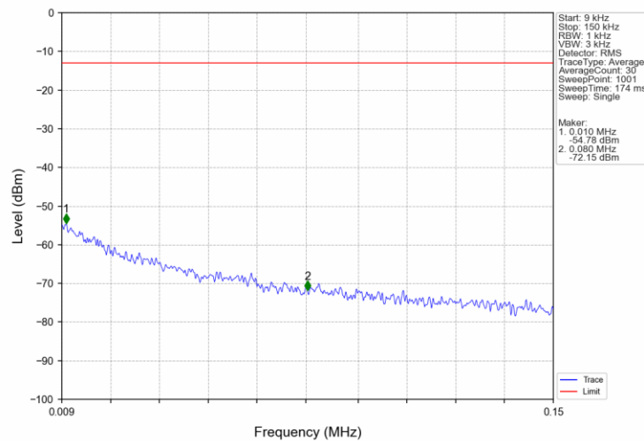
Band66_1.4MHz_16QAM_HCH_1779.3MHz_RB_1_0_NTNV
