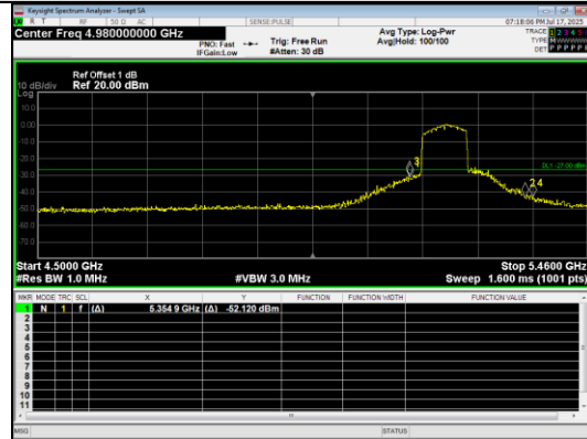
Out Of Band Emission IEEE 802.11ac_Channel 42_80MHz_Antenna 0
