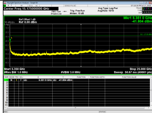
Spurious Emission:5350~25000.0 MHz IEEE 802.11ac_Channel 42_80MHz_Antenna 0
