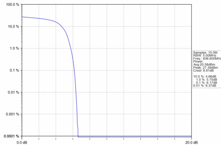
Band5 HSUPA MCH 836.6MHz Subtest 1 NTN
