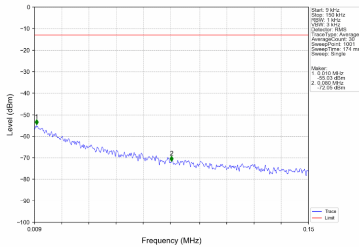
Band66_3MHz_16QAM_HCH_1778.5MHz_RB_1_0_NTNV
