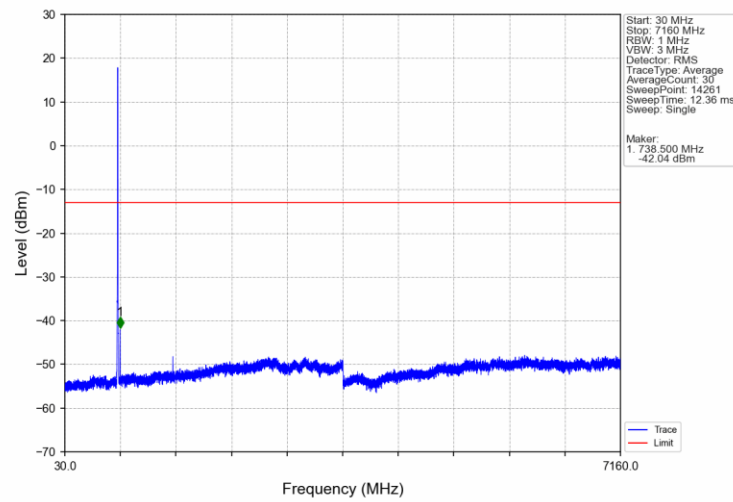
Band12_3MHz_16QAM_MCH_707.5MHz_RB_1_0_NTNV
