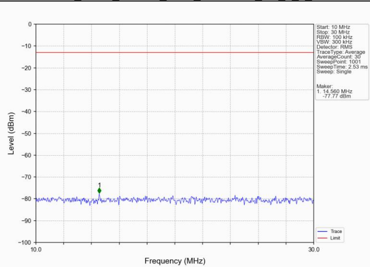
Band12_3MHz_16QAM_MCH_707.5MHz_RB_1_0_NTNV
