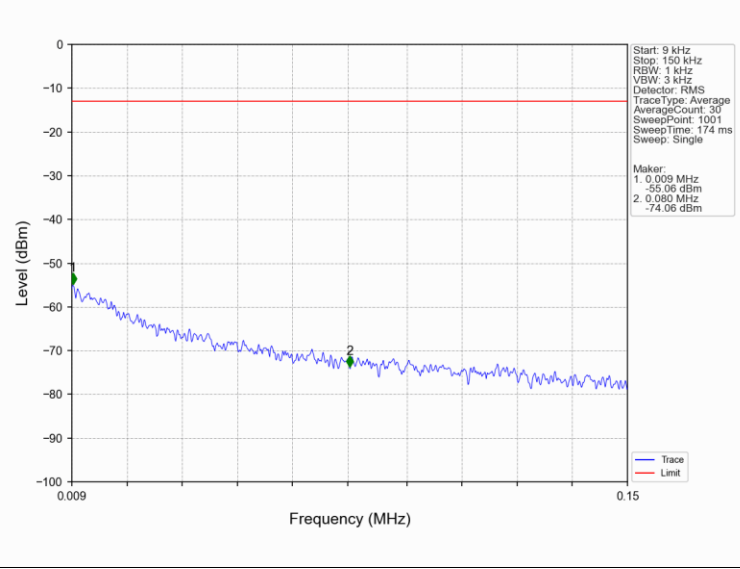
Band5_5MHz_16QAM_HCH_846.5MHz_RB_1_0_NTNV
