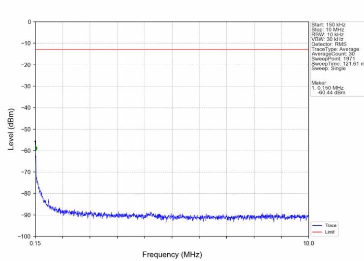
Band5_5MHz_16QAM_HCH_846.5MHz_RB_1_0_NTNV
