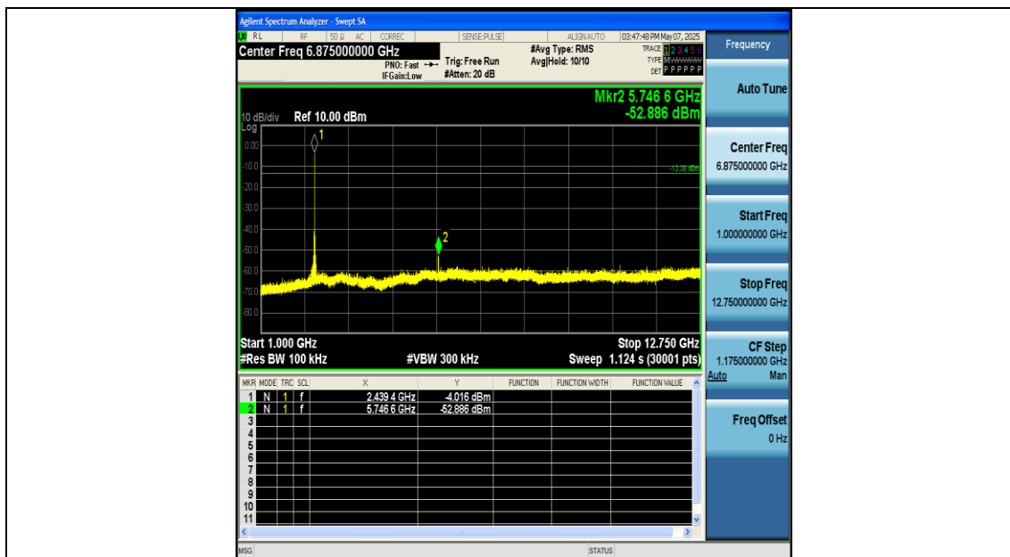
SRD-Ant1-2439-1000~12750-PASS
