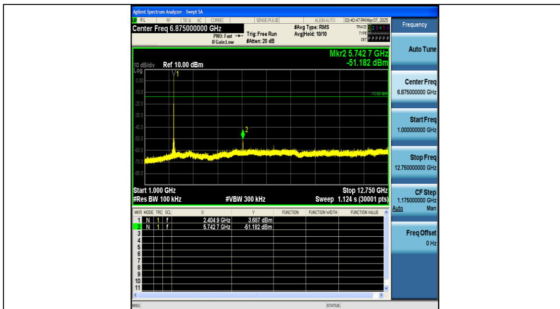
SRD-Ant1-2405-1000~12750-PASS
