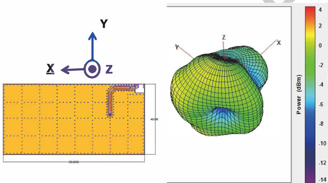
Radiation Pattern
