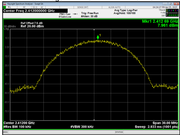
Band Edge NVHT b 2412MHz Ant1 Emission
