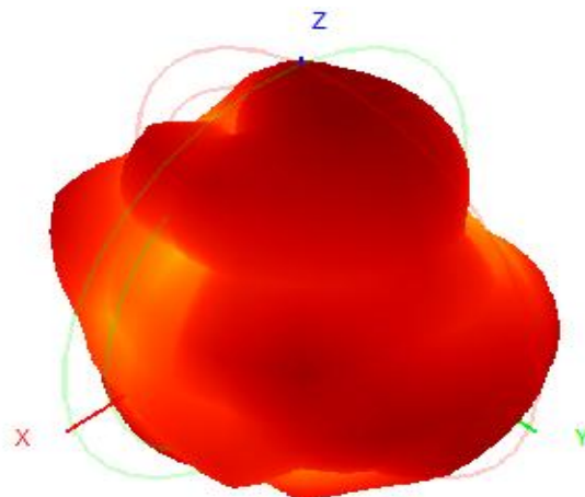
(6) Typical Free Space 3D Radiation Pattern at 2500MHz(unit:dBi)
