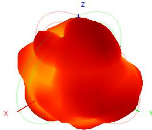
(5) Typical Free Space 3D Radiation Pattern at 2450MHz(unit:dBi)
