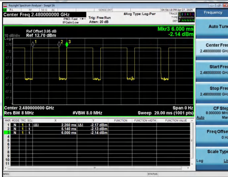
Duty_Cycle_NVNT_ANT1_1-DH5_2480
