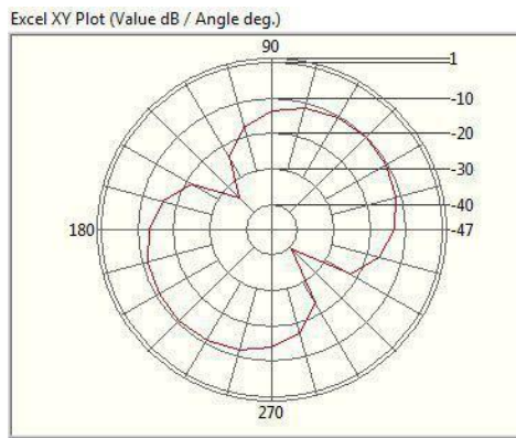
2.485GHz@Theta 0.0 Horizontal
