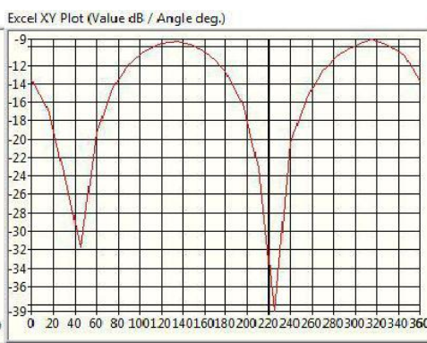
2.485GHz@Theta 0.0 Vertical
