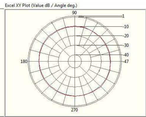
2.485GHz@Theta 0.0 Total
