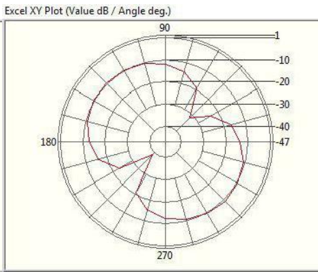
2.485GHz@Theta 0.0 Vertical
