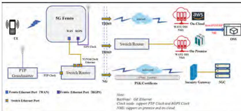
Figure 1. 5G Femtocell Network Diagram
