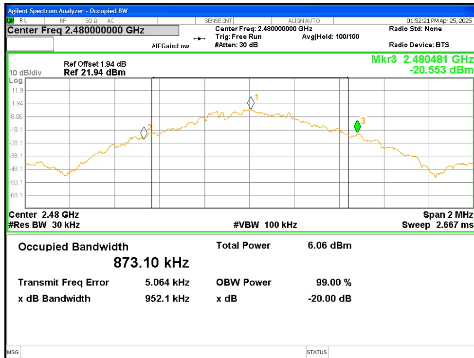
-20dB Bandwidth NVNT 1-DH5 2480MHz
