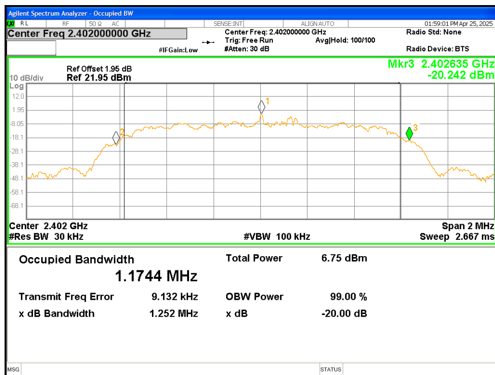
-20dB Bandwidth NVNT 2-DH5 2402MHz
