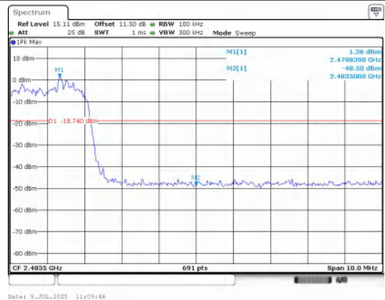
Out Of Band Emission(Right) π/4DQPSK_2-DH5_Channel Hopping
