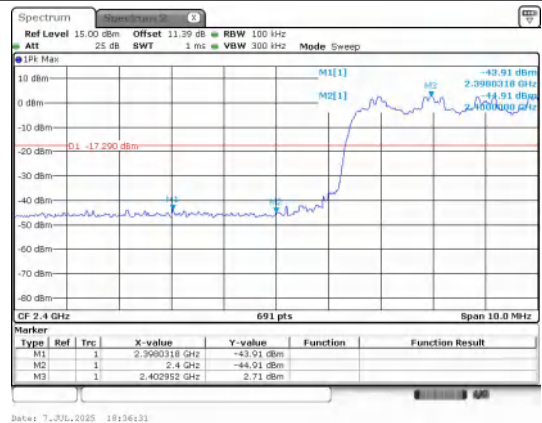
Out Of Band Emission(Left) π/4DQPSK_2-DH5_Channel Hopping
