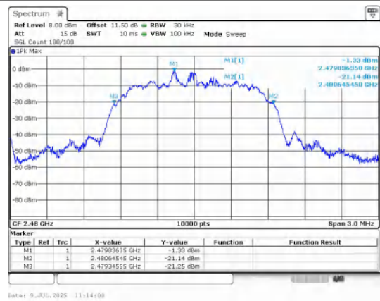
\pi/4 DQPSK_2-DH5_Channel 78
