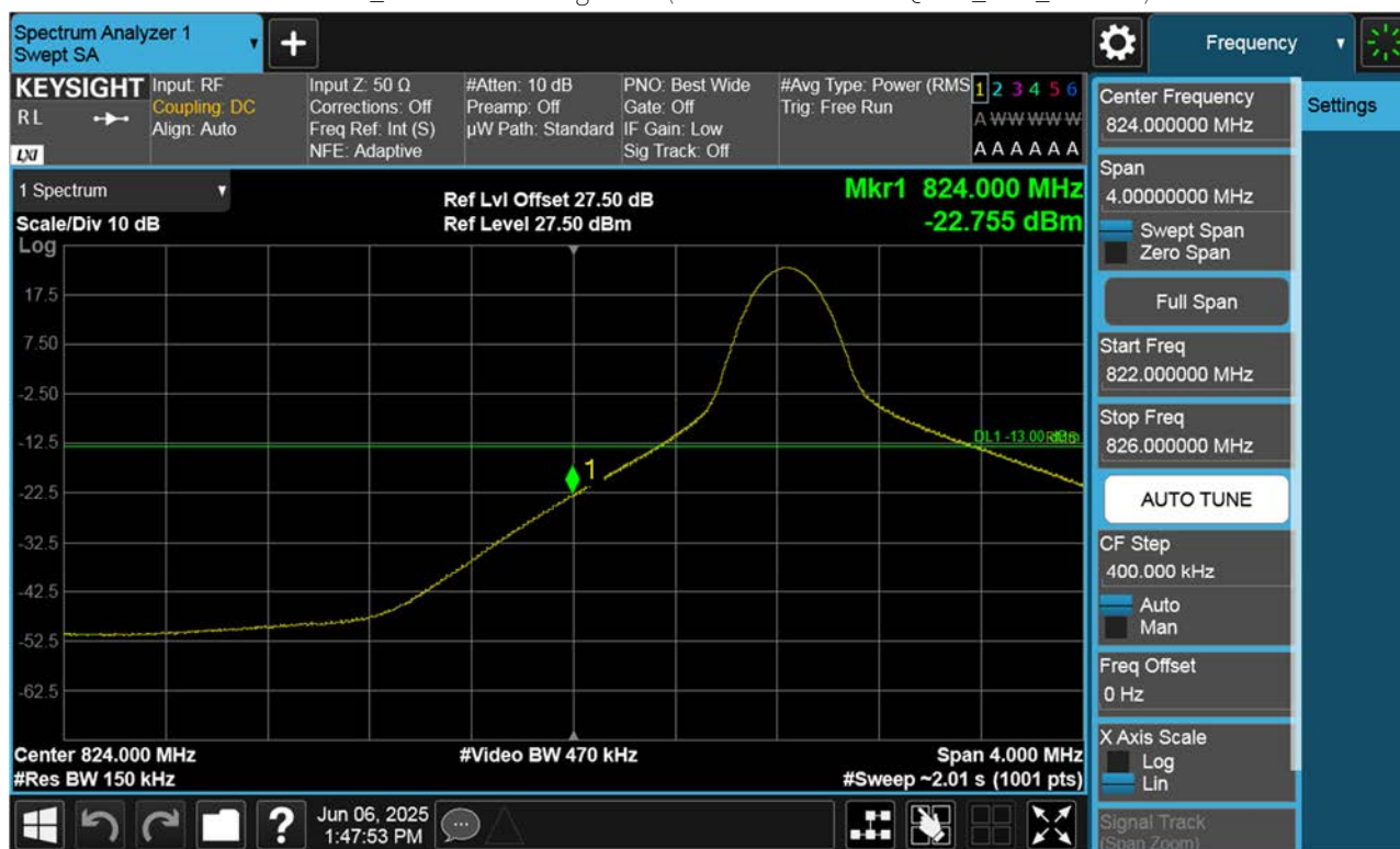
LTE B26_ Lower Band Edge Plot (15 M BW Ch.26865 QPSK_RB1_Offset 0)
