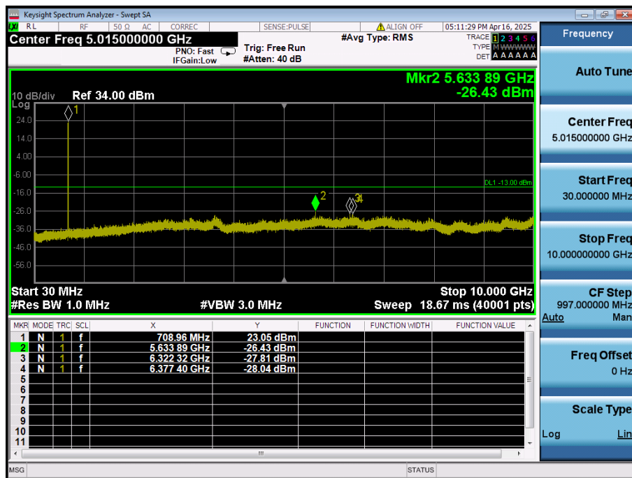
LTE Band 12 / 3MHz / QPSK - RB Size/Offset (15/0) - Mid Channel
