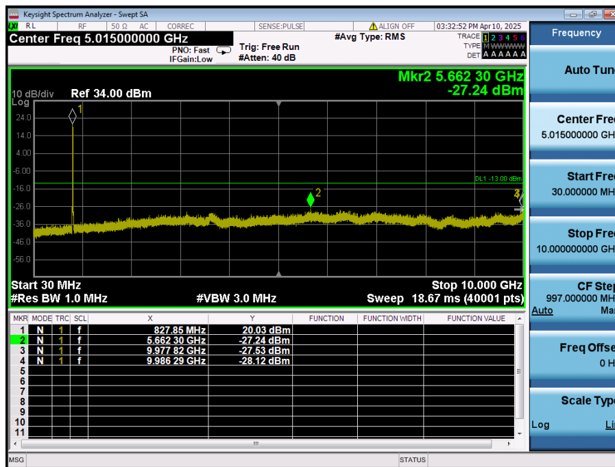
LTE Band 5 / 10MHz / QPSK - RB Size/Offset (50/0) - Low Channel
