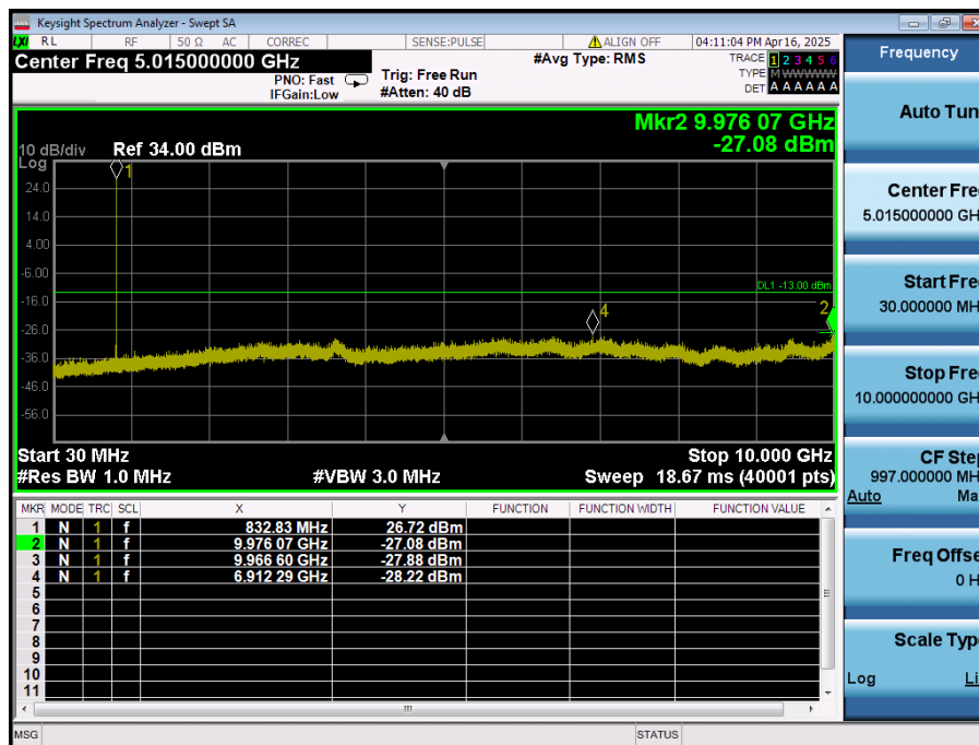
LTE Band 5 / 10MHz / 64QAM - RB Size/Offset (1/0) - Mid Channel
