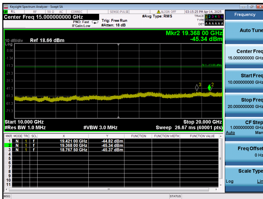
LTE Band 2 / 10MHz / 64QAM - RB Size/Offset (1/25) - High Channel
