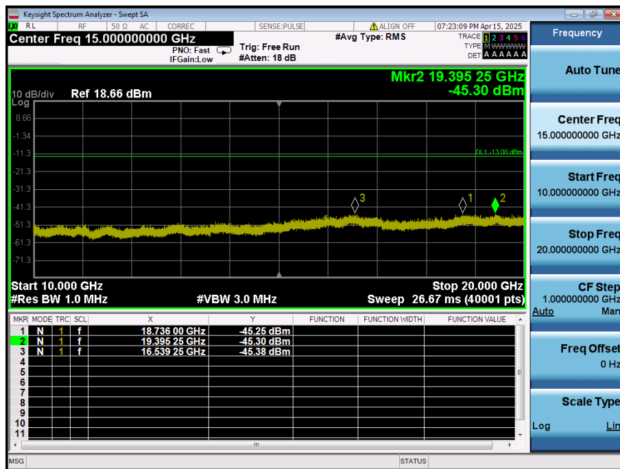
LTE Band 2 / 3MHz / QPSK - RB Size/Offset (1/14) - Mid Channel
