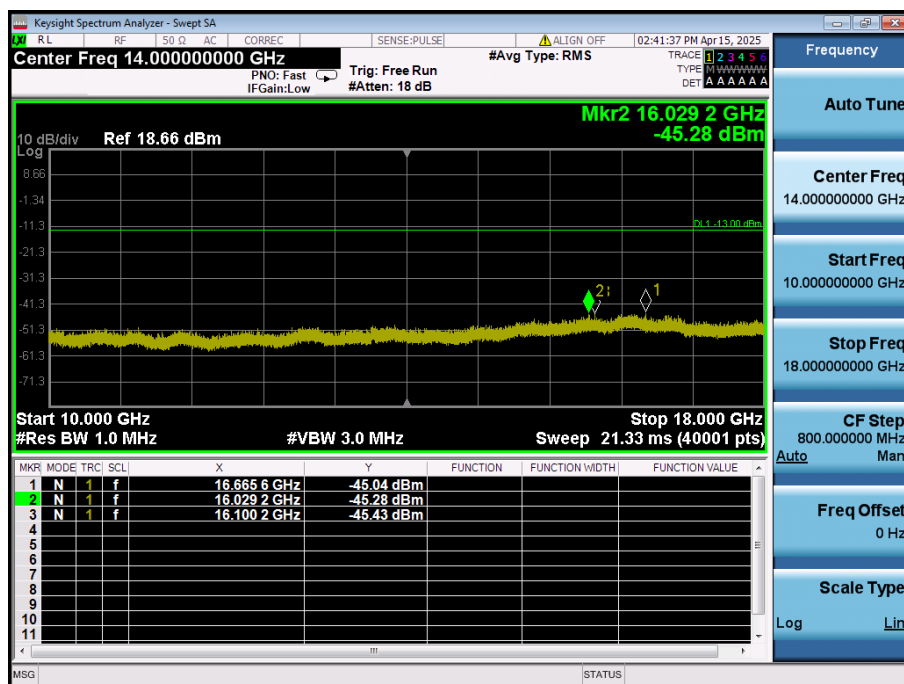
LTE Band 66 / 1.4MHz / 64QAM - RB Size/Offset (1/0) - Low Channel
