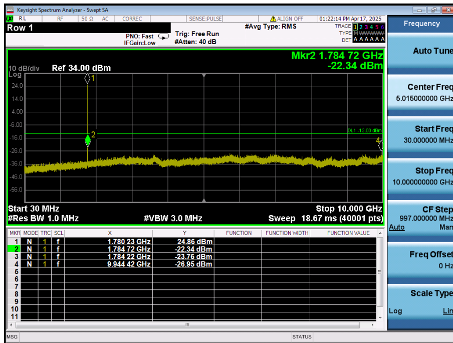
LTE Band 66 / 1.4MHz / QPSK - RB Size/Offset (6/0) - High Channel
