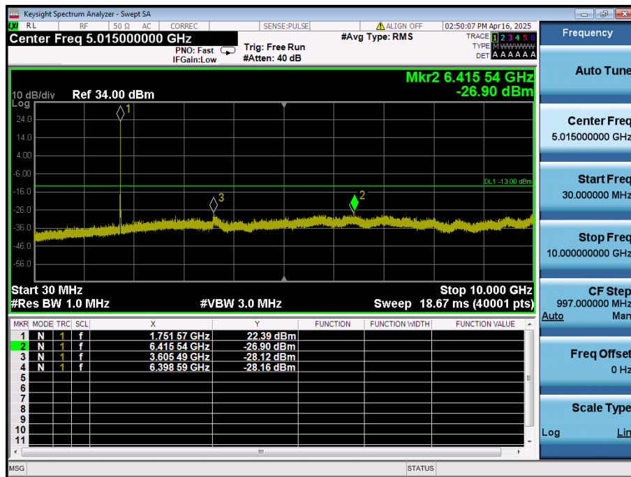
LTE Band 66 / 3MHz / 64QAM - RB Size/Offset (15/0) - Mid Channel
