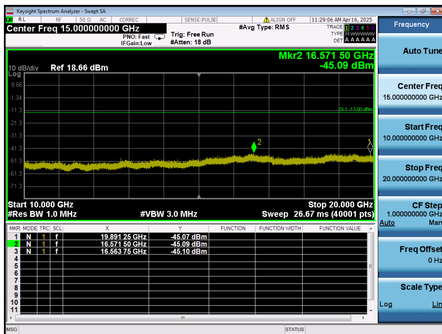
LTE Band 2 / 1.4MHz / 64QAM - RB Size/Offset (1/0) - Mid Channel
