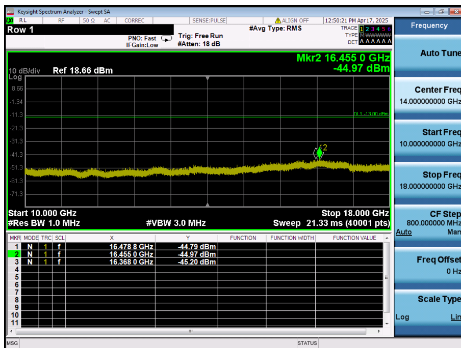
LTE Band 66 / 5MHz / 64QAM - RB Size/Offset (25/0) - High Channel
