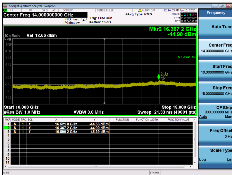
LTE Band 66 / 3MHz / 16QAM - RB Size/Offset (25/0) - Low Channel
