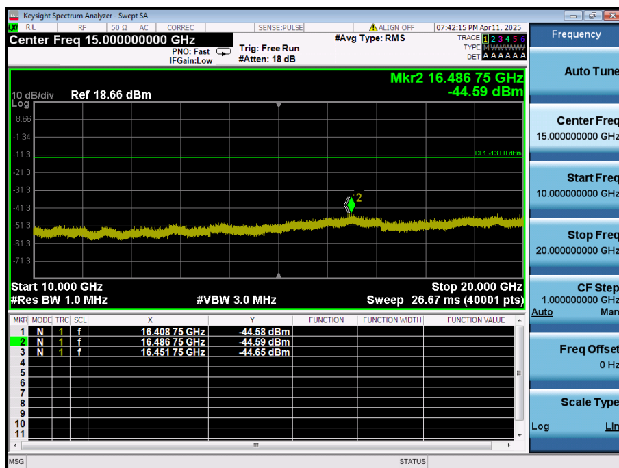
LTE Band 2 / 15MHz / QPSK - RB Size/Offset (1/0) - High Channel
