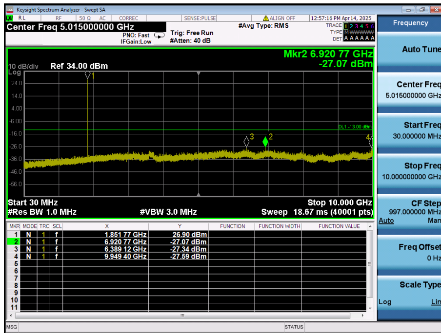
LTE Band 2 / 1.4MHz / 16QAM - RB Size/Offset (1/5) - Low Channel
