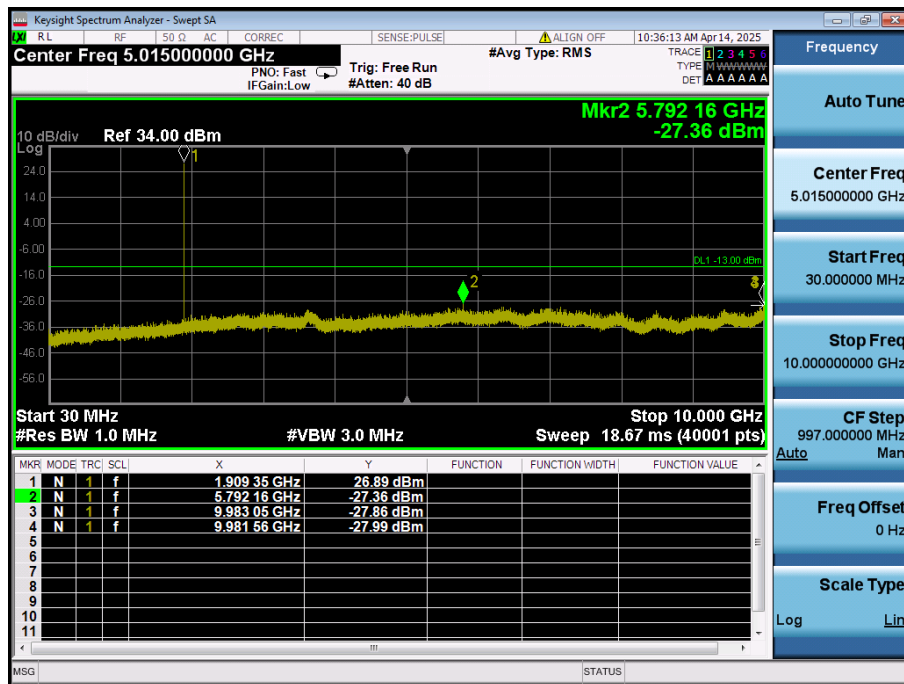
LTE Band 2 / 3MHz / QPSK - RB Size/Offset (1/7) - High Channel
