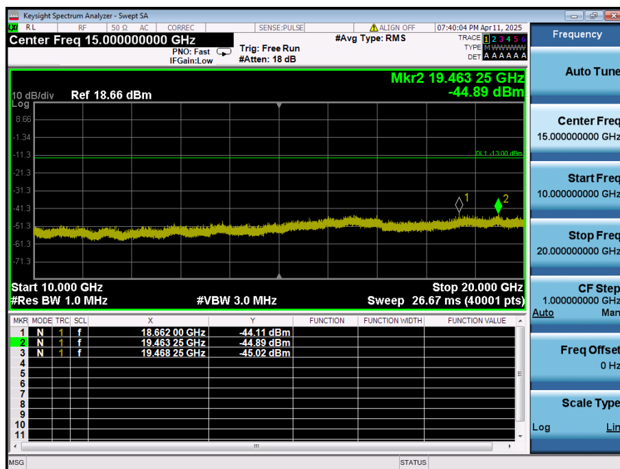
LTE Band 2 / 15MHz / QPSK - RB Size/Offset (75/0) - Low Channel
