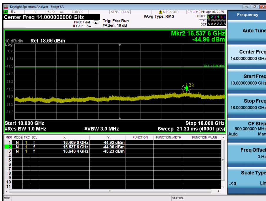
LTE Band 66 / 1.4MHz / 16QAM - RB Size/Offset (6/0) - Mid Channel
