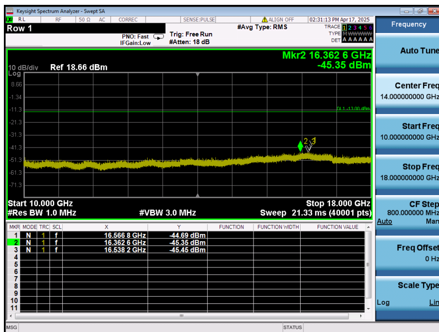
LTE Band 66 / 3MHz / 16QAM - RB Size/Offset (15/0) - High Channel
