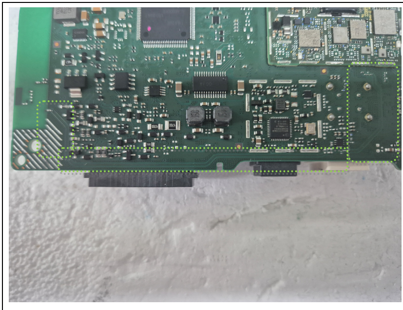
ANT 2 trace path (Bottom)
