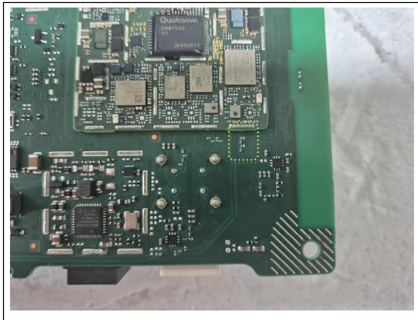
ANT 1 trace path (Bottom)
