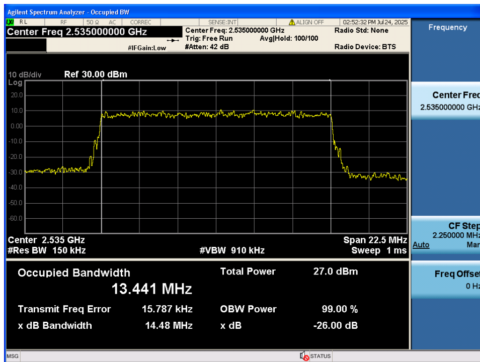
LTE Band 7 / 15MHz / 16QAM - RB Size 75/0
