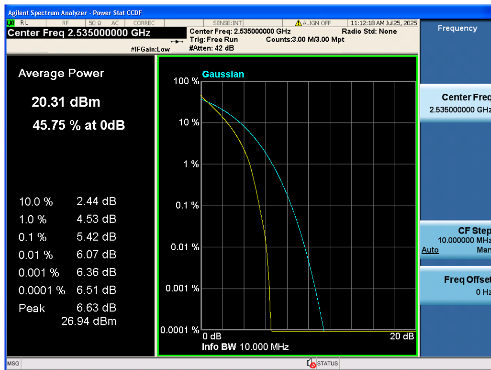
LTE Band 7 / 10MHz / QPSK - RB Size 50/0
