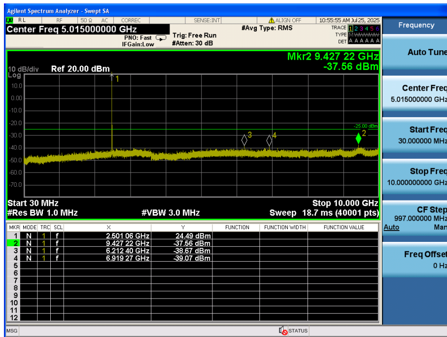
LTE Band 7 / 15MHz / QPSK - RB Size/Offset (1/0) - Low Channel
