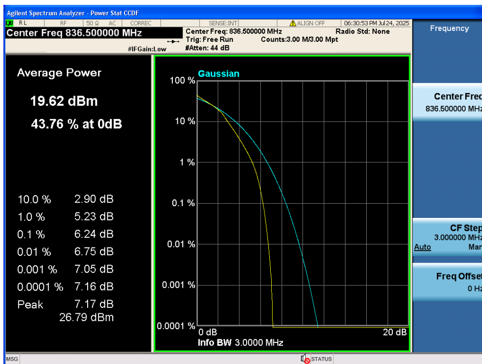
LTE Band 5 / 3MHz / 16QAM - RB Size 15/0
