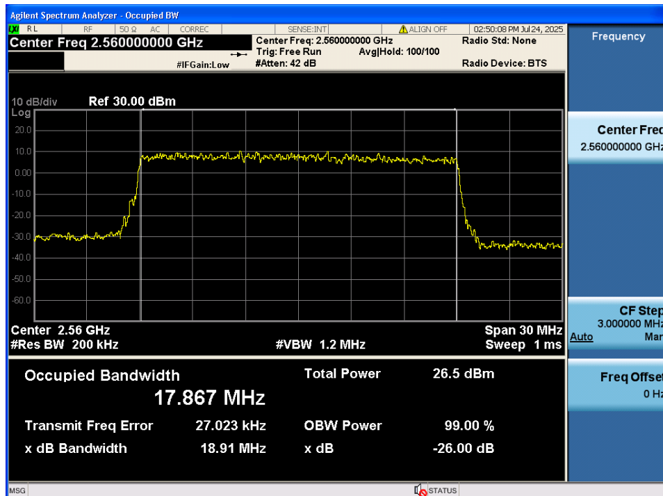
LTE Band 7 / 20MHz / 16QAM - RB Size 100/0
