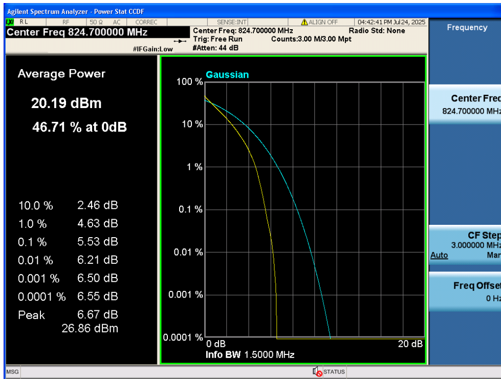
LTE Band 5 / 1.4MHz / QPSK - RB Size 6/0
