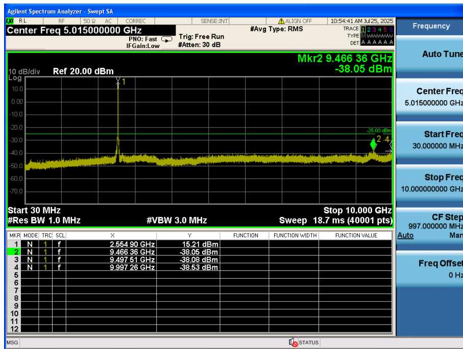
LTE Band 7 / 20MHz / QPSK - RB Size/Offset (100/0) - High Channel
