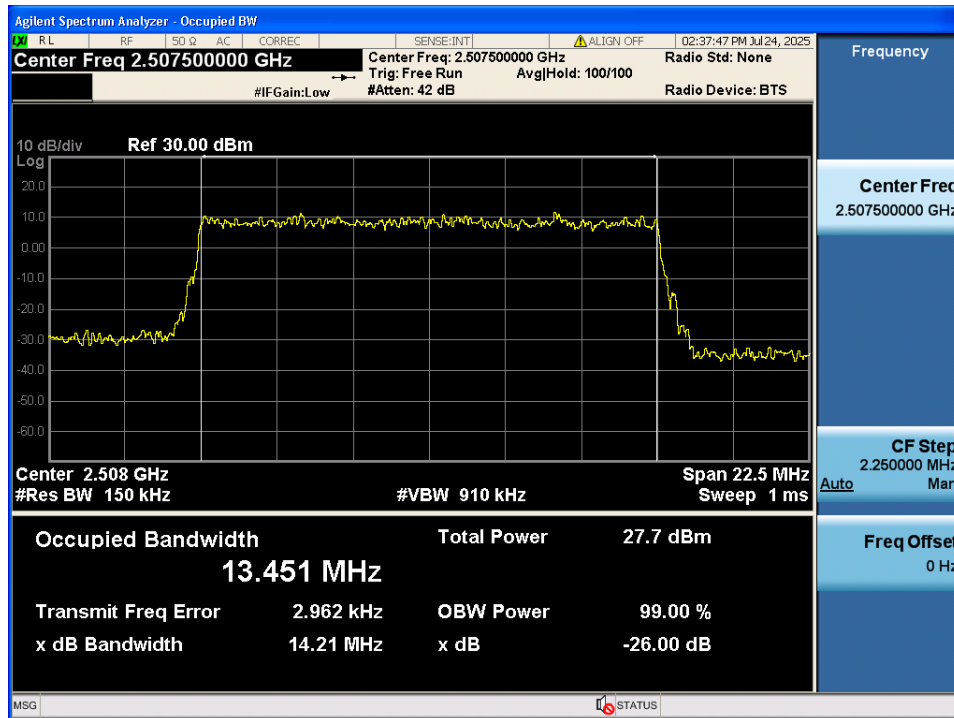
LTE Band 7 / 15MHz / QPSK - RB Size 75/0
