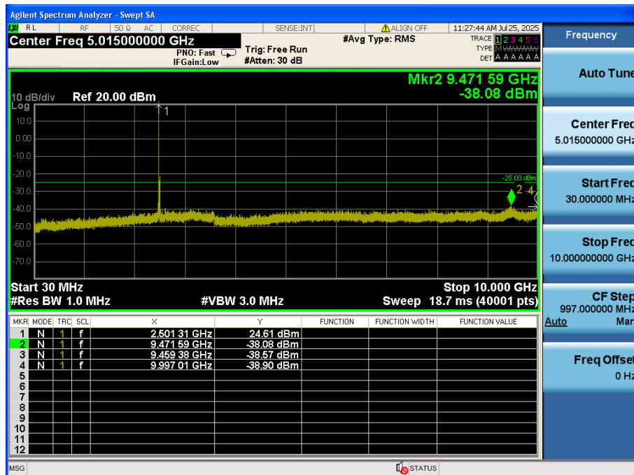
LTE Band 7 / 20MHz / 16QAM - RB Size/Offset (1/0) - Low Channel
