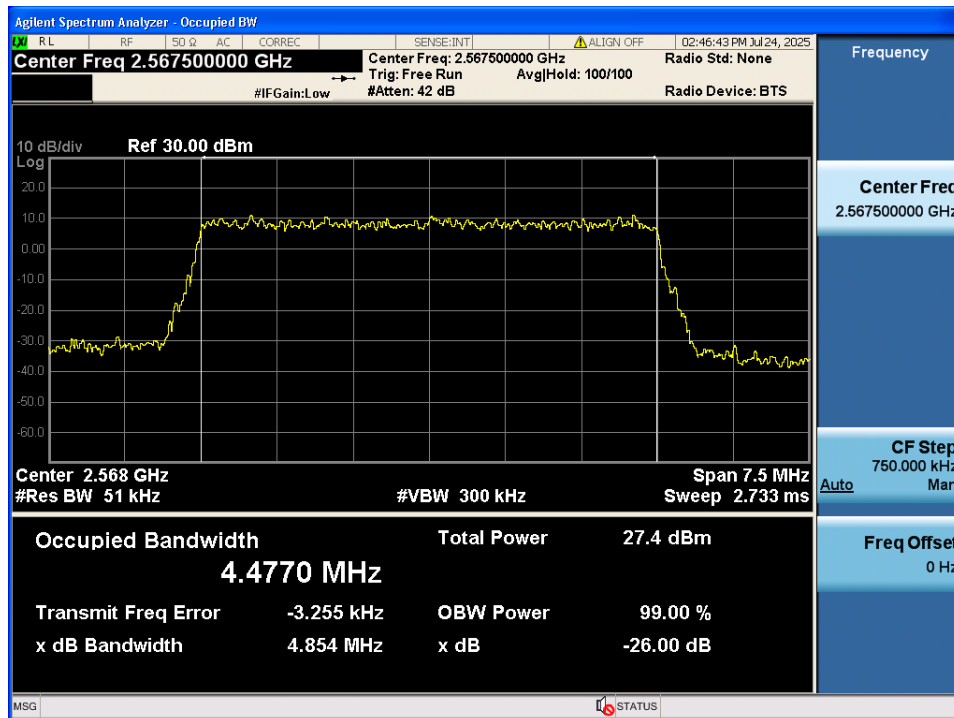
LTE Band 7 / 5MHz / QPSK - RB Size 25/0
