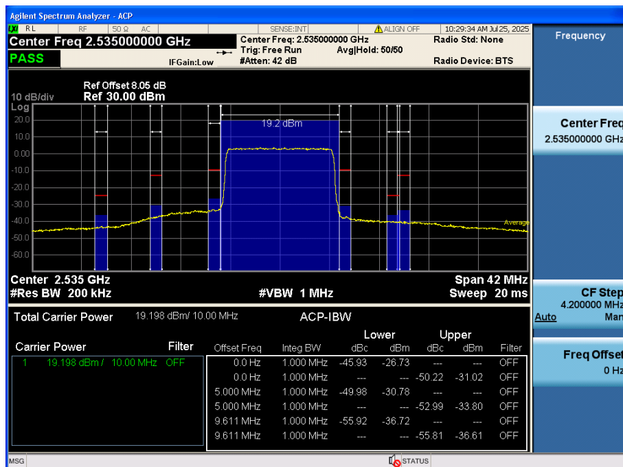
LTE Band 7 / 10MHz / 16QAM - RB Size/Offset (Full RB)
