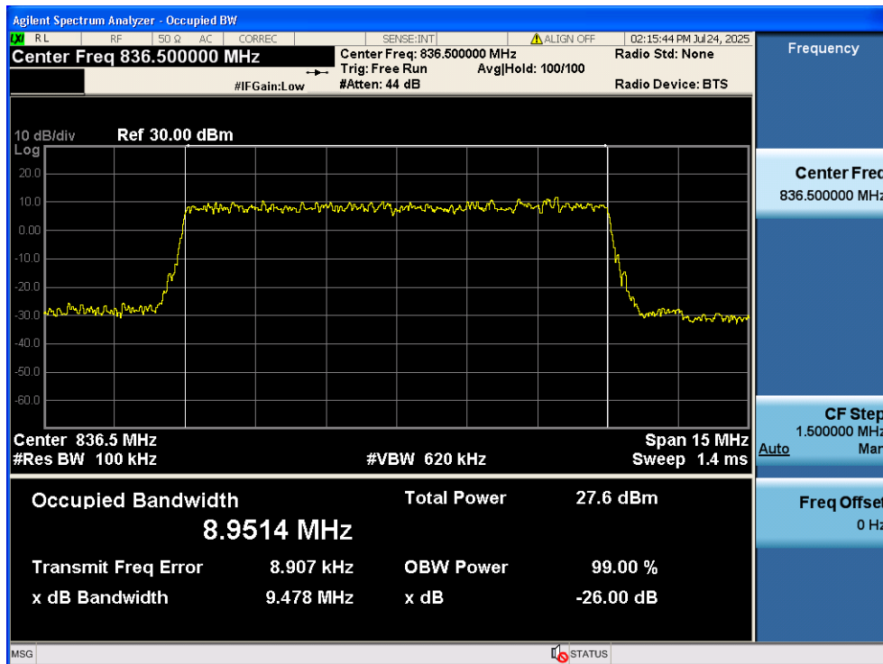
LTE Band 5 / 10MHz / 16QAM - RB Size 50/0
