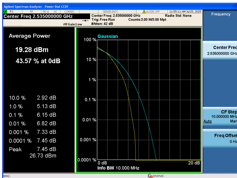
LTE Band 7 / 10MHz / 16QAM - RB Size 50/0
