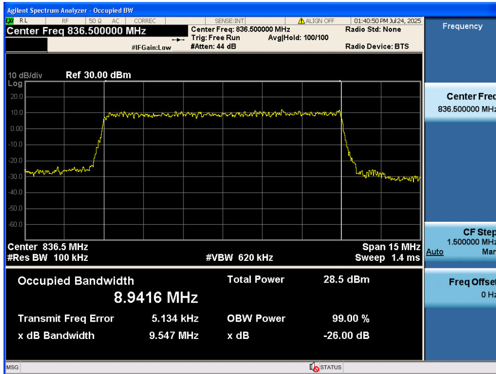
LTE Band 5 / 10MHz / QPSK - RB Size 50/0
