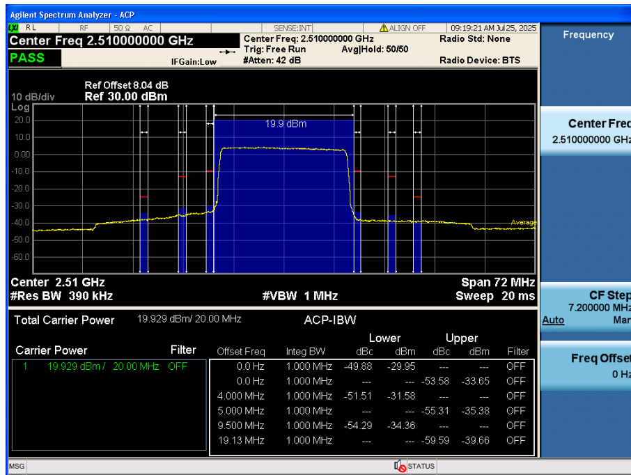
LTE Band 7 / 20MHz / QPSK - RB Size/Offset (Full RB)
