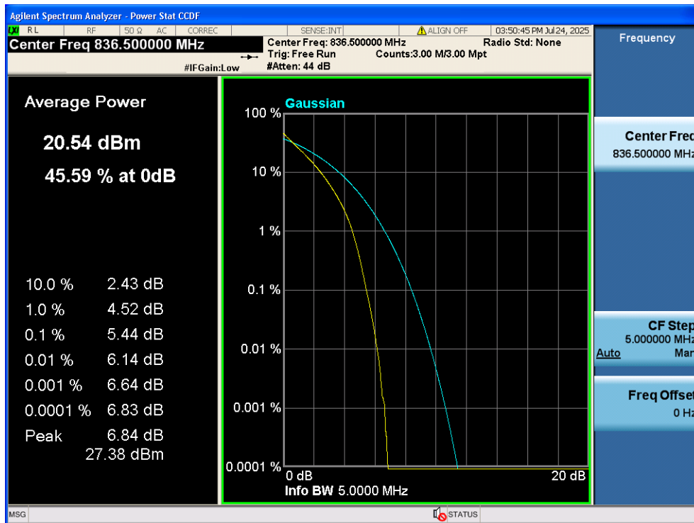
LTE Band 5 / 5MHz / QPSK - RB Size 25/0
