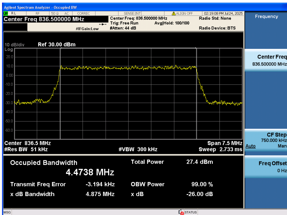
LTE Band 5 / 5MHz / 16QAM - RB Size 25/0
