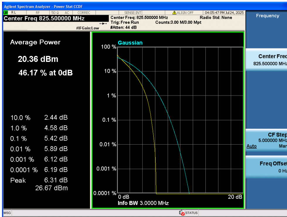
LTE Band 5 / 3MHz / QPSK - RB Size 15/0
