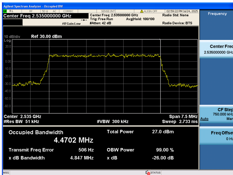
LTE Band 7 / 5MHz / 16QAM - RB Size 25/0
