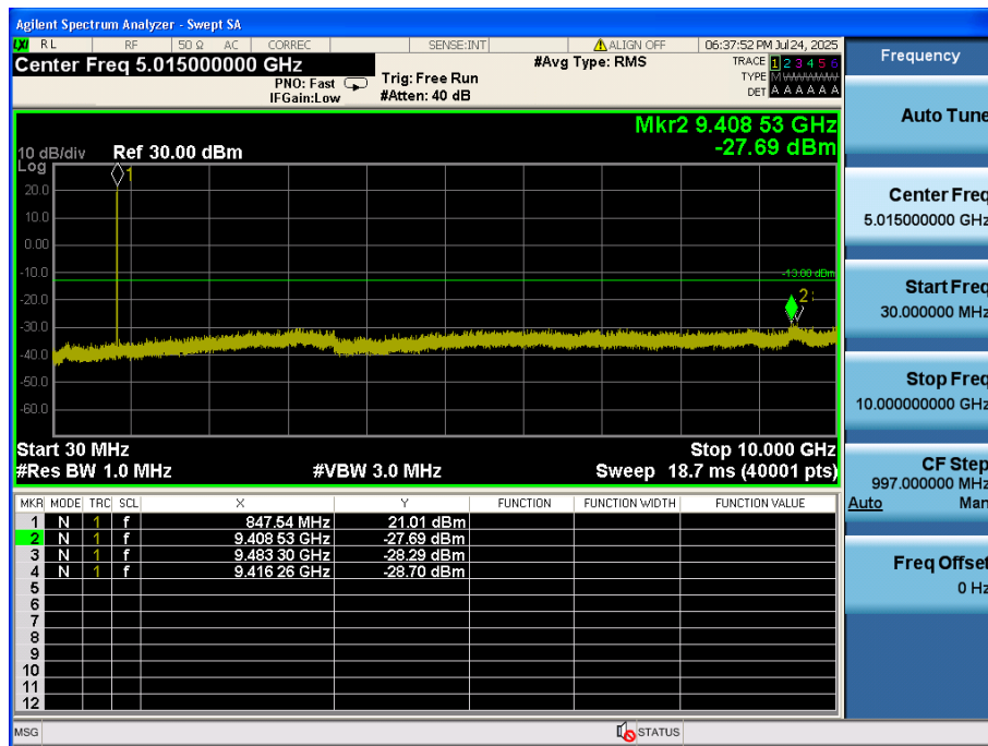
LTE Band 5 / 3MHz / 16QAM - RB Size/Offset (15/0) - High Channel
