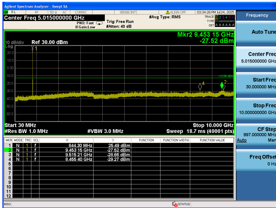
LTE Band 5 / 10MHz / QPSK - RB Size/Offset (1/25) - High Channel
