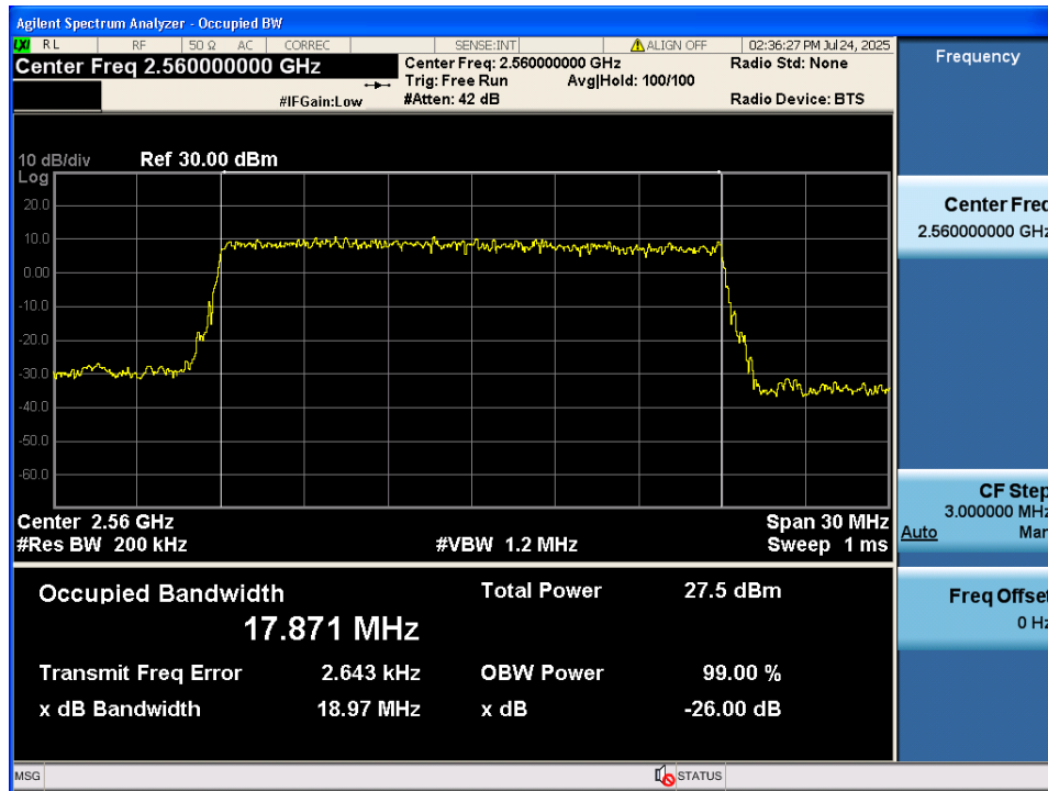
LTE Band 7 / 20MHz / QPSK - RB Size 100/0
