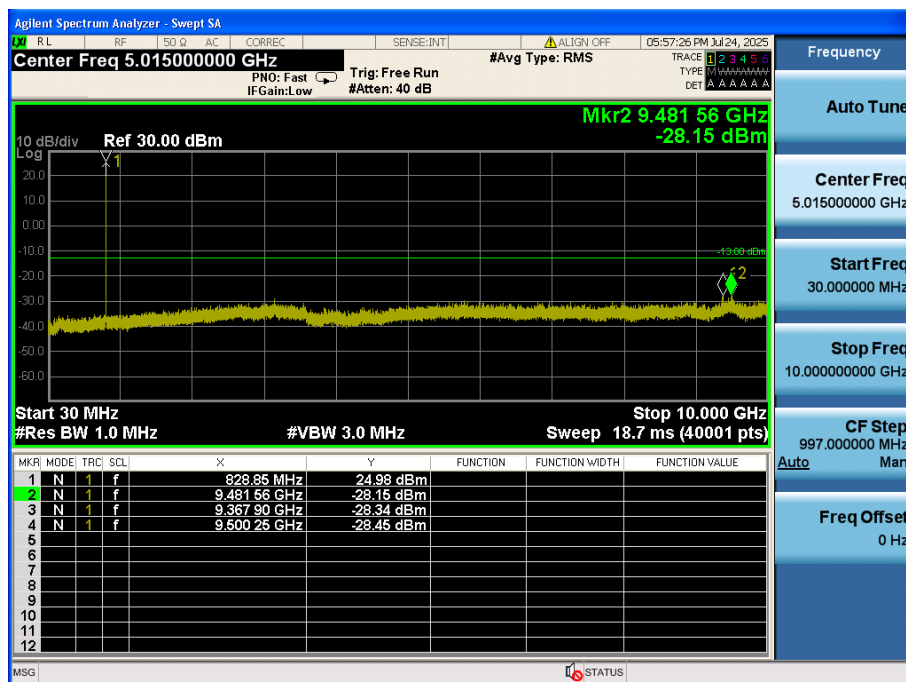
LTE Band 5 / 5MHz / 16QAM - RB Size/Offset (25/0) - Low Channel
