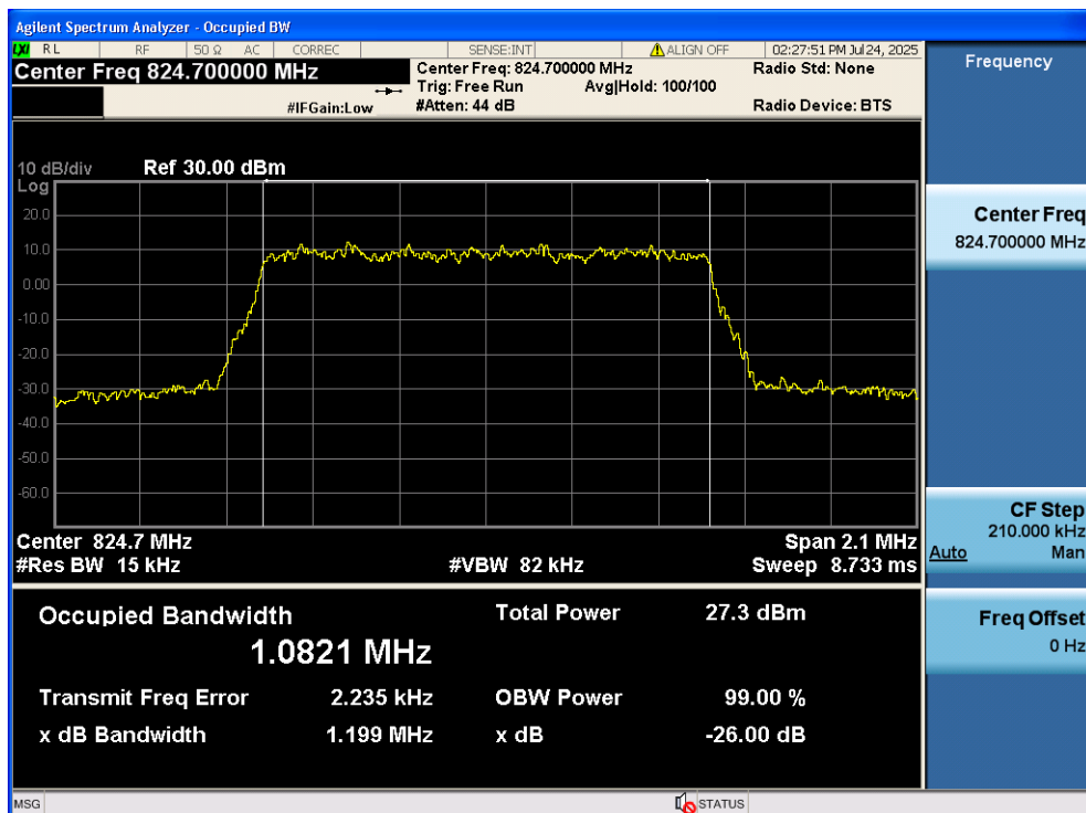
LTE Band 5 / 1.4MHz / 16QAM - RB Size 6/0
