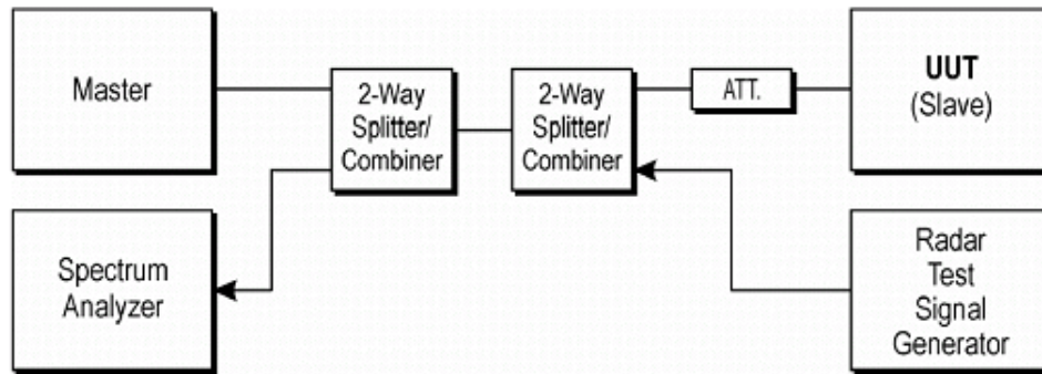
Figure 7-1. Test Setup
