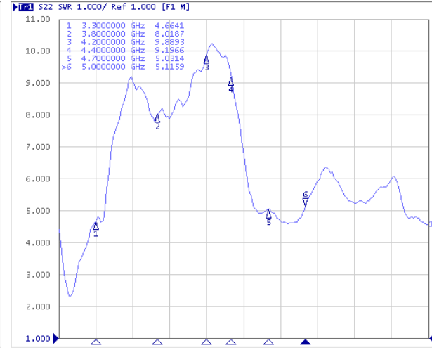
VSWR _ High
