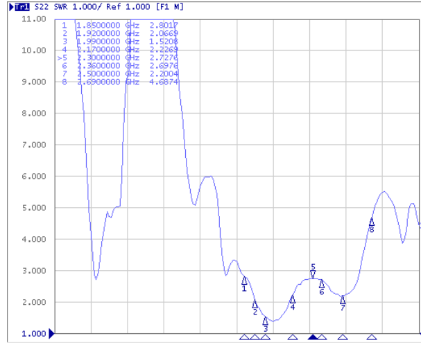
VSWR _ Middle
