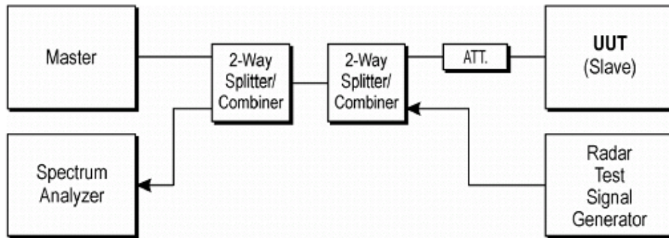
Figure 7-1. Test Setup
