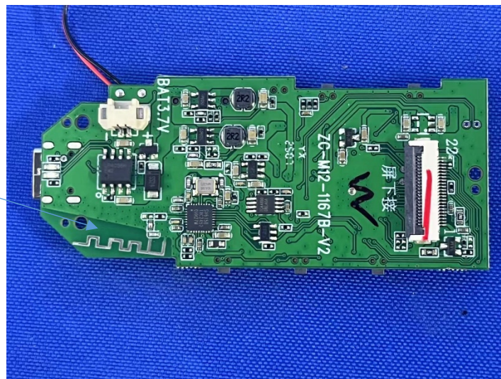
WIFI Antenna
