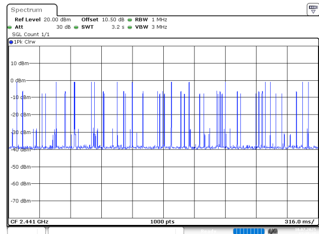
2EDR_DH3_Hopping, Total Hops=14*10=140
