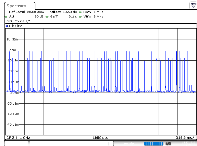
BDR_DH1_Hopping, Total Hops=32*10=320
