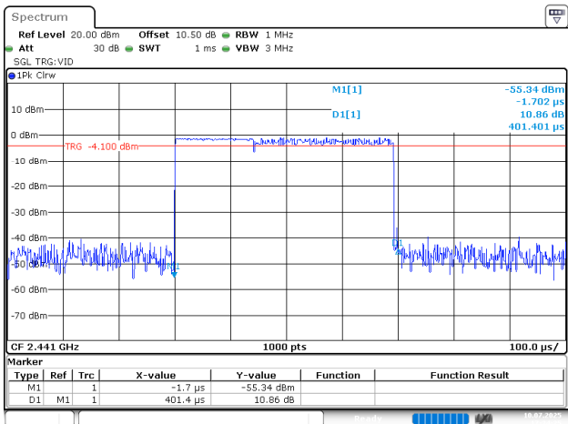
2EDR_DH1_Hopping, Burst Width=0.401ms
