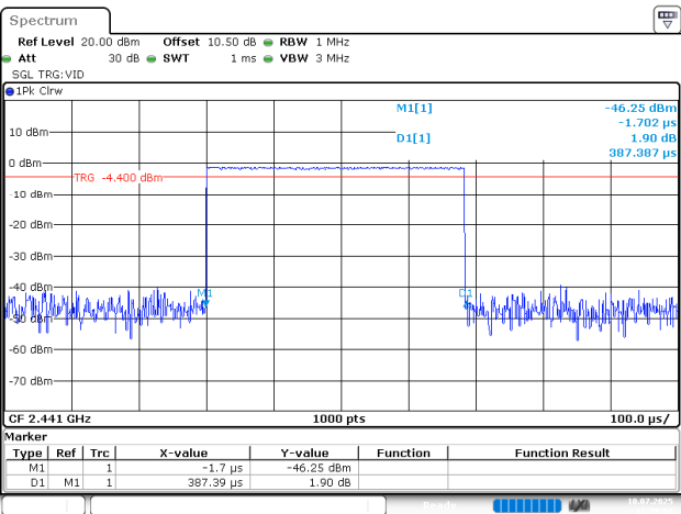
BDR_DH1_Hopping, Burst Width=0.387ms
