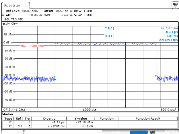
2EDR_DH5_Hopping, Burst Width=2.913ms
