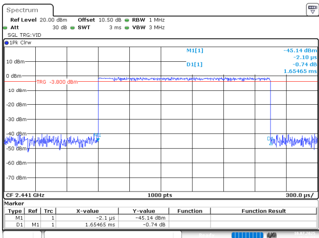
2EDR_DH3_Hopping, Burst Width=1.655ms
