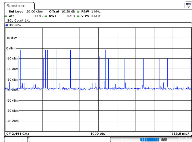
BDR_DH5_Hopping, Total Hops=9*10=90
