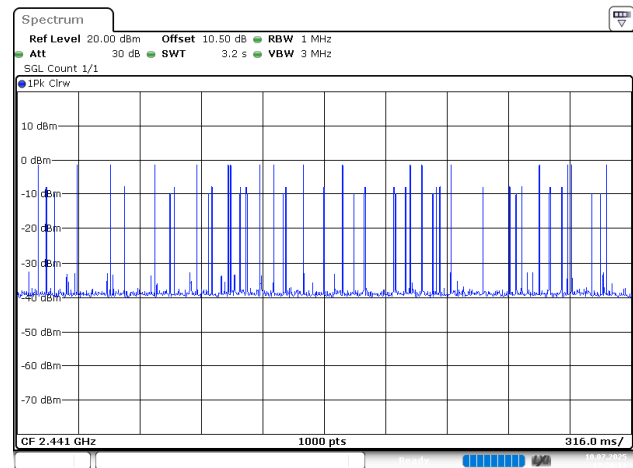
BDR_DH3_Hopping, Total Hops=18*10=180
