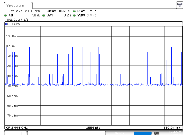
2EDR_DH5_Hopping, Total Hops=12*10=120
