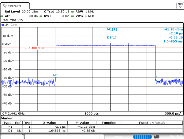
BDR_DH3_Hopping, Burst Width=1.649ms
