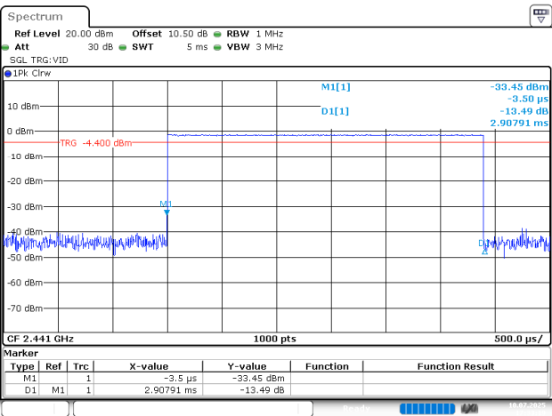
BDR_DH5_Hopping, Burst Width=2.908ms
