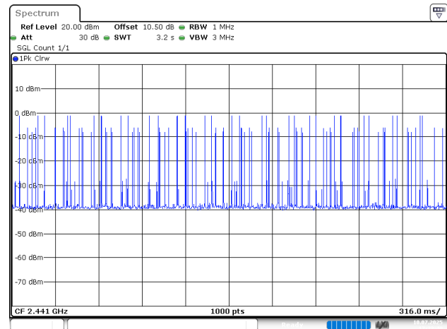
2EDR_DH1_Hopping, Total Hops=31*10=310
