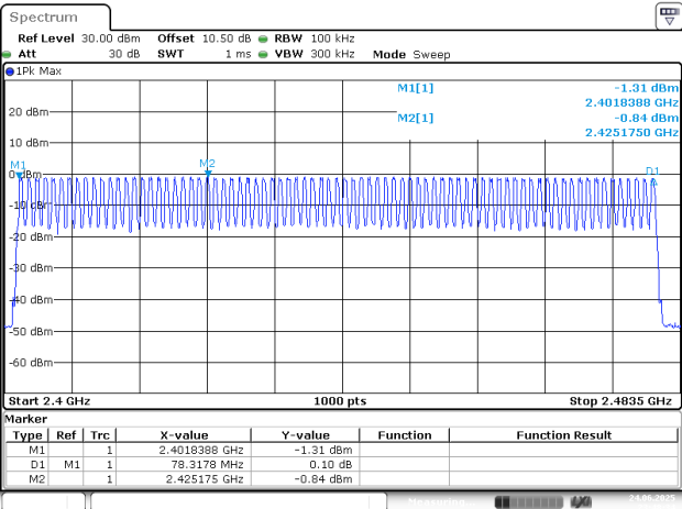
BDR_DH1_Hopping
