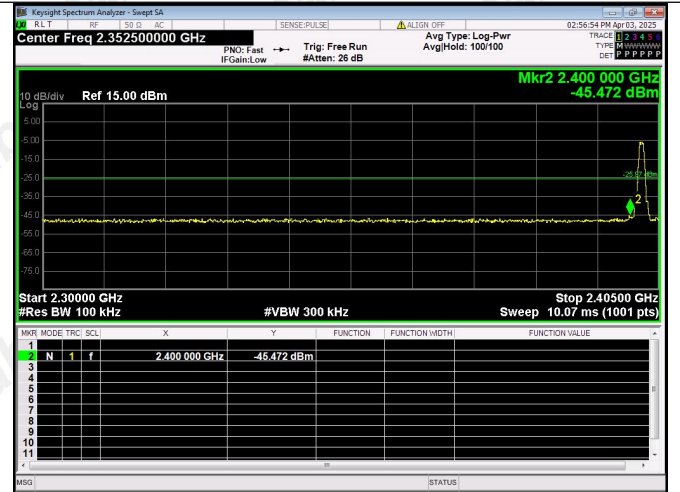
Out Of Band Emission BLE 1M_Channel 0
