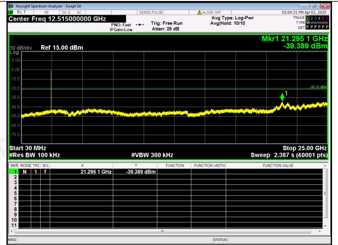
30.0 MHz - 25000.0 MHz BLE 1M_Channel 39
