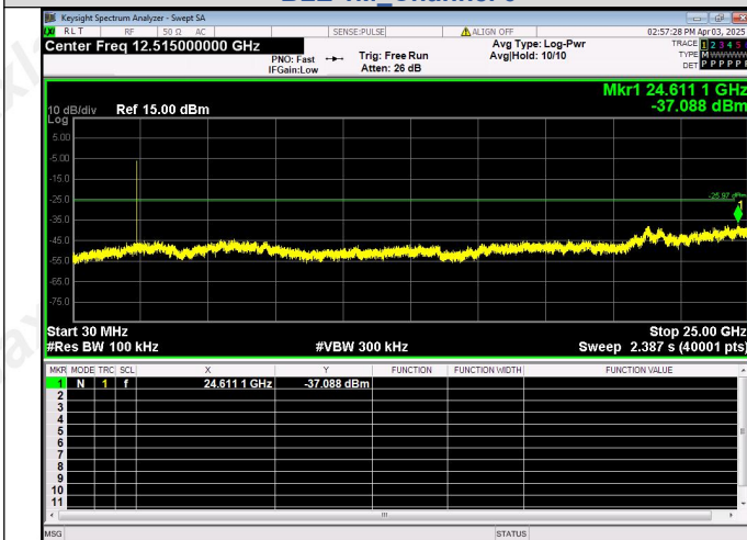
30.0 MHz - 25000.0 MHz BLE 1M_Channel 0
