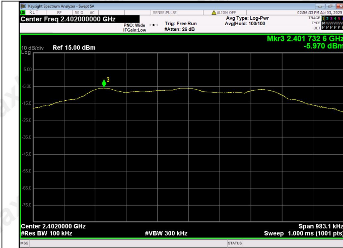
In-Band Reference Level BLE 1M_Channel 0
