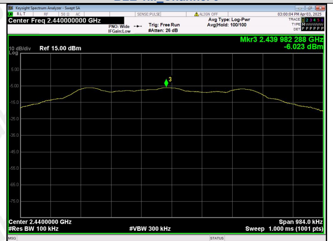
In-Band Reference Level BLE 1M_Channel 19
