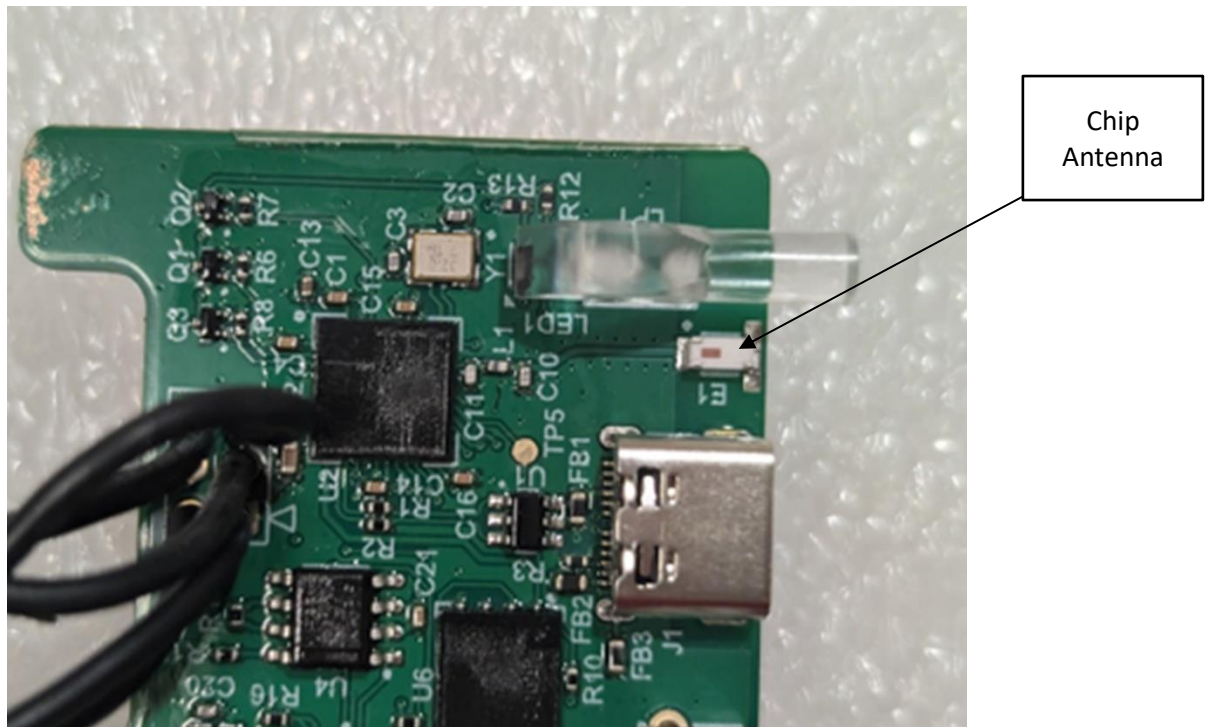
Photograph 3 – Closeup of RF Circuitry
