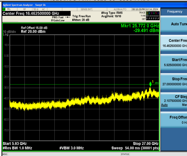
11AC20SISO-Ant1-5825-5925~27000-PASS
