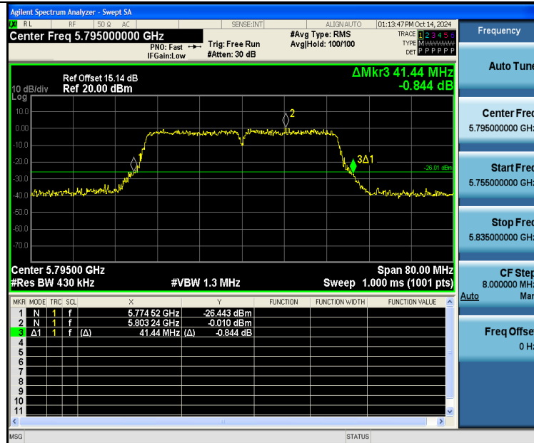
11N40SISO-Ant1-5795
