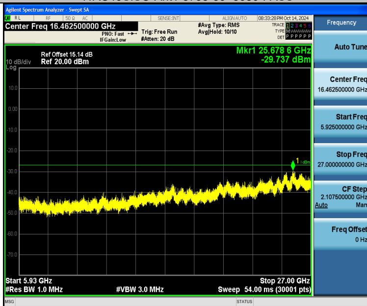
11AC40SISO-Ant1-5795-5925~27000-PASS
