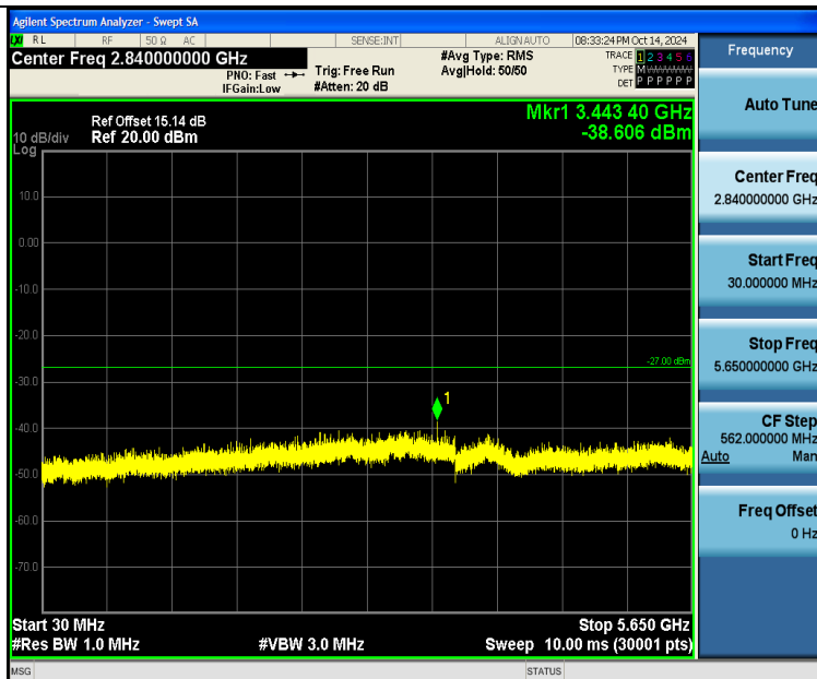
11AC40SISO-Ant1-5795-30~5650-PASS
