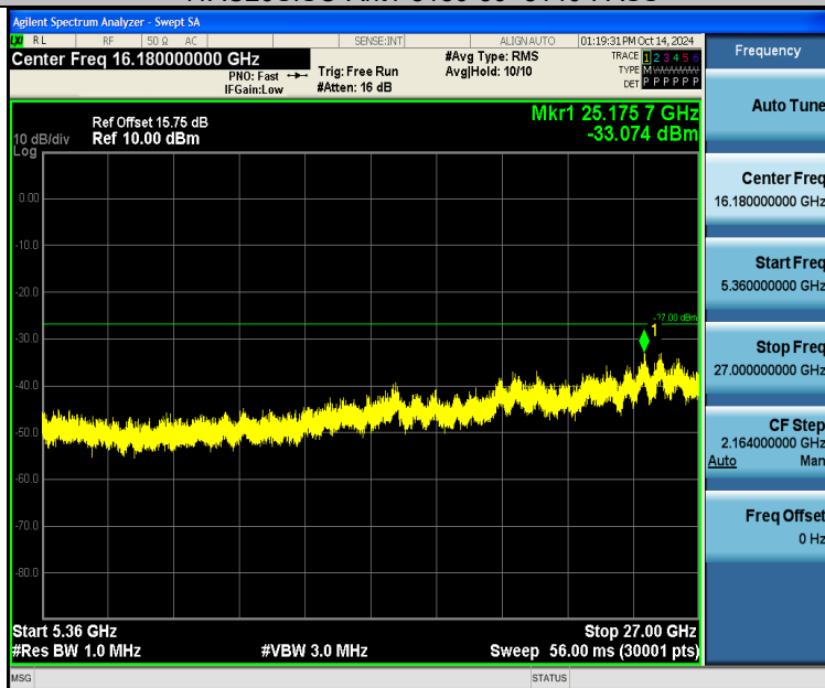
11AC20SISO-Ant1-5180-5360~27000-PASS
