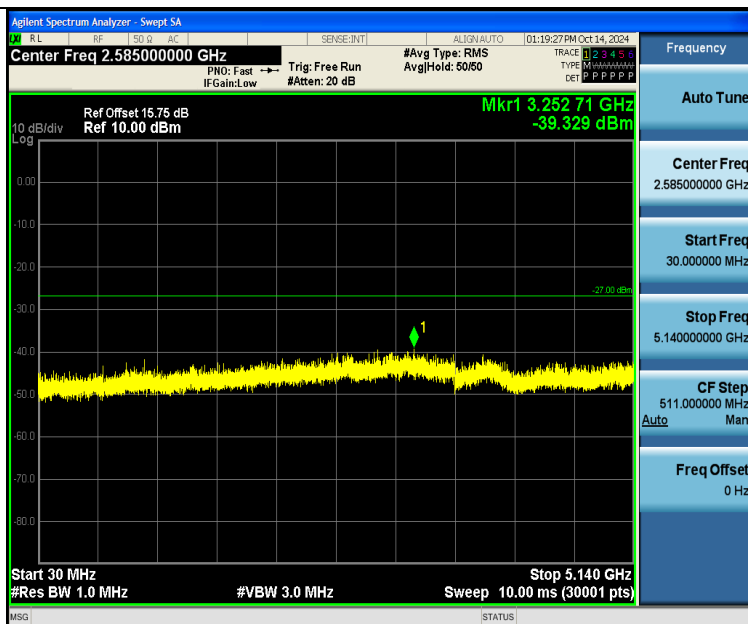
11AC20SISO-Ant1-5180-30~5140-PASS
