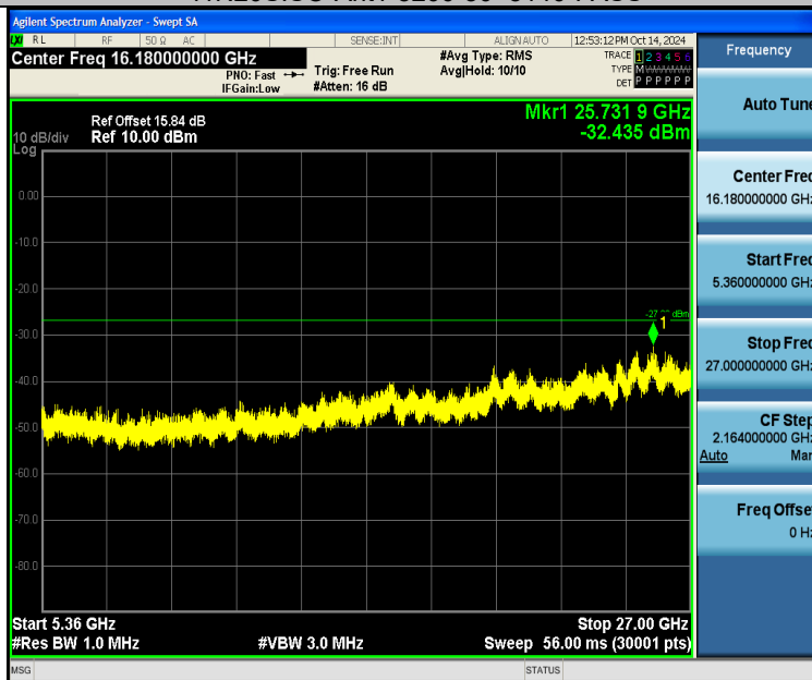
11N20SISO-Ant1-5200-5360~27000-PASS
