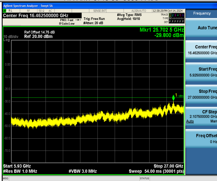
11A-Ant1-5745-5925~27000-PASS
