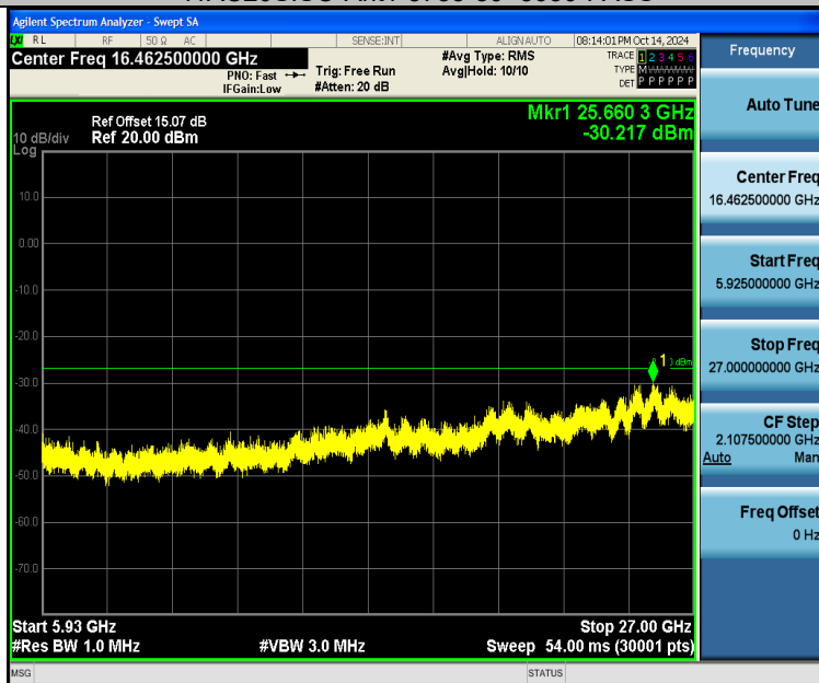
11AC20SISO-Ant1-5785-5925~27000-PASS
