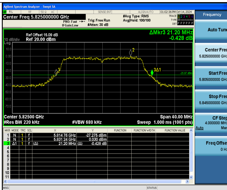
11N20SISO-Ant1-5825
