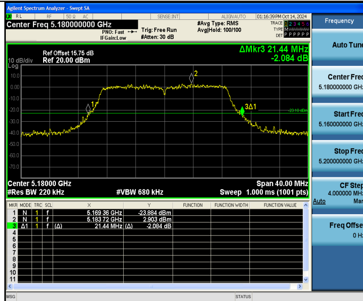
11AC20SISO-Ant1-5180
