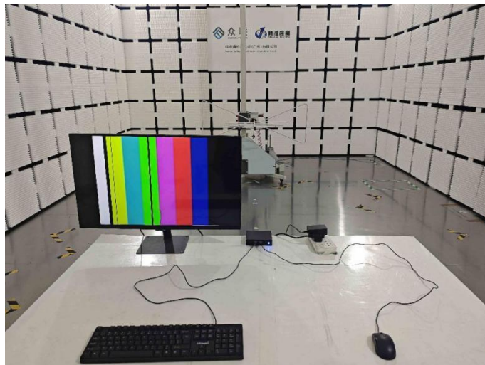
Radiated Emissions From 30M-1GHz
