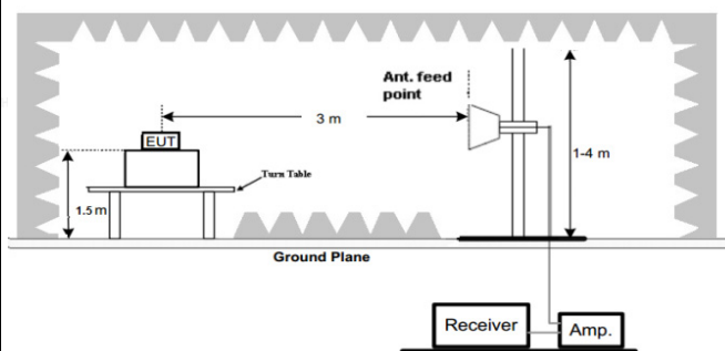
Above 1GHz
