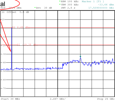
Mode: channel 19
