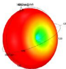
Gain Plot 1
