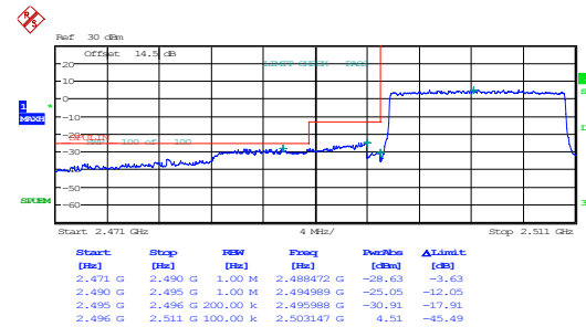
15MHz_Low_QPSK_75@0
