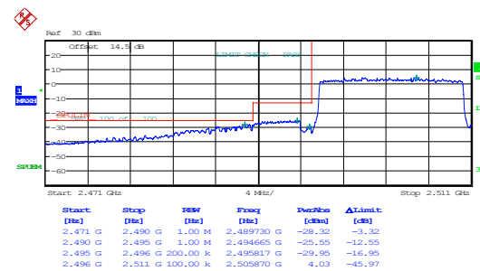
15MHz_Low_16QAM_75@0
