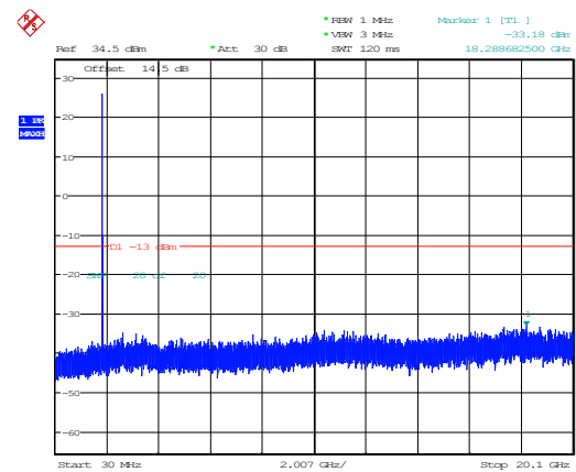
20MHz_Low_QPSK_1@0(30MHz~20.1GHz)
