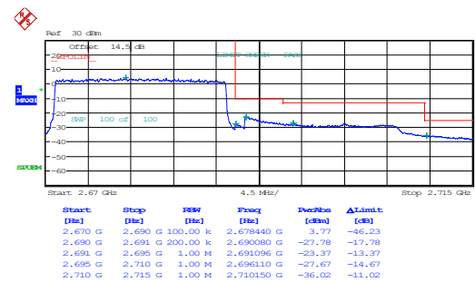
20MHz_High_QPSK_100@0
