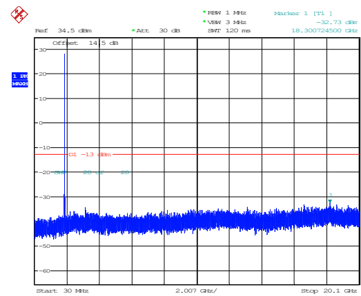
15MHz_Middle_QPSK_1@0(30MHz~20.1GHz)
