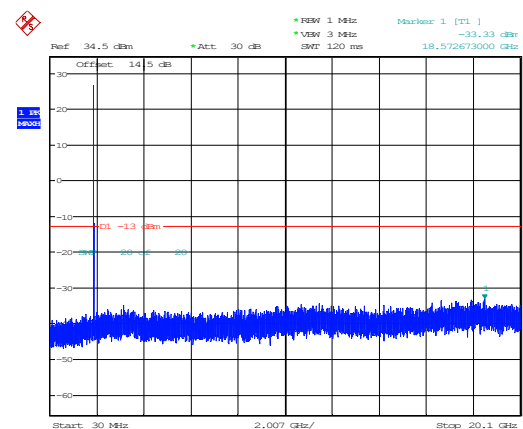
20MHz_High_QPSK_1@0(30MHz~20.1GHz)
