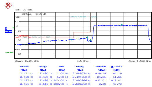
20MHz_Low_16QAM_100@0
