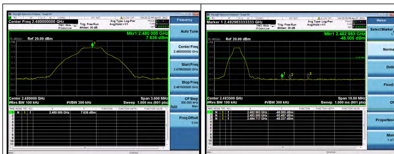
Bluetooth For Classic 1-DH5
