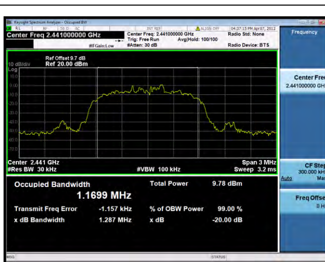
Bluetooth For Classic 3-DH5 2441MHz
