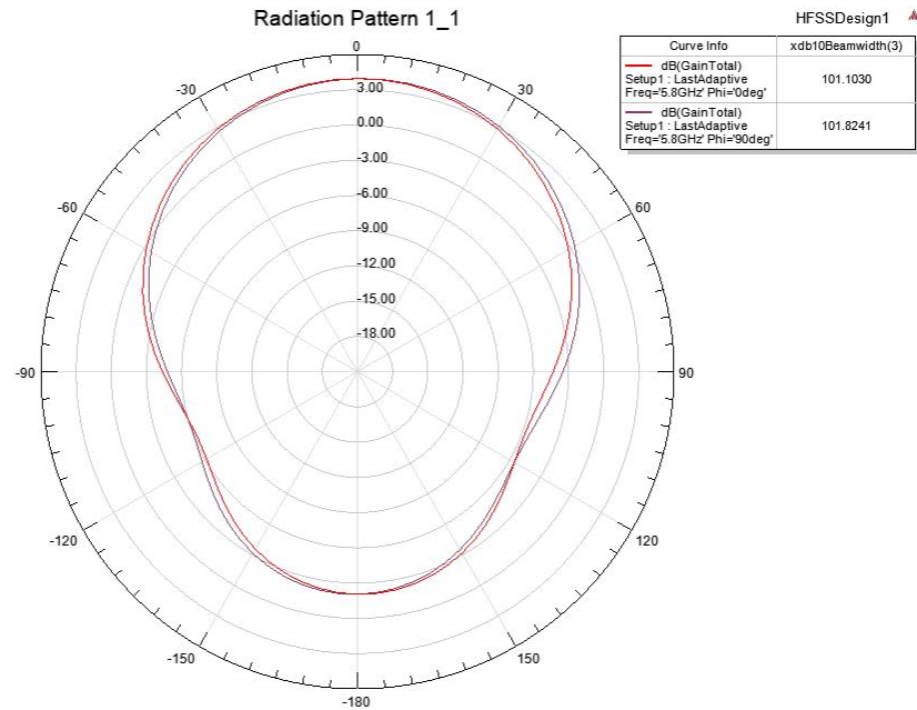
2D Radiation pattern
