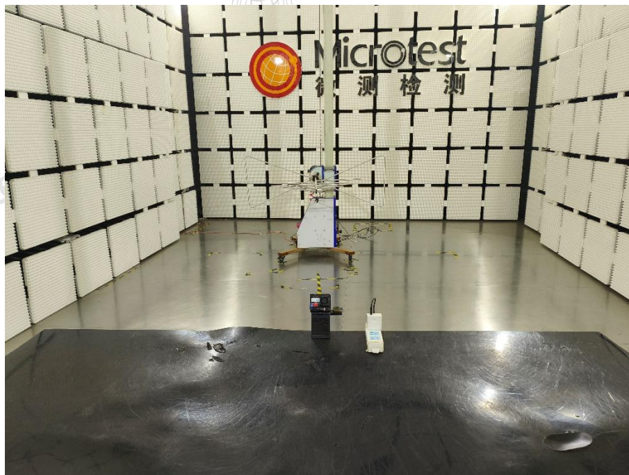
Radiated emissions (above 30MHz) -WPT
