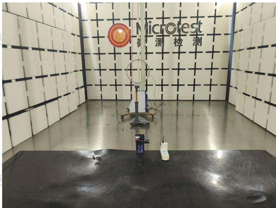
Radiated emissions (below 30MHz)- WPT
