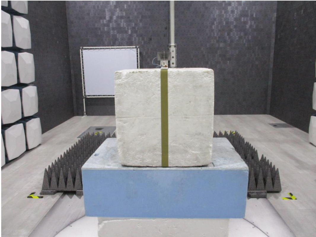
Above 1GHz
