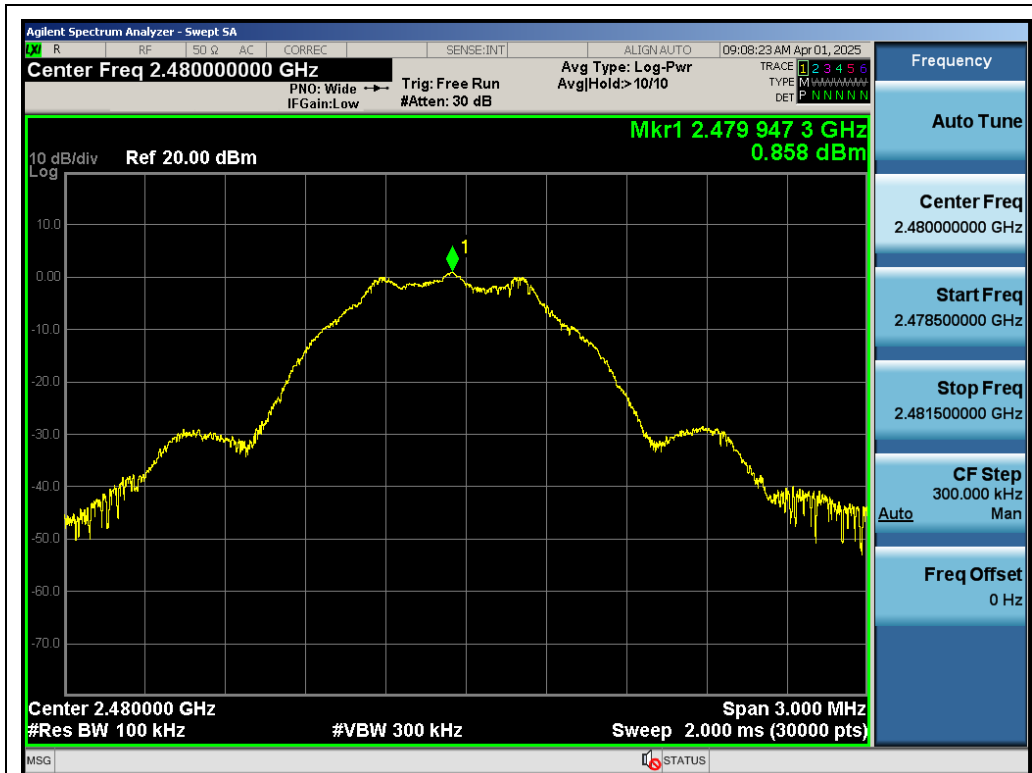
Test_Graph_LE1M_ANT1_2480_1Mbps_Reference Level
