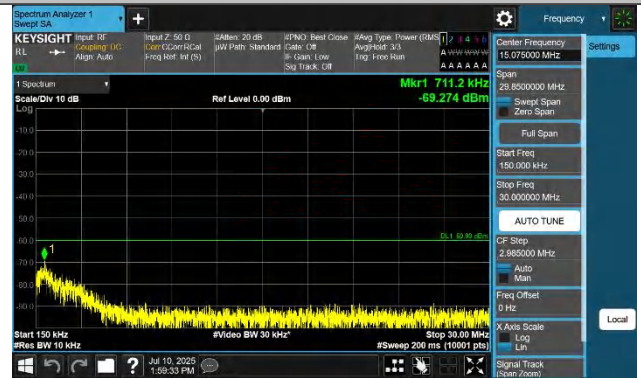
48-48-15MHz-20MHz-QPSK-QPSK-56469-56640-1RB#0-ORB#0-0 .15~30MHz-PASS
