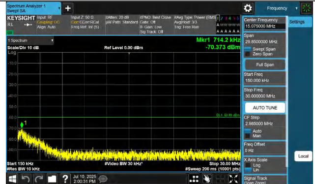
48-48-20MHz-10MHz-QPSK-QPSK-55340-55484-1RB#0-ORB#0-0 .15~30MHz-PASS
