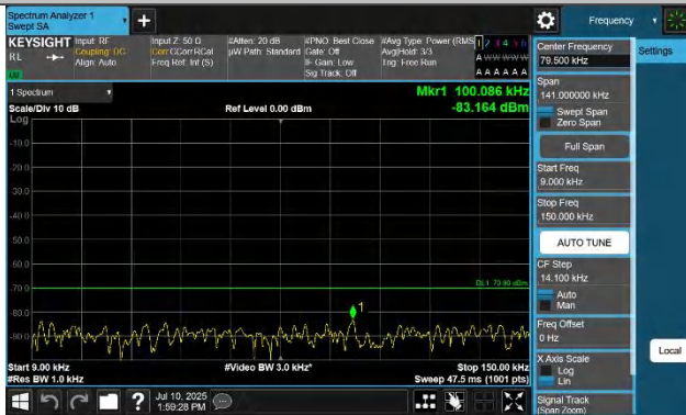
48-48-15MHz-20MHz-QPSK-QPSK-56469-56640-1RB#0-ORB#0-0 .009~0.15MHz-PASS
