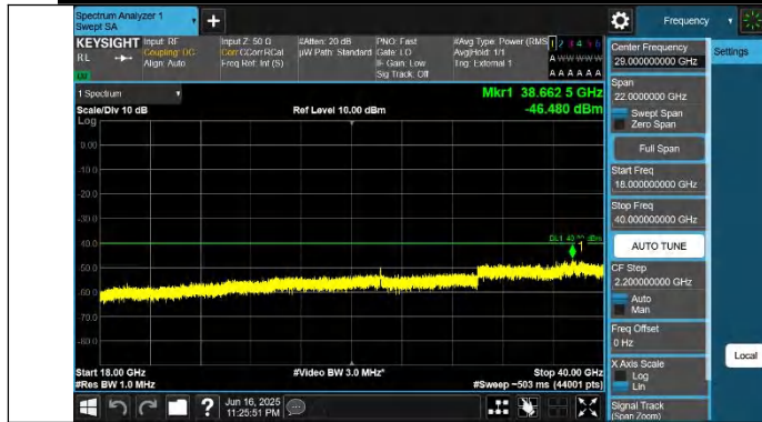
48-48-15MHz-20MHz-QPSK-QPSK-56469-56640-1RB#0-ORB#0-1 8000~40000MHz-PASS
