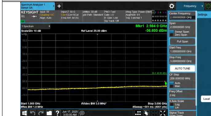
48-48-20MHz-15MHz-QPSK-QPSK-55340-55511-1RB#0-ORB#0-1 000~3000MHz-PASS
