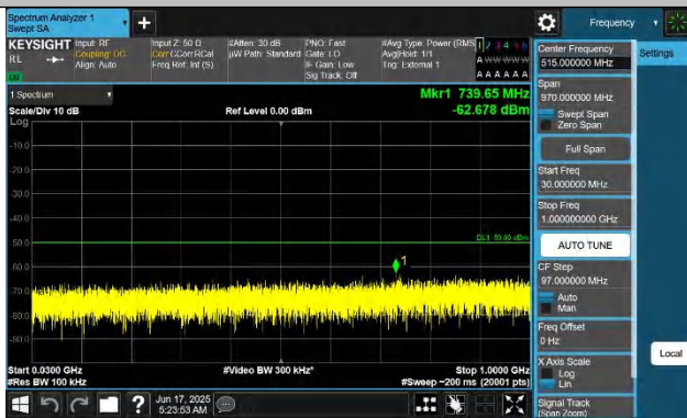
48-48-20MHz-20MHz-QPSK-QPSK-56442-56640-1RB#0-ORB#0-3 0~1000MHz-PASS
