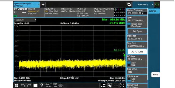
48-48-20MHz-5MHz-QPSK-QPSK-55340-55457-1RB#0-ORB#0-30 ~1000MHz-PASS
