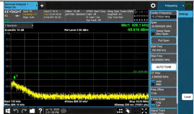
48-48-20MHz-20MHz-QPSK-QPSK-55340-55538-1RB#0-ORB#0-0 .15~30MHz-PASS
