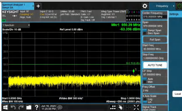
48-48-15MHz-20MHz-QPSK-QPSK-56469-56640-1RB#0-ORB#0-3 0~1000MHz-PASS
