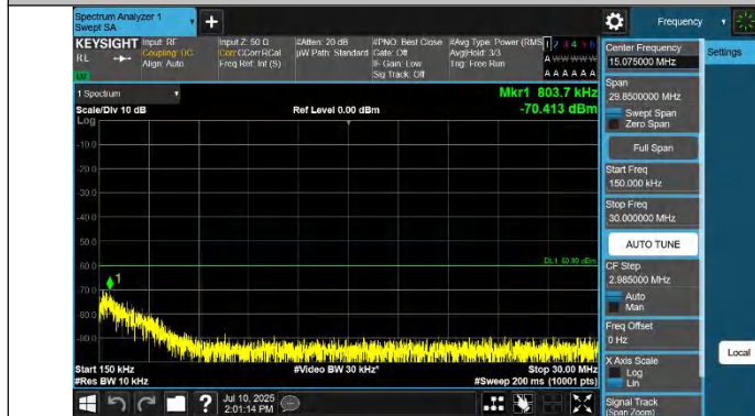
48-48-20MHz-15MHz-QPSK-QPSK-55340-55511-1RB#0-ORB#0-0 .15~30MHz-PASS
