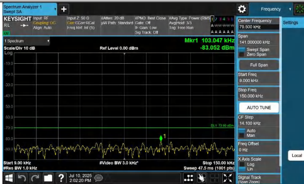
48-48-20MHz-20MHz-QPSK-QPSK-56442-56640-1RB#0-ORB#0-0 .009~0.15MHz-PASS
