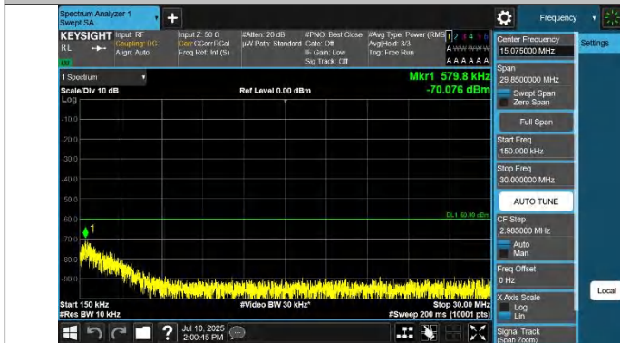
48-48-20MHz-10MHz-QPSK-QPSK-55941-56085-1RB#0-ORB#0-0 .15~30MHz-PASS
