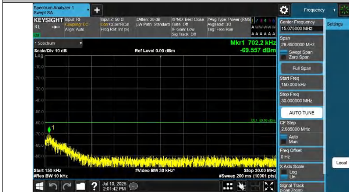
48-48-20MHz-15MHz-QPSK-QPSK-56491-56662-1RB#0-ORB#0-0 .15~30MHz-PASS
