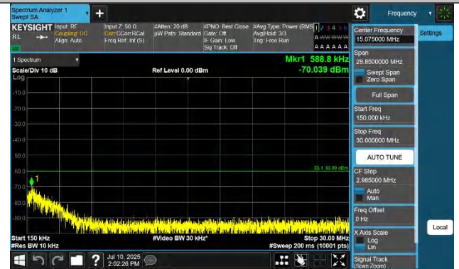
48-48-20MHz-20MHz-QPSK-QPSK-56442-56640-1RB#0-ORB#0-0 .15~30MHz-PASS
