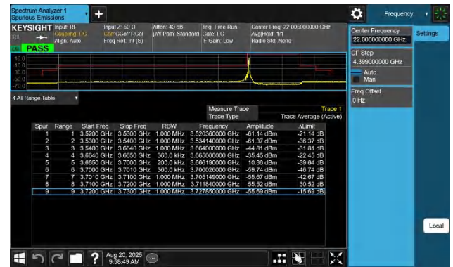
48-48-20MHz-15MHz-QPSK@QPSK-QPSK@QPSK-56491-56662-1RB#0@100RB#0-0RB#75RB#0-PASS
