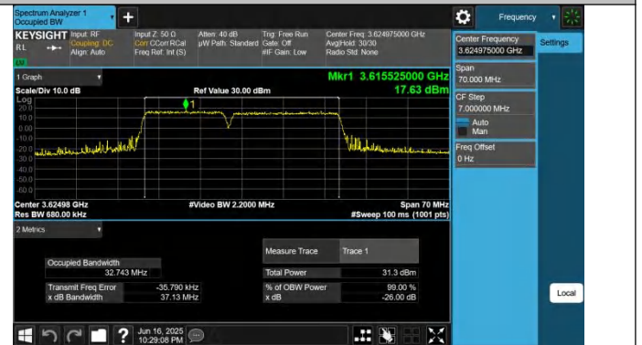
48-48-15MHz-20MHz-64QAM-64QAM-55893-56064-75 RB#0-100RB#0-PASS
