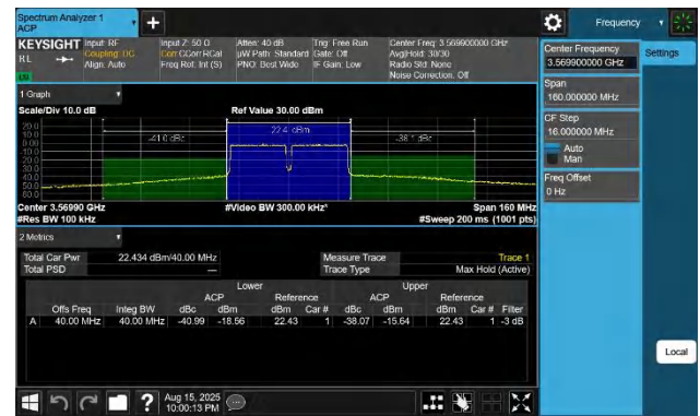
48-48-20MHz-20MHz-16QAM-16QAM-55340-55538-100RB#0-10 0RB#0-PASS
