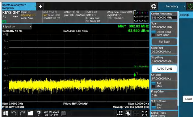
48-48-10MHz-20MHz-QPSK-QPSK-55896-56040-1RB#0-ORB#0-3 0~1000MHz-PASS
