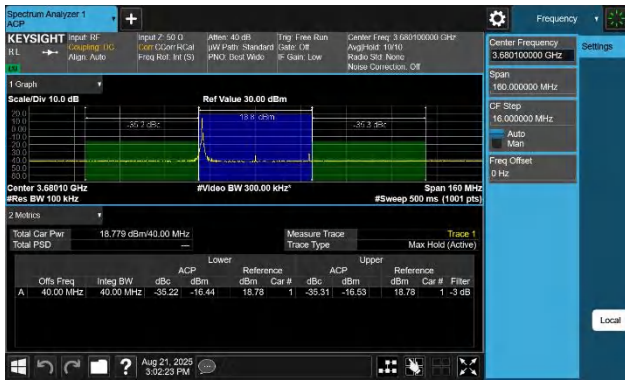
48-48-20MHz-20MHz-256QAM-256QAM-56442-56640-1RB#0-0R B#0-PASS
