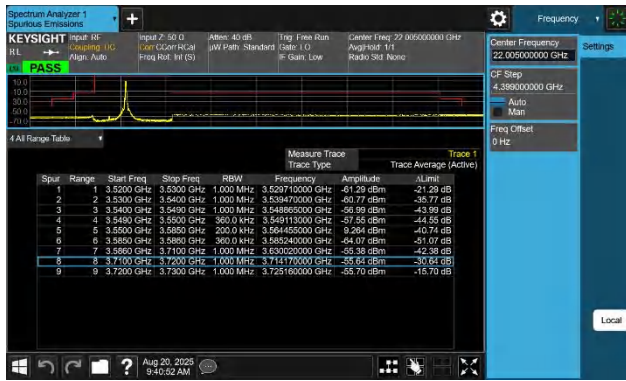
48-48-15MHz-20MHz-QPSK@QPSK-QPSK@QPSK-55318-5548 9-1RB#74@75RB#0-0RB#0@100RB#0-PASS
