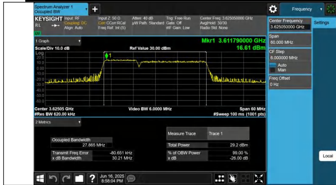
48-48-10MHz-20MHz-256QAM-256QAM-55896-56040-5 ORB#0-100RB#0-PASS
