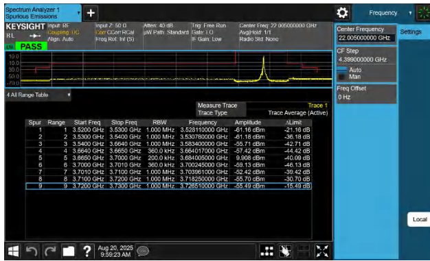
48-48-20MHz-15MHz-QPSK@QPSK-QPSK@QPSK-56491-56662-2-1RB#99@100RB#0-0RB#0@75RB#0-PASS
