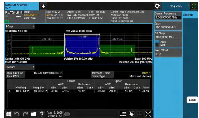
48-48-20MHz-20MHz-16QAM-16QAM-55340-55538-1RB#0-1RB# 99-PASS
