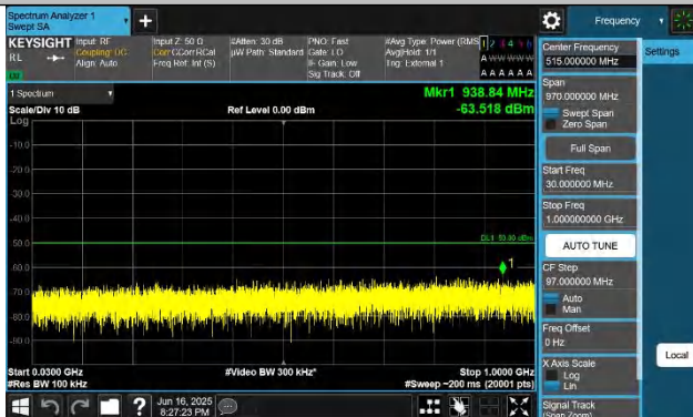
48-48-5MHz-20MHz-QPSK-QPSK-56523-56640-1RB#0-0RB#0-30 ~1000MHz-PASS
