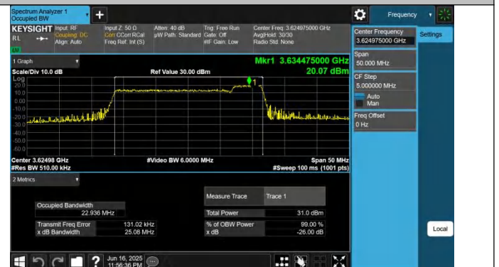
48-48-15MHz-20MHz-16QAM-16QAM-55893-56064-75 RB#0-100RB#0-PASS
