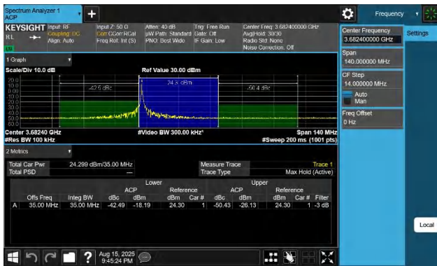
48-48-20MHz-15MHz-16QAM-16QAM-56491-56662-1RB#0-0RB# 75-PASS
