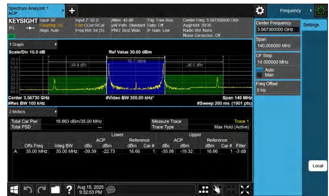
48-48-20MHz-15MHz-16QAM-16QAM-55340-55511-1RB#0-1RB# 74-PASS
