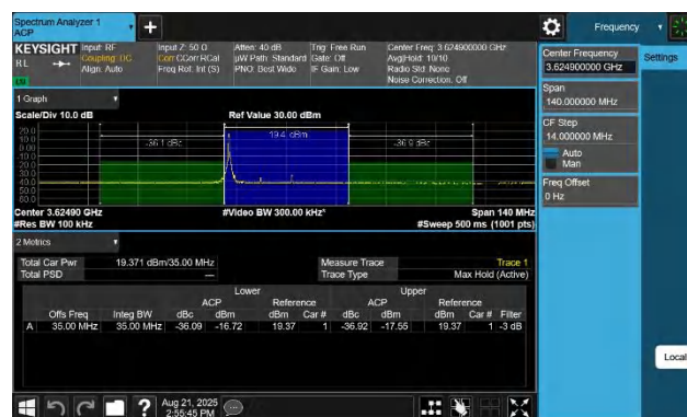
48-48-20MHz-15MHz-256QAM-256QAM-55916-56087-1RB#0-0R B#0-PASS
