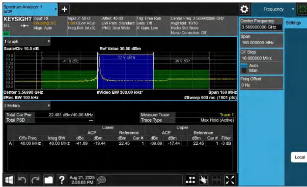
48-48-20MHz-20MHz-QPSK-QPSK-55340-55538-1RB#0-0RB#0-PASS
