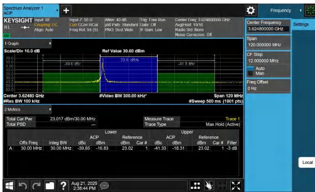
48-48-20MHz-10MHz-16QAM-16QAM-55941-56085-1RB#0-0RB# 0-PASS
