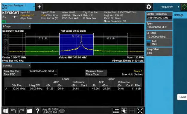
48-48-20MHz-10MHz-16QAM-16QAM-55340-55484-1RB#99-0RB# #0-PASS
