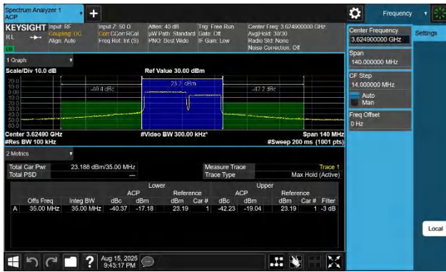
48-48-20MHz-15MHz-16QAM-16QAM-55916-56087-100RB#0-75 RB#0-PASS
