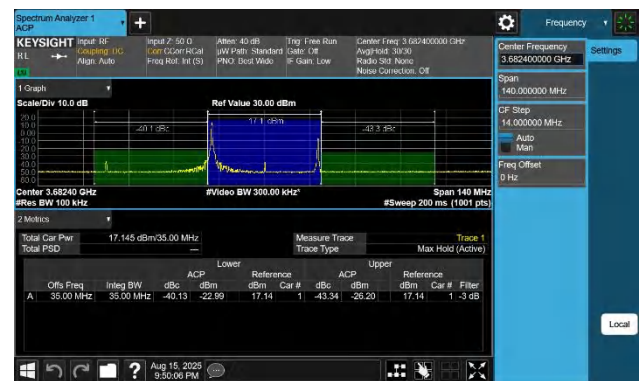
48-48-20MHz-15MHz-64QAM-64QAM-56491-56662-1RB#0-1RB# 74-PASS
