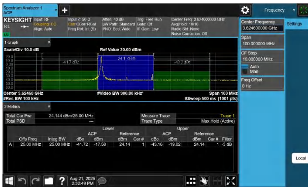
48-48-20MHz-5MHz-QPSK-QPSK-55965-56082-1RB#0-0RB#0-P ASS
