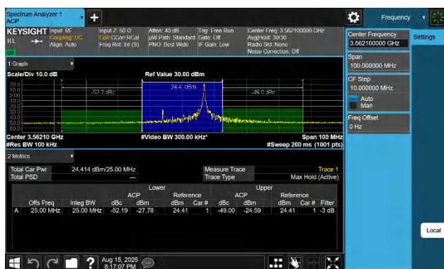
48-48-20MHz-5MHz-16QAM-16QAM-55340-55457-1RB#99-0RB# 0-PASS
