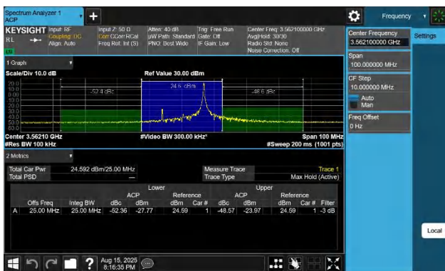
48-48-20MHz-5MHz-QPSK-QPSK-55340-55457-1RB#99-0RB#0-P PASS
