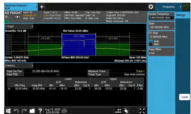
48-48-20MHz-10MHz-16QAM-16QAM-55340-55484-100RB#0-50RB# RB#0-PASS
