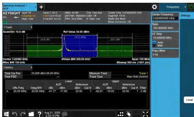
48-48-20MHz-5MHz-16QAM-16QAM-55965-56082-1RB#0-0RB#0 -PASS
