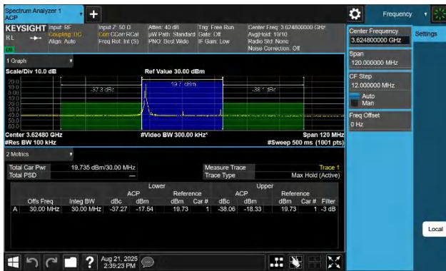
48-48-20MHz-10MHz-256QAM-256QAM-55941-56085-1RB#0-0R B#0-PASS
