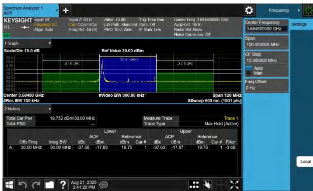
48-48-20MHz-10MHz-256QAM-256QAM-56541-56685-1RB#0-0R B#0-PASS
