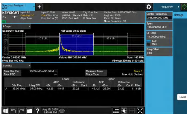
48-48-20MHz-15MHz-64QAM-64QAM-56491-56662-1RB#0-0RB# 75-PASS
