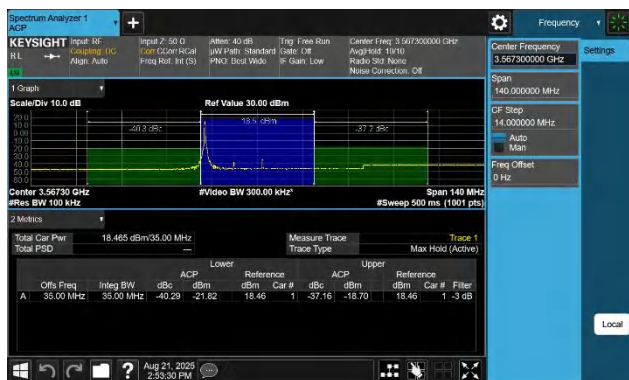
48-48-20MHz-15MHz-256QAM-256QAM-55340-55511-1RB#0-0R B#0-PASS
