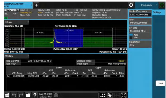
48-48-20MHz-15MHz-16QAM-16QAM-55340-55511-1RB#0-0RB# 0-PASS
