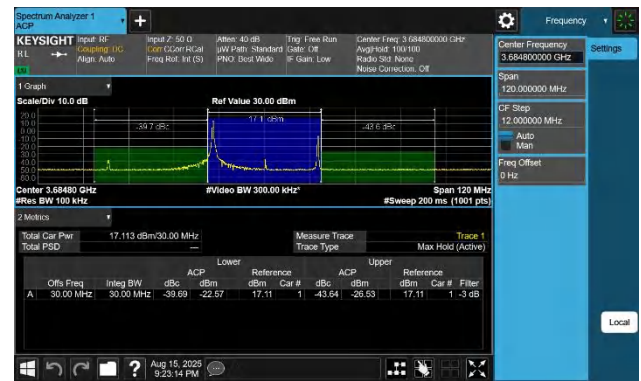
48-48-20MHz-10MHz-256QAM-256QAM-56541-56685-1RB#0-1R B#49-PASS
