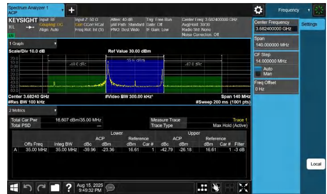
48-48-20MHz-15MHz-16QAM-16QAM-56491-56662-1RB#0-1RB# 74-PASS
