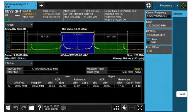
48-48-20MHz-10MHz-256QAM-256QAM-55340-55484-1RB#0-1R B#49-PASS
