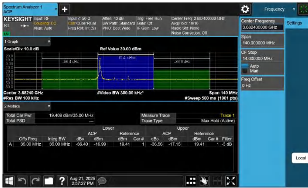
48-48-20MHz-15MHz-256QAM-256QAM-56491-56662-1RB#0-0R B#0-PASS
