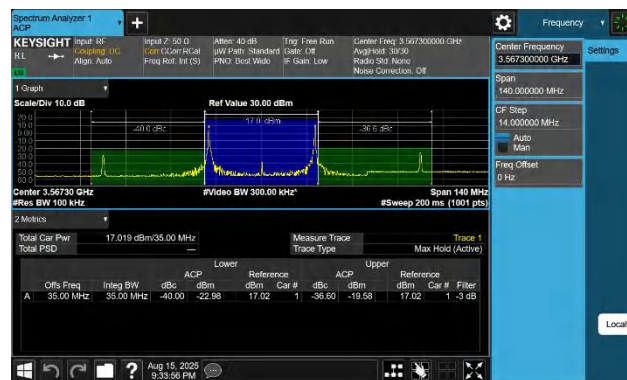
48-48-20MHz-15MHz-256QAM-256QAM-55340-55511-1RB#0-1R B#74-PASS
