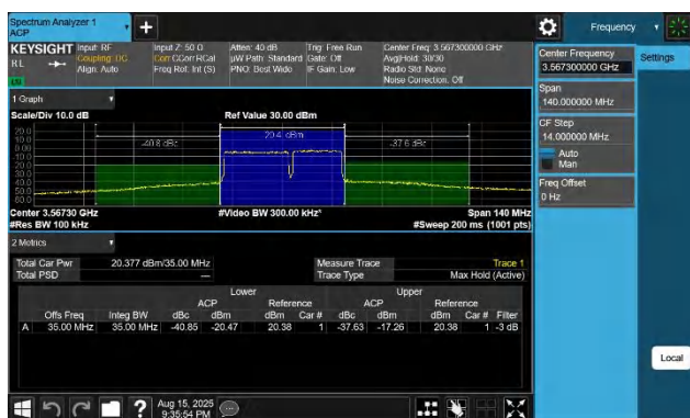
48-48-20MHz-15MHz-256QAM-256QAM-55340-55511-100RB#0-7 5RB#0-PASS
