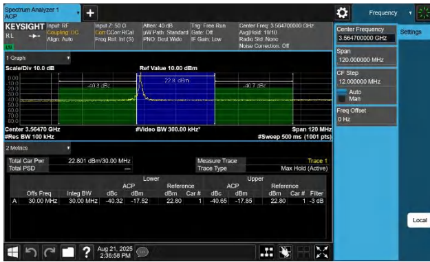
48-48-20MHz-10MHz-16QAM-16QAM-55340-55484-1RB#0-0RB# 0-PASS
