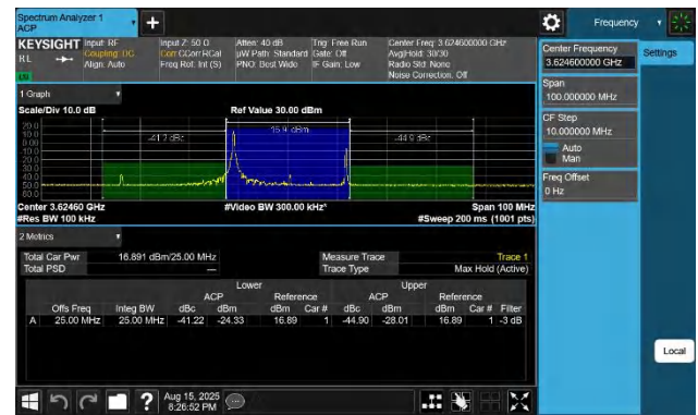
48-48-20MHz-5MHz-QPSK-QPSK-55965-56082-1RB#0-1RB#24-P PASS
