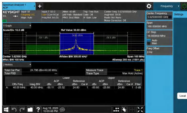
48-48-20MHz-20MHz-QPSK-QPSK-55891-56089-1RB#99-0RB#0- PASS
