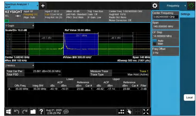
48-48-20MHz-15MHz-16QAM-16QAM-56491-56662-1RB#0-0RB# 0-PASS
