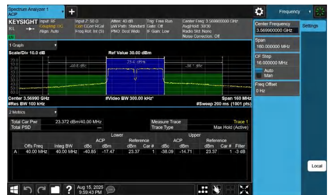
48-48-20MHz-20MHz-QPSK-QPSK-55340-55538-100RB#0-100RB#0-PASS
