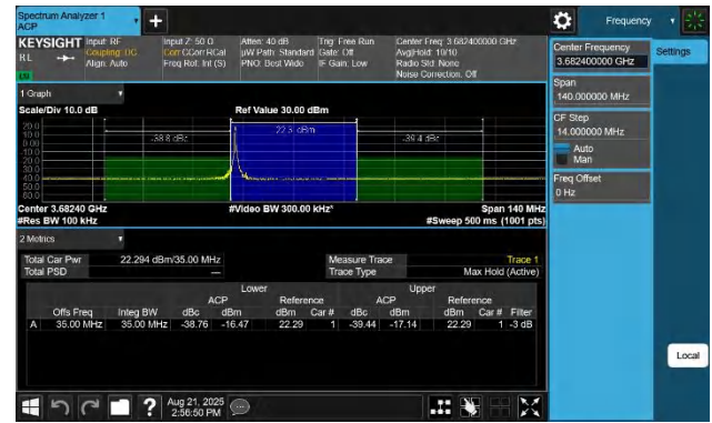
48-48-20MHz-15MHz-64QAM-64QAM-56491-56662-1RB#0-0RB# 0-PASS
