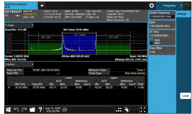
48-48-20MHz-15MHz-256QAM-256QAM-56491-56662-1RB#0-1R B#74-PASS
