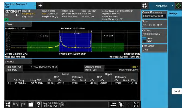
48-48-20MHz-10MHz-256QAM-256QAM-55941-56085-1RB#0-1R B#49-PASS
