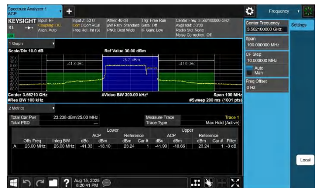
48-48-20MHz-5MHz-QPSK-QPSK-55340-55457-100RB#0-25RB#0-P 0-PASS
