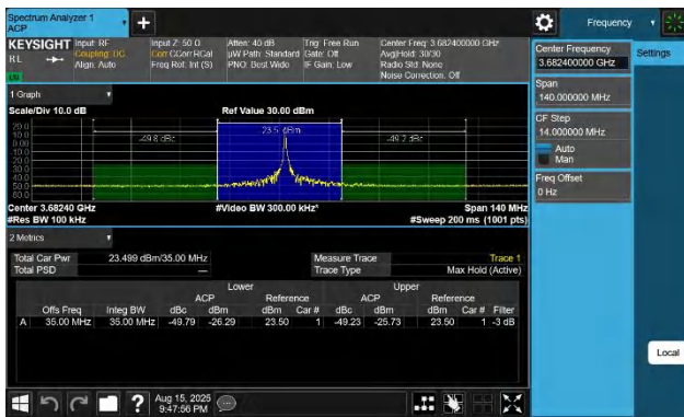
48-48-20MHz-15MHz-64QAM-64QAM-56491-56662-1RB#99-0RB #0-PASS
