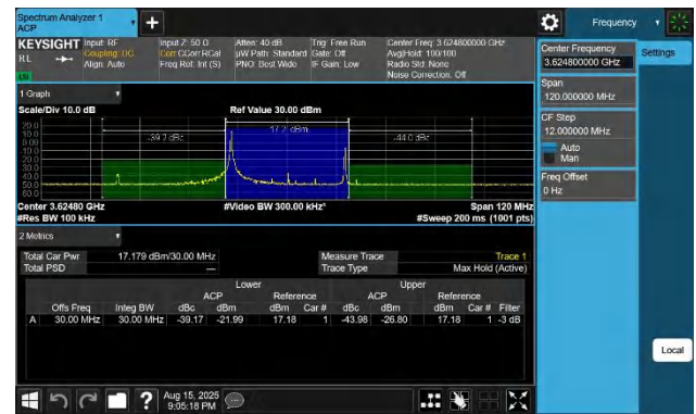
48-48-20MHz-10MHz-16QAM-16QAM-55941-56085-1RB#0-1RB# 49-PASS
