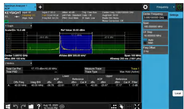
48-48-20MHz-20MHz-QPSK-QPSK-56442-56640-1RB#0-1RB#99- PASS
