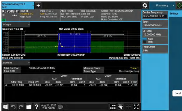
48-48-20MHz-10MHz-256QAM-256QAM-55340-55484-1RB#0-0R B#0-PASS
