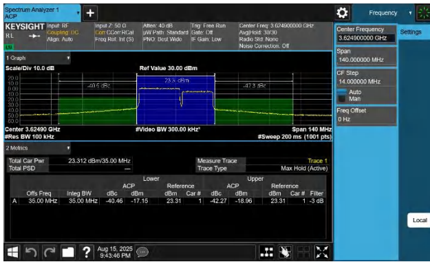
48-48-20MHz-15MHz-64QAM-64QAM-55916-56087-100RB#0-75 RB#0-PASS
