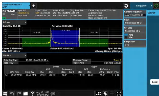
48-48-20MHz-15MHz-256QAM-256QAM-55916-56087-1RB#0-1R B#74-PASS
