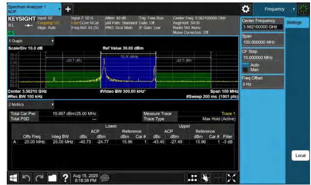
48-48-20MHz-5MHz-QPSK-QPSK-55340-55457-1RB#0-1RB#24-P PASS
