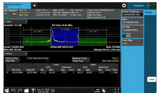
48-48-20MHz-5MHz-16QAM-16QAM-55965-56082-1RB#0-1RB#2 4-PASS
