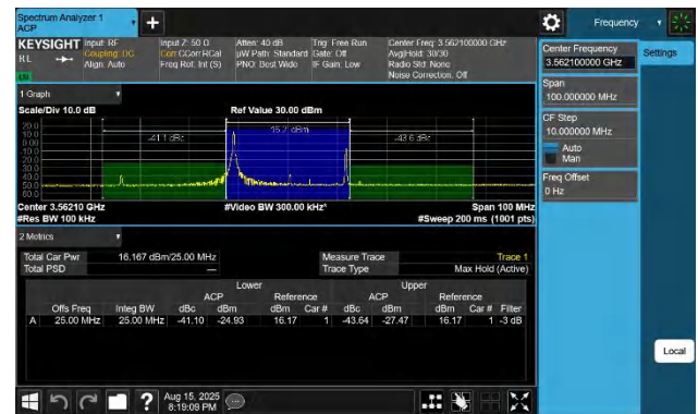
48-48-20MHz-5MHz-16QAM-16QAM-55340-55457-1RB#0-1RB#2 4-PASS
