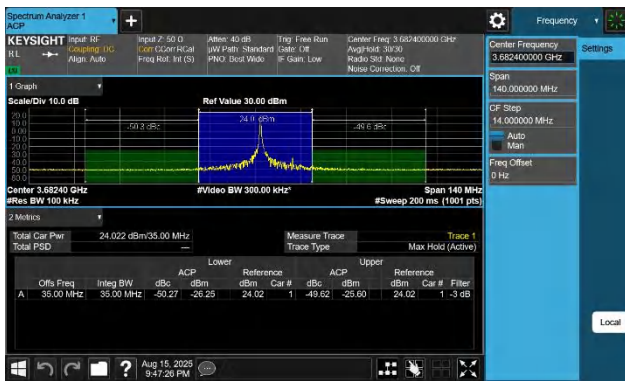
48-48-20MHz-15MHz-16QAM-16QAM-56491-56662-1RB#99-0RB #0-PASS
