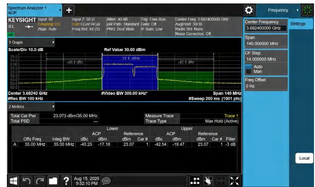
48-48-20MHz-15MHz-64QAM-64QAM-56491-56662-100RB#0-75 RB#0-PASS
