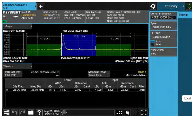
48-48-20MHz-5MHz-16QAM-16QAM-55340-55457-1RB#0-0RB#0 -PASS
