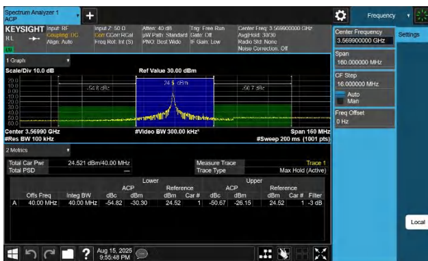
48-48-20MHz-20MHz-QPSK-QPSK-55340-55538-1RB#99-0RB#0-PASS
