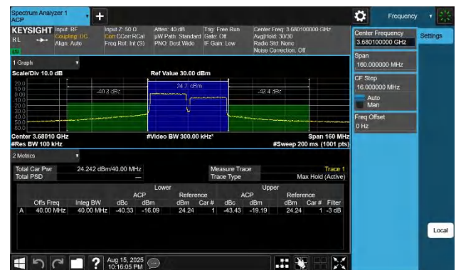
48-48-20MHz-20MHz-QPSK-QPSK-56442-56640-100RB#0-100R B#0-PASS
