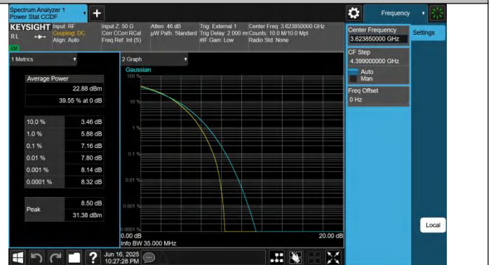
48-48-15MHz-20MHz-64QAM-64QAM-55893-56064-75RB#0 B#0-100RB#0-PASS
