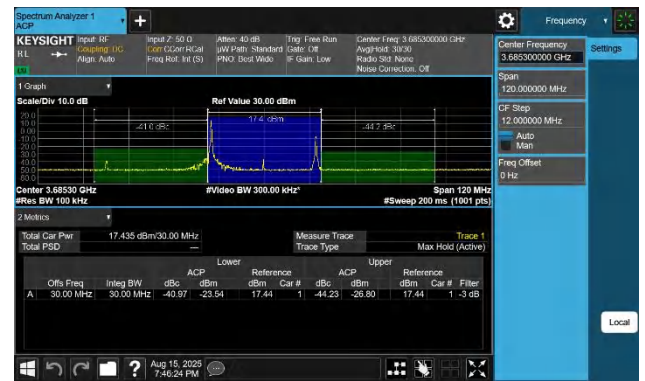
48-48-10MHz-20MHz-256QAM-256QAM-56496-56640-1RB#0-1R B#99-PASS
