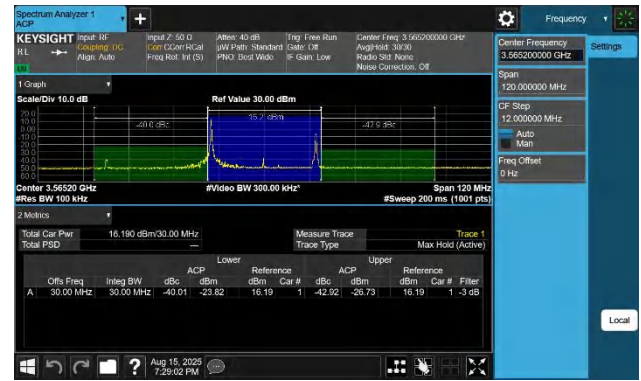
48-48-10MHz-20MHz-16QAM-16QAM-55295-55439-1RB#0-1RB# 99-PASS
