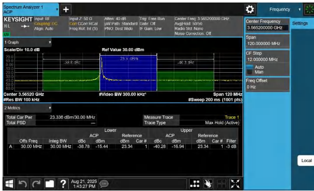
48-48-10MHz-20MHz-16QAM-16QAM-55295-55439-1RB#0-ORB# 0-PASS
