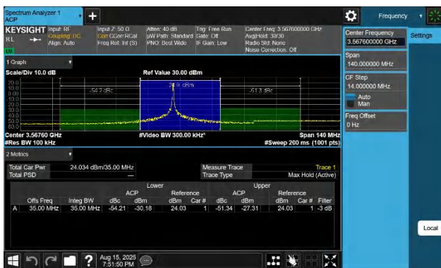
48-48-15MHz-20MHz-QPSK-QPSK-55318-55489-1RB#74-0RB#0-PASS
