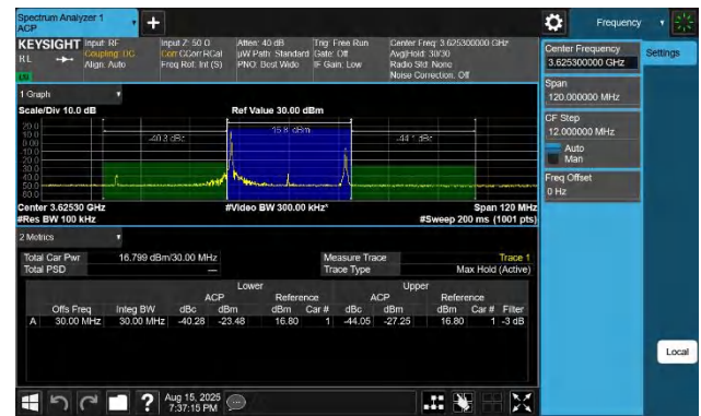
48-48-10MHz-20MHz-16QAM-16QAM-55896-56040-1RB#0-1RB# 99-PASS
