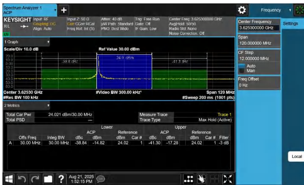
48-48-10MHz-20MHz-16QAM-16QAM-55896-56040-1RB#0-ORB# 0-PASS
