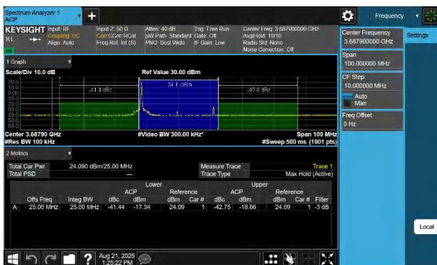
48-48-5MHz-20MHz-QPSK-QPSK-56523-56640-1RB#0-0RB#0-PASS
