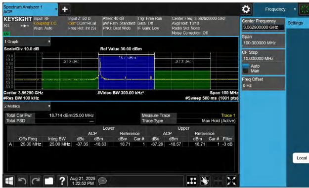
48-48-5MHz-20MHz-256QAM-256QAM-55273-55390-1RB#0-0RB #0-PASS
