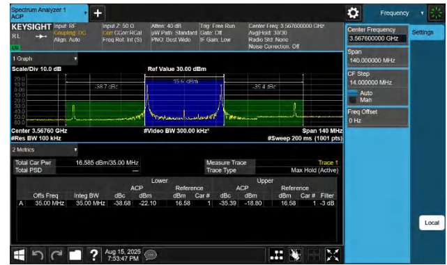
48-48-15MHz-20MHz-QPSK-QPSK-55318-55489-1RB#0-1RB#99-PASS
