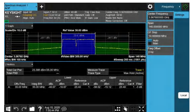
48-48-15MHz-20MHz-QPSK-QPSK-55318-55489-75RB#0-100RB#0-PASS
