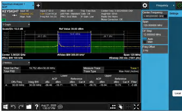
48-48-10MHz-20MHz-256QAM-256QAM-55295-55439-1RB#0-0R B#0-PASS
