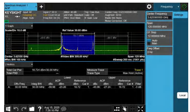
48-48-10MHz-20MHz-256QAM-256QAM-55896-56040-1RB#0-1R B#99-PASS
