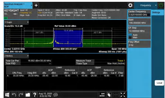
48-48-15MHz-20MHz-64QAM-64QAM-55893-56064-1RB#0-1RB# 99-PASS
