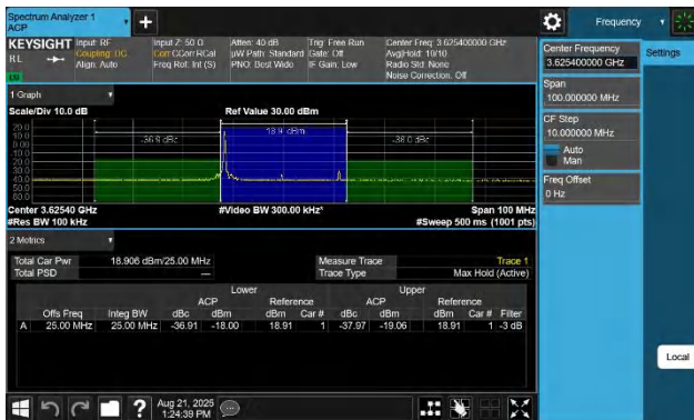
48-48-5MHz-20MHz-256QAM-256QAM-55898-56015-1RB#0-0RB #0-PASS
