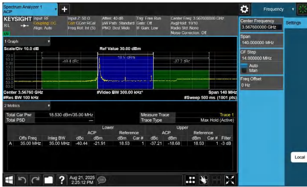
48-48-15MHz-20MHz-256QAM-256QAM-55318-55489-1RB#0-0R B#0-PASS
