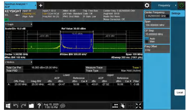
48-48-5MHz-20MHz-256QAM-256QAM-55273-55390-1RB#0-1RB #99-PASS
