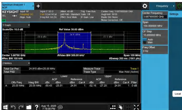
48-48-5MHz-20MHz-QPSK-QPSK-56523-56640-1RB#24-0RB#0-PASS
