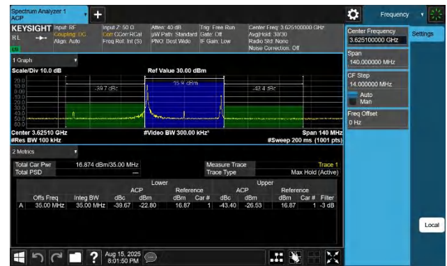
48-48-15MHz-20MHz-QPSK-QPSK-55893-56064-1RB#0-1RB#99-PASS
