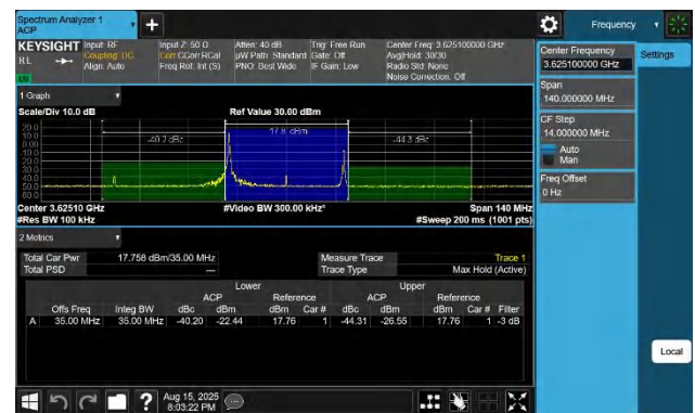
48-48-15MHz-20MHz-256QAM-256QAM-55893-56064-1RB#0-1R B#99-PASS
