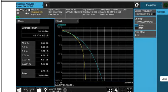
48-48-15MHz-20MHz-256QAM-256QAM-55893-56064-75RB#0 ORB#0-100RB#0-PASS
