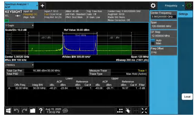
48-48-10MHz-20MHz-256QAM-256QAM-55295-55439-1RB#0-1R B#99-PASS
