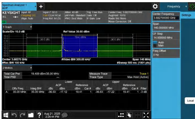
48-48-15MHz-20MHz-256QAM-256QAM-56469-56640-1RB#0-0R B#0-PASS
