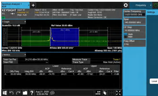
48-48-15MHz-20MHz-QPSK-QPSK-55893-56064-1RB#0-0RB#0-PASS
