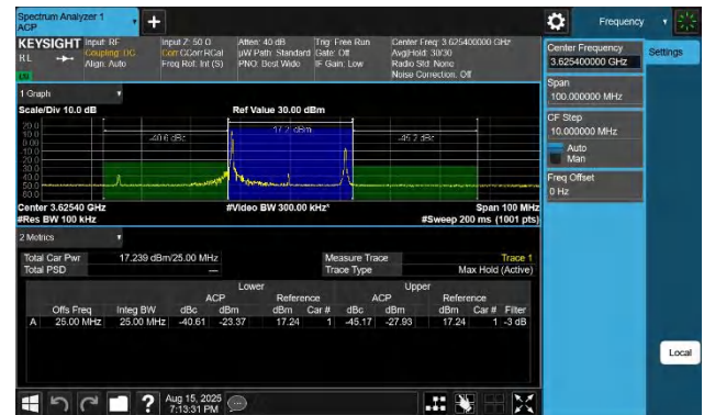
48-48-5MHz-20MHz-256QAM-256QAM-55898-56015-1RB#0-1RB #99-PASS
