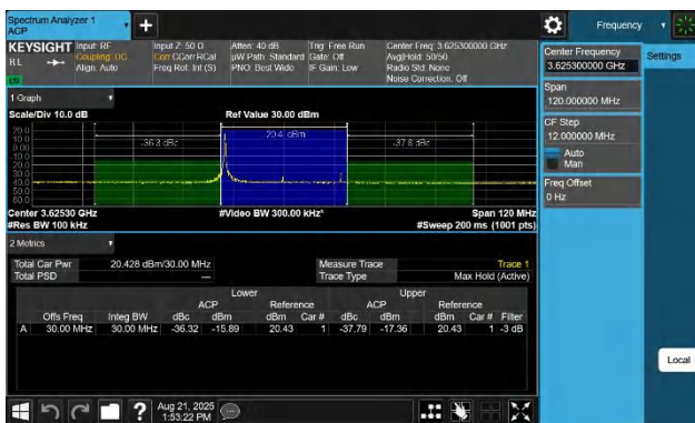
48-48-10MHz-20MHz-256QAM-256QAM-55896-56040-1RB#0-0R B#0-PASS
