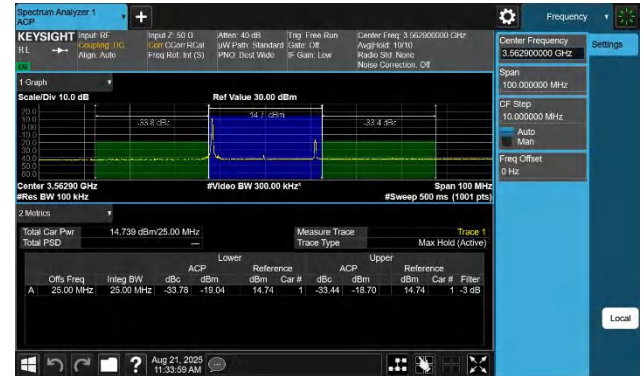
48-48-5MHz-20MHz-QPSK-QPSK-55273-55390-1RB#0-1RB#99- PASS
