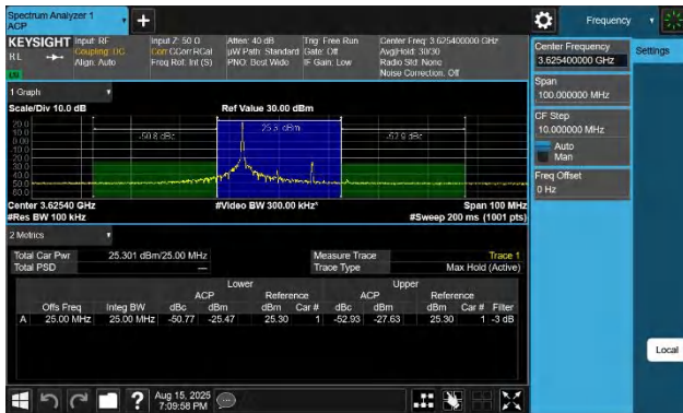
48-48-5MHz-20MHz-QPSK-QPSK-55898-56015-1RB#24-0RB#0-PASS
