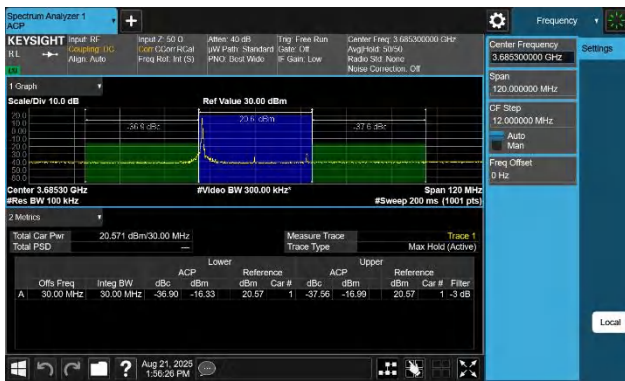
48-48-10MHz-20MHz-256QAM-256QAM-56496-56640-1RB#0-0R B#0-PASS
