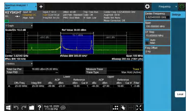
48-48-5MHz-20MHz-QPSK-QPSK-55898-56015-1RB#0-1RB#99- PASS
