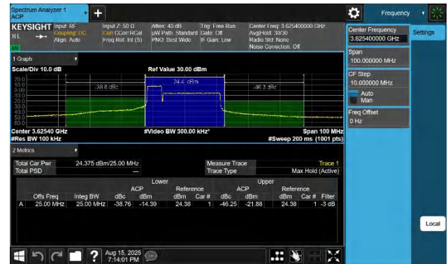
48-48-5MHz-20MHz-QPSK-QPSK-55898-56015-25RB#0-100RB#0-PASS
