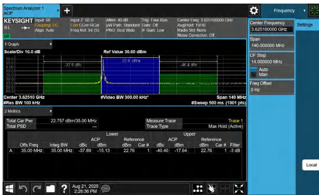
48-48-15MHz-20MHz-64QAM-64QAM-55893-56064-1RB#0-0RB# 0-PASS
