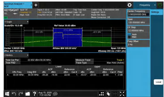
48-48-10MHz-20MHz-16QAM-16QAM-55295-55439-50RB#0-100RB# RB#0-PASS
