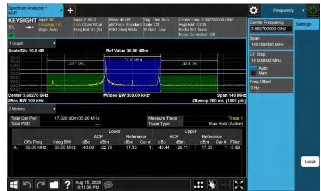
48-48-15MHz-20MHz-256QAM-256QAM-56469-56640-1RB#0-1R B#99-PASS
