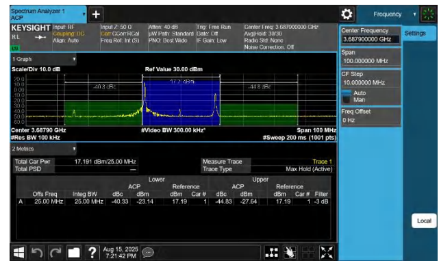
48-48-5MHz-20MHz-256QAM-256QAM-56523-56640-1RB#0-1RB #99-PASS
