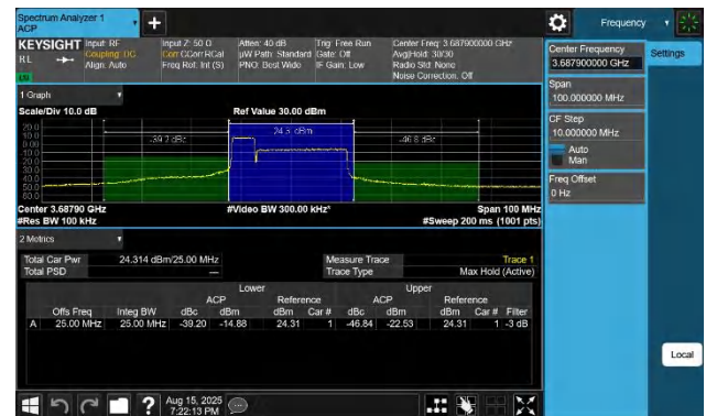
48-48-5MHz-20MHz-QPSK-QPSK-56523-56640-25RB#0-100RB#0-PASS
