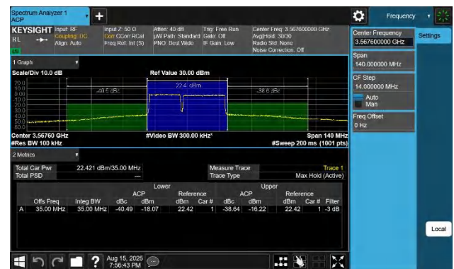
48-48-15MHz-20MHz-64QAM-64QAM-55318-55489-75RB#0-100RB# RB#0-PASS
