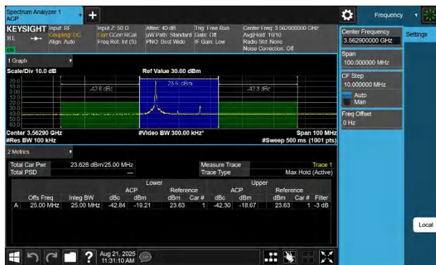
48-48-5MHz-20MHz-QPSK-QPSK-55273-55390-1RB#24-0RB#0- PASS
