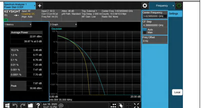
48-48-15MHz-20MHz-16QAM-16QAM-55893-56064-75RB#0 B#0-100RB#0-PASS
