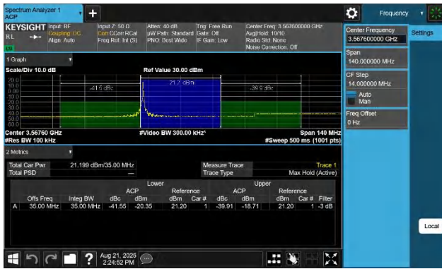
48-48-15MHz-20MHz-64QAM-64QAM-55318-55489-1RB#0-0RB# 0-PASS
