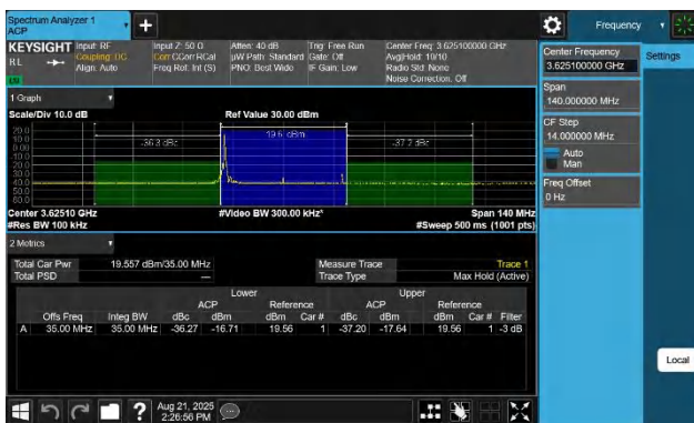
48-48-15MHz-20MHz-256QAM-256QAM-55893-56064-1RB#0-0R B#0-PASS
