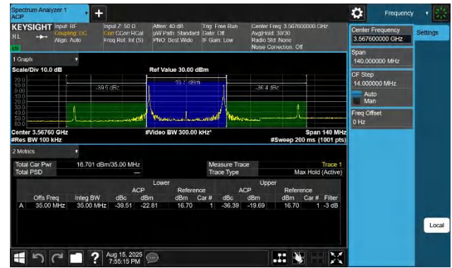
48-48-15MHz-20MHz-256QAM-256QAM-55318-55489-1RB#0-1R B#99-PASS
