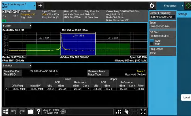
48-48-15MHz-20MHz-QPSK-QPSK-55318-55489-1RB#0-0RB#0-PASS
