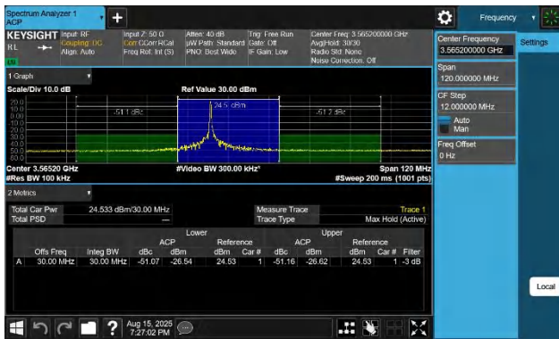
48-48-10MHz-20MHz-16QAM-16QAM-55295-55439-1RB#49-ORB# #0-PASS
