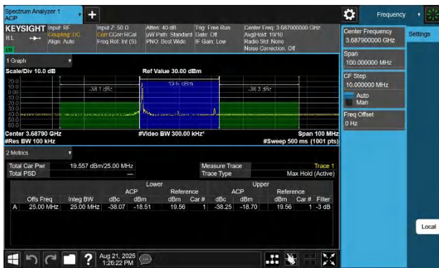
48-48-5MHz-20MHz-256QAM-256QAM-56523-56640-1RB#0-0RB #0-PASS
