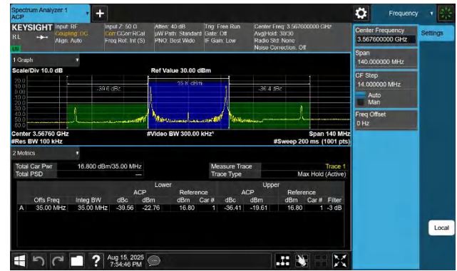
48-48-15MHz-20MHz-64QAM-64QAM-55318-55489-1RB#0-1RB# 99-PASS
