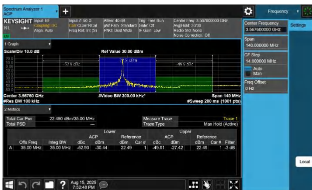
48-48-15MHz-20MHz-64QAM-64QAM-55318-55489-1RB#74-0RB# #0-PASS
