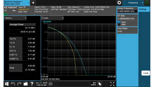
48-48-20MHz-15MHz-64QAM-64QAM-55916-56087-100RB#0-75RB#0-PASS
