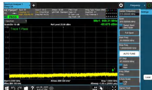
NTNV-n48-PC3-30-30-H-CP-QPSK-Inner_1RB_Right-30-1000-PA SS
