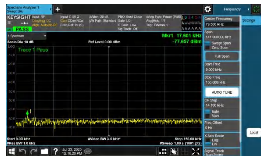
NTNV-n48-PC3-30-40-H-CP-QPSK-Inner_1RB_Right-0.009-0.15-PASS
