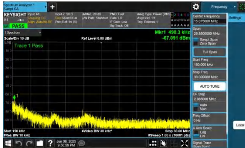
NTNV-n48-PC3-30-40-L-CP-QPSK-Inner_1RB_Right-0.15-30-PA SS
