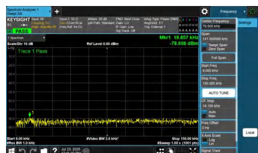
NTNV-n48-PC3-30-40-L-CP-QPSK-Inner_1RB_Right-0.009-0.15- PASS
