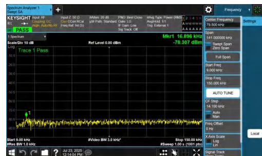
NTNV-n48-PC3-30-40-M-CP-QPSK-Inner_1RB_Right-0.009-0.15- PASS
