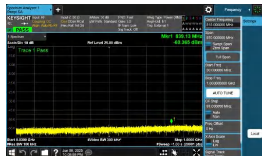
NTNV-n48-PC3-30-40-H-CP-QPSK-Inner_1RB_Right-30-1000-PA-SS
