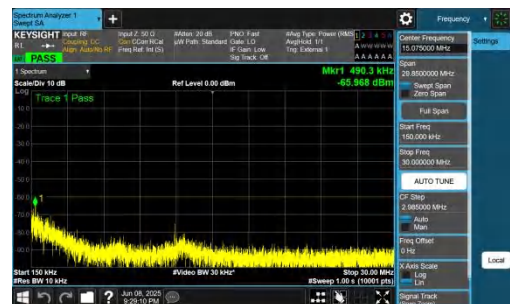
NTNV-n48-PC3-30-30-M-CP-QPSK-Inner_1RB_Left-0.15-30-PASS
