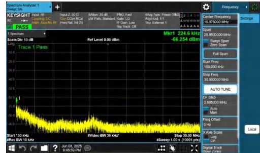
NTNV-n48-PC3-30-40-L-CP-QPSK-Inner_1RB_Left-0.15-30-PASS
