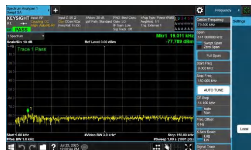
NTNV-n48-PC3-30-20-H-CP-QPSK-Inner_1RB_Right-0.009-0.15-PASS
