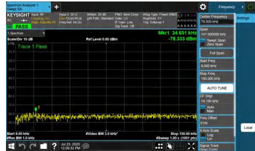
NTNV-n48-PC3-30-30-H-CP-QPSK-Inner_1RB_Right-0.009-0.15- PASS
