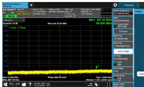
NTNV-n48-PC3-30-20-H-CP-QPSK-Inner_1RB_Left-30-1000-PASS
