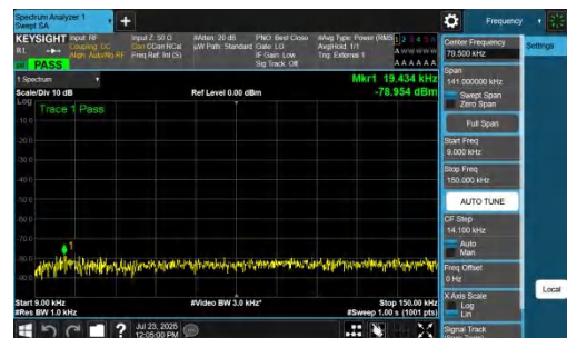
NTNV-n48-PC3-30-30-L-CP-QPSK-Inner_1RB_Right-0.009-0.15- PASS
