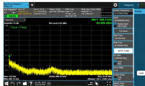
NTNV-n48-PC3-30-20-M-CP-QPSK-Inner_1RB_Left-0.15-30-PAS S
