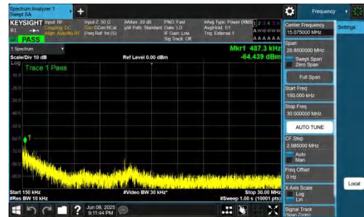
NTNV-n48-PC3-30-20-H-CP-QPSK-Inner_1RB_Left-0.15-30-PASS
