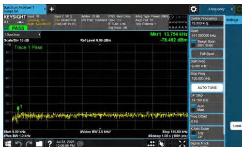
NTNV-n48-PC3-30-30-M-CP-QPSK-Inner_1RB_Left-0.009-0.15-PASS
