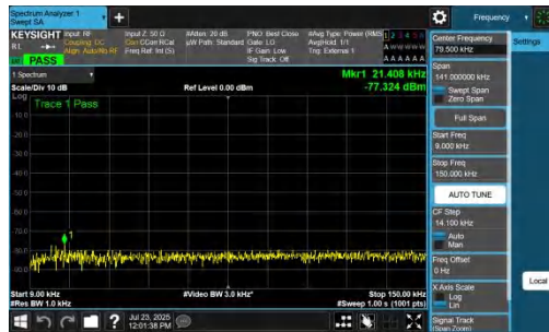
NTNV-n48-PC3-30-20-H-CP-QPSK-Inner_1RB_Left-0.009-0.15-PASS
