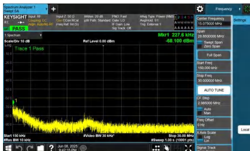
NTNV-n48-PC3-30-30-H-CP-QPSK-Inner_1RB_Right-0.15-30-PA SS
