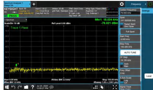
NTNV-n48-PC3-30-20-M-CP-QPSK-Inner_1RB_Right-0.009-0.15- PASS
