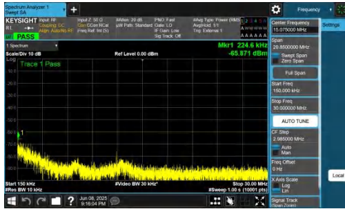
NTVN-n48-PC3-30-20-H-CP-QPSK-Inner_1RB_Right-0.15-30-PA SS
