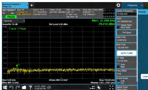
NTNV-n48-PC3-30-30-H-CP-QPSK-Inner_1RB_Left-0.009-0.15- PASS
