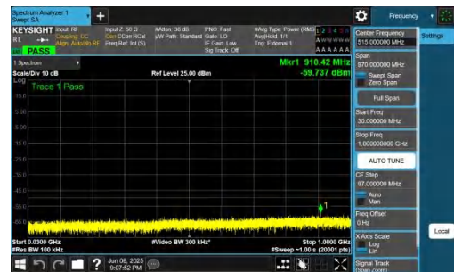
NTNV-n48-PC3-30-20-M-CP-QPSK-Inner_1RB_Right-30-1000-PA SS
