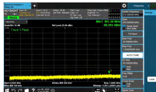
NTNV-n48-PC3-30-30-M-CP-QPSK-Inner_1RB_Right-30-1000-PASS
