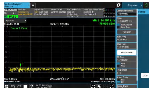
NTNV-n48-PC3-30-30-M-CP-QPSK-Inner_1RB_Right-0.009-0.15-PASS
