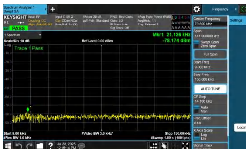
NTNV-n48-PC3-30-40-H-CP-QPSK-Inner_1RB_Left-0.009-0.15- PASS
