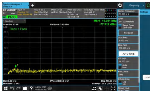
NTNV-n48-PC3-30-20-M-CP-QPSK-Inner_1RB_Left-0.009-0.15- PASS
