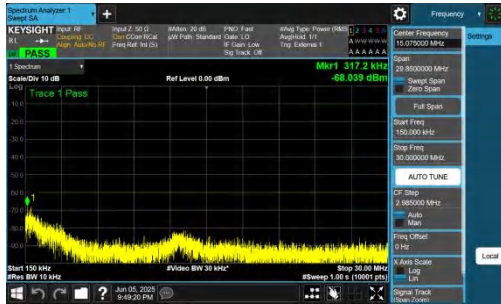
NTNV-n48-PC3-30-15-M-DFT-BPSK-Inner_1RB_Right-0.15-30-P ASS
