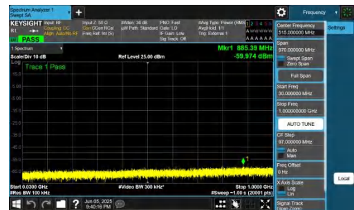
NTNV-n48-PC3-30-15-L-DFT-QPSK-Inner_1RB_Right-30-1000-P ASS
