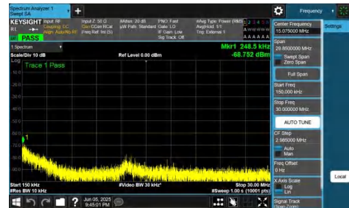
NTNV-n48-PC3-30-15-M-DFT-BPSK-Inner_1RB_Left-0.15-30-PAS
