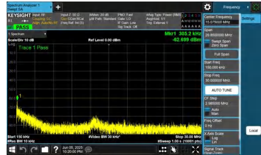
NTNV-n48-PC3-30-20-L-DFT-BPSK-Inner_1RB_Left-0.15-30-PASS
