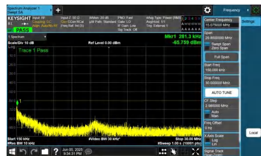
NTNV-n48-PC3-30-15-L-DFT-QPSK-Inner_1RB_Left-0.15-30-PAS S
