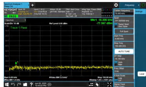
NTNV-n48-PC3-30-20-M-DFT-BPSK-Inner_1RB_Right-0.009-0.15-PASS
