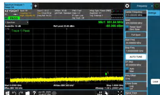
NTNV-n48-PC3-30-20-M-DFT-BPSK-Inner_1RB_Right-30-1000-PASS
