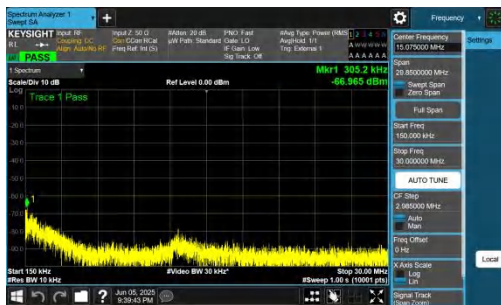
NTNV-n48-PC3-30-15-L-DFT-QPSK-Inner_1RB_Right-0.15-30-P ASS
