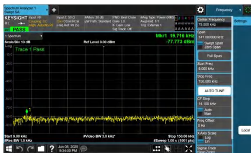
NTNV-n48-PC3-30-15-L-DFT-QPSK-Inner_1RB_Left-0.009-0.15- PASS
