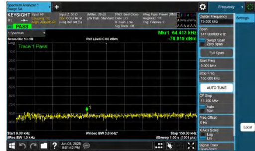
NTNV-n48-PC3-30-10-M-DFT-QPSK-Inner_1RB_Right-0.009-0.15 -PASS
