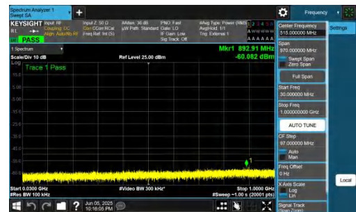
NTNV-n48-PC3-30-15-H-DFT-QPSK-Inner_1RB_Right-30-1000-P ASS
