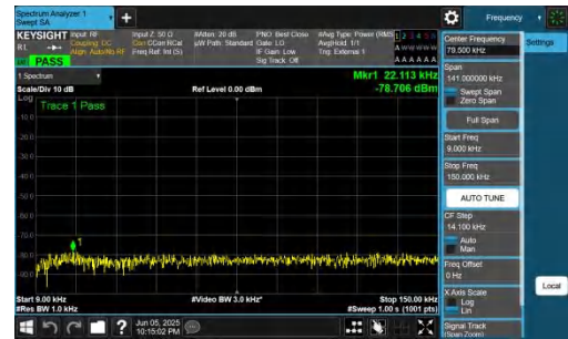
NTNV-n48-PC3-30-15-H-DFT-QPSK-Inner_1RB_Right-0.009-0.15 -PASS
