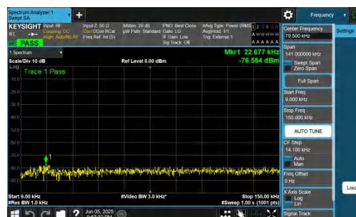
NTNV-n48-PC3-30-15-M-DFT-QPSK-Inner_1RB_Right-0.009-0.15 -PASS
