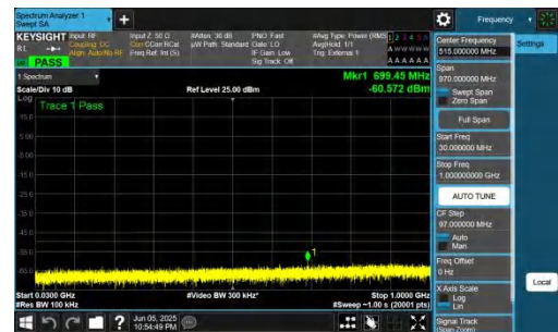
NTNV-n48-PC3-30-20-M-DFT-QPSK-Inner_1RB_Right-30-1000-P ASS
