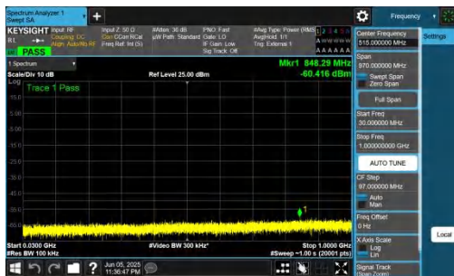
NTNV-n48-PC3-30-30-M-DFT-BPSK-Inner_1RB_Left-30-1000-PASS
