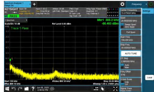
NTNV-n48-PC3-30-10-H-DFT-BPSK-Inner_1RB_Left-0.15-30-PASS
