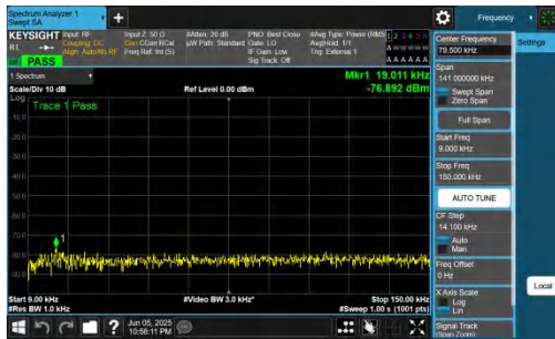
NTNV-n48-PC3-30-20-H-DFT-BPSK-Inner_1RB_Left-0.009-0.15-PASS
