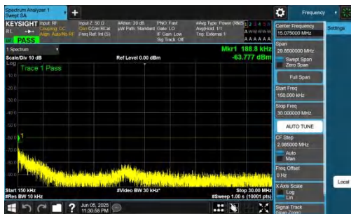
NTNV-n48-PC3-30-30-L-DFT-QPSK-Inner_1RB_Right-0.15-30-P ASS
