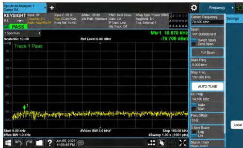
NTNV-n48-PC3-30-30-M-DFT-BPSK-Inner_1RB_Left-0.009-0.15-PASS
