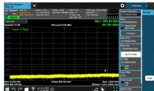
NTNV-n48-PC3-30-30-L-DFT-BPSK-Inner_1RB_Right-30-1000-PASS
