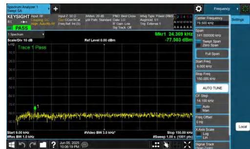
NTNV-n48-PC3-30-15-H-DFT-BPSK-Inner_1RB_Right-0.009-0.15-PASS
