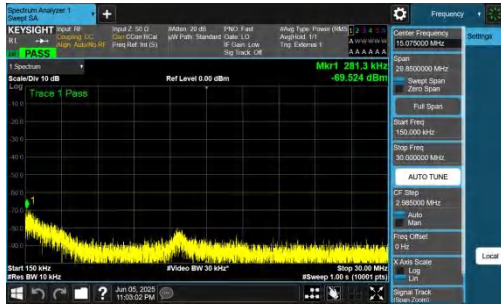
NTNV-n48-PC3-30-20-H-DFT-BPSK-Inner_1RB_Right-0.15-30-P ASS
