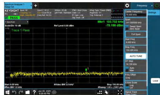
NTNV-n48-PC3-30-15-L-DFT-BPSK-Inner_1RB_Right-0.009-0.15-PASS
