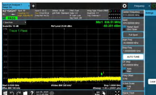
NTNV-n48-PC3-30-15-H-DFT-QPSK-Inner_1RB_Left-30-1000-PASS
