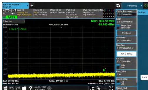
NTNV-n48-PC3-30-15-L-DFT-QPSK-Inner_1RB_Left-30-1000-PA SS
