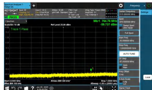
NTNV-n48-PC3-30-15-L-DFT-BPSK-Inner_1RB_Right-30-1000-PASS
