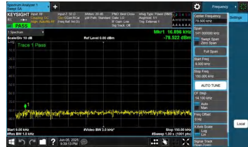
NTNV-n48-PC3-30-15-L-DFT-QPSK-Inner_1RB_Right-0.009-0.15- PASS
