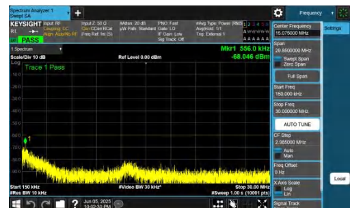
NTNV-n48-PC3-30-15-H-DFT-BPSK-Inner_1RB_Left-0.15-30-PAS S
