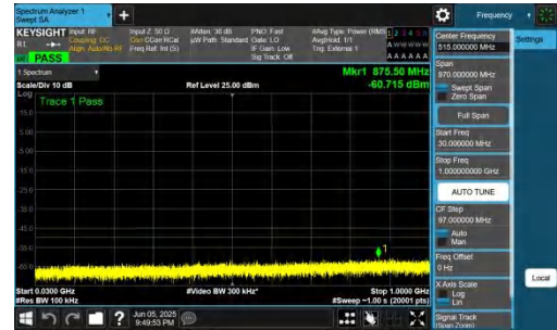
NTNV-n48-PC3-30-15-M-DFT-BPSK-Inner_1RB_Right-30-1000-P ASS
