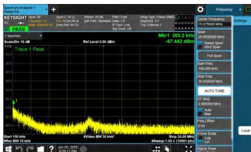
NTNV-n48-PC3-30-15-L-DFT-BPSK-Inner_1RB_Right-0.15-30-PASS
