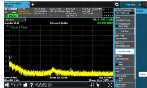
NTNV-n48-PC3-30-30-M-DFT-BPSK-Inner_1RB_Left-0.15-30-PASS
