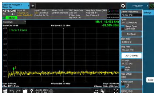
NTNV-n48-PC3-30-15-L-DFT-BPSK-Inner_1RB_Left-0.009-0.15- PASS
