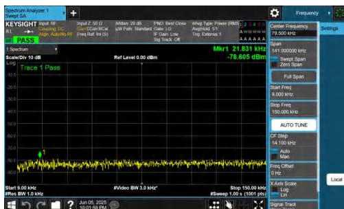
NTNV-n48-PC3-30-15-H-DFT-BPSK-Inner_1RB_Left-0.009-0.15- PASS
