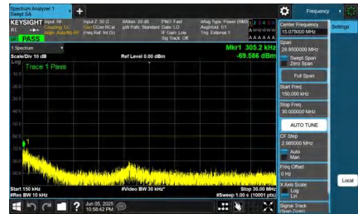
NTNV-n48-PC3-30-20-H-DFT-BPSK-Inner_1RB_Left-0.15-30-PAS S
