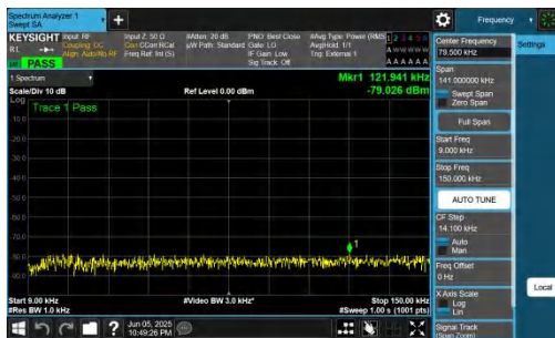
NTNV-n48-PC3-30-20-M-DFT-QPSK-Inner_1RB_Left-0.009-0.15-PASS
