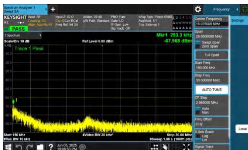
NTNV-n48-PC3-30-15-H-DFT-BPSK-Inner_1RB_Right-0.15-30-PASS
