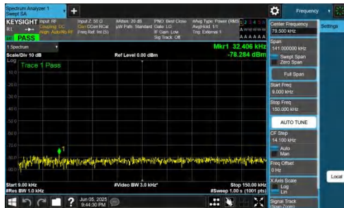
NTNV-n48-PC3-30-15-M-DFT-BPSK-Inner_1RB_Left-0.009-0.15- PASS
