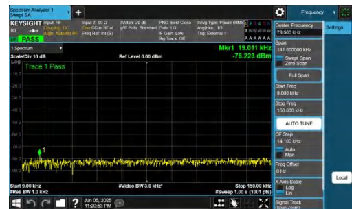
NTNV-n48-PC3-30-30-L-DFT-BPSK-Inner_1RB_Right-0.009-0.15-PASS
