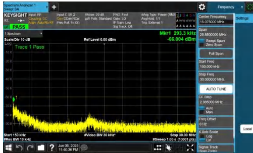
NTNV-n48-PC3-30-30-M-DFT-BPSK-Inner_1RB_Right-0.15-30-P ASS
