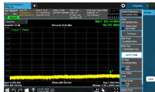
NTNV-n48-PC3-30-15-H-DFT-BPSK-Inner_1RB_Right-30-1000-PASS
