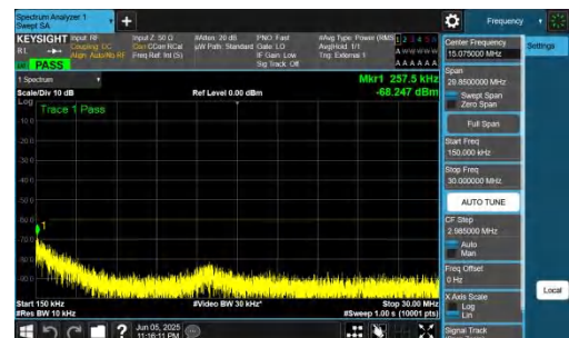
NTNV-n48-PC3-30-30-L-DFT-BPSK-Inner_1RB_Left-0.15-30-PAS S
