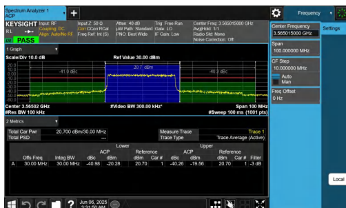
NTNV-n48-PC3-30-30-L-DFT-QPSK-Outer_Full-PASS
