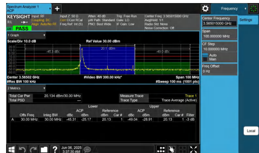
NTNV-n48-PC3-30-30-L-DFT-64QAM-Edge_1RB_Left-PASS
