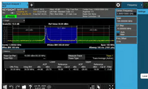
NTNV-n48-PC3-30-30-L-CP-64QAM-Edge_1RB_Left-PASS
