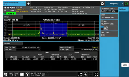
NTNV-n48-PC3-30-30-L-CP-16QAM-Edge_1RB_Left-PASS
