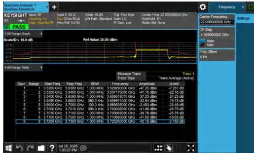
NTNV-n48-PC3-30-40-H-DFT-BPSK-Outer_Full-PASS
