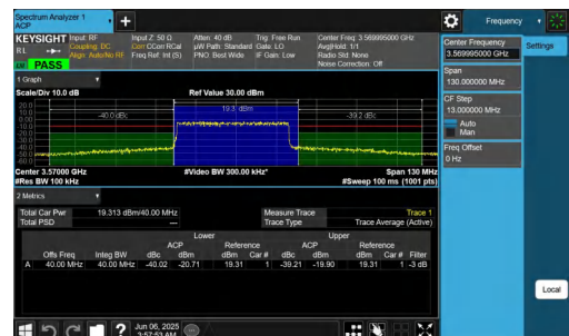
NTVN-n48-PC3-30-40-L-DFT-64QAM-Outer_Full-PASS
