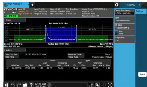
NTNV-n48-PC3-30-30-L-CP-64QAM-Edge_1RB_Left-PASS
