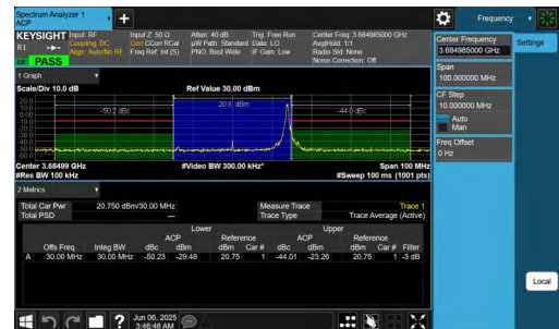
NTNV-n48-PC3-30-30-H-DFT-16QAM-Edge_1RB_Right-PASS
