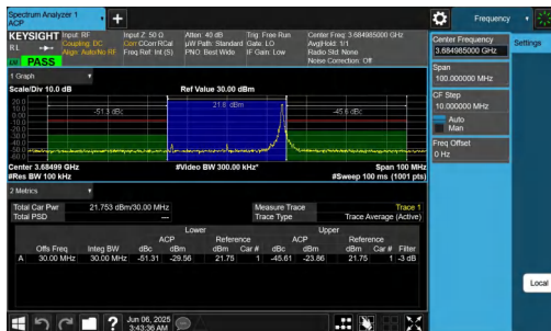
NTNV-n48-PC3-30-30-H-DFT-BPSK-Edge_1RB_Right-PASS
