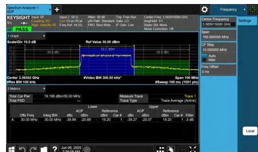
NTNV-n48-PC3-30-30-L-DFT-64QAM-Outer_Full-PASS
