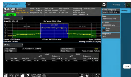
NTNV-n48-PC3-30-30-L-DFT-QPSK-Outer_Full-PASS
