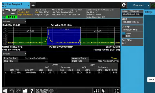
NTNV-n48-PC3-30-30-L-DFT-64QAM-Edge_1RB_Left-PASS
