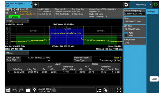
NTNV-n48-PC3-30-30-L-DFT-256QAM-Outer_Full-PASS
