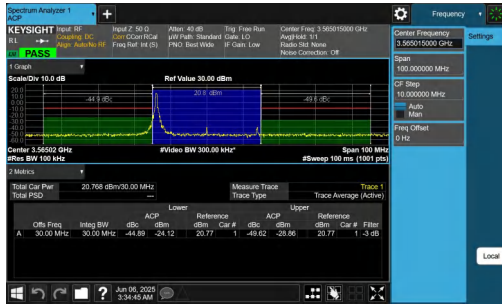
NTNV-n48-PC3-30-30-L-DFT-16QAM-Edge_1RB_Left-PASS
