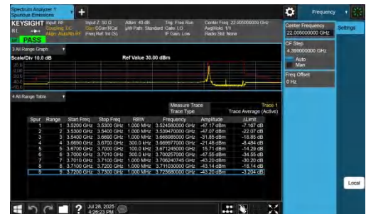
NTNV-n48-PC3-30-30-H-DFT-QPSK-Edge_1RB_Left-PASS
