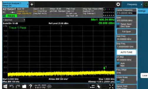
NTNV-n48-PC3-30-10-L-DFT-BPSK-Inner_1RB_Left-30-1000-PASS
