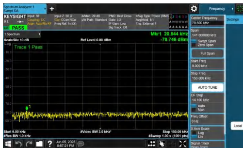
NTNV-n48-PC3-30-10-M-DFT-QPSK-Inner_1RB_Left-0.009-0.15-PASS
