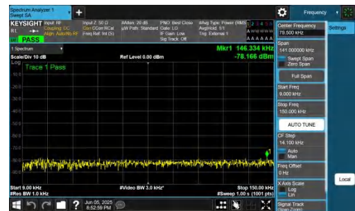
NTNV-n48-PC3-30-10-M-DFT-BPSK-Inner_1RB_Right-0.009-0.15-PASS
