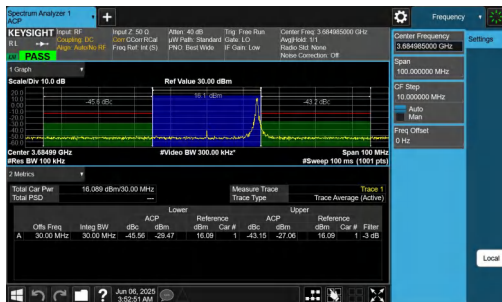
NTNV-n48-PC3-30-30-H-CP-256QAM-Edge_1RB_Right-PASS
