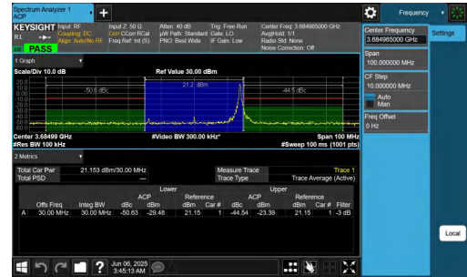
NTNV-n48-PC3-30-30-H-DFT-QPSK-Edge_1RB_Right-PASS
