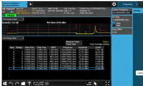
NTNV-n48-PC3-30-40-H-DFT-QPSK-Edge_1RB_Right-PASS
