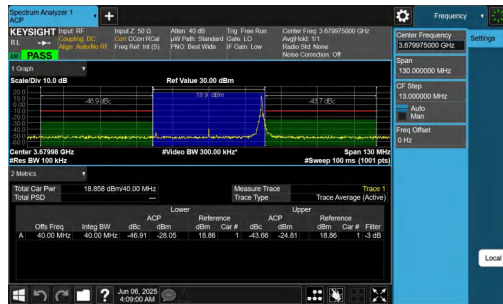
NTNV-n48-PC3-30-40-H-DFT-64QAM-Edge_1RB_Right-PASS
