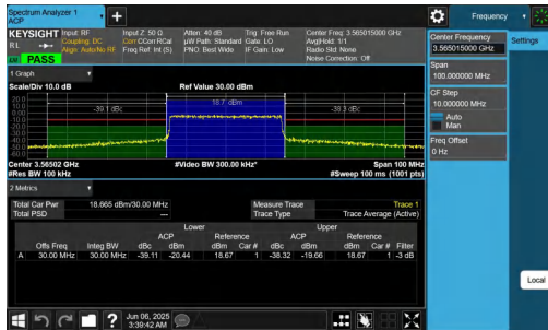
NTNV-n48-PC3-30-30-L-CP-16QAM-Outer_Full-PASS
