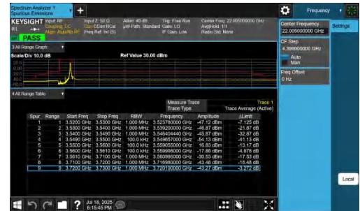
NTNV-n48-PC3-30-10-L-DFT-BPSK-Edge_1RB_Right-PASS
