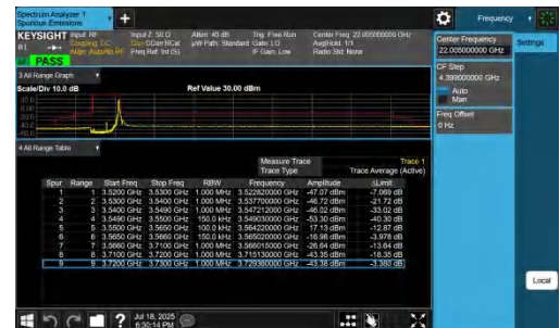
NTNV-n48-PC3-30-15-L-DFT-BPSK-Edge_1RB_Right-PASS
