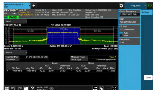
NTNV-n48-PC3-30-40-H-DFT-BPSK-Outer_Full-PASS
