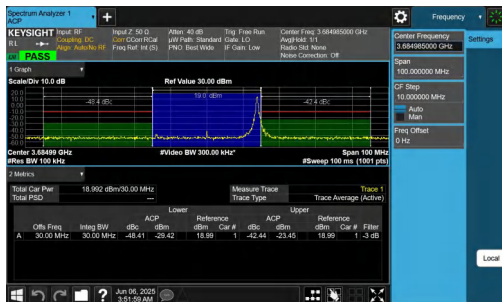
NTNV-n48-PC3-30-30-H-CP-16QAM-Edge_1RB_Right-PASS
