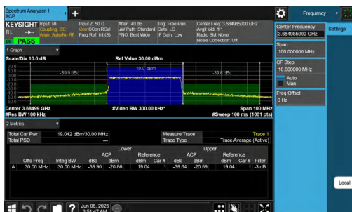
NTNV-n48-PC3-30-30-H-CP-16QAM-Outer_Full-PASS
