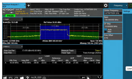
NTNV-n48-PC3-30-40-H-DFT-256QAM-Outer_Full-PASS
