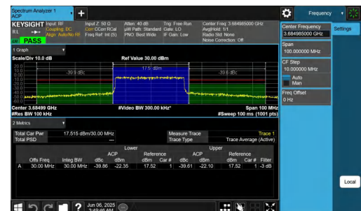
NTNV-n48-PC3-30-30-H-DFT-256QAM-Outer_Full-PASS
