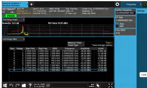
NTNV-n48-PC3-30-10-L-DFT-BPSK-Edge_1RB_Left-PASS
