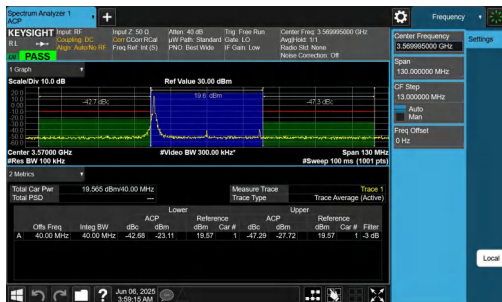
NTVN-n48-PC3-30-40-L-DFT-64QAM-Edge_1RB_Left-PASS
