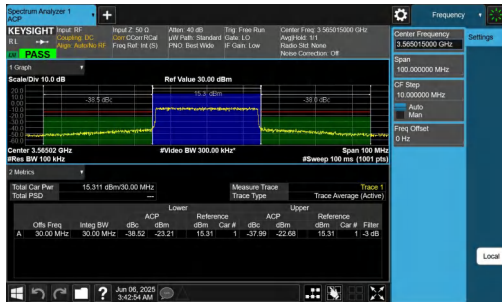
NTNV-n48-PC3-30-30-L-CP-256QAM-Outer_Full-PASS
