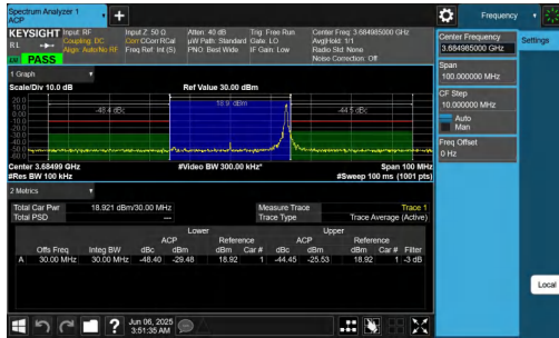
NTVN-n48-PC3-30-30-H-CP-QPSK-Edge_1RB_Right-PASS
