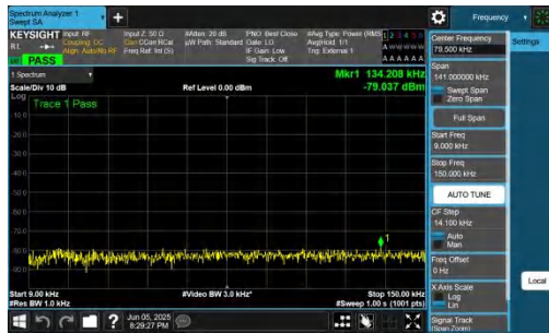
NTNV-n48-PC3-30-10-L-DFT-BPSK-Inner_1RB_Left-0.009-0.15-PASS
