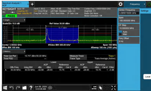
NTNV-n48-PC3-30-30-L-CP-256QAM-Edge_1RB_Left-PASS
