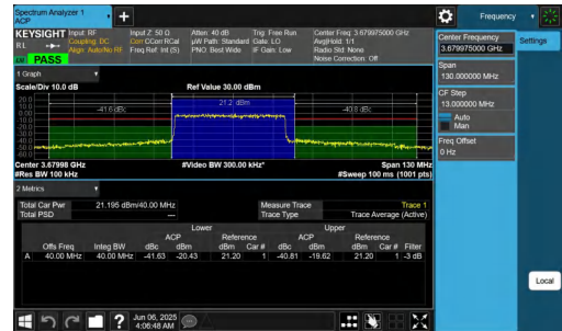
NTNV-n48-PC3-30-40-H-DFT-QPSK-Outer_Full-PASS
