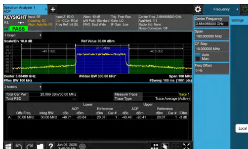
NTNV-n48-PC3-30-30-H-DFT-16QAM-Outer_Full-PASS
