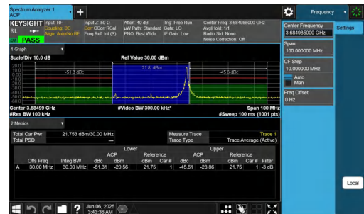
NTNV-n48-PC3-30-30-H-DFT-BPSK-Edge_1RB_Right-PASS
