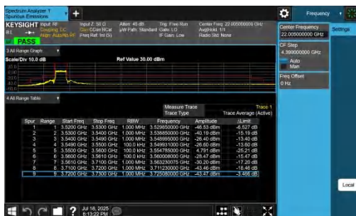
NTNV-n48-PC3-30-10-L-DFT-BPSK-Outer_Full-PASS
