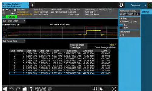
NTNV-n48-PC3-30-30-H-DFT-BPSK-Outer_Full-PASS
