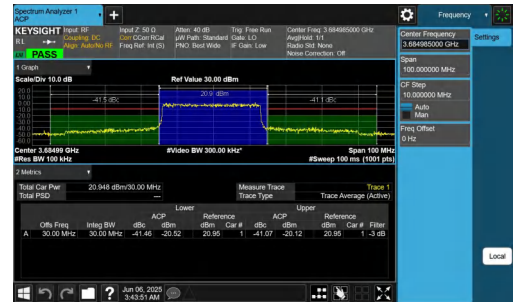
NTNV-n48-PC3-30-30-H-DFT-QPSK-Outer_Full-PASS
