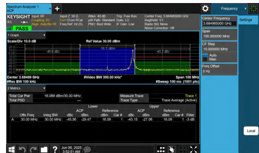
NTNV-n48-PC3-30-30-H-CP-256QAM-Edge_1RB_Right-PASS
