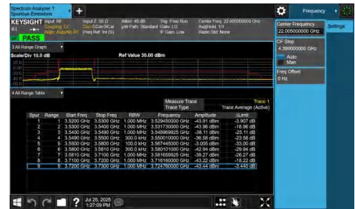
NTNV-n48-PC3-30-30-L-DFT-QPSK-Outer_Full-PASS
