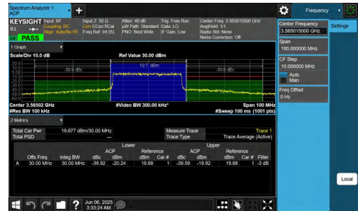
NTNV-n48-PC3-30-30-L-DFT-16QAM-Outer_Full-PASS
