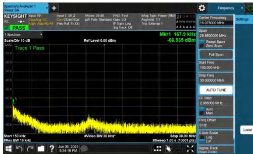
NTNV-n48-PC3-30-10-L-DFT-BPSK-Inner_1RB_Right-0.15-30-P ASS
