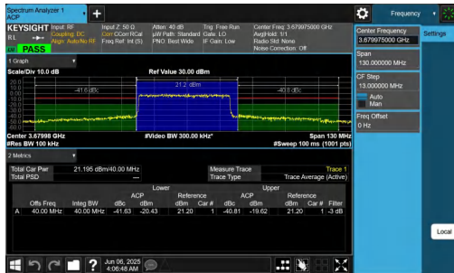
NTNV-n48-PC3-30-40-H-DFT-QPSK-Outer_Full-PASS
