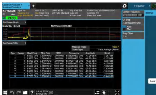
NTNV-n48-PC3-30-10-L-DFT-QPSK-Edge_1RB_Right-PASS
