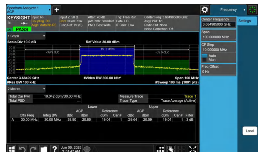
NTNV-n48-PC3-30-30-H-CP-16QAM-Outer_Full-PASS
