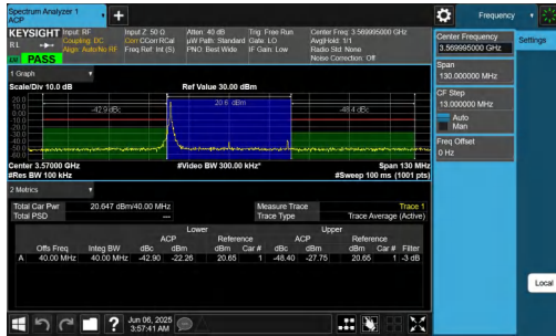
NTVN-n48-PC3-30-40-L-DFT-16QAM-Edge_1RB_Left-PASS
