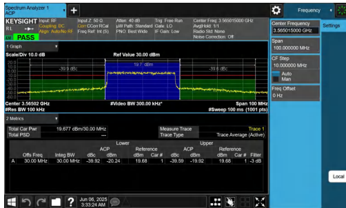
NTNV-n48-PC3-30-30-L-DFT-16QAM-Outer_Full-PASS
