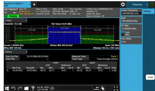
NTNV-n48-PC3-30-30-H-CP-QPSK-Outer_Full-PASS
