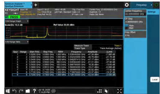
NTNV-n48-PC3-30-40-L-DFT-BPSK-Edge_1RB_Right-PASS
