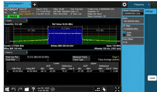
NTNV-n48-PC3-30-40-L-CP-256QAM-Outer_Full-PASS
