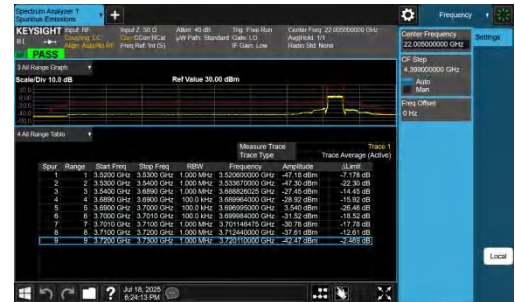
NTNV-n48-PC3-30-10-H-DFT-QPSK-Outer_Full-PASS
