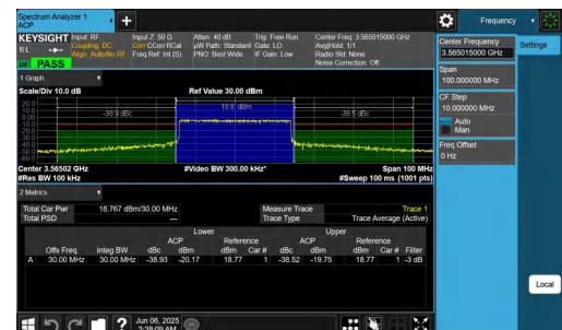
NTNV-n48-PC3-30-30-L-CP-QPSK-Outer_Full-PASS
