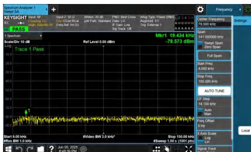
NTNV-n48-PC3-30-10-M-DFT-BPSK-Inner_1RB_Left-0.009-0.15- PASS
