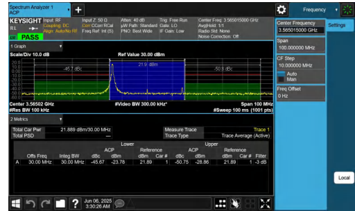
NTNV-n48-PC3-30-30-L-DFT-BPSK-Edge_1RB_Left-PASS
