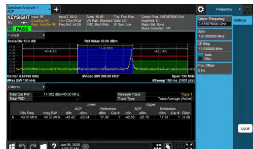
NTNV-n48-PC3-30-40-H-DFT-256QAM-Edge_1RB_Right-PASS
