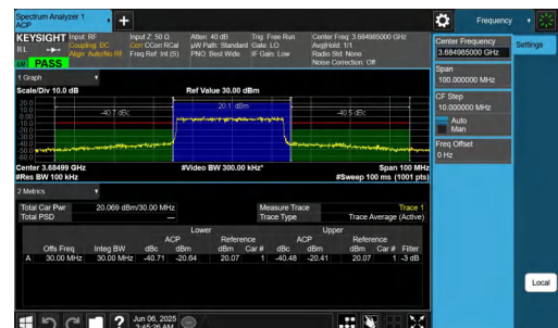
NTNV-n48-PC3-30-30-H-DFT-16QAM-Outer_Full-PASS
