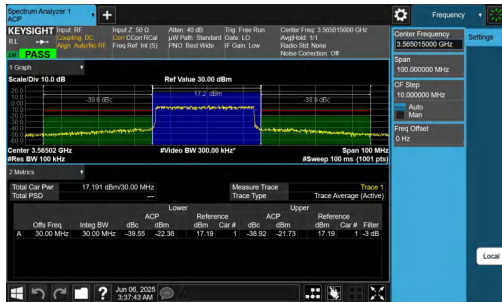
NTNV-n48-PC3-30-30-L-DFT-256QAM-Outer_Full-PASS
