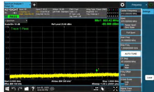
NTNV-n48-PC3-30-10-L-DFT-BPSK-Inner_1RB_Right-30-1000-PA SS
