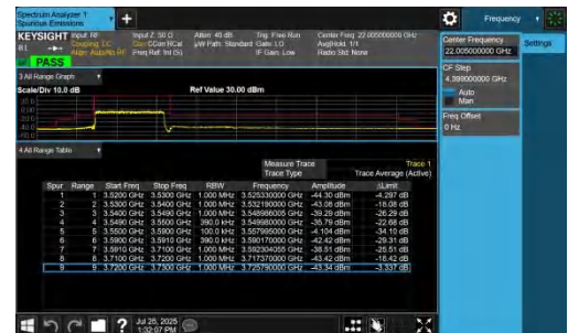
NTNV-n48-PC3-30-40-L-DFT-QPSK-Outer_Full-PASS
