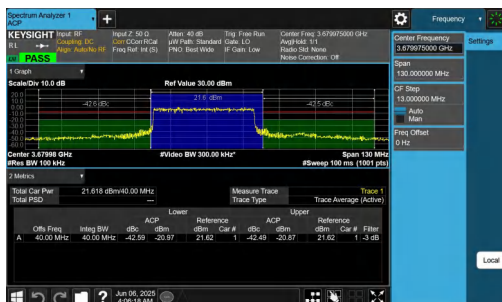
NTNV-n48-PC3-30-40-H-DFT-BPSK-Outer_Full-PASS
