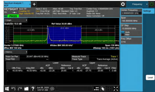
NTVN-n48-PC3-30-40-L-DFT-16QAM-Edge_1RB_Left-PASS
