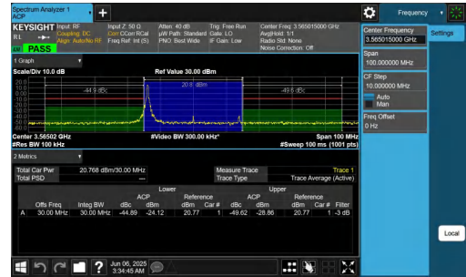
NTNV-n48-PC3-30-30-L-DFT-16QAM-Edge_1RB_Left-PASS
