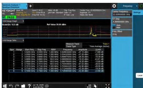
NTNV-n48-PC3-30-10-H-DFT-BPSK-Edge_1RB_Left-PASS
