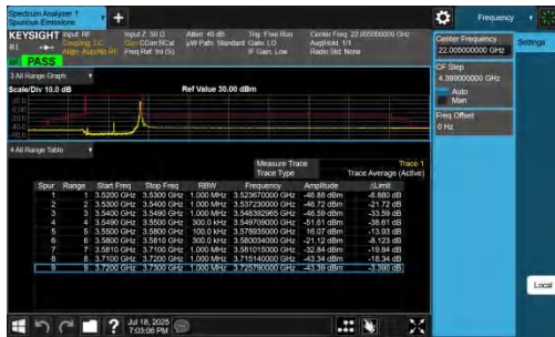
NTNV-n48-PC3-30-30-L-DFT-QPSK-Edge_1RB_Right-PASS
