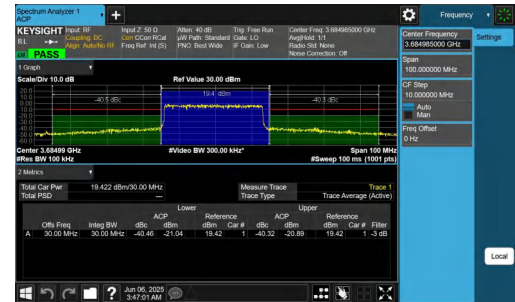
NTNV-n48-PC3-30-30-H-DFT-64QAM-Outer_Full-PASS
