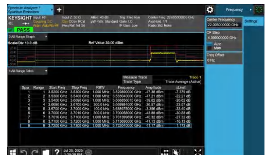
NTNV-n48-PC3-30-30-H-DFT-QPSK-Outer_Full-PASS
