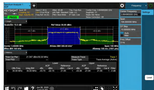
NTNV-n48-PC3-30-30-H-DFT-BPSK-Outer_Full-PASS
