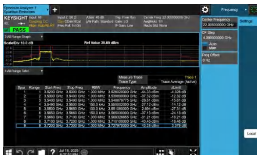
NTNV-n48-PC3-30-15-L-DFT-BPSK-Outer_Full-PASS
