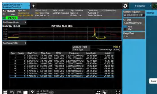
NTNV-n48-PC3-30-20-H-DFT-BPSK-Edge_1RB_Left-PASS
