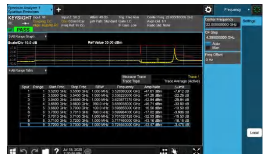
NTNV-n48-PC3-30-40-H-DFT-BPSK-Edge_1RB_Right-PASS
