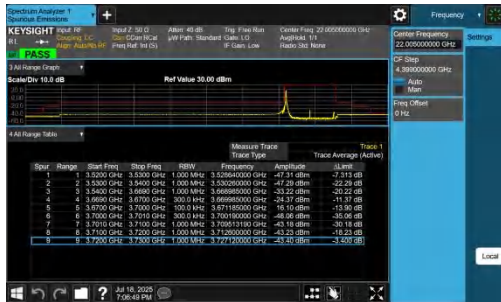
NTNV-n48-PC3-30-30-H-DFT-BPSK-Edge_1RB_Left-PASS
