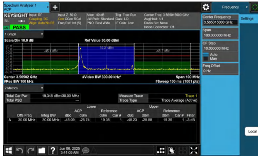
NTNV-n48-PC3-30-30-L-CP-16QAM-Edge_1RB_Left-PASS
