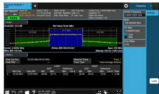
NTNV-n48-PC3-30-30-L-CP-64QAM-Outer_Full-PASS
