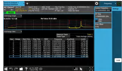
NTNV-n48-PC3-30-30-H-DFT-BPSK-Edge_1RB_Right-PASS
