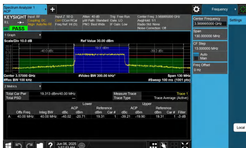
NTVN-n48-PC3-30-40-L-DFT-64QAM-Outer_Full-PASS
