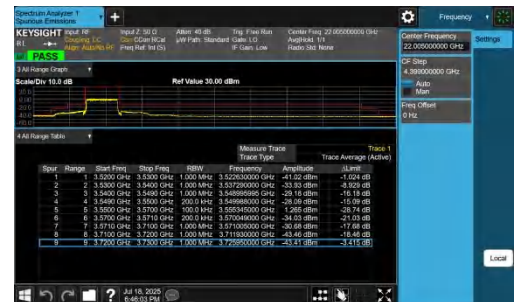
NTNV-n48-PC3-30-20-L-DFT-QPSK-Outer_Full-PASS
