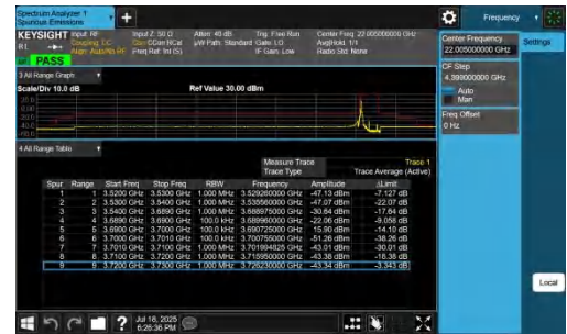
NTNV-n48-PC3-30-10-H-DFT-QPSK-Edge_1RB_Left-PASS
