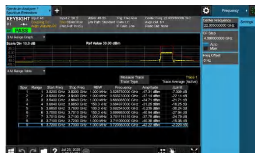
NTNV-n48-PC3-30-15-H-DFT-QPSK-Outer Full-PASS
