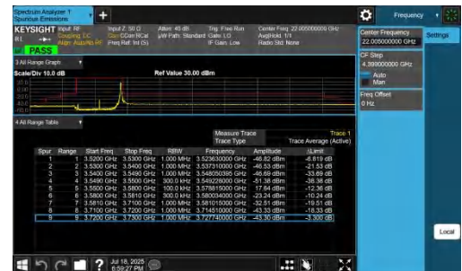
NTNV-n48-PC3-30-30-L-DFT-BPSK-Edge_1RB_Right-PASS
