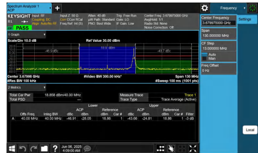
NTNV-n48-PC3-30-40-H-DFT-64QAM-Edge_1RB_Right-PASS
