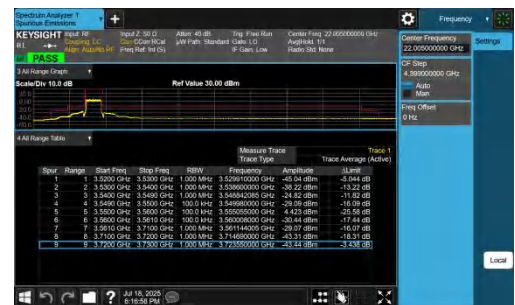
NTNV-n48-PC3-30-10-L-DFT-QPSK-Outer_Full-PASS
