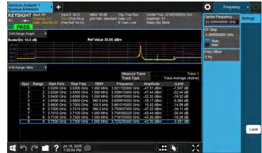
NTNV-n48-PC3-30-40-H-DFT-QPSK-Edge_1RB_Left-PASS
