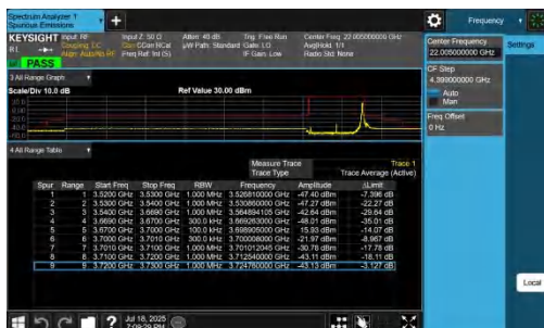
NTNV-n48-PC3-30-30-H-DFT-QPSK-Edge_1RB_Right-PASS
