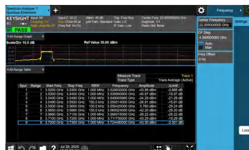
NTNV-n48-PC3-30-15-L-DFT-QPSK-Outer Full-PASS
