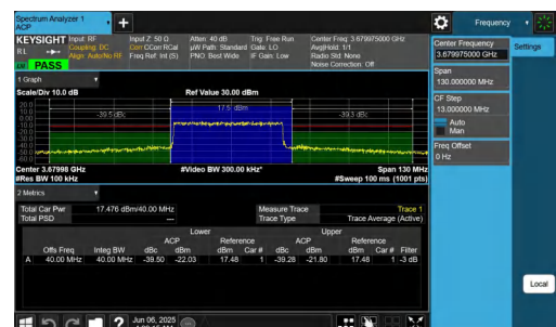
NTNV-n48-PC3-30-40-H-DFT-256QAM-Outer_Full-PASS
