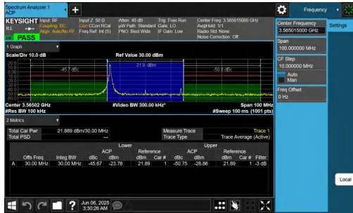
NTNV-n48-PC3-30-30-L-DFT-BPSK-Edge_1RB_Left-PASS
