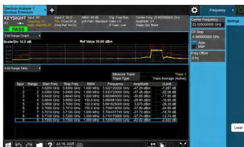
NTNV-n48-PC3-30-15-H-DFT-BPSK-Outer Full-PASS
