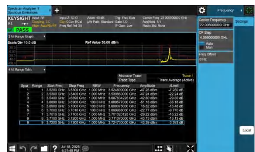
NTNV-n48-PC3-30-10-H-DFT-BPSK-Edge_1RB_Right-PASS
