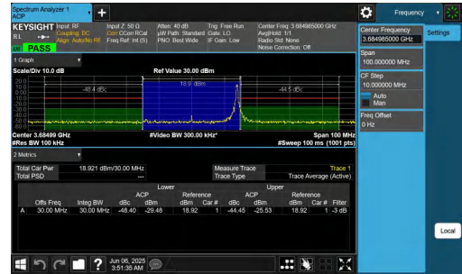
NTVN-n48-PC3-30-30-H-CP-QPSK-Edge_1RB_Right-PASS
