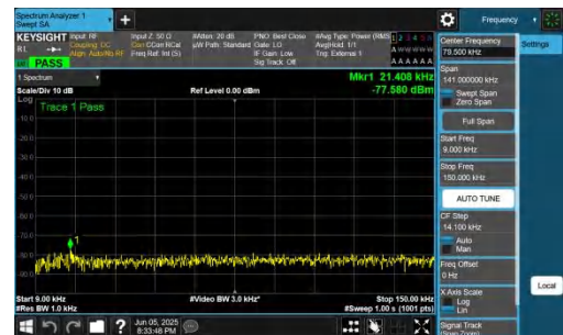
NTNV-n48-PC3-30-10-L-DFT-BPSK-Inner_1RB_Right-0.009-0.15-PASS
