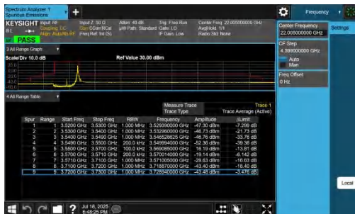
NTNV-n48-PC3-30-20-L-DFT-QPSK-Edge_1RB_Right-PASS
