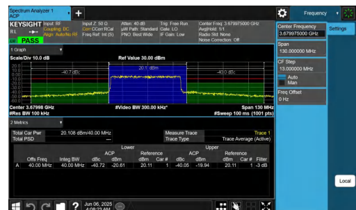
NTNV-n48-PC3-30-40-H-DFT-16QAM-Outer_Full-PASS
