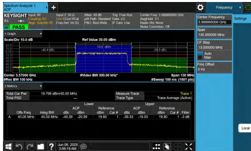
NTVN-n48-PC3-30-40-L-DFT-16QAM-Outer_Full-PASS
