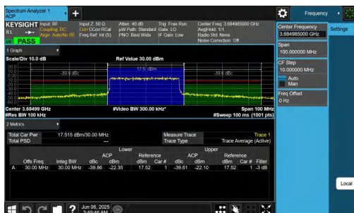
NTNV-n48-PC3-30-30-H-DFT-256QAM-Outer_Full-PASS
