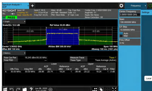
NTNV-n48-PC3-30-30-L-CP-64QAM-Outer_Full-PASS
