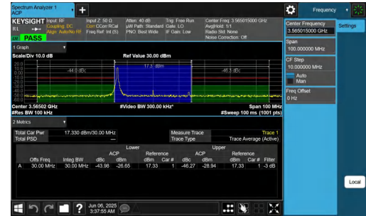
NTNV-n48-PC3-30-30-L-DFT-256QAM-Edge_1RB_Left-PASS
