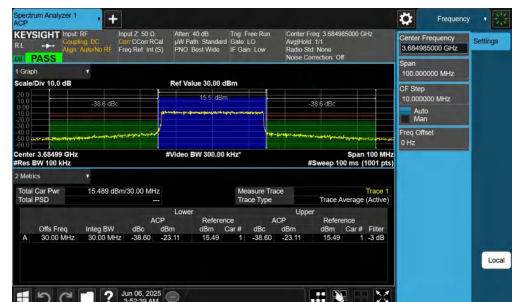
NTNV-n48-PC3-30-30-H-CP-256QAM-Outer_Full-PASS
