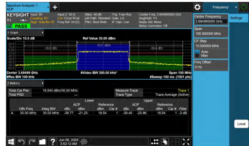
NTNV-n48-PC3-30-30-H-CP-64QAM-Outer_Full-PASS
