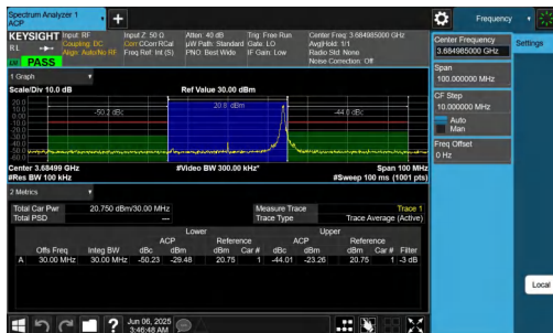
NTNV-n48-PC3-30-30-H-DFT-16QAM-Edge_1RB_Right-PASS
