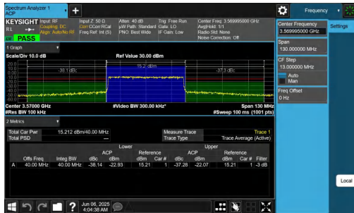
NTNV-n48-PC3-30-40-L-CP-256QAM-Outer_Full-PASS
