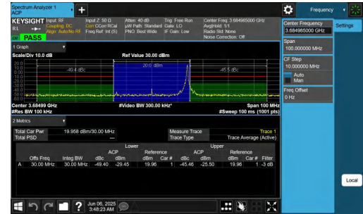
NTNV-n48-PC3-30-30-H-DFT-64QAM-Edge_1RB_Right-PASS
