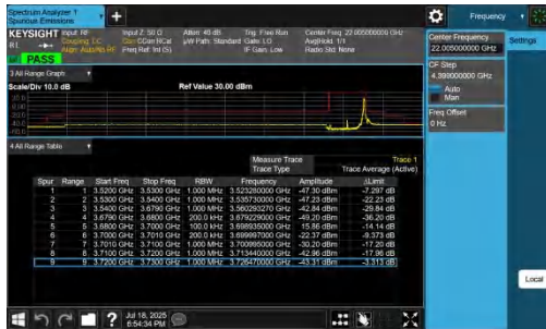
NTNV-n48-PC3-30-20-H-DFT-QPSK-Edge_1RB_Right-PASS
