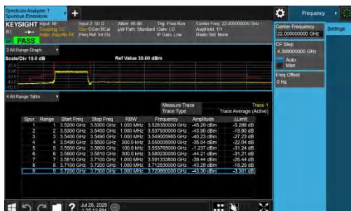
NTNV-n48-PC3-30-30-L-DFT-BPSK-Outer_Full-PASS
