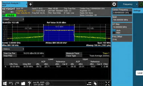
NTNV-n48-PC3-30-30-H-CP-QPSK-Outer_Full-PASS
