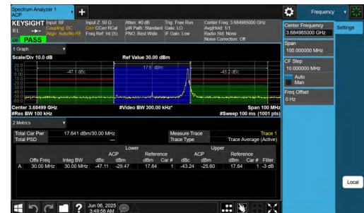
NTNV-n48-PC3-30-30-H-DFT-256QAM-Edge_1RB_Right-PASS
