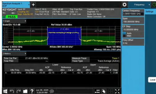
NTNV-n48-PC3-30-30-L-DFT-BPSK-Outer_Full-PASS
