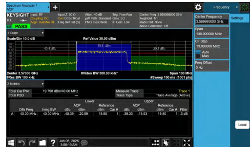
NTVN-n48-PC3-30-40-L-DFT-16QAM-Outer_Full-PASS
