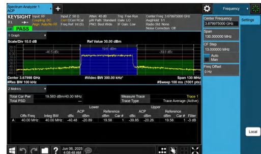
NTNV-n48-PC3-30-40-H-DFT-64QAM-Outer_Full-PASS
