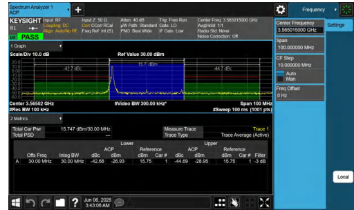
NTNV-n48-PC3-30-30-L-CP-256QAM-Edge_1RB_Left-PASS
