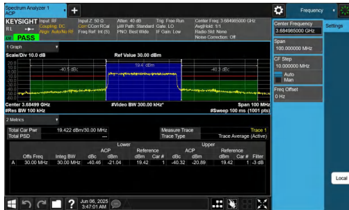
NTNV-n48-PC3-30-30-H-DFT-64QAM-Outer_Full-PASS
