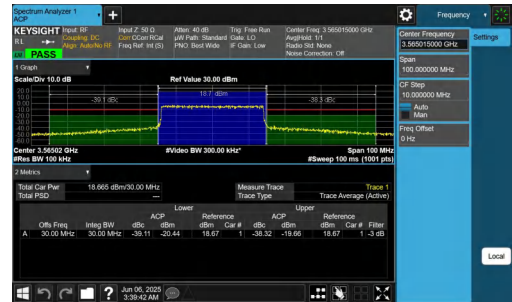
NTNV-n48-PC3-30-30-L-CP-16QAM-Outer_Full-PASS
