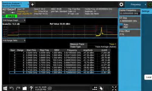
NTNV-n48-PC3-30-10-H-DFT-QPSK-Edge_1RB_Right-PASS
