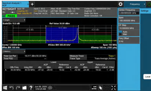
NTNV-n48-PC3-30-30-H-CP-64QAM-Edge_1RB_Right-PASS
