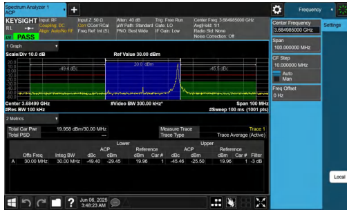
NTNV-n48-PC3-30-30-H-DFT-64QAM-Edge_1RB_Right-PASS
