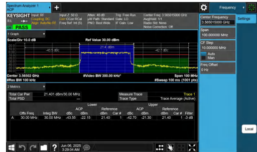
NTNV-n48-PC3-30-30-L-DFT-BPSK-Outer_Full-PASS
