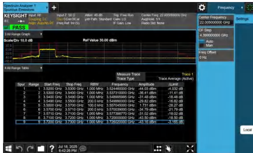
NTNV-n48-PC3-30-20-L-DFT-BPSK-Outer_Full-PASS
