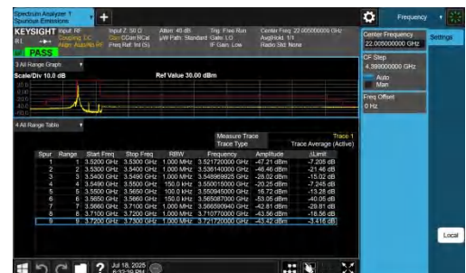
NTNV-n48-PC3-30-15-L-DFT-QPSK-Edge_1RB_Left-PASS
