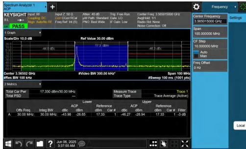
NTNV-n48-PC3-30-30-L-DFT-256QAM-Edge_1RB_Left-PASS
