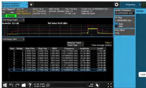
NTNV-n48-PC3-30-20-H-DFT-BPSK-Outer_Full-PASS
