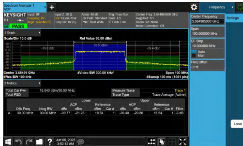
NTNV-n48-PC3-30-30-H-CP-64QAM-Outer_Full-PASS
