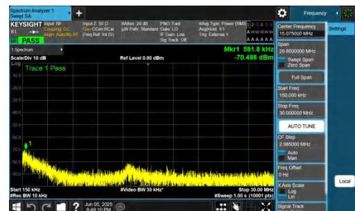
NTNV-n48-PC3-30-10-M-DFT-BPSK-Inner_1RB_Left-0.15-30-PAS S
