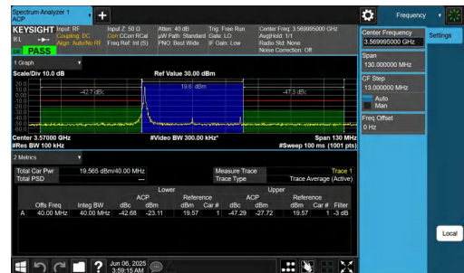
NTVN-n48-PC3-30-40-L-DFT-64QAM-Edge_1RB_Left-PASS
