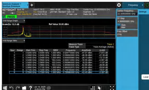
NTNV-n48-PC3-30-15-L-DFT-BPSK-Edge_1RB_Left-PASS
