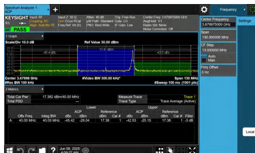
NTNV-n48-PC3-30-40-H-DFT-256QAM-Edge_1RB_Right-PASS
