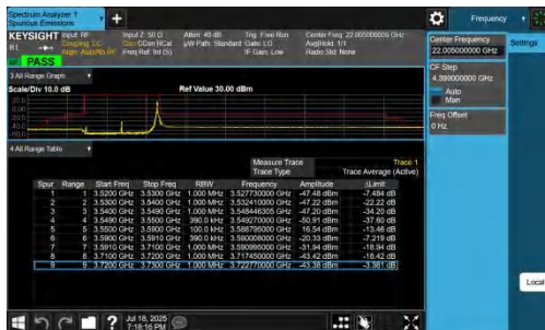
NTNV-n48-PC3-30-40-L-DFT-QPSK-Edge_1RB_Right-PASS
