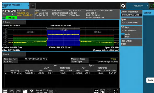
NTNV-n48-PC3-30-30-H-CP-256QAM-Outer_Full-PASS
