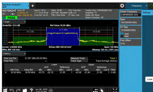
NTNV-n48-PC3-30-30-H-DFT-BPSK-Outer_Full-PASS
