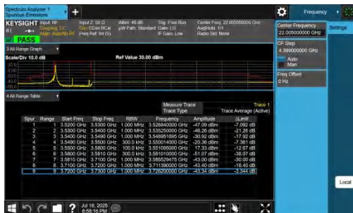
NTNV-n48-PC3-30-30-L-DFT-BPSK-Edge_1RB_Left-PASS
