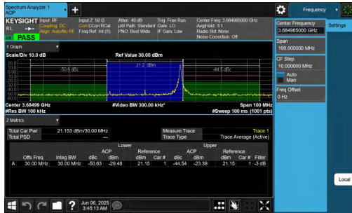
NTNV-n48-PC3-30-30-H-DFT-QPSK-Edge_1RB_Right-PASS
