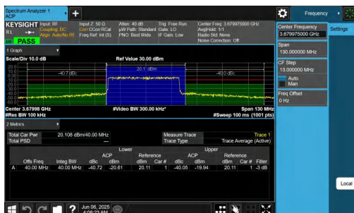
NTNV-n48-PC3-30-40-H-DFT-16QAM-Outer_Full-PASS
