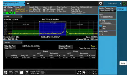
NTNV-n48-PC3-30-30-H-CP-64QAM-Edge_1RB_Right-PASS
