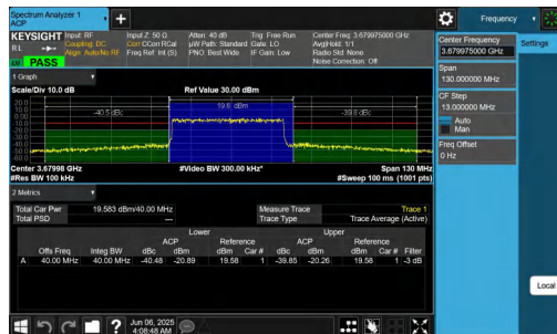
NTNV-n48-PC3-30-40-H-DFT-64QAM-Outer_Full-PASS
