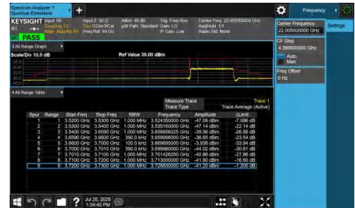
NTNV-n48-PC3-30-40-H-DFT-QPSK-Outer_Full-PASS
