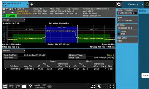
NTNV-n48-PC3-30-30-H-DFT-QPSK-Outer_Full-PASS
