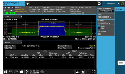
NTNV-n48-PC3-30-30-L-CP-256QAM-Outer_Full-PASS
