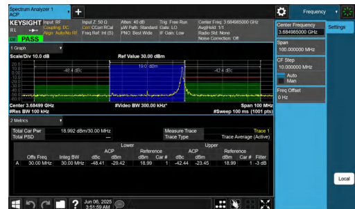
NTNV-n48-PC3-30-30-H-CP-16QAM-Edge_1RB_Right-PASS
