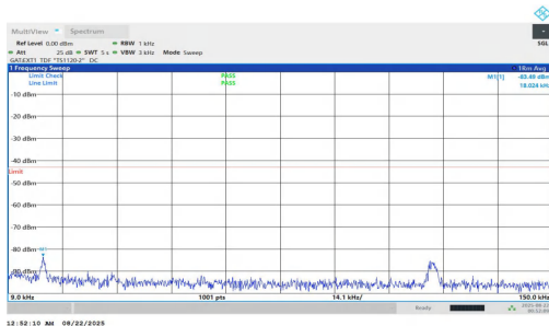
NTNV-n78(3700-3800)-PC1.5-30-50-M-DFT-BPSK-Inner_1RB_Left-0.009-0.15-PASS
