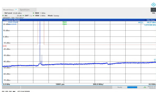
NTNV-n78(3700-3800)-PC1.5-30-40-M-DFT-QPSK-Inner_1RB_Left-3 000-6000-PASS
