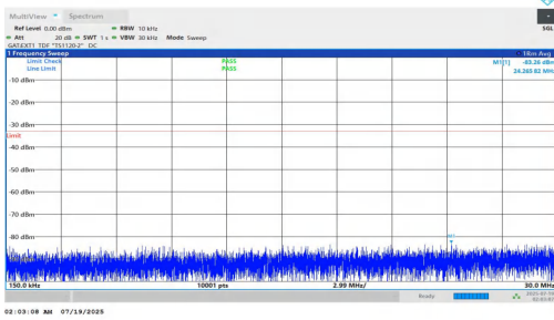
NTNV-n78(3700-3800)-PC1.5-30-40-M-DFT-BPSK-Inner_1RB_Right-0.15-30-PASS
