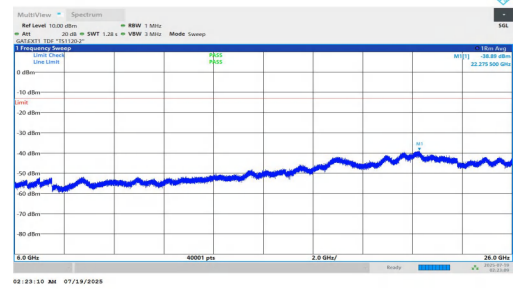
NTNV-n78(3700-3800)-PC1.5-30-50-M-DFT-BPSK-Inner_1RB_Left-60 00-26000-PASS
