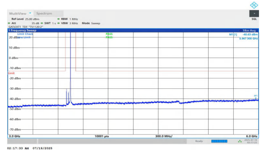
NTNV-n78(3700-3800)-PC1.5-30-50-L-DFT-BPSK-Inner_1RB_Right-3 000-6000-PASS
