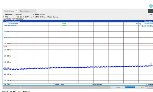
NTNV-n78(3700-3800)-PC1.5-30-40-H-DFT-BPSK-Inner_1RB_Left-1000-3000-PASS
