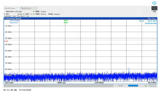
NTNV-n78(3700-3800)-PC1.5-30-40-H-DFT-QPSK-Inner_1RB_Left-0.15-30-PASS
