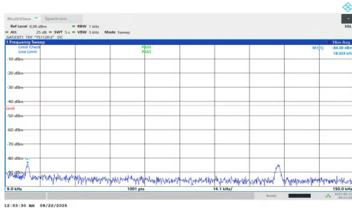
NTNV-n78(3700-3800)-PC1.5-30-50-M-DFT-QPSK-Inner_1RB_Left-0.009-0.15-PASS
