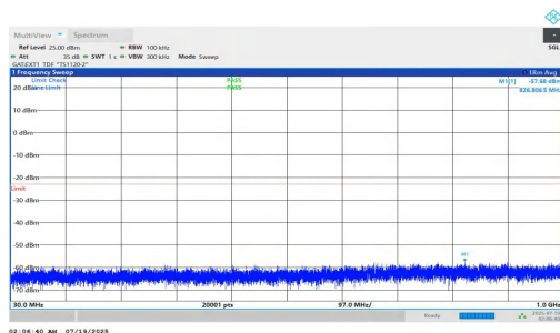
NTNV-n78(3700-3800)-PC1.5-30-40-M-DFT-QPSK-Inner_1RB_Right- 30-1000-PASS
