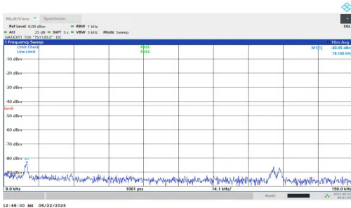
NTNV-n78(3700-3800)-PC1.5-30-40-H-DFT-QPSK-Inner_1RB_Left-0.009-0.15-PASS
