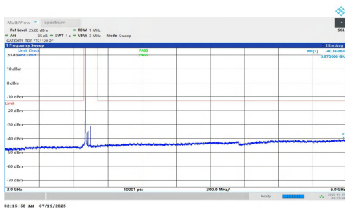
NTV-n78(3700-3800)-PC1.5-30-50-L-DFT-BPSK-Inner_1RB_Left-3000-6000-PASS
