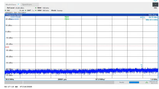
NTNV-n78(3700-3800)-PC1.5-30-50-L-DFT-BPSK-Inner_1RB_Right-3 0-1000-PASS
