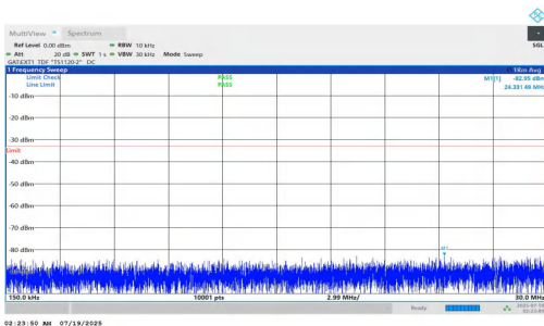
NTNV-n78(3700-3800)-PC1.5-30-50-M-DFT-BPSK-Inner_1RB_Right- 0.15-30-PASS
