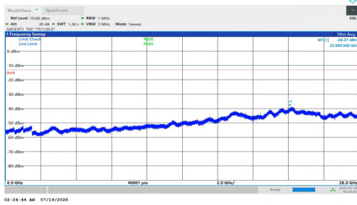
NTNV-n78(3700-3800)-PC1.5-30-50-M-DFT-BPSK-Inner_1RB_Right-6000-26000-PASS
