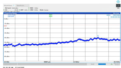
NTNV-n78(3700-3800)-PC1.5-30-40-M-DFT-BPSK-Inner_1RB_Left-6000-26000-PASS
