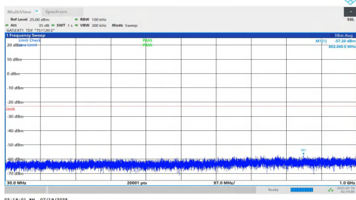
NTNV-n78(3700-3800)-PC1.5-30-50-L-DFT-QPSK-Inner_1RB_Left-3 0-1000-PASS
