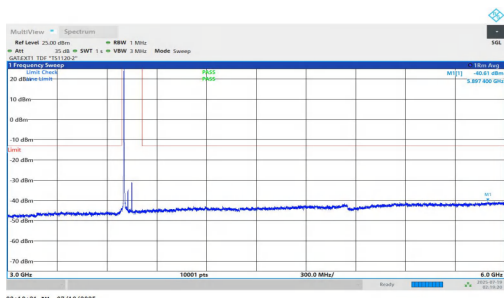
NTNV-n78(3700-3800)-PC1.5-30-50-L-DFT-QPSK-Inner_1RB_Left-3 000-6000-PASS
