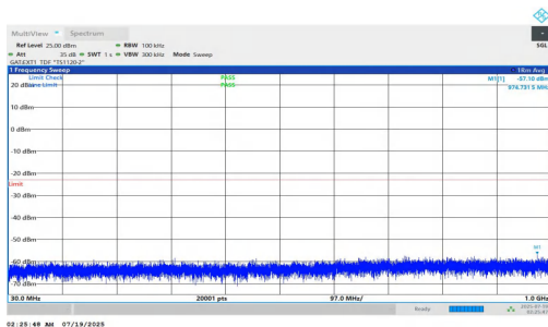
NTNV-n78(3700-3800)-PC1.5-30-50-M-DFT-QPSK-Inner_1RB_Left-30-1000-PASS
