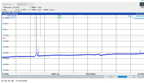
NTNV-n78(3700-3800)-PC1.5-30-50-M-DFT-BPSK-Inner_1RB_Left-3 000-6000-PASS
