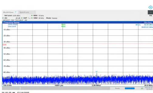
NTNV-n78(3700-3800)-PC1.5-30-50-L-DFT-QPSK-Inner_1RB_Right- 0.15-30-PASS
