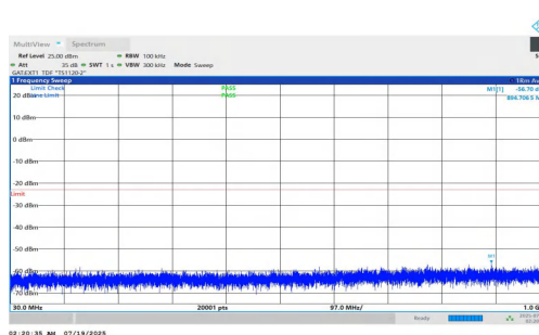
NTNV-n78(3700-3800)-PC1.5-30-50-L-DFT-QPSK-Inner_1RB_Right-3 0-1000-PASS
