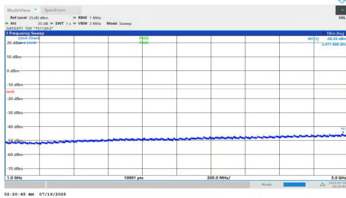
NTNV-n78(3700-3800)-PC1.5-30-50-L-DFT-QPSK-Inner_1RB_Right-1000-3000-PASS
