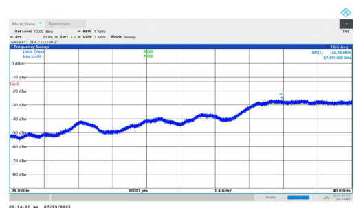
NTNV-n78(3700-3800)-PC1.5-30-40-H-DFT-QPSK-Inner_1RB_Right-2 6000-40000-PASS
