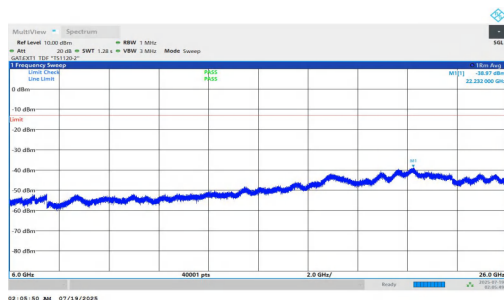
NTNV-n78(3700-3800)-PC1.5-30-40-M-DFT-QPSK-Inner_1RB_Left-60 00-26000-PASS
