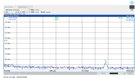
NTVN-n78(3700-3800)-PC1.5-30-40-H-DFT-BPSK-Inner_1RB_Right-0 .009-0.15-PASS
