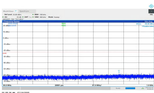
NTNV-n78(3700-3800)-PC1.5-30-40-H-DFT-BPSK-Inner_1RB_Left-300-1000-PASS
