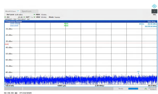
NTNV-n78(3700-3800)-PC1.5-30-40-M-DFT-QPSK-Inner_1RB_Left-0.15-30-PASS
