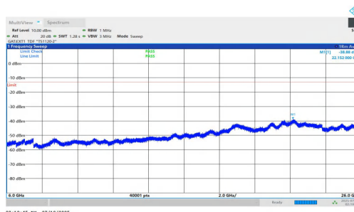
NTNV-n78(3700-3800)-PC1.5-30-50-L-DFT-QPSK-Inner_1RB_Left-60 00-26000-PASS
