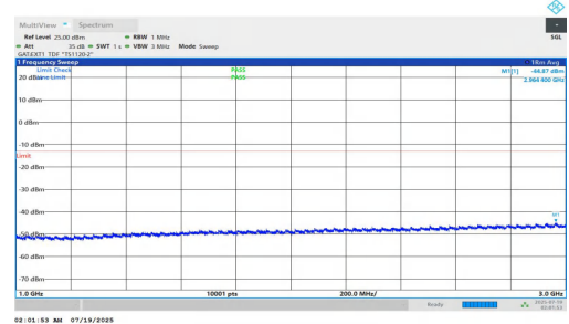
NTNV-n78(3700-3800)-PC1.5-30-40-M-DFT-BPSK-Inner_1RB_Left-1000-3000-PASS
