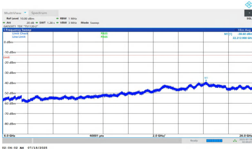
NTNV-n78(3700-3800)-PC1.5-30-40-M-DFT-BPSK-Inner_1RB_Right-6000-26000-PASS
