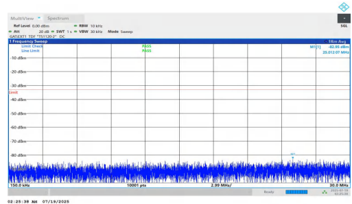
NTNV-n78(3700-3800)-PC1.5-30-50-M-DFT-QPSK-Inner_1RB_Left-0.15-30-PASS
