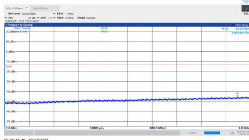
NTNV-n78(3700-3800)-PC1.5-30-40-M-DFT-QPSK-Inner_1RB_Left-10 00-3000-PASS
