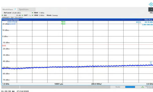
NTNV-n78(3700-3800)-PC1.5-30-40-L-DFT-QPSK-Inner_1RB_Right- 1000-3000-PASS
