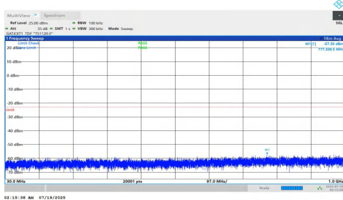
NTV-n78(3700-3800)-PC1.5-30-50-L-DFT-BPSK-Inner_1RB_Left-30-1000-PASS
