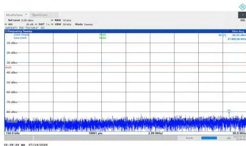
NTNV-n78(3700-3800)-PC1.5-30-40-H-DFT-BPSK-Inner_1RB_Left-0.15-30-PASS
