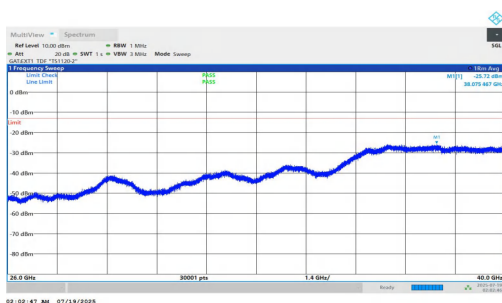
NTNV-n78(3700-3800)-PC1.5-30-40-M-DFT-BPSK-Inner_1RB_Left-26000-40000-PASS
