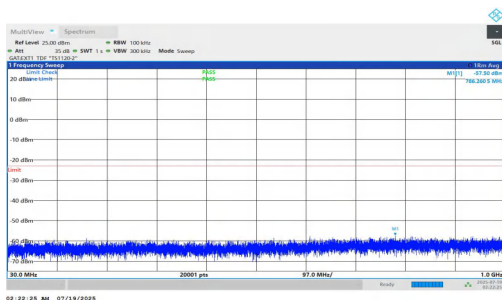
NTNV-n78(3700-3800)-PC1.5-30-50-M-DFT-BPSK-Inner_1RB_Left-30-1000-PASS
