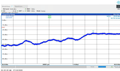
NTNV-n78(3700-3800)-PC1.5-30-50-M-DFT-BPSK-Inner_1RB_Left-2 6000-40000-PASS
