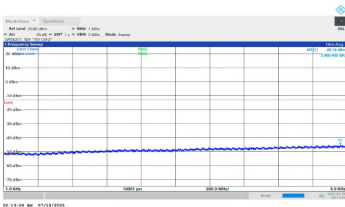
NTNV-n78(3700-3800)-PC1.5-30-40-H-DFT-QPSK-Inner_1RB_Right- 1000-3000-PASS
