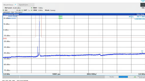
NTNV-n78(3700-3800)-PC1.5-30-40-M-DFT-QPSK-Inner_1RB_Right-3000-6000-PASS
