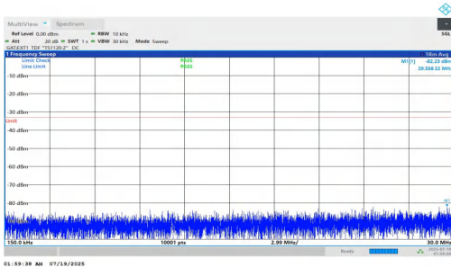
NTNV-n78(3700-3800)-PC1.5-30-40-L-DFT-QPSK-Inner_1RB_Right- 0.15-30-PASS
