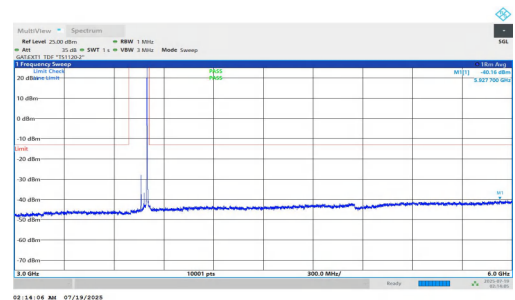
NTNV-n78(3700-3800)-PC1.5-30-40-H-DFT-QPSK-Inner_1RB_Right-3 000-6000-PASS
