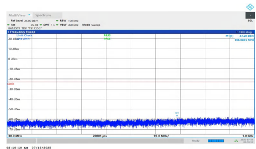
NTVN-n78(3700-3800)-PC1.5-30-40-H-DFT-BPSK-Inner_1RB_Right-3 0-1000-PASS
