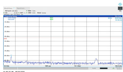
NTNV-n78(3700-3800)-PC1.5-30-40-M-DFT-BPSK-Inner_1RB_Right-0.009-0.15-PASS
