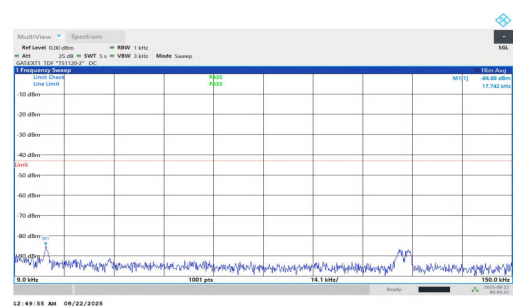
NTV-n78(3700-3800)-PC1.5-30-50-L-DFT-BPSK-Inner_1RB_Right-0.009-0.15-PASS
