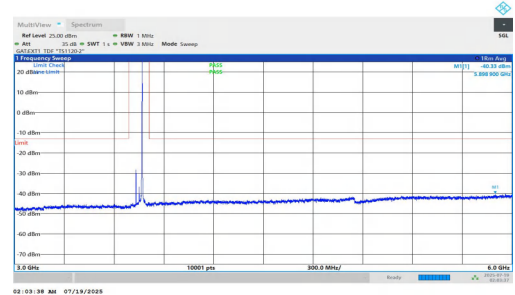
NTNV-n78(3700-3800)-PC1.5-30-40-M-DFT-BPSK-Inner_1RB_Right-3000-6000-PASS
