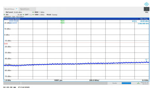
NTNV-n78(3700-3800)-PC1.5-30-50-M-DFT-QPSK-Inner_1RB_Left-1000-3000-PASS
