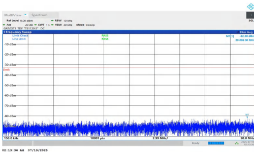
NTNV-n78(3700-3800)-PC1.5-30-40-H-DFT-QPSK-Inner_1RB_Right- 0.15-30-PASS
