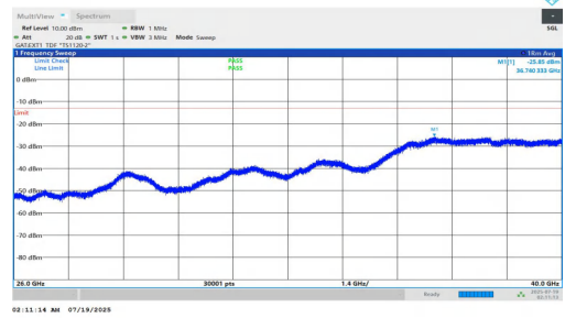
NTNV-n78(3700-3800)-PC1.5-30-40-H-DFT-BPSK-Inner_1RB_Right-26000-40000-PASS
