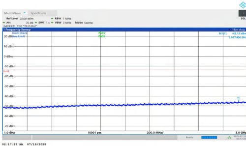
NTNV-n78(3700-3800)-PC1.5-30-50-L-DFT-BPSK-Inner_1RB_Right-1000-3000-PASS
