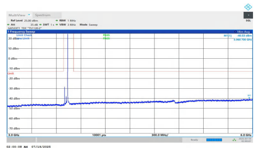
NTNV-n78(3700-3800)-PC1.5-30-40-L-DFT-QPSK-Inner_1RB_Right-3 000-6000-PASS
