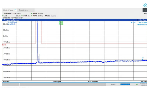
NTNV-n78(3700-3800)-PC1.5-30-50-M-DFT-QPSK-Inner_1RB_Left-3000-6000-PASS
