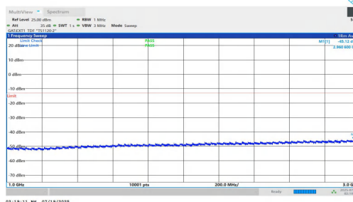
NTNV-n78(3700-3800)-PC1.5-30-50-L-DFT-QPSK-Inner_1RB_Left-10 00-3000-PASS
