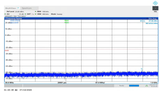
NTNV-n78(3700-3800)-PC1.5-30-20-M-DFT-QPSK-Inner_1RB_Right- 30-1000-PASS
