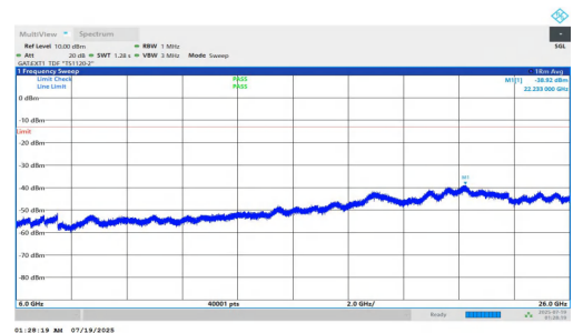
NTNV-n78(3700-3800)-PC1.5-30-20-H-DFT-BPSK-Inner_1RB_Left-6000-26000-PASS
