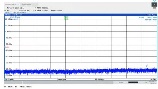
NTNV-n78(3700-3800)-PC1.5-30-25-M-DFT-BPSK-Inner_1RB_Right-3 0-1000-PASS
