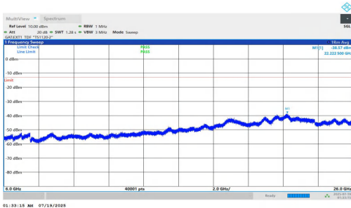
NTNV-n78(3700-3800)-PC1.5-30-20-H-DFT-QPSK-Inner_1RB_Right-6000-26000-PASS
