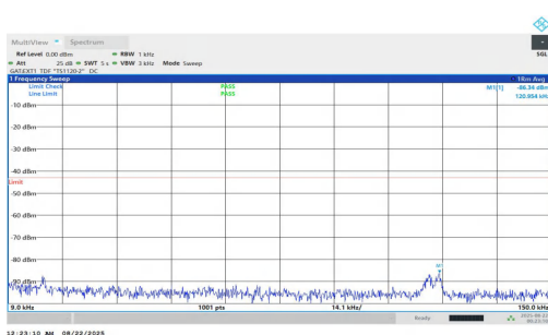
NTNV-n78(3700-3800)-PC1.5-30-20-H-DFT-QPSK-Inner_1RB_Left-0.009-0.15-PASS
