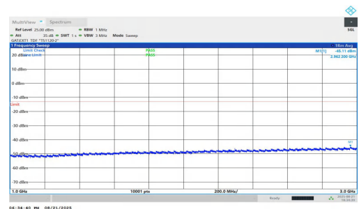
NTNV-n78(3700-3800)-PC1.5-30-25-L-DFT-BPSK-Inner_1RB_Left-1000-3000-PASS
