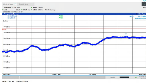
NTVN-n78(3700-3800)-PC1.5-30-25-L-DFT-QPSK-Inner_1RB_Left-2 6000-40000-PASS
