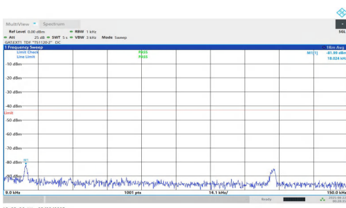
NTNV-n78(3700-3800)-PC1.5-30-25-M-DFT-QPSK-Inner_1RB_Left-0.009-0.15-PASS
