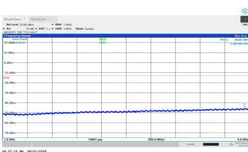
NTNV-n78(3700-3800)-PC1.5-30-25-L-DFT-BPSK-Inner_1RB_Right- 1000-3000-PASS
