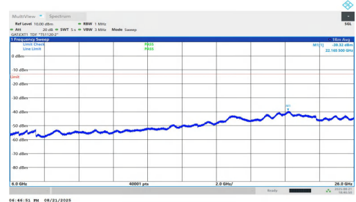
NTNV-n78(3700-3800)-PC1.5-30-25-M-DFT-BPSK-Inner_1RB_Left-6000-26000-PASS
