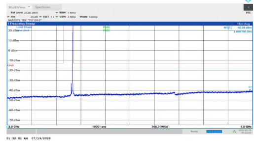
NTNV-n78(3700-3800)-PC1.5-30-20-H-DFT-QPSK-Inner_1RB_Right-3000-6000-PASS
