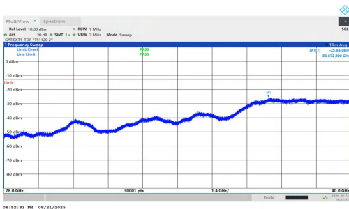
NTNV-n78(3700-3800)-PC1.5-30-25-M-DFT-QPSK-Inner_1RB_Left-2 6000-40000-PASS
