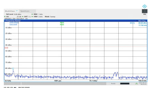
NTNV-n78(3700-3800)-PC1.5-30-20-H-DFT-BPSK-Inner_1RB_Right-0.009-0.15-PASS
