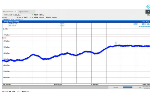
NTNV-n78(3700-3800)-PC1.5-30-20-H-DFT-BPSK-Inner_1RB_Left-26000-40000-PASS
