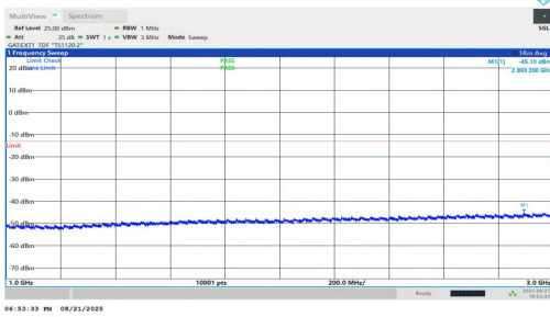
NTNV-n78(3700-3800)-PC1.5-30-25-M-DFT-QPSK-Inner_1RB_Right-1000-3000-PASS
