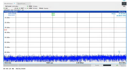
NTNV-n78(3700-3800)-PC1.5-30-25-M-DFT-BPSK-Inner_1RB_Left-0.15-30-PASS
