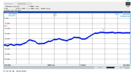
NTNV-n78(3700-3800)-PC1.5-30-25-H-DFT-BPSK-Inner_1RB_Right-26000-40000-PASS
