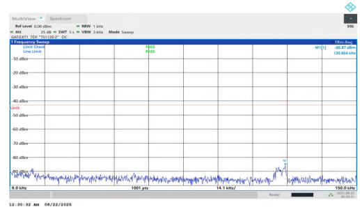
NTNV-n78(3700-3800)-PC1.5-30-25-H-DFT-BPSK-Inner_1RB_Right-0 .009-0.15-PASS
