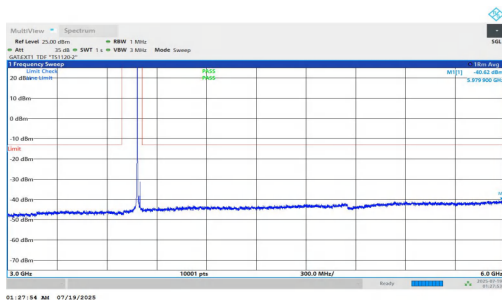
NTNV-n78(3700-3800)-PC1.5-30-20-H-DFT-BPSK-Inner_1RB_Left-3000-6000-PASS
