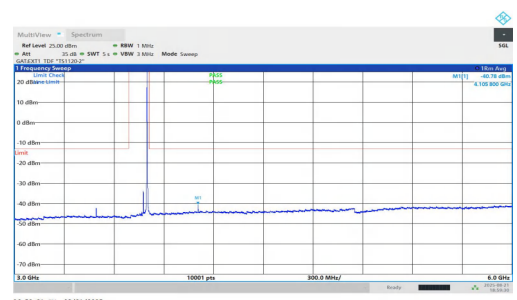
NTNV-n78(3700-3800)-PC1.5-30-25-H-DFT-BPSK-Inner_1RB_Right-3 000-6000-PASS
