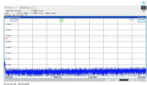
NTVN-n78(3700-3800)-PC1.5-30-25-L-DFT-QPSK-Inner_1RB_Left-0.15-5-30-PASS
