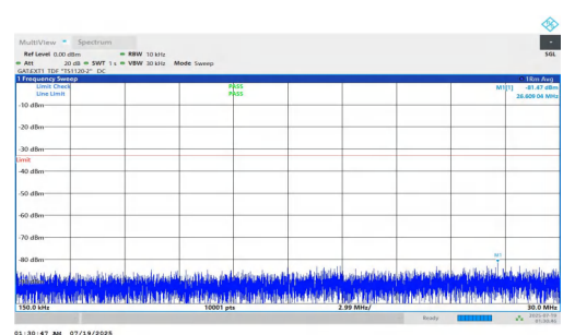
NTNV-n78(3700-3800)-PC1.5-30-20-H-DFT-QPSK-Inner_1RB_Left-0.15-30-PASS
