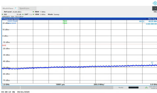
NTNV-n78(3700-3800)-PC1.5-30-25-M-DFT-BPSK-Inner_1RB_Right-1000-3000-PASS
