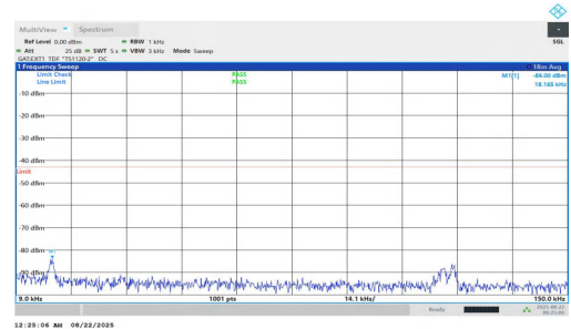
NTNV-n78(3700-3800)-PC1.5-30-25-L-DFT-BPSK-Inner_1RB_Right-0. 009-0.15-PASS
