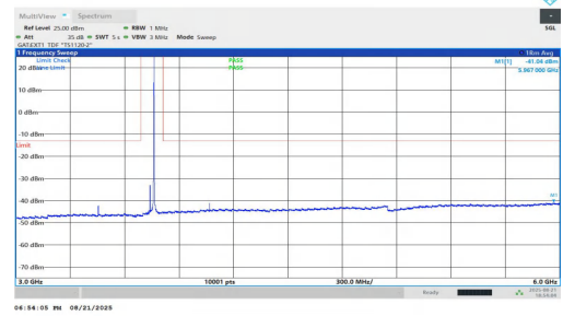
NTNV-n78(3700-3800)-PC1.5-30-25-M-DFT-QPSK-Inner_1RB_Right-3000-6000-PASS
