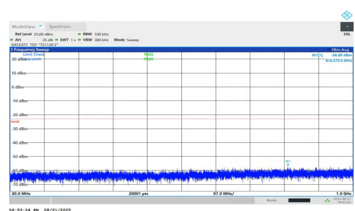
NTNV-n78(3700-3800)-PC1.5-30-25-M-DFT-QPSK-Inner_1RB_Right- 30-1000-PASS
