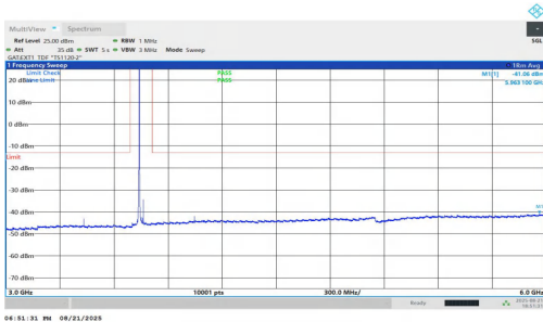
NTNV-n78(3700-3800)-PC1.5-30-25-M-DFT-QPSK-Inner_1RB_Left-3 000-6000-PASS
