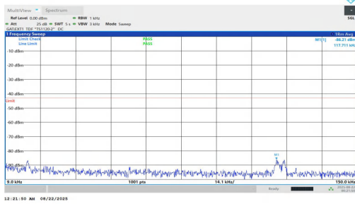
NTNV-n78(3700-3800)-PC1.5-30-20-H-DFT-BPSK-Inner_1RB_Left-0.009-0.15-PASS
