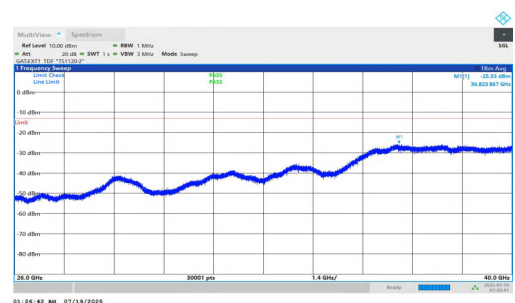
NTNV-n78(3700-3800)-PC1.5-30-20-M-DFT-QPSK-Inner_1RB_Right- 26000-40000-PASS
