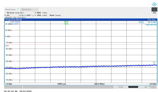
NTVN-n78(3700-3800)-PC1.5-30-25-L-DFT-QPSK-Inner_1RB_Left-10000-30000-PASS
