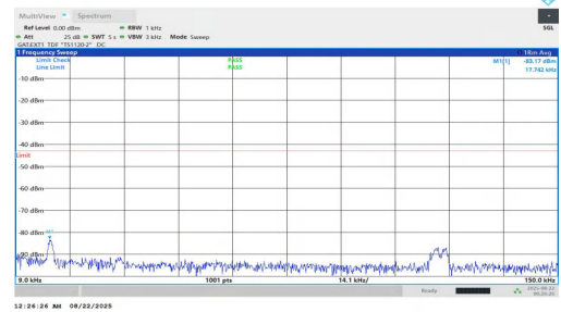
NTVN-n78(3700-3800)-PC1.5-30-25-L-DFT-QPSK-Inner_1RB_Right-0 .009-0.15-PASS
