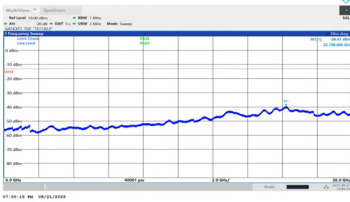
NTNV-n78(3700-3800)-PC1.5-30-25-H-DFT-BPSK-Inner_1RB_Right-6000-26000-PASS
