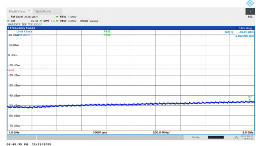
NTNV-n78(3700-3800)-PC1.5-30-25-M-DFT-BPSK-Inner_1RB_Left-1000-3000-PASS
