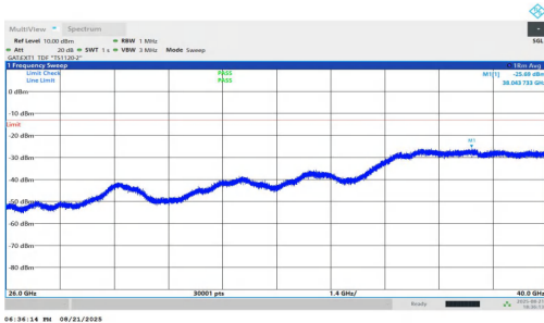
NTNV-n78(3700-3800)-PC1.5-30-25-L-DFT-BPSK-Inner_1RB_Left-26 000-40000-PASS
