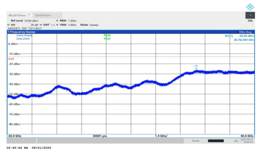
NTNV-n78(3700-3800)-PC1.5-30-25-M-DFT-BPSK-Inner_1RB_Right-2 6000-40000-PASS
