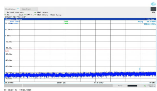
NTVN-n78(3700-3800)-PC1.5-30-25-L-DFT-QPSK-Inner_1RB_Right-3 0-1000-PASS
