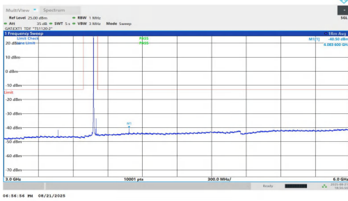
NTNV-n78(3700-3800)-PC1.5-30-25-H-DFT-BPSK-Inner_1RB_Left-3 000-6000-PASS
