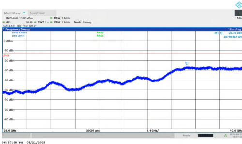
NTNV-n78(3700-3800)-PC1.5-30-25-H-DFT-BPSK-Inner_1RB_Left-2 6000-40000-PASS
