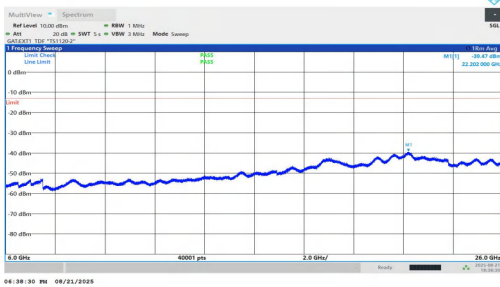
NTVN-n78(3700-3800)-PC1.5-30-25-L-DFT-BPSK-Inner_1RB_Right-6000-26000-PASS
