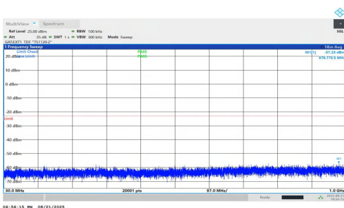
NTNV-n78(3700-3800)-PC1.5-30-25-H-DFT-BPSK-Inner_1RB_Left-300-1000-PASS
