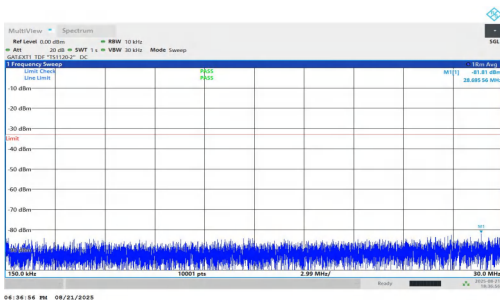
NTNV-n78(3700-3800)-PC1.5-30-25-L-DFT-BPSK-Inner_1RB_Right- 0.15-30-PASS
