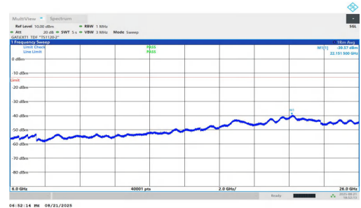
NTNV-n78(3700-3800)-PC1.5-30-25-M-DFT-QPSK-Inner_1RB_Left-60 00-26000-PASS
