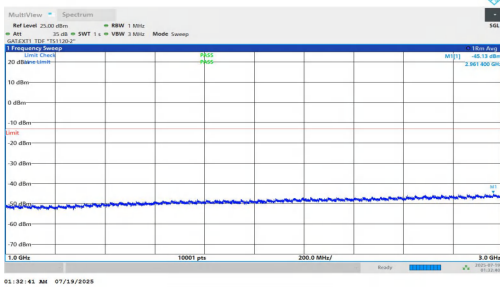
NTNV-n78(3700-3800)-PC1.5-30-20-H-DFT-QPSK-Inner_1RB_Right-1000-3000-PASS
