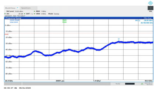
NTNV-n78(3700-3800)-PC1.5-30-25-M-DFT-QPSK-Inner_1RB_Right-26000-40000-PASS
