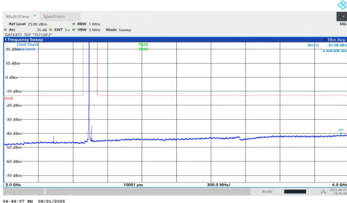
NTNV-n78(3700-3800)-PC1.5-30-25-M-DFT-BPSK-Inner_1RB_Left-3000-6000-PASS
