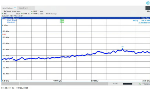
NTNV-n78(3700-3800)-PC1.5-30-25-M-DFT-QPSK-Inner_1RB_Right-6000-26000-PASS
