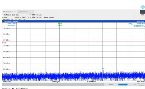
NTNV-n78(3700-3800)-PC1.5-30-20-H-DFT-QPSK-Inner_1RB_Right- 0.15-30-PASS
