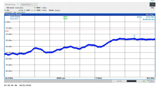
NTVN-n78(3700-3800)-PC1.5-30-25-L-DFT-BPSK-Inner_1RB_Right-26000-40000-PASS
