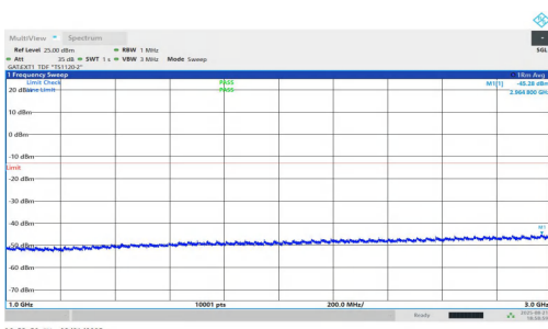
NTNV-n78(3700-3800)-PC1.5-30-25-H-DFT-BPSK-Inner_1RB_Right- 1000-3000-PASS
