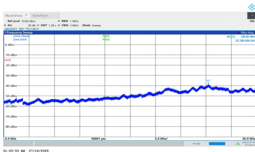
NTNV-n78(3700-3800)-PC1.5-30-20-H-DFT-BPSK-Inner_1RB_Right-6000-26000-PASS
