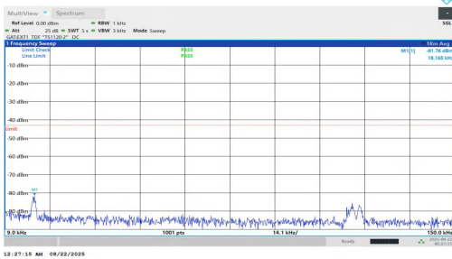
NTNV-n78(3700-3800)-PC1.5-30-25-M-DFT-BPSK-Inner_1RB_Left-0.009-0.15-PASS
