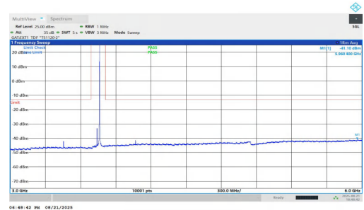
NTNV-n78(3700-3800)-PC1.5-30-25-M-DFT-BPSK-Inner_1RB_Right-3 000-6000-PASS
