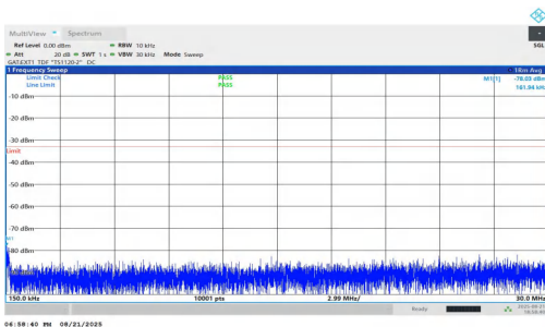
NTNV-n78(3700-3800)-PC1.5-30-25-H-DFT-BPSK-Inner_1RB_Right- 0.15-30-PASS
