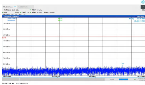
NTNV-n78(3700-3800)-PC1.5-30-20-H-DFT-BPSK-Inner_1RB_Right-0.15-30-PASS
