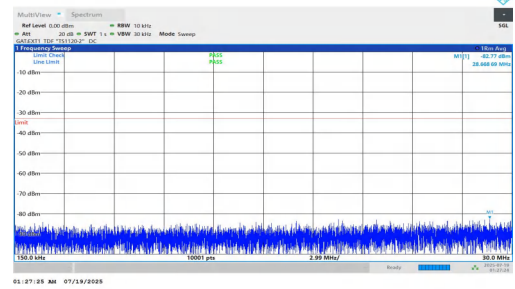
NTNV-n78(3700-3800)-PC1.5-30-20-H-DFT-BPSK-Inner_1RB_Left-0.15-30-PASS
