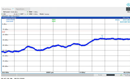
NTNV-n78(3700-3800)-PC1.5-30-25-M-DFT-BPSK-Inner_1RB_Left-26000-40000-PASS
