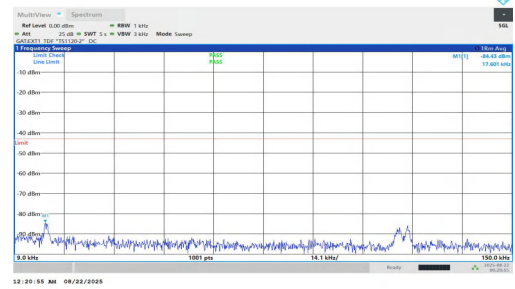
NTNV-n78(3700-3800)-PC1.5-30-20-M-DFT-QPSK-Inner_1RB_Right- 0.009-0.15-PASS
