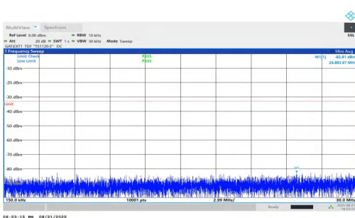
NTNV-n78(3700-3800)-PC1.5-30-25-M-DFT-QPSK-Inner_1RB_Right- 0.15-30-PASS
