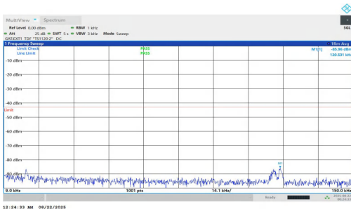
NTNV-n78(3700-3800)-PC1.5-30-25-L-DFT-BPSK-Inner_1RB_Left-0.009-0.15-PASS
