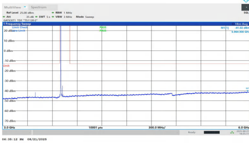
NTNV-n78(3700-3800)-PC1.5-30-25-L-DFT-BPSK-Inner_1RB_Left-30 00-6000-PASS
