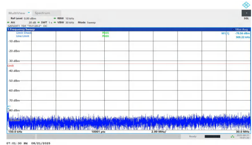
NTNV-n78(3700-3800)-PC1.5-30-25-H-DFT-QPSK-Inner_1RB_Left-0.15-30-PASS
