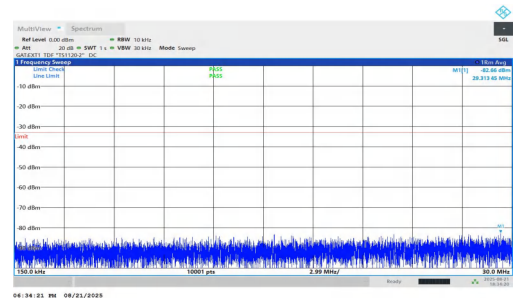
NTNV-n78(3700-3800)-PC1.5-30-25-L-DFT-BPSK-Inner_1RB_Left-0.15-5-30-PASS
