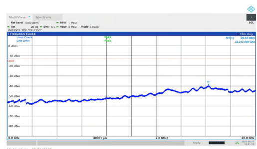
NTVN-n78(3700-3800)-PC1.5-30-25-L-DFT-QPSK-Inner_1RB_Left-60000-260000-PASS
