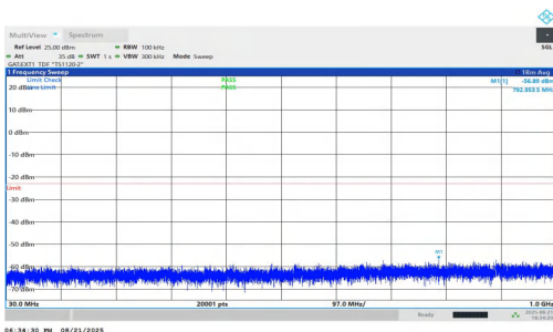
NTNV-n78(3700-3800)-PC1.5-30-25-L-DFT-BPSK-Inner_1RB_Left-30-1000-PASS
