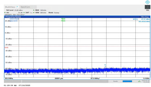
NTNV-n78(3700-3800)-PC1.5-30-20-H-DFT-BPSK-Inner_1RB_Right-3 0-1000-PASS
