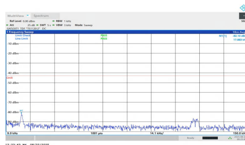
NTNV-n78(3700-3800)-PC1.5-30-20-H-DFT-QPSK-Inner_1RB_Right-0 .009-0.15-PASS
