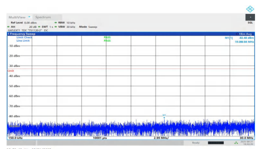
NTNV-n78(3700-3800)-PC1.5-30-25-M-DFT-QPSK-Inner_1RB_Left-0.15-30-PASS
