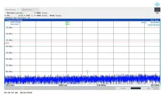
NTNV-n78(3700-3800)-PC1.5-30-25-H-DFT-BPSK-Inner_1RB_Left-0.15-5-30-PASS
