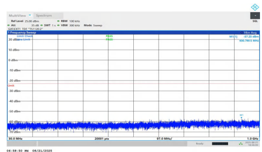
NTNV-n78(3700-3800)-PC1.5-30-25-H-DFT-BPSK-Inner_1RB_Right-3 0-1000-PASS
