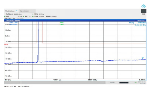
NTNV-n78(3700-3800)-PC1.5-30-25-L-DFT-BPSK-Inner_1RB_Right-3 000-6000-PASS
