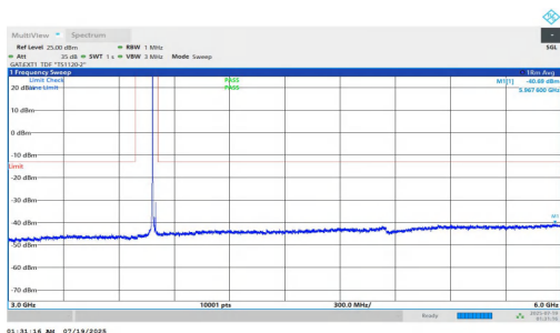
NTNV-n78(3700-3800)-PC1.5-30-20-H-DFT-QPSK-Inner_1RB_Left-3 000-6000-PASS
