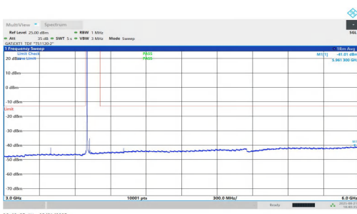
NTVN-n78(3700-3800)-PC1.5-30-25-L-DFT-QPSK-Inner_1RB_Left-30000-60000-PASS
