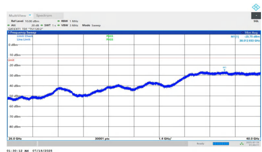
NTNV-n78(3700-3800)-PC1.5-30-20-H-DFT-BPSK-Inner_1RB_Right-2 6000-40000-PASS
