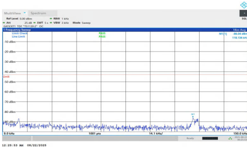
NTVN-n78(3700-3800)-PC1.5-30-25-L-DFT-QPSK-Inner_1RB_Left-0.009-0.15-PASS
