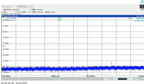
NTNV-n78(3700-3800)-PC1.5-30-25-M-DFT-BPSK-Inner_1RB_Left-30-1000-PASS
