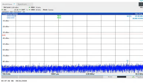
NTNV-n78(3700-3800)-PC1.5-30-25-M-DFT-BPSK-Inner_1RB_Right-0.15-30-PASS
