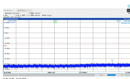
NTNV-n78(3700-3800)-PC1.5-30-20-H-DFT-QPSK-Inner_1RB_Right-3 0-1000-PASS
