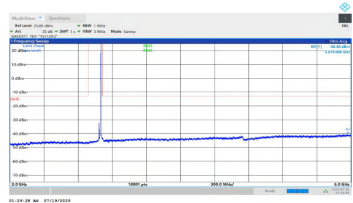
NTNV-n78(3700-3800)-PC1.5-30-20-H-DFT-BPSK-Inner_1RB_Right-3 000-6000-PASS
