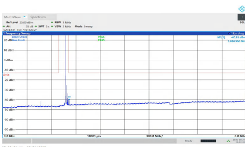
NTNV-n78(3700-3800)-PC1.5-30-25-H-DFT-QPSK-Inner_1RB_Left-30000-60000-PASS
