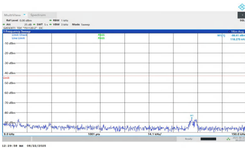
NTNV-n78(3700-3800)-PC1.5-30-25-H-DFT-BPSK-Inner_1RB_Left-0.009-0.15-PASS
