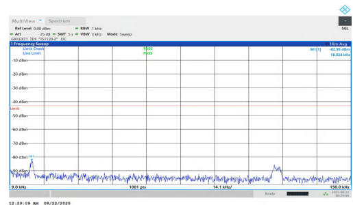
NTNV-n78(3700-3800)-PC1.5-30-25-M-DFT-QPSK-Inner_1RB_Right- 0.009-0.15-PASS
