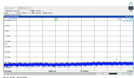
NTNV-n78(3700-3800)-PC1.5-30-25-L-DFT-BPSK-Inner_1RB_Right-3 0-1000-PASS
