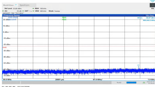
NTNV-n78(3700-3800)-PC1.5-30-20-H-DFT-QPSK-Inner_1RB_Left-3 0-1000-PASS
