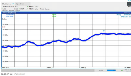
NTNV-n78(3700-3800)-PC1.5-30-20-M-DFT-QPSK-Inner_1RB_Left-2 6000-40000-PASS
