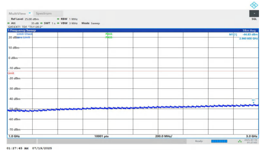
NTNV-n78(3700-3800)-PC1.5-30-20-H-DFT-BPSK-Inner_1RB_Left-1000-3000-PASS
