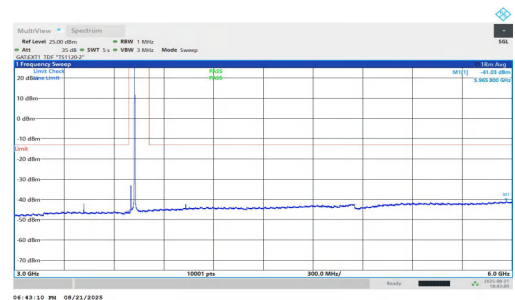
NTVN-n78(3700-3800)-PC1.5-30-25-L-DFT-QPSK-Inner_1RB_Right-3 000-6000-PASS
