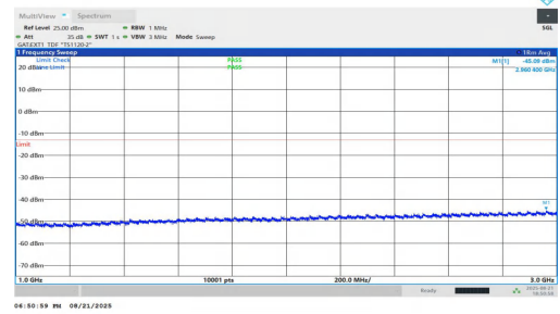
NTNV-n78(3700-3800)-PC1.5-30-25-M-DFT-QPSK-Inner_1RB_Left-10 00-3000-PASS
