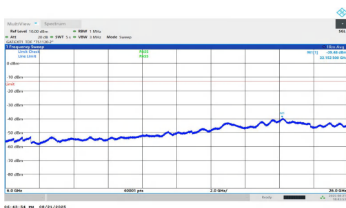
NTVN-n78(3700-3800)-PC1.5-30-25-L-DFT-QPSK-Inner_1RB_Right-6000-26000-PASS
