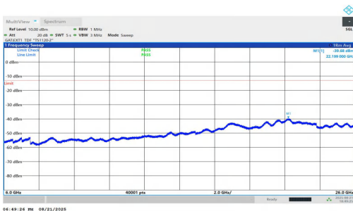
NTNV-n78(3700-3800)-PC1.5-30-25-M-DFT-BPSK-Inner_1RB_Right-6000-26000-PASS
