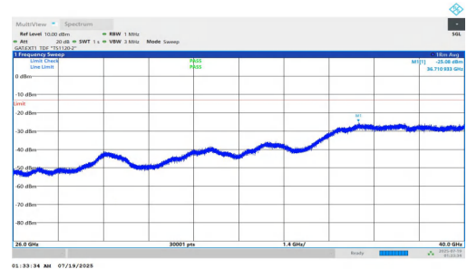
NTNV-n78(3700-3800)-PC1.5-30-20-H-DFT-QPSK-Inner_1RB_Right-26000-40000-PASS
