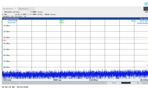
NTVN-n78(3700-3800)-PC1.5-30-25-L-DFT-QPSK-Inner_1RB_Right-0.15-30-PASS
