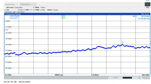
NTNV-n78(3700-3800)-PC1.5-30-25-L-DFT-BPSK-Inner_1RB_Left-60 00-26000-PASS
