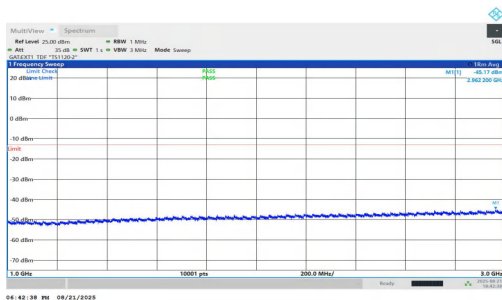
NTVN-n78(3700-3800)-PC1.5-30-25-L-DFT-QPSK-Inner_1RB_Right-1000-3000-PASS
