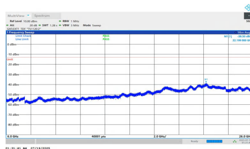
NTNV-n78(3700-3800)-PC1.5-30-20-H-DFT-QPSK-Inner_1RB_Left-60 00-26000-PASS
