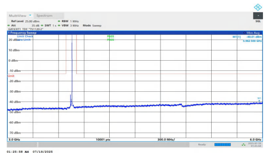
NTNV-n78(3700-3800)-PC1.5-30-20-M-DFT-QPSK-Inner_1RB_Right- 3000-6000-PASS
