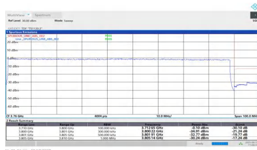
NTNV-n78(3700-3800)-PC1.5-30-90-H-DFT-QPSK-Outer_Full-PAS
