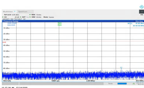
NTNV-n78(3700-3800)-PC1.5-30-10-L-DFT-QPSK-Inner_1RB_Right- 0.15-30-PASS
