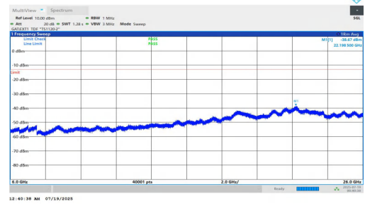
NTNV-n78(3700-3800)-PC1.5-30-10-M-DFT-BPSK-Inner_1RB_Left-60 00-26000-PASS
