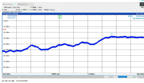
NTNV-n78(3700-3800)-PC1.5-30-10-M-DFT-QPSK-Inner_1RB_Left-2 6000-40000-PASS
