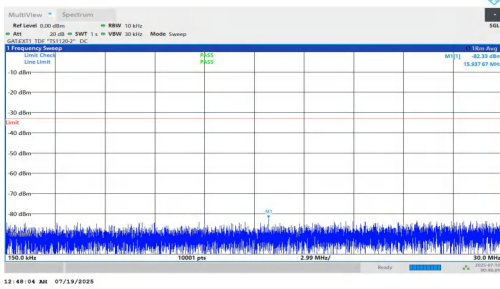
NTNV-n78(3700-3800)-PC1.5-30-10-H-DFT-BPSK-Inner_1RB_Right-0.15-30-PASS
