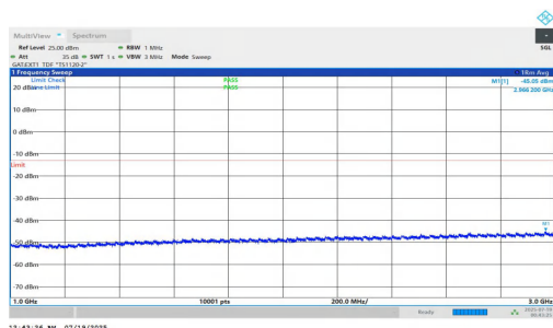
NTNV-n78(3700-3800)-PC1.5-30-10-M-DFT-QPSK-Inner_1RB_Left-1000-3000-PASS
