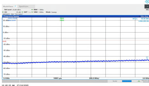
NTNV-n78(3700-3800)-PC1.5-30-10-M-DFT-QPSK-Inner_1RB_Right- 1000-3000-PASS
