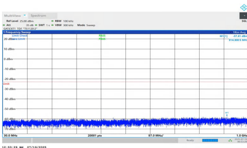
NTNV-n78(3700-3800)-PC1.5-30-15-L-DFT-BPSK-Inner_1RB_Left-30-1000-PASS
