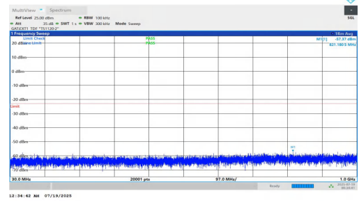
NTNV-n78(3700-3800)-PC1.5-30-10-L-DFT-BPSK-Inner_1RB_Right-3 0-1000-PASS
