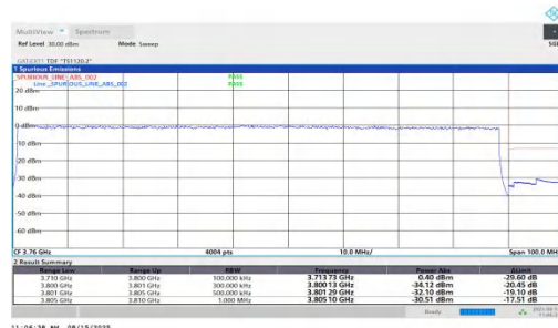
NTNV-n78(3700-3800)-PC1.5-30-90-H-DFT-BPSK-Outer_Full-PAS
