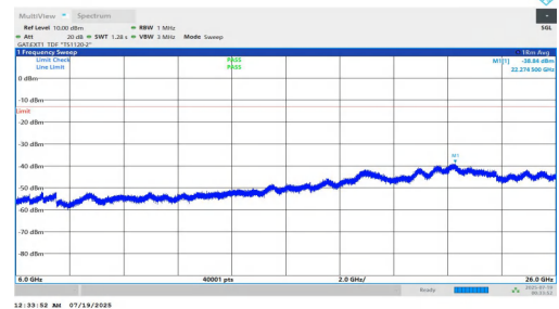
NTNV-n78(3700-3800)-PC1.5-30-10-L-DFT-BPSK-Inner_1RB_Left-6000-26000-PASS
