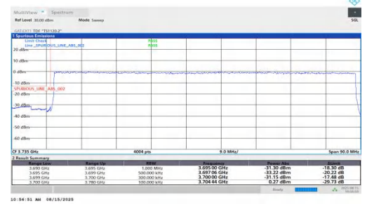
NTNV-n78(3700-3800)-PC1.5-30-80-L-DFT-QPSK-Outer_Full-PASS
