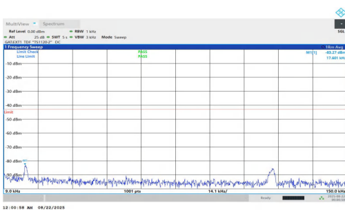
NTNV-n78(3700-3800)-PC1.5-30-10-L-DFT-QPSK-Inner_1RB_Left-0.009-0.15-PASS
