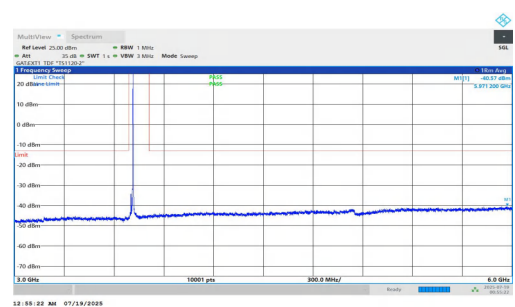
NTNV-n78(3700-3800)-PC1.5-30-15-L-DFT-BPSK-Inner_1RB_Right-3 000-6000-PASS
