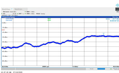
NTNV-n78(3700-3800)-PC1.5-30-10-H-DFT-BPSK-Inner_1RB_Left-26000-40000-PASS
