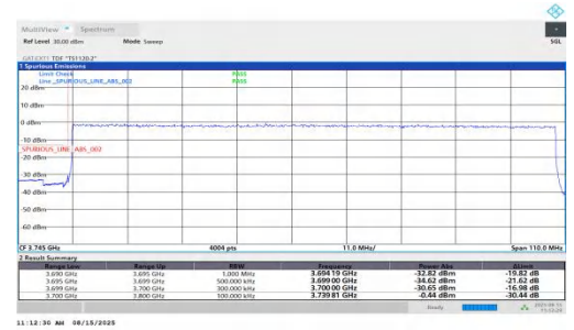
NTNV-n78(3700-3800)-PC1.5-30-100-L-DFT-QPSK-Outer_Full-PA SS
