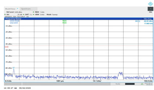
NTNV-n78(3700-3800)-PC1.5-30-15-L-DFT-BPSK-Inner_1RB_Right-0. 009-0.15-PASS
