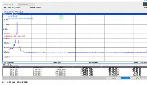
NTNV-n78(3700-3800)-PC1.5-30-100-L-DFT-BPSK-Edge_1RB_Left-PAS S
