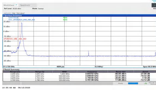
NTNV-n78(3700-3800)-PC1.5-30-80-L-DFT-BPSK-Edge_1RB_Left-PASS
