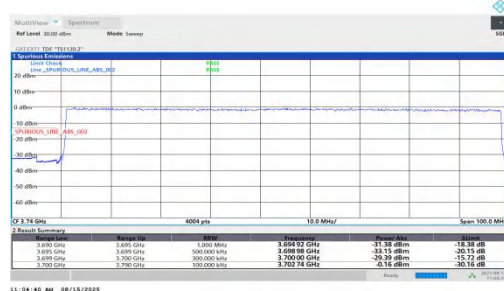
NTNV-n78(3700-3800)-PC1.5-30-90-L-DFT-QPSK-Outer_Full-PAS
