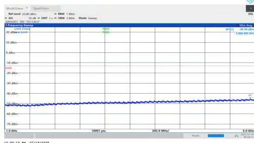
NTNV-n78(3700-3800)-PC1.5-30-10-H-DFT-QPSK-Inner_1RB_Left-10 00-3000-PASS
