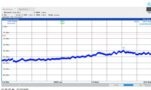
NTNV-n78(3700-3800)-PC1.5-30-10-H-DFT-BPSK-Inner_1RB_Right-6000-26000-PASS
