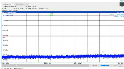
NTNV-n78(3700-3800)-PC1.5-30-10-H-DFT-QPSK-Inner_1RB_Left-3 0-1000-PASS
