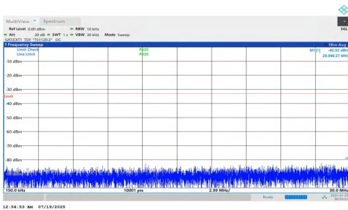
NTNV-n78(3700-3800)-PC1.5-30-15-L-DFT-BPSK-Inner_1RB_Right- 0.15-30-PASS
