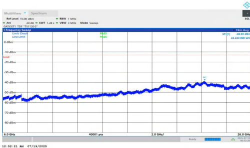
NTNV-n78(3700-3800)-PC1.5-30-10-H-DFT-QPSK-Inner_1RB_Right-6000-26000-PASS
