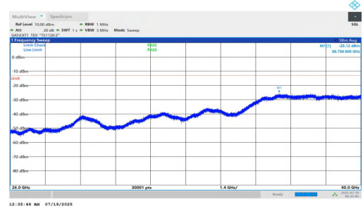
NTNV-n78(3700-3800)-PC1.5-30-10-L-DFT-BPSK-Inner_1RB_Right-2 6000-40000-PASS
