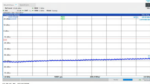
NTNV-n78(3700-3800)-PC1.5-30-10-L-DFT-QPSK-Inner_1RB_Left-10 00-3000-PASS
