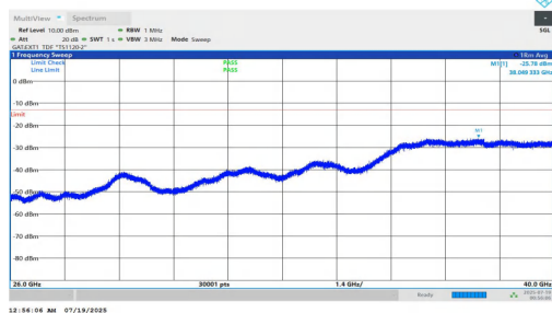
NTVN-n78(3700-3800)-PC1.5-30-15-L-DFT-BPSK-Inner_1RB_Right-26000-40000-PASS
