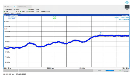
NTNV-n78(3700-3800)-PC1.5-30-10-L-DFT-QPSK-Inner_1RB_Right-26000-40000-PASS
