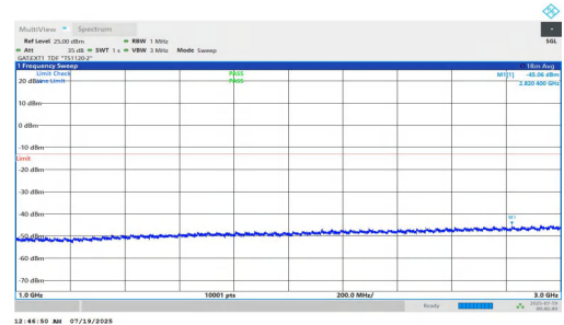
NTNV-n78(3700-3800)-PC1.5-30-10-H-DFT-BPSK-Inner_1RB_Left-1000-3000-PASS
