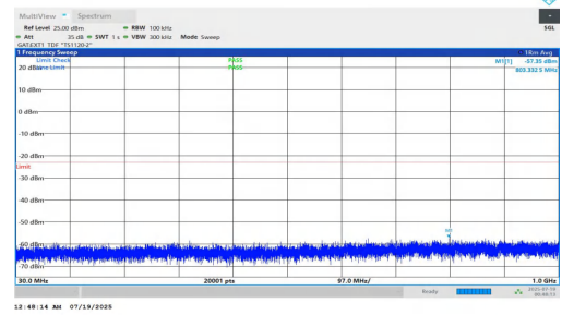
NTNV-n78(3700-3800)-PC1.5-30-10-H-DFT-BPSK-Inner_1RB_Right-3 0-1000-PASS
