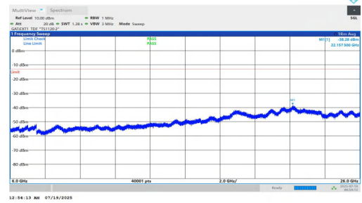
NTNV-n78(3700-3800)-PC1.5-30-15-L-DFT-BPSK-Inner_1RB_Left-60 00-26000-PASS
