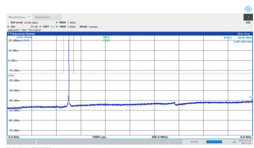
NTNV-n78(3700-3800)-PC1.5-30-10-M-DFT-BPSK-Inner_1RB_Right-3 000-6000-PASS
