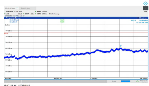
NTNV-n78(3700-3800)-PC1.5-30-10-H-DFT-BPSK-Inner_1RB_Left-6000-26000-PASS
