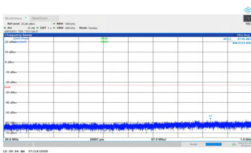
NTNV-n78(3700-3800)-PC1.5-30-10-M-DFT-BPSK-Inner_1RB_Left-30-1000-PASS
