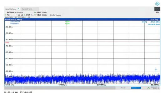
NTNV-n78(3700-3800)-PC1.5-30-15-L-DFT-BPSK-Inner_1RB_Left-0.15-5-30-PASS
