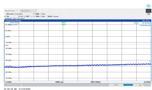
NTNV-n78(3700-3800)-PC1.5-30-10-M-DFT-BPSK-Inner_1RB_Left-1000-3000-PASS
