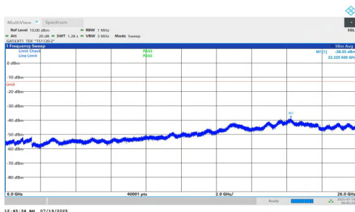
NTNV-n78(3700-3800)-PC1.5-30-10-M-DFT-QPSK-Inner_1RB_Right- 6000-26000-PASS
