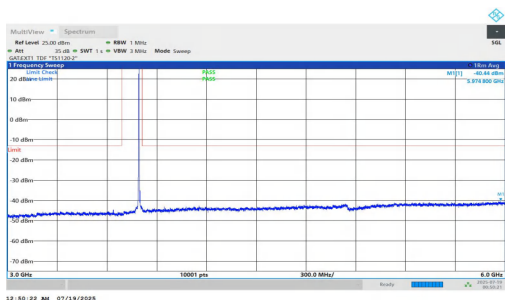
NTNV-n78(3700-3800)-PC1.5-30-10-H-DFT-QPSK-Inner_1RB_Left-3 000-6000-PASS
