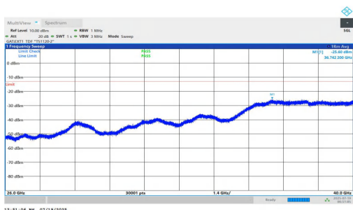
NTNV-n78(3700-3800)-PC1.5-30-10-H-DFT-QPSK-Inner_1RB_Left-2 6000-40000-PASS
