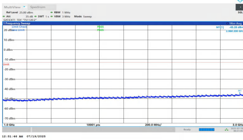
NTNV-n78(3700-3800)-PC1.5-30-10-H-DFT-QPSK-Inner_1RB_Right-1000-3000-PASS
