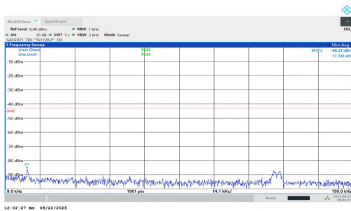
NTNV-n78(3700-3800)-PC1.5-30-10-M-DFT-BPSK-Inner_1RB_Left-0.009-0.15-PASS
