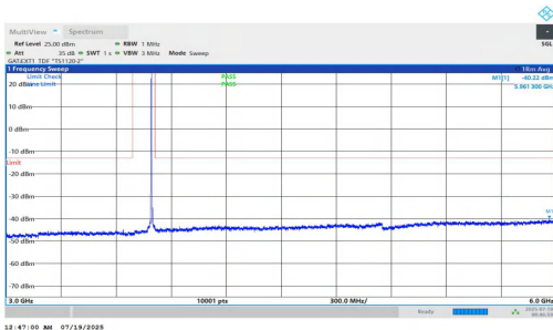
NTNV-n78(3700-3800)-PC1.5-30-10-H-DFT-BPSK-Inner_1RB_Left-3000-6000-PASS
