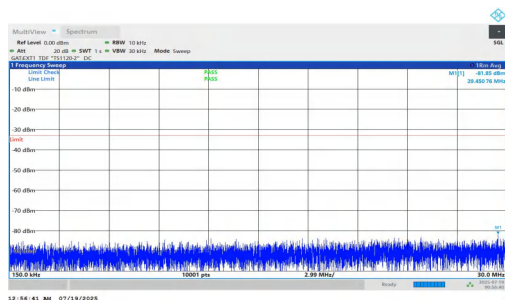
NTVN-n78(3700-3800)-PC1.5-30-15-L-DFT-QPSK-Inner_1RB_Left-0.15-5-30-PASS
