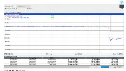
NTNV-n78(3700-3800)-PC1.5-30-80-H-DFT-BPSK-Outer_Full-PASS
