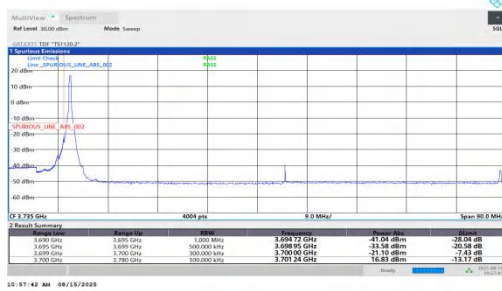
NTNV-n78(3700-3800)-PC1.5-30-80-L-DFT-QPSK-Edge_1RB_Left-PASS
