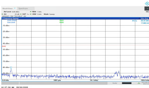
NTNV-n78(3700-3800)-PC1.5-30-15-L-DFT-BPSK-Inner_1RB_Left-0.009-0.15-PASS
