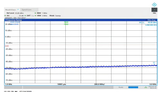
NTNV-n78(3700-3800)-PC1.5-30-15-L-DFT-BPSK-Inner_1RB_Left-1000-3000-PASS
