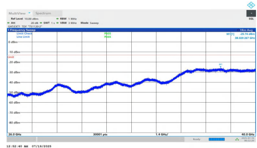
NTNV-n78(3700-3800)-PC1.5-30-10-H-DFT-QPSK-Inner_1RB_Right-26000-40000-PASS
