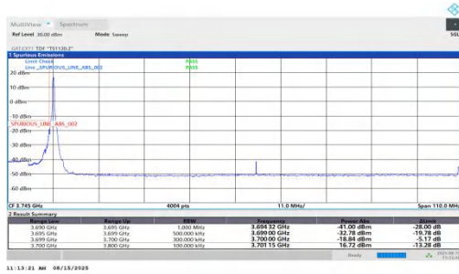
NTNV-n78(3700-3800)-PC1.5-30-100-L-DFT-QPSK-Edge_1RB_Left-PAS S
