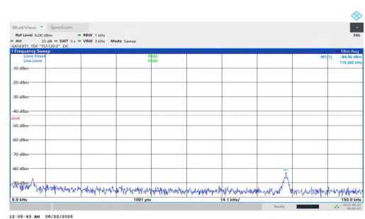
NTNV-n78(3700-3800)-PC1.5-30-10-H-DFT-BPSK-Inner_1RB_Right-0.009-0.15-PASS
