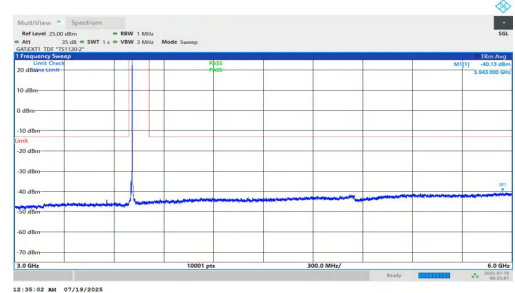
NTNV-n78(3700-3800)-PC1.5-30-10-L-DFT-BPSK-Inner_1RB_Right-3 000-6000-PASS
