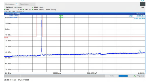
NTNV-n78(3700-3800)-PC1.5-30-10-H-DFT-QPSK-Inner_1RB_Right-3000-6000-PASS
