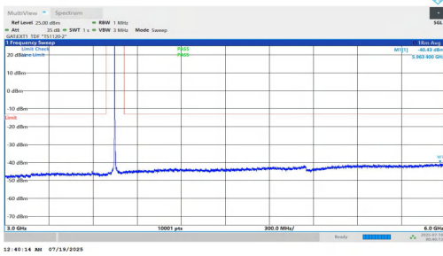
NTNV-n78(3700-3800)-PC1.5-30-10-M-DFT-BPSK-Inner_1RB_Left-3 000-6000-PASS
