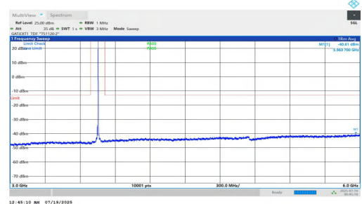
NTNV-n78(3700-3800)-PC1.5-30-10-M-DFT-QPSK-Inner_1RB_Right- 3000-6000-PASS
