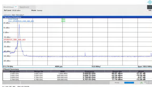
NTNV-n78(3700-3800)-PC1.5-30-90-L-DFT-BPSK-Edge_1RB_Left-PASS
