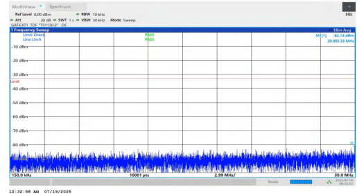
NTNV-n78(3700-3800)-PC1.5-30-10-L-DFT-BPSK-Inner_1RB_Left-0.15-30-PASS
