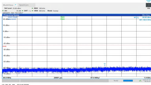
NTNV-n78(3700-3800)-PC1.5-30-10-L-DFT-QPSK-Inner_1RB_Left-3 0-1000-PASS
