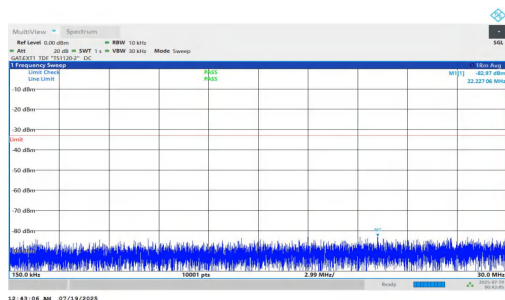
NTNV-n78(3700-3800)-PC1.5-30-10-M-DFT-QPSK-Inner_1RB_Left-0.15-30-PASS
