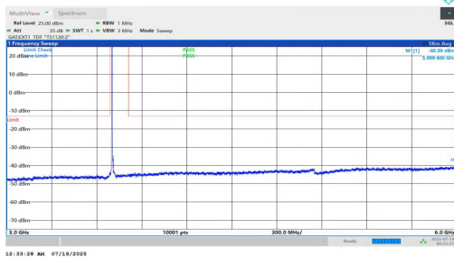
NTNV-n78(3700-3800)-PC1.5-30-10-L-DFT-BPSK-Inner_1RB_Left-3000-6000-PASS
