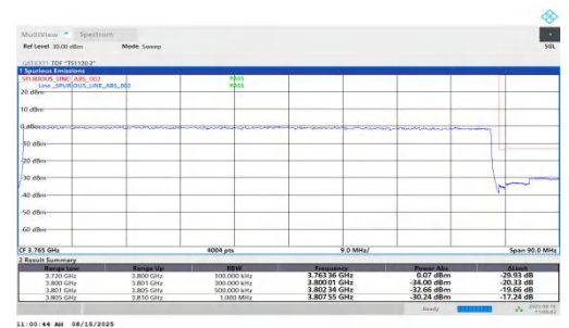
NTNV-n78(3700-3800)-PC1.5-30-80-H-DFT-QPSK-Outer_Full-PASS
