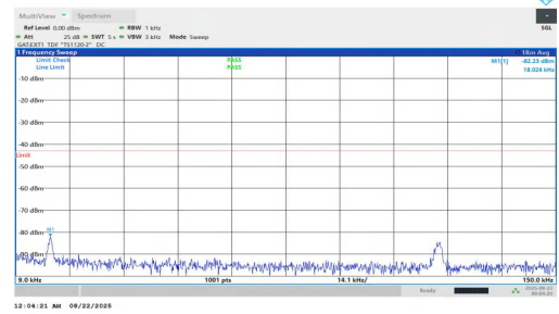
NTNV-n78(3700-3800)-PC1.5-30-10-M-DFT-QPSK-Inner_1RB_Right- 0.009-0.15-PASS
