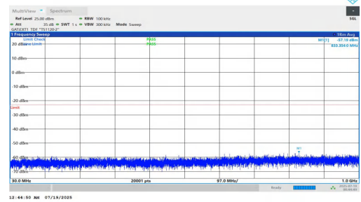
NTNV-n78(3700-3800)-PC1.5-30-10-M-DFT-QPSK-Inner_1RB_Right- 30-1000-PASS
