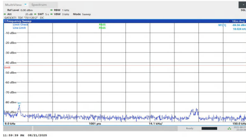
NTNV-n78(3700-3800)-PC1.5-30-10-L-DFT-BPSK-Inner_1RB_Left-0.009-0.15-PASS
