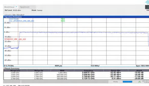
NTNV-n78(3700-3800)-PC1.5-30-90-L-DFT-BPSK-Outer_Full-PAS S
