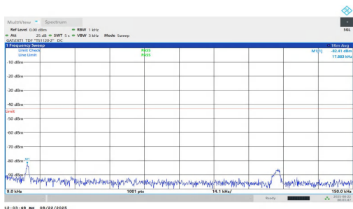
NTNV-n78(3700-3800)-PC1.5-30-10-M-DFT-QPSK-Inner_1RB_Left-0.009-0.15-PASS
