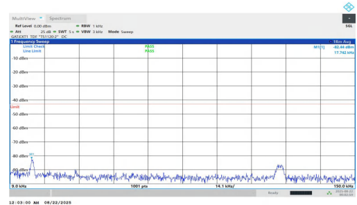
NTNV-n78(3700-3800)-PC1.5-30-10-M-DFT-BPSK-Inner_1RB_Right-0 .009-0.15-PASS
