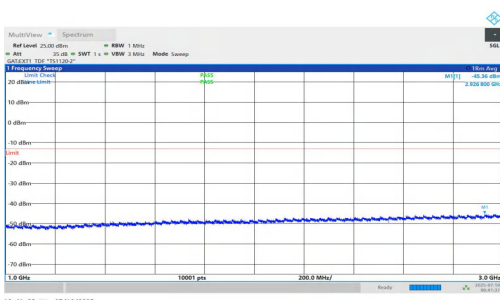
NTNV-n78(3700-3800)-PC1.5-30-10-M-DFT-BPSK-Inner_1RB_Right- 1000-3000-PASS
