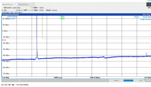
NTNV-n78(3700-3800)-PC1.5-30-15-L-DFT-BPSK-Inner_1RB_Left-30 00-6000-PASS
