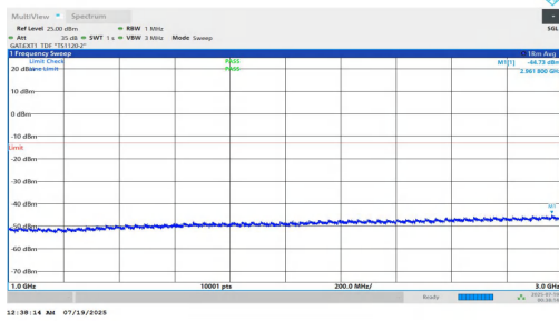
NTNV-n78(3700-3800)-PC1.5-30-10-L-DFT-QPSK-Inner_1RB_Right-1000-3000-PASS
