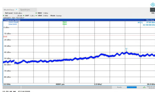
NTNV-n78(3700-3800)-PC1.5-30-10-H-DFT-QPSK-Inner_1RB_Left-60 00-26000-PASS
