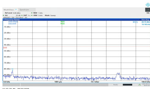
NTNV-n78(3700-3800)-PC1.5-30-10-H-DFT-QPSK-Inner_1RB_Right-0 .009-0.15-PASS
