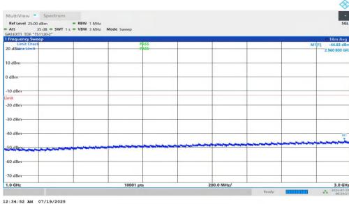
NTNV-n78(3700-3800)-PC1.5-30-10-L-DFT-BPSK-Inner_1RB_Right-1000-3000-PASS
