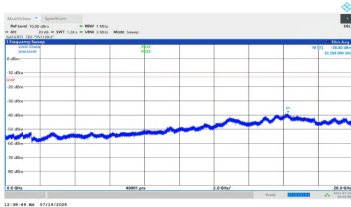
NTNV-n78(3700-3800)-PC1.5-30-10-L-DFT-QPSK-Inner_1RB_Right-6000-26000-PASS
