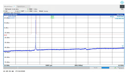
NTNV-n78(3700-3800)-PC1.5-30-10-H-DFT-BPSK-Inner_1RB_Right-3 000-6000-PASS
