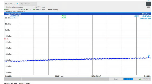
NTNV-n78(3700-3800)-PC1.5-30-10-L-DFT-BPSK-Inner_1RB_Left-1000-3000-PASS
