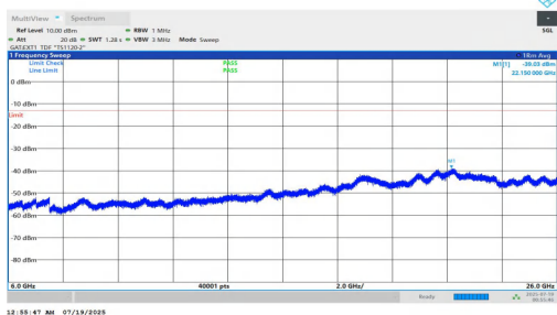
NTVN-n78(3700-3800)-PC1.5-30-15-L-DFT-BPSK-Inner_1RB_Right-6000-26000-PASS
