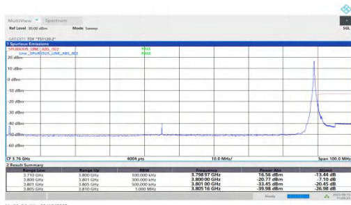
NTNV-n78(3700-3800)-PC1.5-30-90-H-DFT-QPSK-Edge_1RB_Right-PA SS
