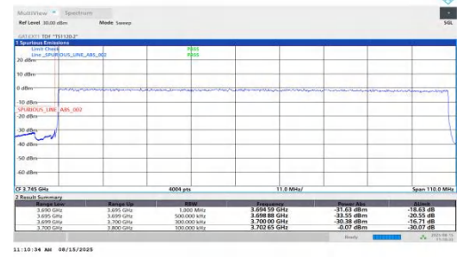
NTNV-n78(3700-3800)-PC1.5-30-100-L-DFT-BPSK-Outer_Full-PA SS
