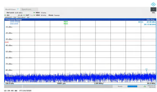
NTNV-n78(3700-3800)-PC1.5-30-10-M-DFT-BPSK-Inner_1RB_Left-0.15-30-PASS
