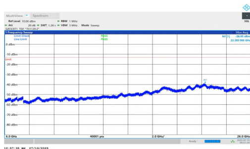
NTVN-n78(3700-3800)-PC1.5-30-15-L-DFT-QPSK-Inner_1RB_Left-60000-260000-PASS
