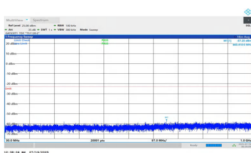
NTNV-n78(3700-3800)-PC1.5-30-10-L-DFT-QPSK-Inner_1RB_Right-3 0-1000-PASS
