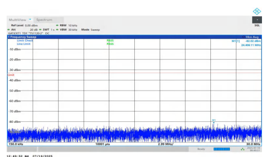
NTNV-n78(3700-3800)-PC1.5-30-10-H-DFT-QPSK-Inner_1RB_Left-0.15-30-PASS
