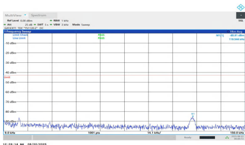
NTVN-n78(3700-3800)-PC1.5-30-15-L-DFT-QPSK-Inner_1RB_Left-0.009-0.15-PASS
