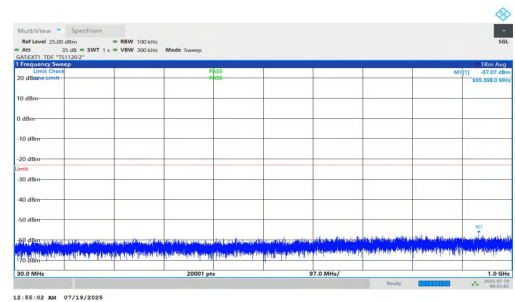
NTNV-n78(3700-3800)-PC1.5-30-15-L-DFT-BPSK-Inner_1RB_Right-3 0-1000-PASS
