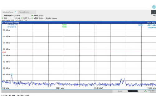
NTNV-n78(3700-3800)-PC1.5-30-10-H-DFT-QPSK-Inner_1RB_Left-0.009-0.15-PASS
