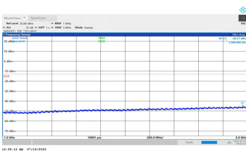
NTNV-n78(3700-3800)-PC1.5-30-15-L-DFT-BPSK-Inner_1RB_Right- 1000-3000-PASS
