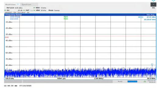
NTNV-n78(3700-3800)-PC1.5-30-10-H-DFT-BPSK-Inner_1RB_Left-0.15-30-PASS
