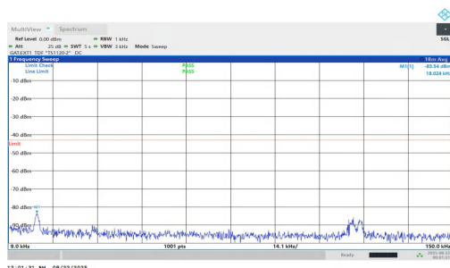
NTNV-n78(3700-3800)-PC1.5-30-10-L-DFT-QPSK-Inner_1RB_Right-0 .009-0.15-PASS
