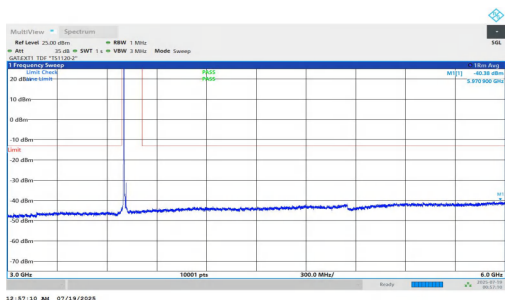
NTVN-n78(3700-3800)-PC1.5-30-15-L-DFT-QPSK-Inner_1RB_Left-30000-60000-PASS
