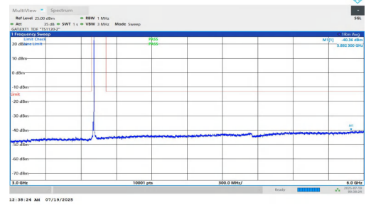
NTNV-n78(3700-3800)-PC1.5-30-10-L-DFT-QPSK-Inner_1RB_Right-3000-6000-PASS
