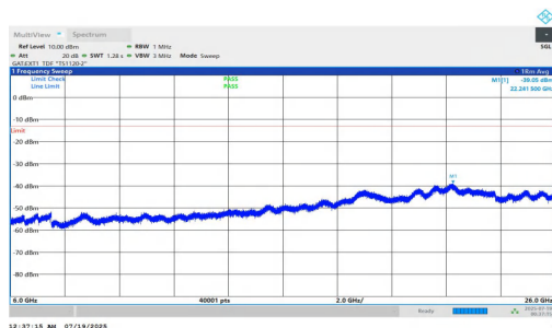
NTNV-n78(3700-3800)-PC1.5-30-10-L-DFT-QPSK-Inner_1RB_Left-60 00-26000-PASS
