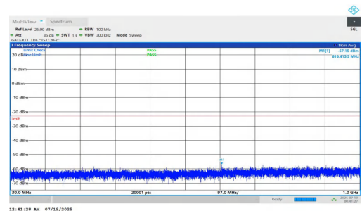
NTNV-n78(3700-3800)-PC1.5-30-10-M-DFT-BPSK-Inner_1RB_Right-3 0-1000-PASS
