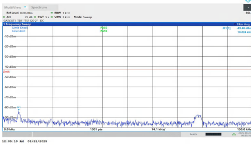
NTNV-n78(3700-3800)-PC1.5-30-10-H-DFT-BPSK-Inner_1RB_Left-0.009-0.15-PASS
