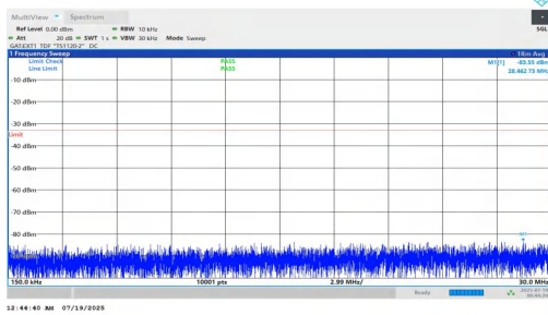
NTNV-n78(3700-3800)-PC1.5-30-10-M-DFT-QPSK-Inner_1RB_Right- 0.15-30-PASS
