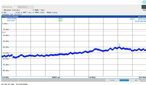
NTNV-n78(3700-3800)-PC1.5-30-10-L-DFT-BPSK-Inner_1RB_Right-6000-26000-PASS
