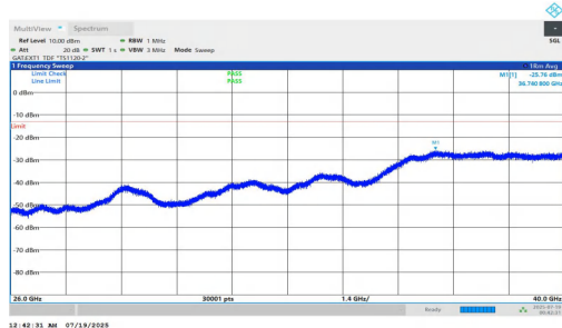
NTNV-n78(3700-3800)-PC1.5-30-10-M-DFT-BPSK-Inner_1RB_Right-26000-40000-PASS
