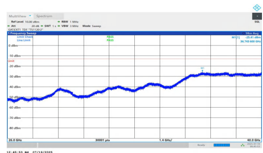
NTNV-n78(3700-3800)-PC1.5-30-10-M-DFT-QPSK-Inner_1RB_Right- 26000-40000-PASS
