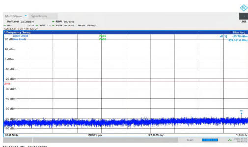
NTNV-n78(3700-3800)-PC1.5-30-10-M-DFT-QPSK-Inner_1RB_Left-30-1000-PASS
