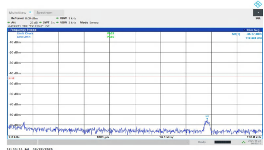
NTNV-n78(3700-3800)-PC1.5-30-10-L-DFT-BPSK-Inner_1RB_Right-0.009-0.15-PASS
