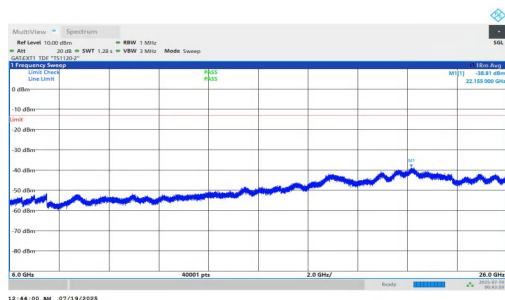
NTNV-n78(3700-3800)-PC1.5-30-10-M-DFT-QPSK-Inner_1RB_Left-6000-26000-PASS
