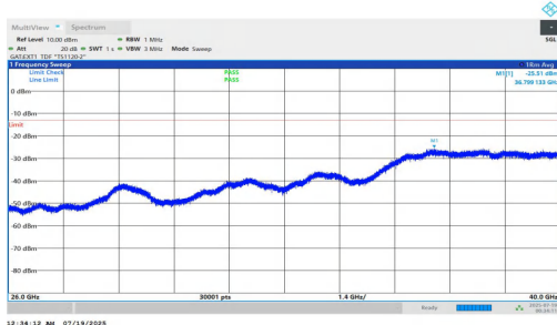
NTNV-n78(3700-3800)-PC1.5-30-10-L-DFT-BPSK-Inner_1RB_Left-26000-40000-PASS
