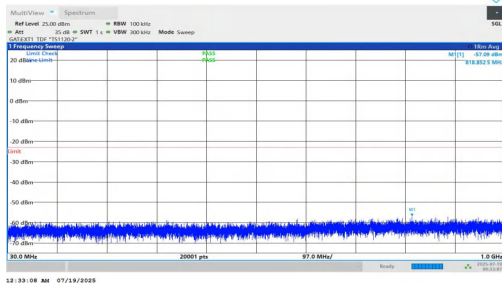
NTNV-n78(3700-3800)-PC1.5-30-10-L-DFT-BPSK-Inner_1RB_Left-30-1000-PASS
