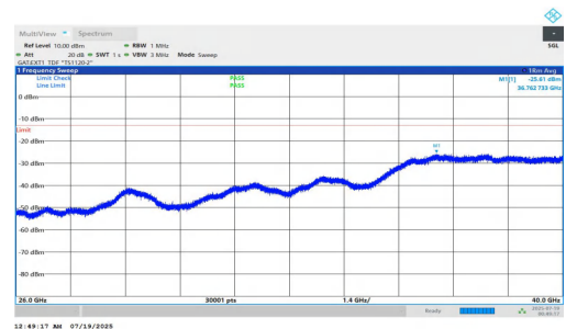
NTNV-n78(3700-3800)-PC1.5-30-10-H-DFT-BPSK-Inner_1RB_Right-2 6000-40000-PASS
