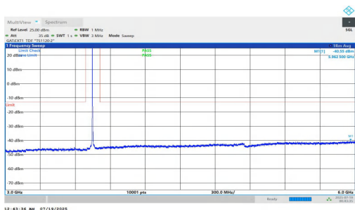
NTNV-n78(3700-3800)-PC1.5-30-10-M-DFT-QPSK-Inner_1RB_Left-3000-6000-PASS
