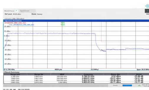
NTNV-n78(3700-3800)-PC1.5-30-20-H-DFT-QPSK-Outer_Full-PAS S
