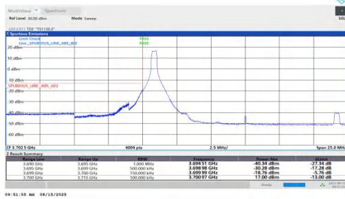
NTNV-n78(3700-3800)-PC1.5-30-15-L-DFT-QPSK-Edge_1RB_Left-PASS S
