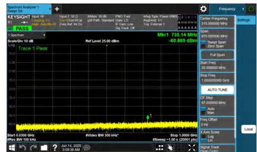
NTNV-n78(3700-3800)-PC2-30-100-L-DFT-QPSK-Inner_1RB_Right-3000-1000-PASS
