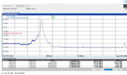
NTNV-n78(3700-3800)-PC1.5-30-25-L-DFT-BPSK-Edge_1RB_Left-PASS
