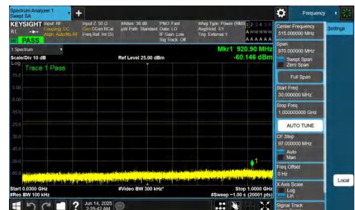
NTNV-n78(3700-3800)-PC2-30-90-M-DFT-BPSK-Inner_1RB_Right-30- 1000-PASS
