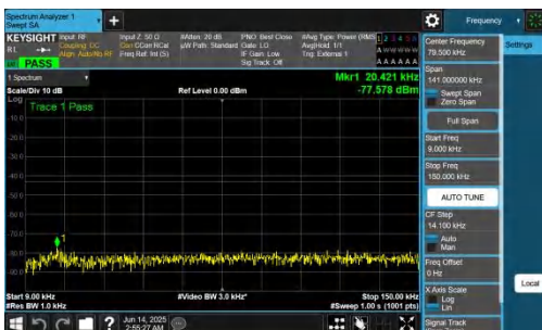
NTNV-n78(3700-3800)-PC2-30-100-L-DFT-BPSK-Inner_1RB_Left-0.0 09-0.15-PASS
