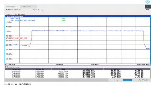
NTNV-n78(3700-3800)-PC1.5-30-50-L-DFT-QPSK-Outer_Full-PASS S
