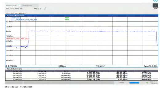
NTNV-n78(3700-3800)-PC1.5-30-60-L-DFT-QPSK-Outer_Full-PASS
