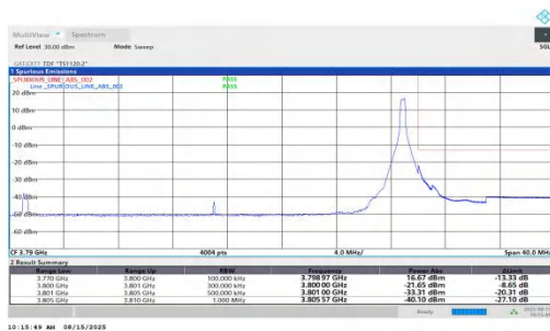
NTNV-n78(3700-3800)-PC1.5-30-30-H-DFT-QPSK-Edge_1RB_Right-PA
