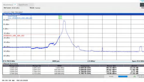
NTNV-n78(3700-3800)-PC1.5-30-15-L-DFT-BPSK-Edge_1RB_Left-PASS
