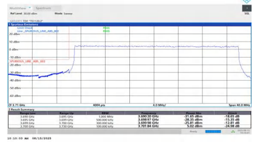
NTNV-n78(3700-3800)-PC1.5-30-30-L-DFT-BPSK-Outer_Full-PASS
