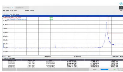
NTNV-n78(3700-3800)-PC1.5-30-70-H-DFT-QPSK-Edge_1RB_Right-PA SS
