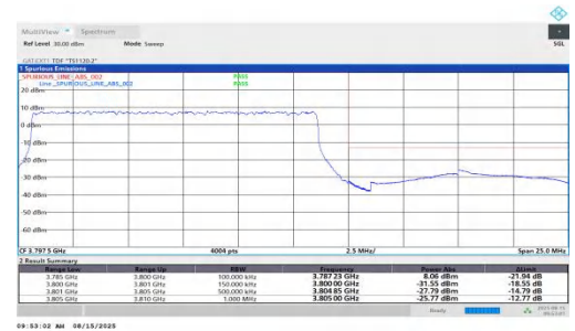
NTNV-n78(3700-3800)-PC1.5-30-15-H-DFT-BPSK-Outer_Full-PASS S
