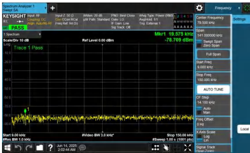
NTNV-n78(3700-3800)-PC2-30-90-L-DFT-BPSK-Inner_1RB_Left-0.00 9-0.15-PASS
