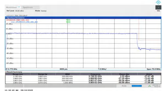
NTNV-n78(3700-3800)-PC1.5-30-60-H-DFT-BPSK-Outer_Full-PASS
