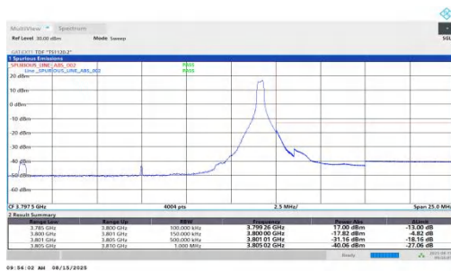
NTNV-n78(3700-3800)-PC1.5-30-15-H-DFT-QPSK-Edge_1RB_Right-PA SS
