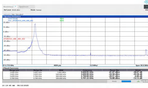
NTNV-n78(3700-3800)-PC1.5-30-40-L-DFT-QPSK-Edge_1RB_Left-PAS S
