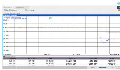
NTNV-n78(3700-3800)-PC1.5-30-70-H-DFT-QPSK-Outer_Full-PAS S
