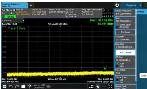
NTNV-n78(3700-3800)-PC2-30-90-L-DFT-BPSK-Inner_1RB_Left-30-1000-PASS
