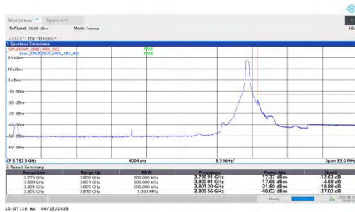
NTNV-n78(3700-3800)-PC1.5-30-25-H-DFT-BPSK-Edge_1RB_Right-PASS
