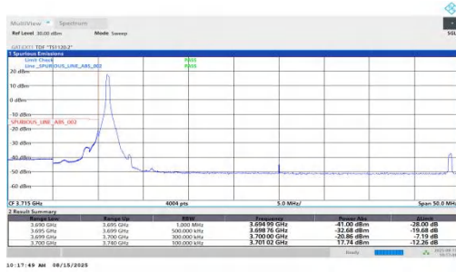
NTNV-n78(3700-3800)-PC1.5-30-40-L-DFT-BPSK-Edge_1RB_Left-PASS
