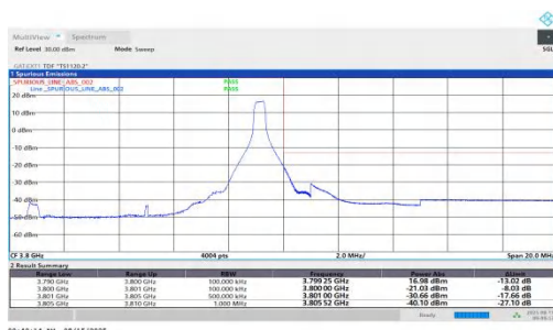
NTVN-n78(3700-3800)-PC1.5-30-10-H-DFT-QPSK-Edge_1RB_Right-PA SS
