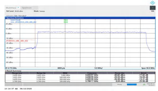
NTNV-n78(3700-3800)-PC1.5-30-40-L-DFT-BPSK-Outer_Full-PAS S
