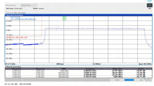
NTNV-n78(3700-3800)-PC1.5-30-30-L-DFT-QPSK-Outer_Full-PASS
