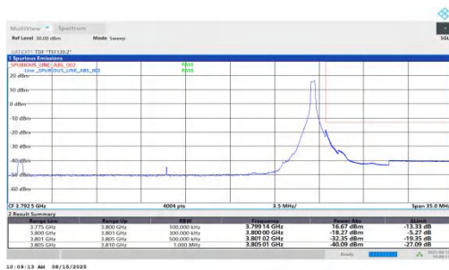
NTNV-n78(3700-3800)-PC1.5-30-25-H-DFT-QPSK-Edge_1RB_Right-PASS
