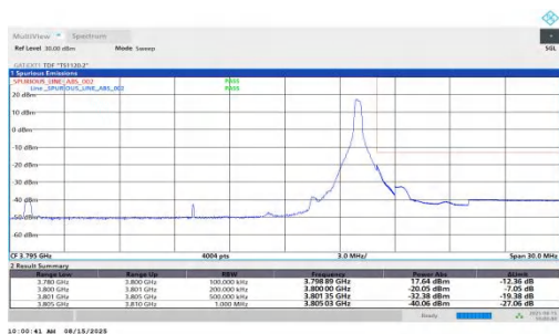
NTNV-n78(3700-3800)-PC1.5-30-20-H-DFT-BPSK-Edge_1RB_Right-PA SS
