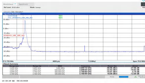
NTNV-n78(3700-3800)-PC1.5-30-60-L-DFT-BPSK-Edge_1RB_Left-PASS
