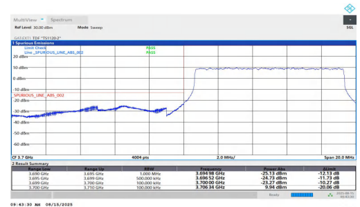
NTVN-n78(3700-3800)-PC1.5-30-10-L-DFT-BPSK-Outer_Full-PASS S
