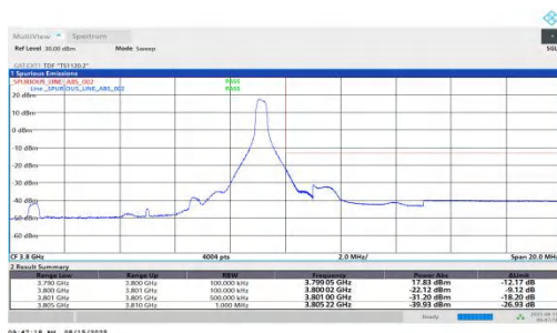
NTVN-n78(3700-3800)-PC1.5-30-10-H-DFT-BPSK-Edge_1RB_Right-PA SS
