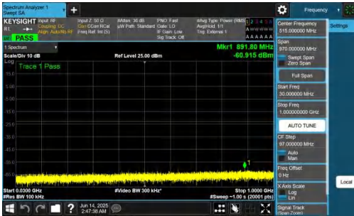
NTVN-n78(3700-3800)-PC2-30-90-H-DFT-QPSK-Inner_1RB_Left-30-1000-PASS
