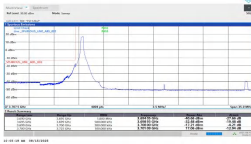
NTNV-n78(3700-3800)-PC1.5-30-25-L-DFT-QPSK-Edge_1RB_Left-PASS
