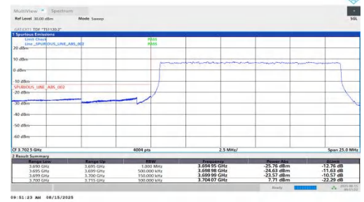
NTNV-n78(3700-3800)-PC1.5-30-15-L-DFT-QPSK-Outer_Full-PASS S
