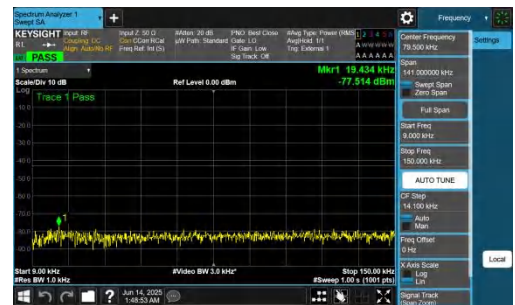
NTNV-n78(3700-3800)-PC2-30-80-H-DFT-BPSK-Inner_1RB_Right-0.0 09-0.15-PASS
