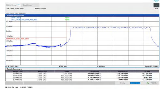
NTNV-n78(3700-3800)-PC1.5-30-15-L-DFT-BPSK-Outer_Full-PASS S
