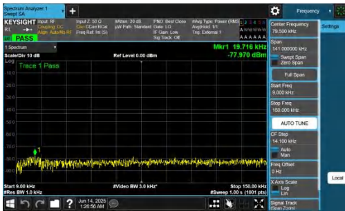
NTNV-n78(3700-3800)-PC2-30-80-M-DFT-BPSK-Inner_1RB_Left-0.0 09-0.15-PASS
