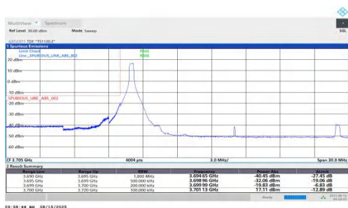
NTNV-n78(3700-3800)-PC1.5-30-20-L-DFT-QPSK-Edge_1RB_Left-PAS
