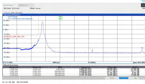
NTNV-n78(3700-3800)-PC1.5-30-30-L-DFT-QPSK-Edge_1RB_Left-PASS
