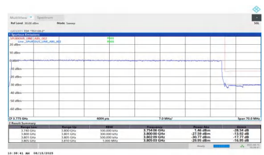
NTNV-n78(3700-3800)-PC1.5-30-60-H-DFT-QPSK-Outer_Full-PASS
