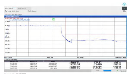
NTVN-n78(3700-3800)-PC1.5-30-10-H-DFT-QPSK-Outer_Full-PASS S
