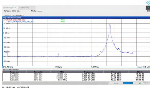
NTNV-n78(3700-3800)-PC1.5-30-30-H-DFT-BPSK-Edge_1RB_Right-PA
