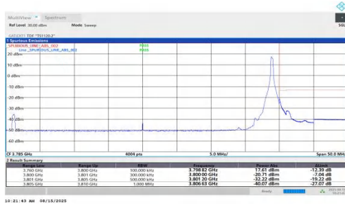
NTNV-n78(3700-3800)-PC1.5-30-40-H-DFT-BPSK-Edge_1RB_Right-PA SS
