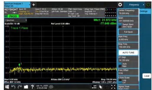
NTNV-n78(3700-3800)-PC2-30-90-M-DFT-QPSK-Inner_1RB_Right-0.0 09-0.15-PASS
