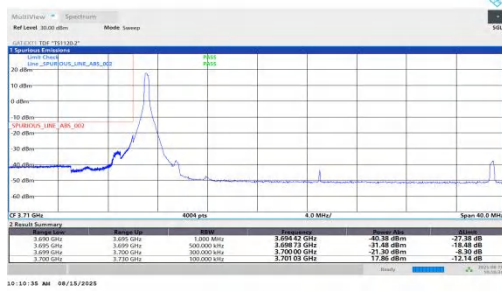
NTNV-n78(3700-3800)-PC1.5-30-30-L-DFT-BPSK-Edge_1RB_Left-PASS
