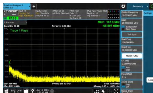
NTNV-n78(3700-3800)-PC2-30-90-M-DFT-BPSK-Inner_1RB_Left-0.15 -30-PASS
