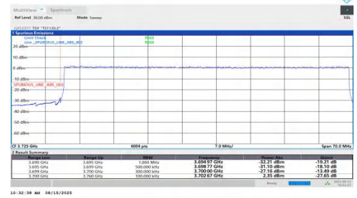
NTNV-n78(3700-3800)-PC1.5-30-60-L-DFT-BPSK-Outer_Full-PASS
