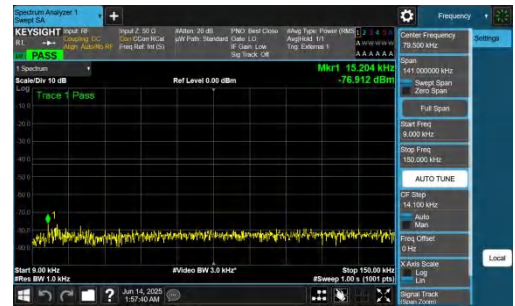
NTNV-n78(3700-3800)-PC2-30-80-H-DFT-QPSK-Inner_1RB_Right-009-0.15-PASS
