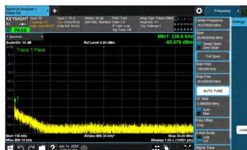
NTNV-n78(3700-3800)-PC2-30-90-M-DFT-QPSK-Inner_1RB_Left-0.15 -30-PASS
