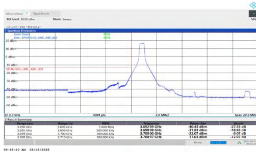
NTVN-n78(3700-3800)-PC1.5-30-10-L-DFT-QPSK-Edge_1RB_Left-PASS S
