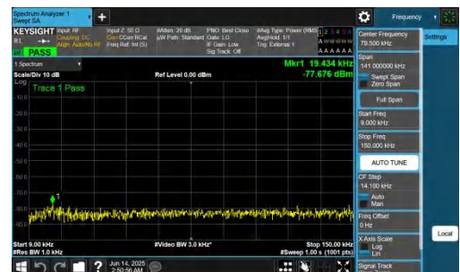
NTVN-n78(3700-3800)-PC2-30-90-H-DFT-QPSK-Inner_1RB_Right-0.009-0.15-PASS
