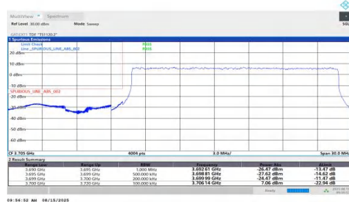
NTNV-n78(3700-3800)-PC1.5-30-20-L-DFT-BPSK-Outer_Full-PAS S
