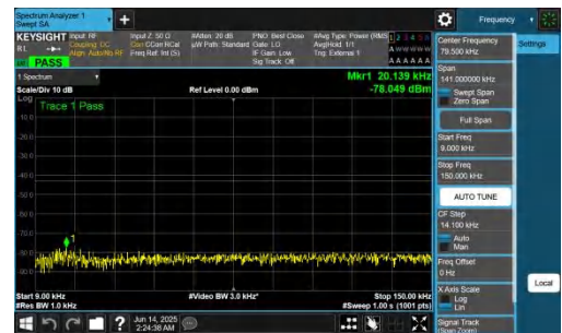
NTNV-n78(3700-3800)-PC2-30-90-M-DFT-BPSK-Inner_1RB_Right-0.0 09-0.15-PASS
