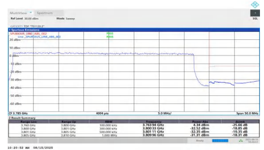
NTNV-n78(3700-3800)-PC1.5-30-40-H-DFT-BPSK-Outer_Full-PAS S
