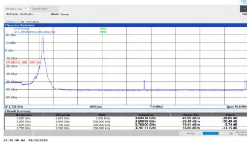
NTNV-n78(3700-3800)-PC1.5-30-60-L-DFT-QPSK-Edge_1RB_Left-PASS
