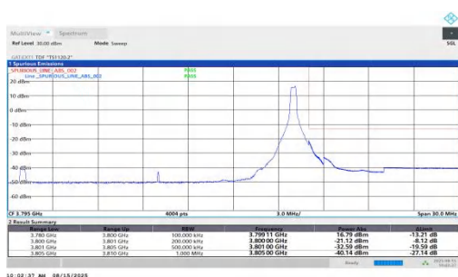
NTNV-n78(3700-3800)-PC1.5-30-20-H-DFT-QPSK-Edge_1RB_Right-PA SS
