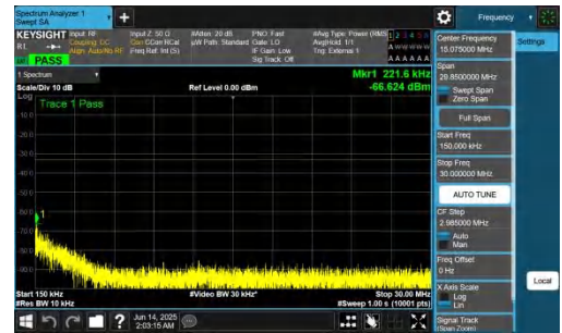
NTNV-n78(3700-3800)-PC2-30-90-L-DFT-BPSK-Inner_1RB_Left-0.15-30-PASS
