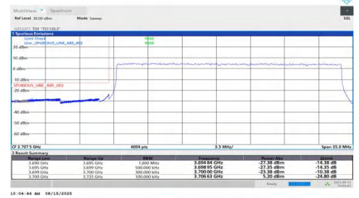
NTNV-n78(3700-3800)-PC1.5-30-25-L-DFT-QPSK-Outer_Full-PASS
