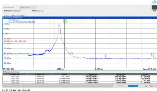
NTNV-n78(3700-3800)-PC1.5-30-20-L-DFT-BPSK-Edge_1RB_Left-PASS
