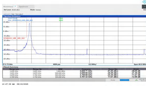
NTNV-n78(3700-3800)-PC1.5-30-50-L-DFT-QPSK-Edge_1RB_Left-PASS S
