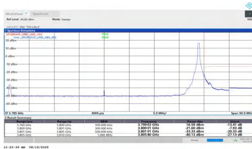
NTNV-n78(3700-3800)-PC1.5-30-40-H-DFT-QPSK-Edge_1RB_Right-PA SS
