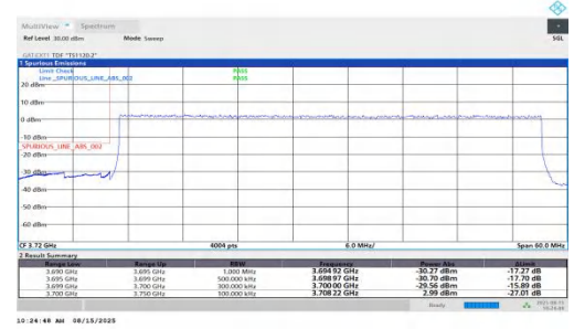
NTNV-n78(3700-3800)-PC1.5-30-50-L-DFT-BPSK-Outer_Full-PASS S
