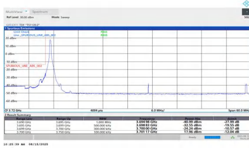
NTNV-n78(3700-3800)-PC1.5-30-50-L-DFT-BPSK-Edge_1RB_Left-PASS
