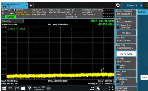
NTNV-n78(3700-3800)-PC2-30-90-H-DFT-BPSK-Inner_1RB_Left-30- 1000-PASS
