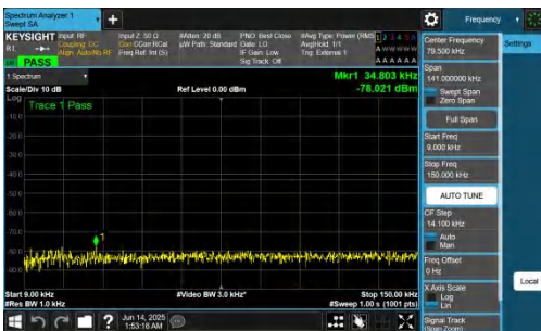
NTNV-n78(3700-3800)-PC2-30-80-H-DFT-QPSK-Inner_1RB_Left-0.009-0.15-PASS
