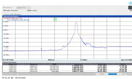
NTNV-n78(3700-3800)-PC1.5-30-15-H-DFT-BPSK-Edge_1RB_Right-PA SS
