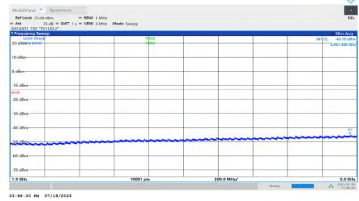
NTNV-n78(3450-3550)-PC1.5-30-70-H-DFT-QPSK-Inner_1RB_Left-10 00-3000-PASS
