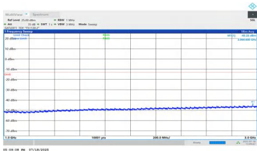
NTNV-n78(3450-3550)-PC1.5-30-90-M-DFT-QPSK-Inner_1RB_Right- 1000-3000-PASS
