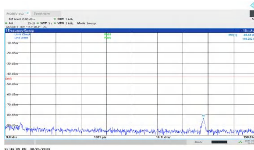
NTNV-n78(3450-3550)-PC1.5-30-80-H-DFT-BPSK-Inner_1RB_Right-0 .009-0.15-PASS
