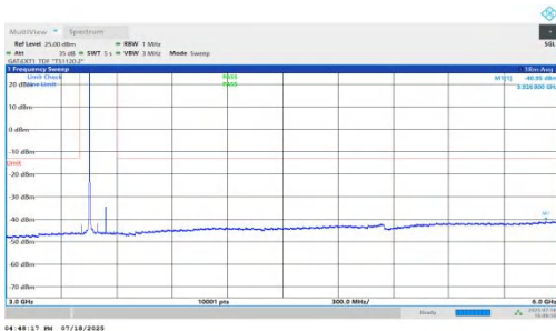
NTNV-n78(3450-3550)-PC1.5-30-90-L-DFT-BPSK-Inner_1RB_Left-3000-6000-PASS
