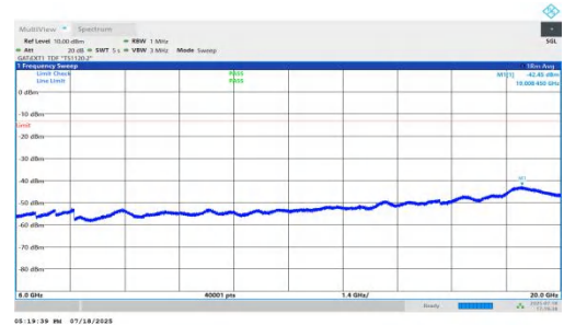
NTNV-n78(3450-3550)-PC1.5-30-90-H-DFT-QPSK-Inner_1RB_Left-60 00-20000-PASS
