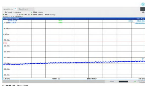
NTNV-n78(3450-3550)-PC1.5-30-100-L-DFT-BPSK-Inner_1RB_Left-1000-3000-PASS
