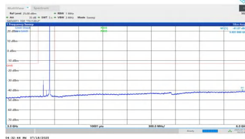
NTNV-n78(3450-3550)-PC1.5-30-80-M-DFT-QPSK-Inner_1RB_Right-3000-6000-PASS
