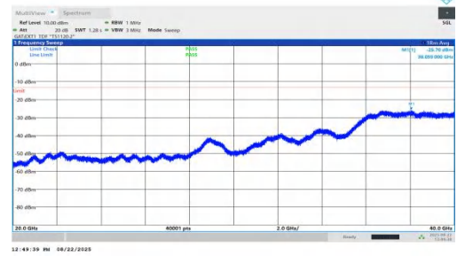
NTNV-n78(3450-3550)-PC1.5-30-80-H-DFT-BPSK-Inner_1RB_Right-20000-40000-PASS
