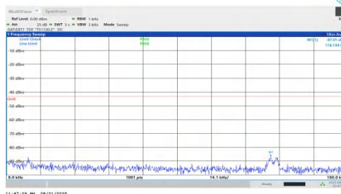
NTNV-n78(3450-3550)-PC1.5-30-80-H-DFT-QPSK-Inner_1RB_Right-0 .009-0.15-PASS
