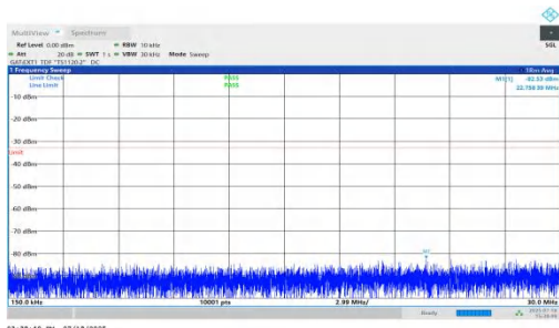
NTNV-n78(3450-3550)-PC1.5-30-70-M-DFT-QPSK-Inner_1RB_Right- 0.15-30-PASS
