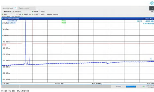
NTNV-n78(3450-3550)-PC1.5-30-90-H-DFT-QPSK-Inner_1RB_Left-3 000-6000-PASS
