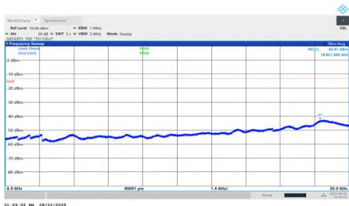
NTNV-n78(3450-3550)-PC1.5-30-100-L-DFT-QPSK-Inner_1RB_Right-6000-20000-PASS
