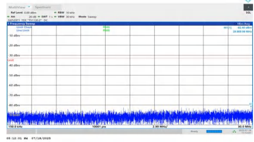
NTNV-n78(3450-3550)-PC1.5-30-90-H-DFT-BPSK-Inner_1RB_Left-0.15-30-PASS
