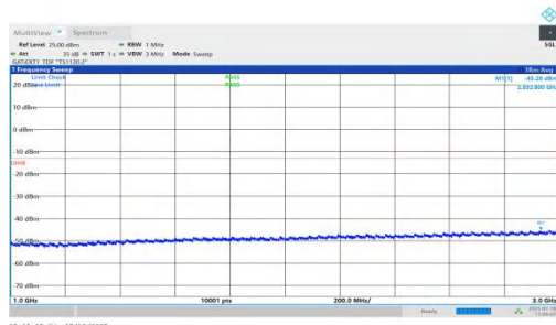
NTNV-n78(3450-3550)-PC1.5-30-90-M-DFT-BPSK-Inner_1RB_Left-1000-3000-PASS
