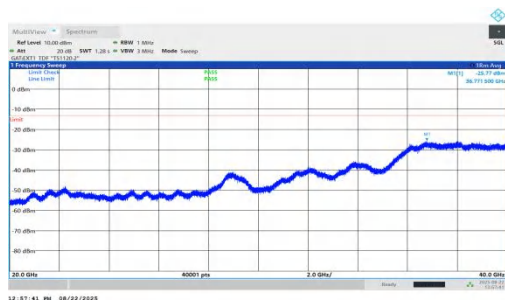
NTNV-n78(3450-3550)-PC1.5-30-90-H-DFT-QPSK-Inner_1RB_Right-20000-40000-PASS
