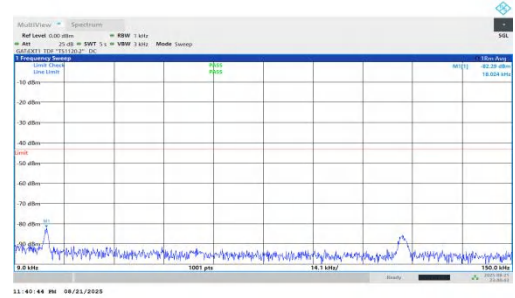
NTNV-n78(3450-3550)-PC1.5-30-80-L-DFT-BPSK-Inner_1RB_Right-0. 009-0.15-PASS
