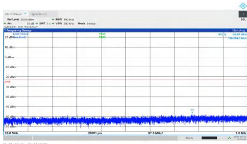
NTNV-n78(3450-3550)-PC1.5-30-100-L-DFT-QPSK-Inner_1RB_Left- 30-1000-PASS
