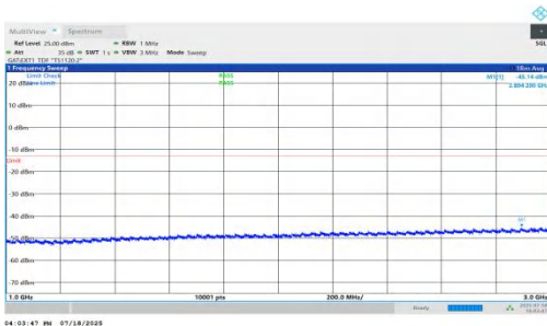
NTVN-n78(3450-3550)-PC1.5-30-80-L-DFT-QPSK-Inner_1RB_Right- 1000-3000-PASS
