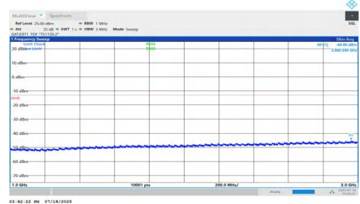
NTNV-n78(3450-3550)-PC1.5-30-70-H-DFT-BPSK-Inner_1RB_Left-1000-3000-PASS
