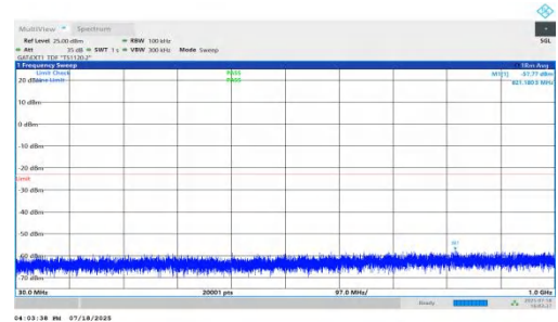
NTVN-n78(3450-3550)-PC1.5-30-80-L-DFT-QPSK-Inner_1RB_Right-3 0-1000-PASS
