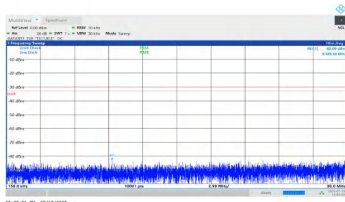
NTNV-n78(3450-3550)-PC1.5-30-90-M-DFT-QPSK-Inner_1RB_Left-0.15-30-PASS
