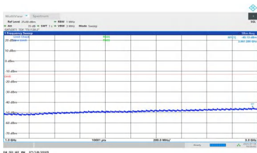
NTNV-n78(3450-3550)-PC1.5-30-90-L-DFT-BPSK-Inner_1RB_Right-1000-3000-PASS
