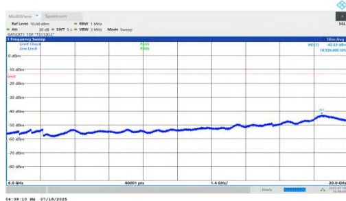
NTNV-n78(3450-3550)-PC1.5-30-80-M-DFT-BPSK-Inner_1RB_Left-6000-20000-PASS
