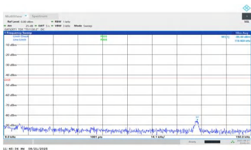
NTNV-n78(3450-3550)-PC1.5-30-80-H-DFT-BPSK-Inner_1RB_Left-0.009-0.15-PASS
