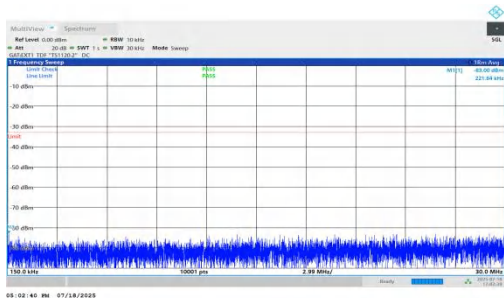
NTNV-n78(3450-3550)-PC1.5-30-90-M-DFT-BPSK-Inner_1RB_Right- 0.15-30-PASS
