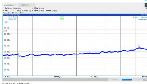
NTNV-n78(3450-3550)-PC1.5-30-90-M-DFT-BPSK-Inner_1RB_Left-60 00-20000-PASS
