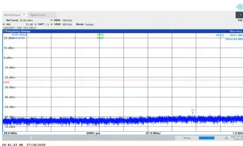
NTNV-n78(3450-3550)-PC1.5-30-80-H-DFT-QPSK-Inner_1RB_Left-30-1000-PASS
