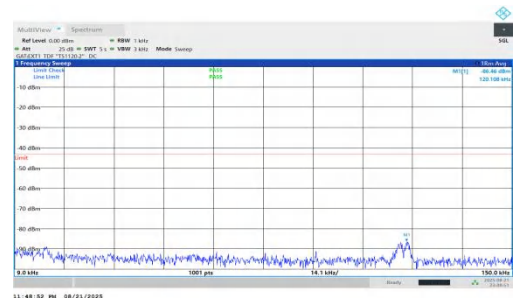
NTNV-n78(3450-3550)-PC1.5-30-90-L-DFT-BPSK-Inner_1RB_Right-0.009-0.15-PASS
