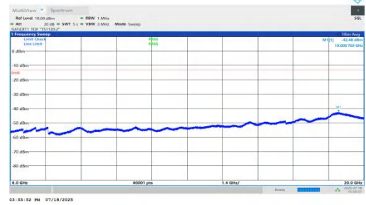
NTNV-n78(3450-3550)-PC1.5-30-80-L-DFT-BPSK-Inner_1RB_Left-60 00-20000-PASS
