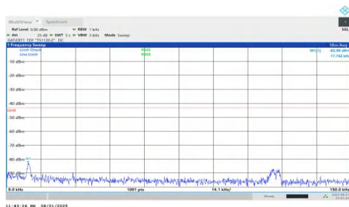
NTNV-n78(3450-3550)-PC1.5-30-80-M-DFT-BPSK-Inner_1RB_Right-0.009-0.15-PASS
