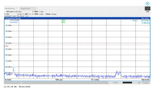
NTV-n78(3450-3550)-PC1.5-30-90-L-DFT-QPSK-Inner_1RB_Right-0 .009-0.15-PASS
