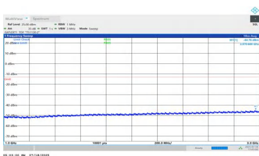
NTNV-n78(3450-3550)-PC1.5-30-90-M-DFT-BPSK-Inner_1RB_Right- 1000-3000-PASS
