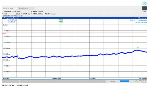
NTNV-n78(3450-3550)-PC1.5-30-90-H-DFT-BPSK-Inner_1RB_Right-6000-20000-PASS
