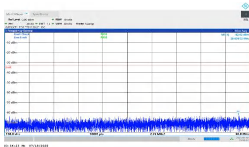
NTNV-n78(3450-3550)-PC1.5-30-80-L-DFT-BPSK-Inner_1RB_Left-0.15-30-PASS
