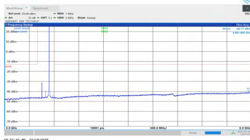
NTNV-n78(3450-3550)-PC1.5-30-90-L-DFT-QPSK-Inner_1RB_Right-3000-6000-PASS
