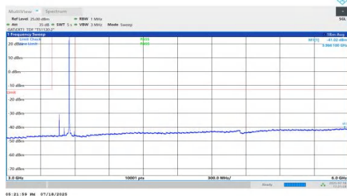
NTNV-n78(3450-3550)-PC1.5-30-90-H-DFT-QPSK-Inner_1RB_Right-3000-6000-PASS
