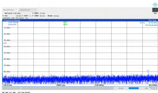
NTNV-n78(3450-3550)-PC1.5-30-80-H-DFT-QPSK-Inner_1RB_Right- 0.15-30-PASS
