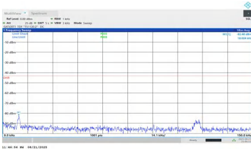
NTNV-n78(3450-3550)-PC1.5-30-80-H-DFT-QPSK-Inner_1RB_Left-0.009-0.15-PASS
