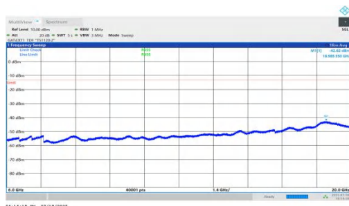
NTNV-n78(3450-3550)-PC1.5-30-80-M-DFT-QPSK-Inner_1RB_Left-60 00-20000-PASS
