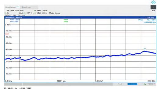
NTNV-n78(3450-3550)-PC1.5-30-70-H-DFT-BPSK-Inner_1RB_Left-6000-20000-PASS
