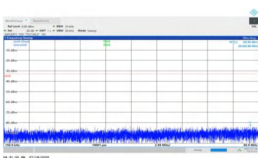
NTNV-n78(3450-3550)-PC1.5-30-80-M-DFT-QPSK-Inner_1RB_Right- 0.15-30-PASS
