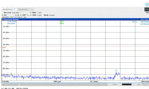
NTNV-n78(3450-3550)-PC1.5-30-80-M-DFT-QPSK-Inner_1RB_Left-0.009-0.15-PASS
