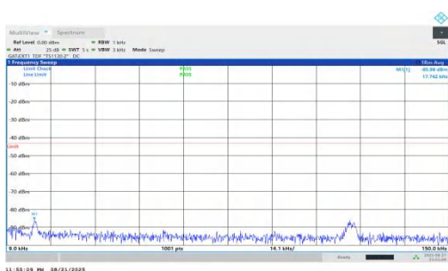
NTNV-n78(3450-3550)-PC1.5-30-90-H-DFT-QPSK-Inner_1RB_Left-0.009-0.15-PASS
