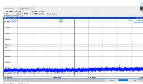
NTNV-n78(3450-3550)-PC1.5-30-70-M-DFT-QPSK-Inner_1RB_Right- 30-1000-PASS
