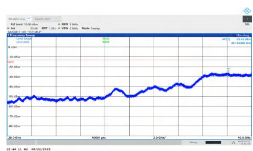
NTVN-n78(3450-3550)-PC1.5-30-80-L-DFT-QPSK-Inner_1RB_Right-2 0000-40000-PASS
