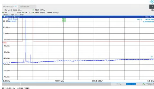
NTNV-n78(3450-3550)-PC1.5-30-90-H-DFT-BPSK-Inner_1RB_Left-3000-6000-PASS
