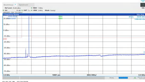
NTNV-n78(3450-3550)-PC1.5-30-70-H-DFT-QPSK-Inner_1RB_Right-3000-6000-PASS
