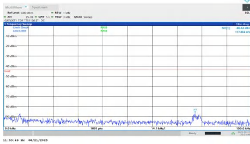
NTNV-n78(3450-3550)-PC1.5-30-90-H-DFT-BPSK-Inner_1RB_Left-0.009-0.15-PASS
