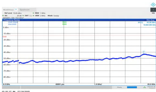
NTNV-n78(3450-3550)-PC1.5-30-70-H-DFT-QPSK-Inner_1RB_Right-6000-20000-PASS
