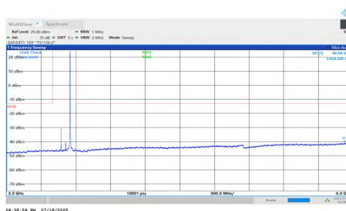
NTNV-n78(3450-3550)-PC1.5-30-80-H-DFT-BPSK-Inner_1RB_Right-3 000-6000-PASS
