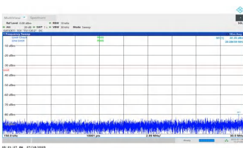
NTNV-n78(3450-3550)-PC1.5-30-90-H-DFT-QPSK-Inner_1RB_Right- 0.15-30-PASS
