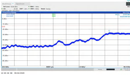
NTVN-n78(3450-3550)-PC1.5-30-80-L-DFT-QPSK-Inner_1RB_Left-2 0000-40000-PASS
