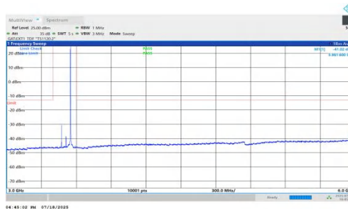
NTNV-n78(3450-3550)-PC1.5-30-80-H-DFT-QPSK-Inner_1RB_Right-3 000-6000-PASS
