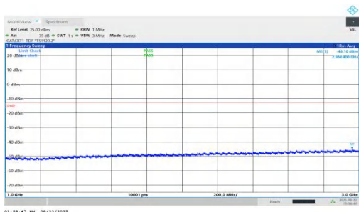
NTNV-n78(3450-3550)-PC1.5-30-100-L-DFT-QPSK-Inner_1RB_Right-1000-3000-PASS
