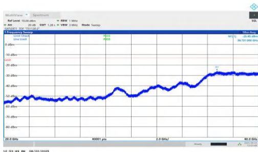
NTNV-n78(3450-3550)-PC1.5-30-90-M-DFT-BPSK-Inner_1RB_Left-2 0000-40000-PASS
