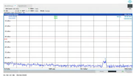
NTNV-n78(3450-3550)-PC1.5-30-100-L-DFT-BPSK-Inner_1RB_Right- 0.009-0.15-PASS
