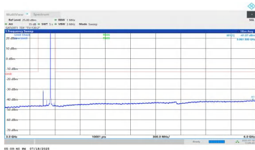
NTNV-n78(3450-3550)-PC1.5-30-90-M-DFT-QPSK-Inner_1RB_Right- 3000-6000-PASS
