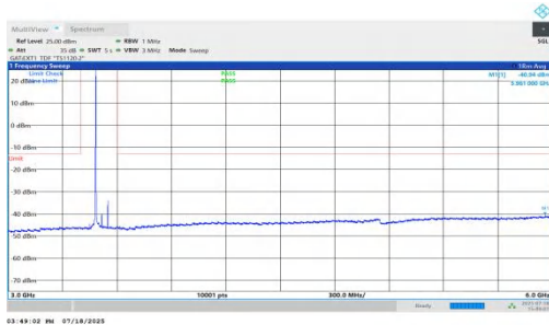
NTNV-n78(3450-3550)-PC1.5-30-70-H-DFT-QPSK-Inner_1RB_Left-3 000-6000-PASS
