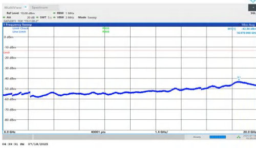
NTNV-n78(3450-3550)-PC1.5-30-80-H-DFT-BPSK-Inner_1RB_Right-6000-20000-PASS
