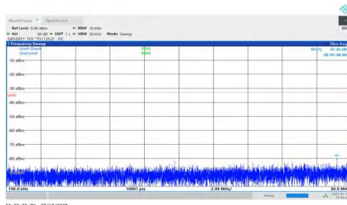
NTVN-n78(3450-3550)-PC1.5-30-80-L-DFT-QPSK-Inner_1RB_Left-0.15-30-PASS
