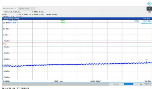
NTNV-n78(3450-3550)-PC1.5-30-80-H-DFT-QPSK-Inner_1RB_Right- 1000-3000-PASS
