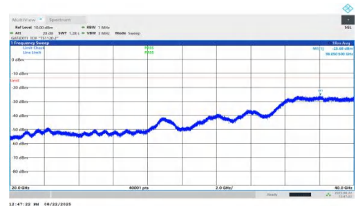
NTNV-n78(3450-3550)-PC1.5-30-80-M-DFT-BPSK-Inner_1RB_Right-2 0000-40000-PASS
