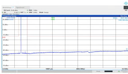
NTNV-n78(3450-3550)-PC1.5-30-100-L-DFT-QPSK-Inner_1RB_Left- 3000-6000-PASS
