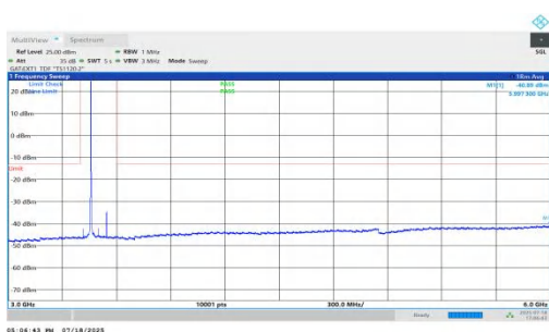
NTNV-n78(3450-3550)-PC1.5-30-90-M-DFT-QPSK-Inner_1RB_Left-3000-6000-PASS
