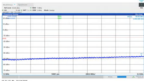
NTNV-n78(3450-3550)-PC1.5-30-70-H-DFT-QPSK-Inner_1RB_Right-1000-3000-PASS
