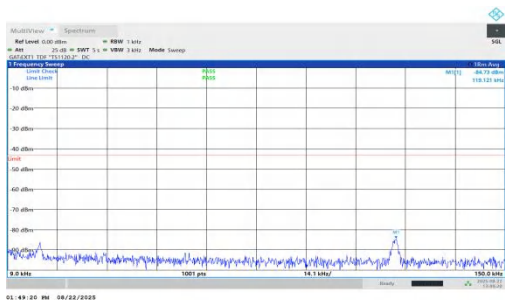
NTNV-n78(3450-3550)-PC1.5-30-100-L-DFT-BPSK-Inner_1RB_Left-0.009-0.15-PASS
