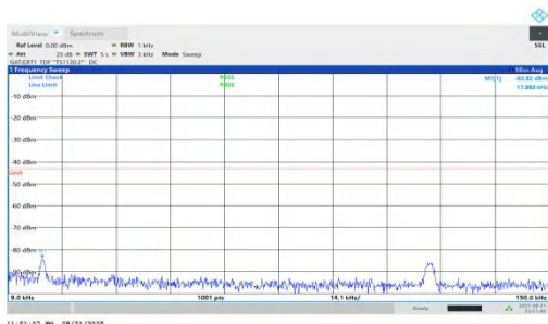
NTNV-n78(3450-3550)-PC1.5-30-90-M-DFT-BPSK-Inner_1RB_Left-0.009-0.15-PASS
