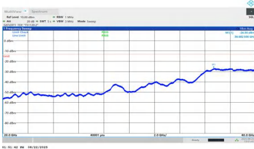
NTNV-n78(3450-3550)-PC1.5-30-100-L-DFT-BPSK-Inner_1RB_Left-2 0000-40000-PASS
