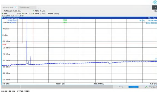
NTNV-n78(3450-3550)-PC1.5-30-70-H-DFT-BPSK-Inner_1RB_Left-3000-6000-PASS
