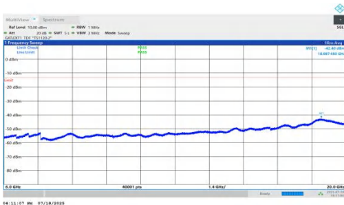
NTNV-n78(3450-3550)-PC1.5-30-80-M-DFT-BPSK-Inner_1RB_Right-6000-20000-PASS
