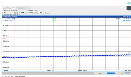
NTNV-n78(3450-3550)-PC1.5-30-70-M-DFT-QPSK-Inner_1RB_Right- 1000-3000-PASS
