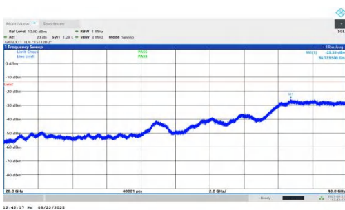
NTNV-n78(3450-3550)-PC1.5-30-70-H-DFT-BPSK-Inner_1RB_Left-20000-40000-PASS
