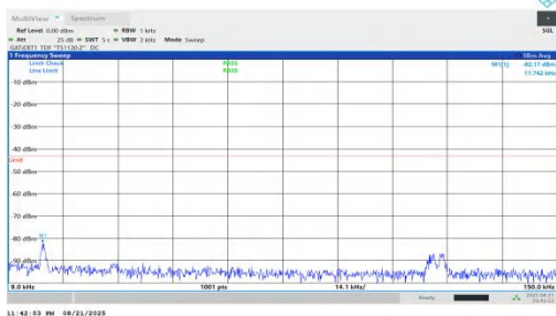
NTNV-n78(3450-3550)-PC1.5-30-80-M-DFT-BPSK-Inner_1RB_Left-0.009-0.15-PASS
