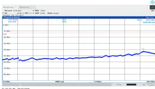
NTNV-n78(3450-3550)-PC1.5-30-100-L-DFT-BPSK-Inner_1RB_Right -6000-20000-PASS
