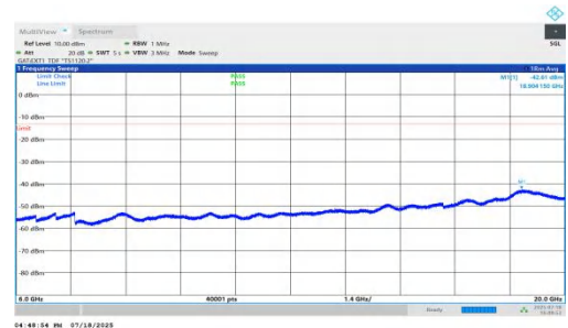
NTNV-n78(3450-3550)-PC1.5-30-90-L-DFT-BPSK-Inner_1RB_Left-6000-20000-PASS
