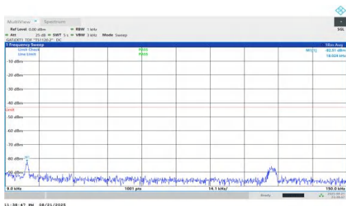
NTNV-n78(3450-3550)-PC1.5-30-70-H-DFT-QPSK-Inner_1RB_Left-0.009-0.15-PASS
