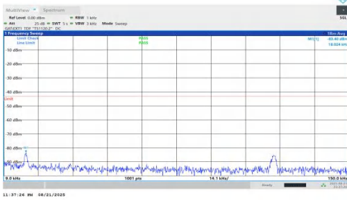
NTNV-n78(3450-3550)-PC1.5-30-70-H-DFT-BPSK-Inner_1RB_Left-0.009-0.15-PASS
