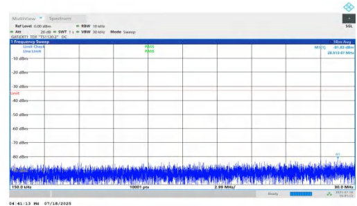
NTNV-n78(3450-3550)-PC1.5-30-80-H-DFT-QPSK-Inner_1RB_Left-0.15-30-PASS
