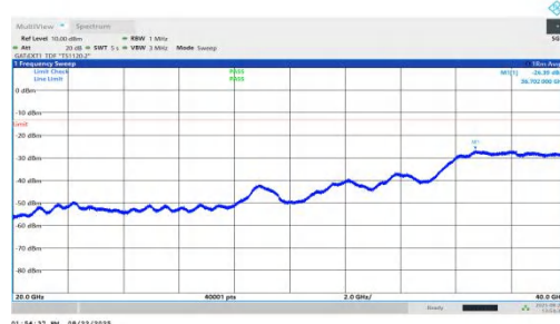
NTNV-n78(3450-3550)-PC1.5-30-100-L-DFT-BPSK-Inner_1RB_Right- 20000-40000-PASS
