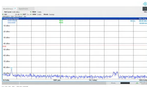
NTVN-n78(3450-3550)-PC1.5-30-80-L-DFT-QPSK-Inner_1RB_Left-0.009-0.15-PASS
