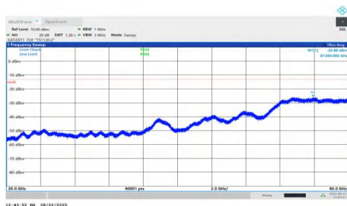
NTNV-n78(3450-3550)-PC1.5-30-70-H-DFT-QPSK-Inner_1RB_Right-20000-40000-PASS
