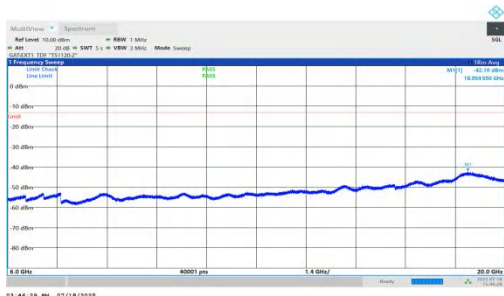
NTNV-n78(3450-3550)-PC1.5-30-70-H-DFT-BPSK-Inner_1RB_Right-6000-20000-PASS
