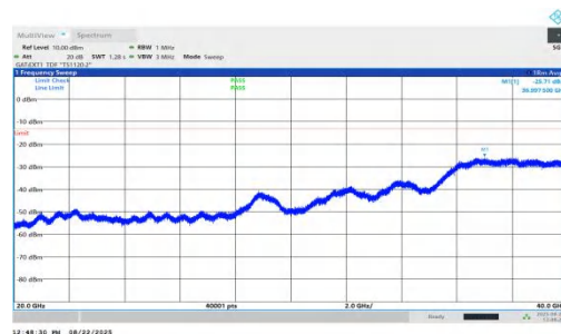
NTNV-n78(3450-3550)-PC1.5-30-80-M-DFT-QPSK-Inner_1RB_Right-20000-40000-PASS
