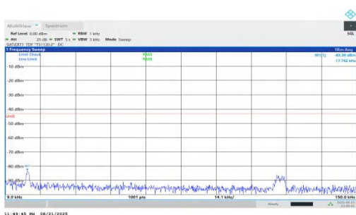
NTNV-n78(3450-3550)-PC1.5-30-90-L-DFT-QPSK-Inner_1RB_Left-0.009-0.15-PASS
