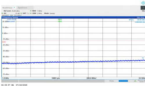
NTNV-n78(3450-3550)-PC1.5-30-80-M-DFT-BPSK-Inner_1RB_Right-1000-3000-PASS
