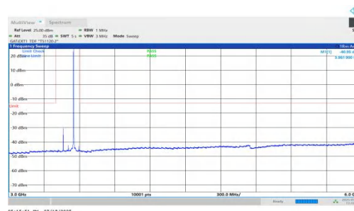
NTNV-n78(3450-3550)-PC1.5-30-90-H-DFT-BPSK-Inner_1RB_Right-3 000-6000-PASS
