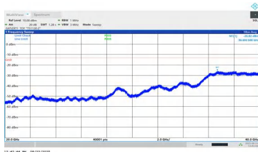
NTNV-n78(3450-3550)-PC1.5-30-70-H-DFT-BPSK-Inner_1RB_Right-2 0000-40000-PASS
