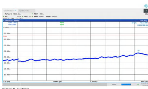
NTNV-n78(3450-3550)-PC1.5-30-90-M-DFT-QPSK-Inner_1RB_Left-6000-20000-PASS
