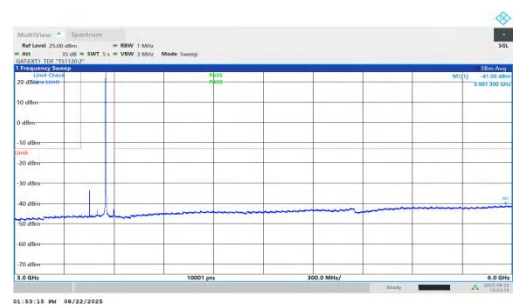
NTNV-n78(3450-3550)-PC1.5-30-100-L-DFT-BPSK-Inner_1RB_Right- 3000-6000-PASS
