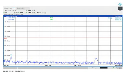
NTNV-n78(3450-3550)-PC1.5-30-70-H-DFT-BPSK-Inner_1RB_Right-0.009-0.15-PASS
