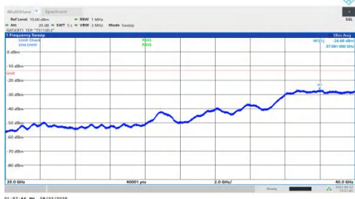
NTNV-n78(3450-3550)-PC1.5-30-100-L-DFT-QPSK-Inner_1RB_Left-20000-40000-PASS
