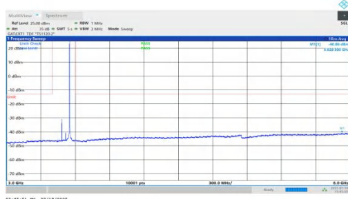
NTNV-n78(3450-3550)-PC1.5-30-70-H-DFT-BPSK-Inner_1RB_Right-3 000-6000-PASS
