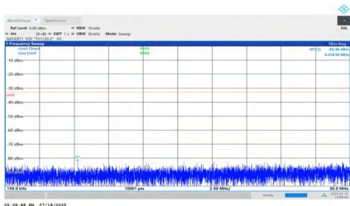
NTNV-n78(3450-3550)-PC1.5-30-90-M-DFT-QPSK-Inner_1RB_Right- 0.15-30-PASS
