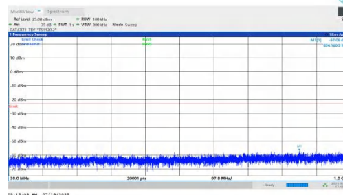
NTNV-n78(3450-3550)-PC1.5-30-90-H-DFT-BPSK-Inner_1RB_Right-3 0-1000-PASS
