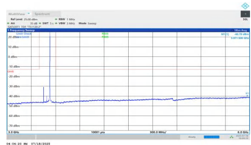
NTVN-n78(3450-3550)-PC1.5-30-80-L-DFT-QPSK-Inner_1RB_Right-3 000-6000-PASS
