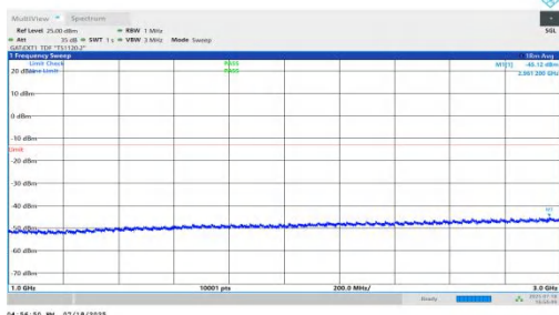
NTNV-n78(3450-3550)-PC1.5-30-90-L-DFT-QPSK-Inner_1RB_Right-1000-3000-PASS
