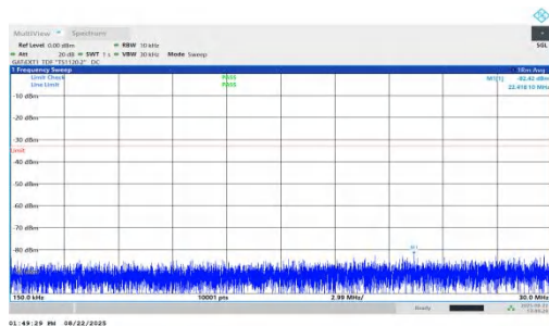
NTNV-n78(3450-3550)-PC1.5-30-100-L-DFT-BPSK-Inner_1RB_Left-0.15-30-PASS
