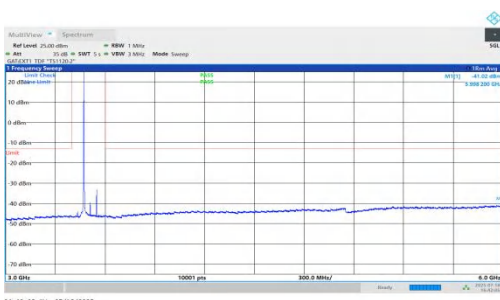
NTNV-n78(3450-3550)-PC1.5-30-80-H-DFT-QPSK-Inner_1RB_Left-3000-6000-PASS
