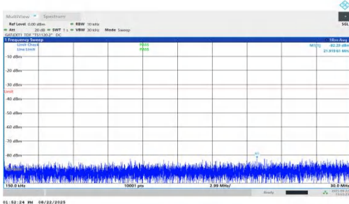
NTNV-n78(3450-3550)-PC1.5-30-100-L-DFT-BPSK-Inner_1RB_Right -0.15-30-PASS
