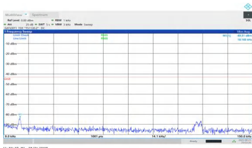
NTNV-n78(3450-3550)-PC1.5-30-90-M-DFT-QPSK-Inner_1RB_Left-0.009-0.15-PASS
