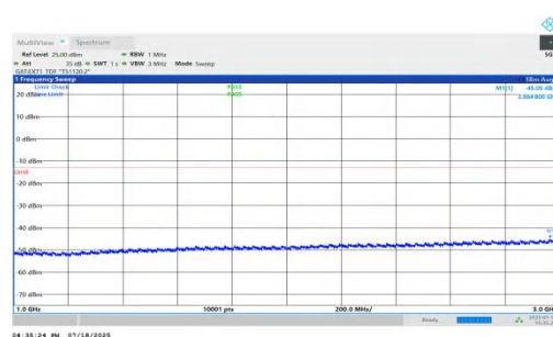
NTNV-n78(3450-3550)-PC1.5-30-80-H-DFT-BPSK-Inner_1RB_Left-1000-3000-PASS
