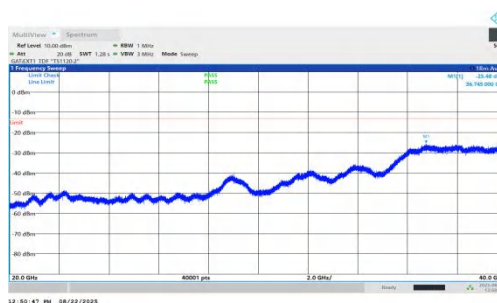
NTNV-n78(3450-3550)-PC1.5-30-80-H-DFT-QPSK-Inner_1RB_Right-2 0000-40000-PASS
