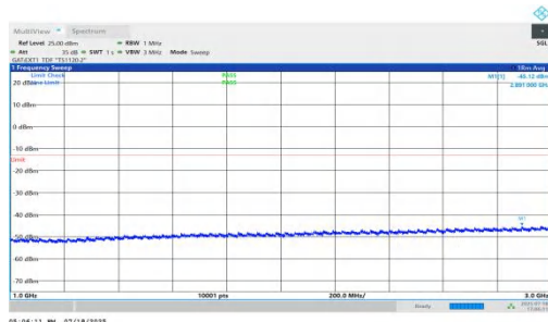
NTNV-n78(3450-3550)-PC1.5-30-90-M-DFT-QPSK-Inner_1RB_Left-1000-3000-PASS
