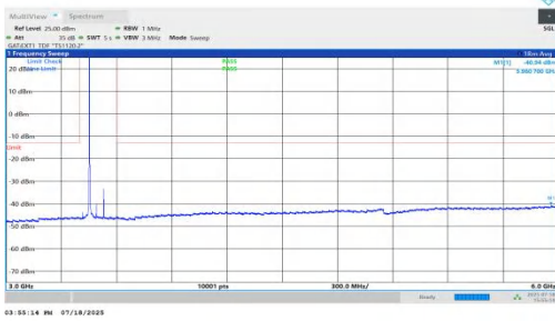
NTNV-n78(3450-3550)-PC1.5-30-80-L-DFT-BPSK-Inner_1RB_Left-30 00-6000-PASS
