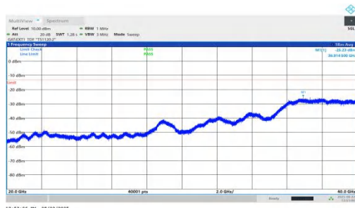
NTNV-n78(3450-3550)-PC1.5-30-90-L-DFT-QPSK-Inner_1RB_Right-20000-40000-PASS
