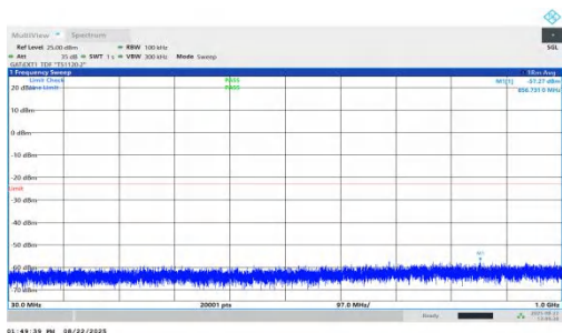
NTNV-n78(3450-3550)-PC1.5-30-100-L-DFT-BPSK-Inner_1RB_Left-30-1000-PASS
