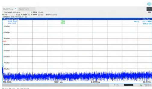
NTNV-n78(3450-3550)-PC1.5-30-100-L-DFT-QPSK-Inner_1RB_Right-0.15-30-PASS
