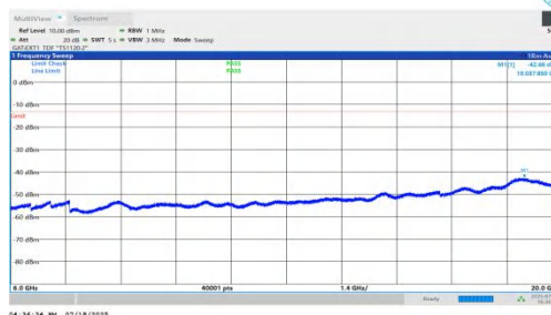
NTNV-n78(3450-3550)-PC1.5-30-80-H-DFT-BPSK-Inner_1RB_Left-60 00-20000-PASS
