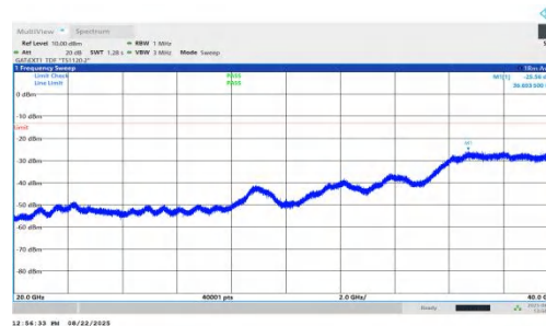
NTNV-n78(3450-3550)-PC1.5-30-90-H-DFT-BPSK-Inner_1RB_Right-2 0000-40000-PASS
