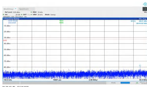
NTNV-n78(3450-3550)-PC1.5-30-90-M-DFT-BPSK-Inner_1RB_Left-0.15-30-PASS
