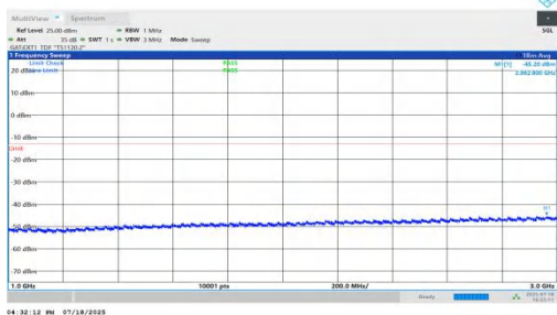
NTNV-n78(3450-3550)-PC1.5-30-80-M-DFT-QPSK-Inner_1RB_Right-1000-3000-PASS
