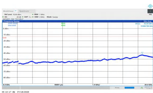
NTNV-n78(3450-3550)-PC1.5-30-90-M-DFT-QPSK-Inner_1RB_Right- 6000-20000-PASS
