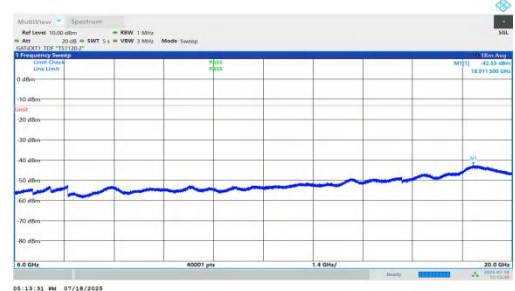
NTNV-n78(3450-3550)-PC1.5-30-90-H-DFT-BPSK-Inner_1RB_Left-6000-20000-PASS
