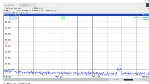
NTNV-n78(3450-3550)-PC1.5-30-70-M-DFT-QPSK-Inner_1RB_Right- 0.009-0.15-PASS
