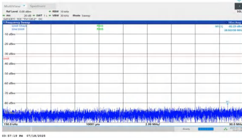
NTNV-n78(3450-3550)-PC1.5-30-80-L-DFT-BPSK-Inner_1RB_Right- 0.15-30-PASS
