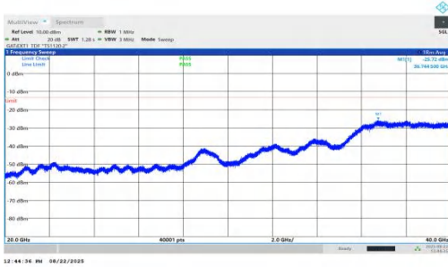
NTNV-n78(3450-3550)-PC1.5-30-80-L-DFT-BPSK-Inner_1RB_Left-20 000-40000-PASS
