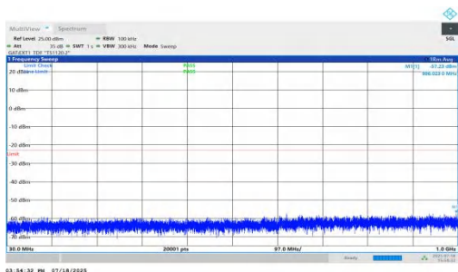
NTNV-n78(3450-3550)-PC1.5-30-80-L-DFT-BPSK-Inner_1RB_Left-30-1000-PASS
