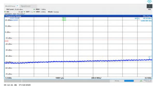
NTNV-n78(3450-3550)-PC1.5-30-90-H-DFT-BPSK-Inner_1RB_Left-1000-3000-PASS
