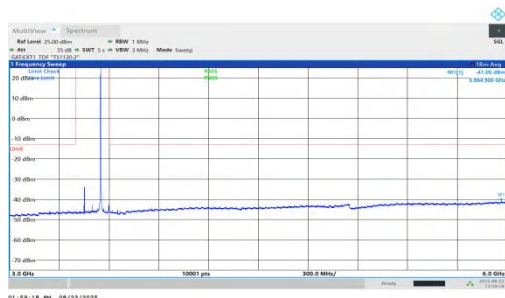
NTNV-n78(3450-3550)-PC1.5-30-100-L-DFT-QPSK-Inner_1RB_Right-3000-6000-PASS
