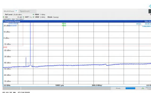
NTNV-n78(3450-3550)-PC1.5-30-90-M-DFT-BPSK-Inner_1RB_Right-3 000-6000-PASS
