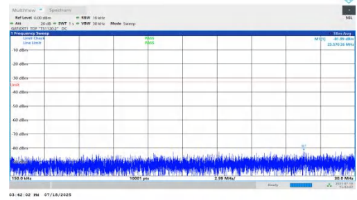
NTNV-n78(3450-3550)-PC1.5-30-70-H-DFT-BPSK-Inner_1RB_Left-0.15-30-PASS
