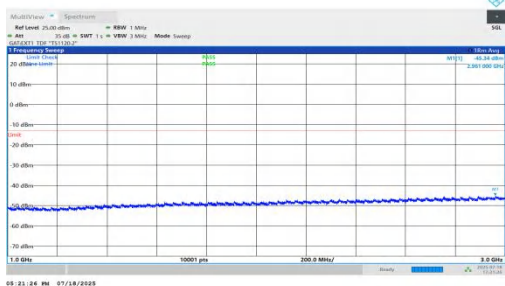
NTNV-n78(3450-3550)-PC1.5-30-90-H-DFT-QPSK-Inner_1RB_Right-1000-3000-PASS
