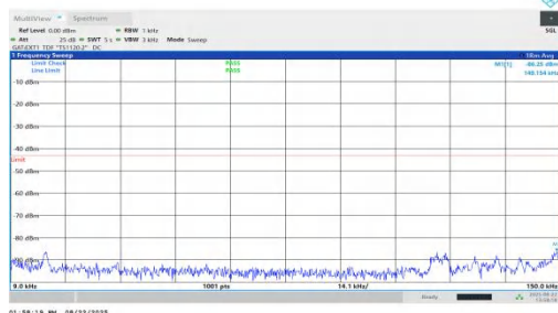
NTNV-n78(3450-3550)-PC1.5-30-100-L-DFT-QPSK-Inner_1RB_Right-0.009-0.15-PASS
