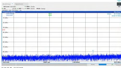
NTNV-n78(3450-3550)-PC1.5-30-70-H-DFT-BPSK-Inner_1RB_Right-0.15-30-PASS
