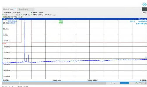
NTNV-n78(3450-3550)-PC1.5-30-80-M-DFT-QPSK-Inner_1RB_Left-3 000-6000-PASS
