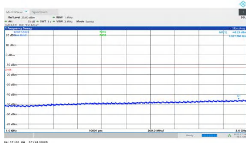
NTNV-n78(3450-3550)-PC1.5-30-80-M-DFT-BPSK-Inner_1RB_Left-1000-3000-PASS
