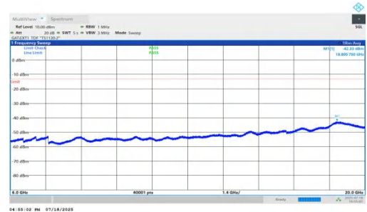
NTV-n78(3450-3550)-PC1.5-30-90-L-DFT-QPSK-Inner_1RB_Left-60 00-20000-PASS
