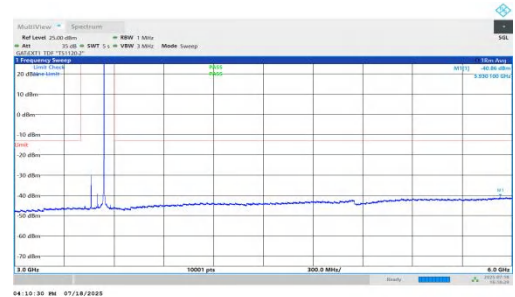
NTNV-n78(3450-3550)-PC1.5-30-80-M-DFT-BPSK-Inner_1RB_Right-3 000-6000-PASS
