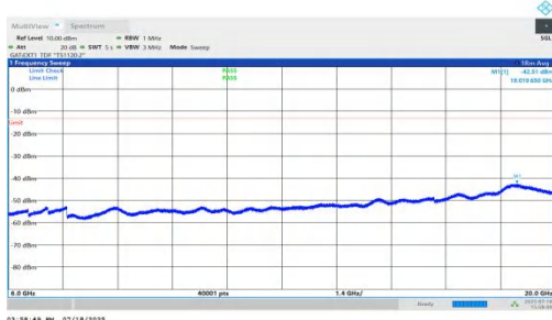
NTVN-n78(3450-3550)-PC1.5-30-80-L-DFT-BPSK-Inner_1RB_Right-6000-20000-PASS
