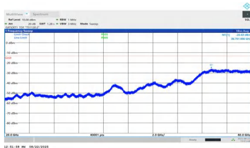
NTNV-n78(3450-3550)-PC1.5-30-90-L-DFT-BPSK-Inner_1RB_Right-2 0000-40000-PASS
