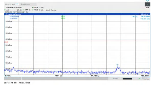
NTVN-n78(3450-3550)-PC1.5-30-80-L-DFT-QPSK-Inner_1RB_Right-0 .009-0.15-PASS
