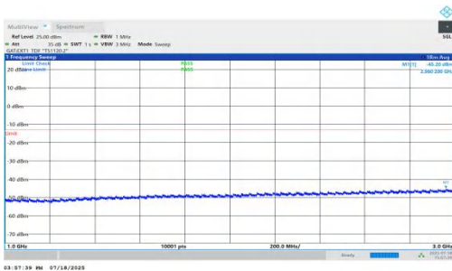
NTNV-n78(3450-3550)-PC1.5-30-80-L-DFT-BPSK-Inner_1RB_Right- 1000-3000-PASS
