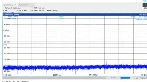
NTNV-n78(3450-3550)-PC1.5-30-90-L-DFT-BPSK-Inner_1RB_Right-3 0-1000-PASS
