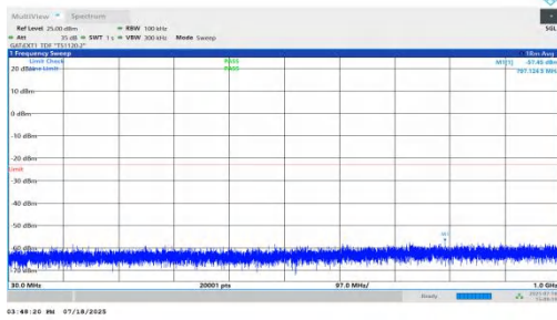
NTNV-n78(3450-3550)-PC1.5-30-70-H-DFT-QPSK-Inner_1RB_Left-3 0-1000-PASS
