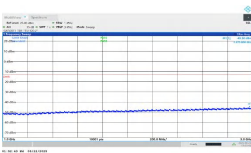
NTNV-n78(3450-3550)-PC1.5-30-100-L-DFT-BPSK-Inner_1RB_Right -1000-3000-PASS
