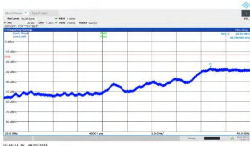
NTNV-n78(3450-3550)-PC1.5-30-80-H-DFT-BPSK-Inner_1RB_Left-2 0000-40000-PASS
