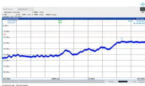
NTNV-n78(3450-3550)-PC1.5-30-80-M-DFT-BPSK-Inner_1RB_Left-20000-40000-PASS
