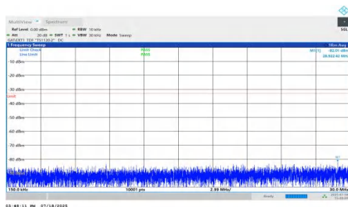
NTNV-n78(3450-3550)-PC1.5-30-70-H-DFT-QPSK-Inner_1RB_Left-0.15-30-PASS
