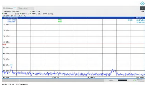
NTNV-n78(3450-3550)-PC1.5-30-80-L-DFT-BPSK-Inner_1RB_Left-0.009-0.15-PASS
