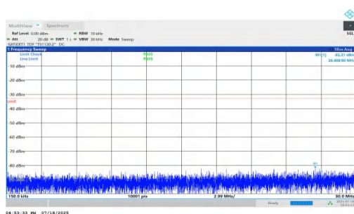
NTNV-n78(3450-3550)-PC1.5-30-90-L-DFT-QPSK-Inner_1RB_Left-0.1 5-30-PASS
