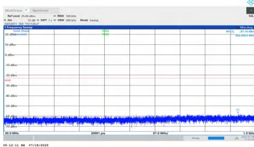
NTNV-n78(3450-3550)-PC1.5-30-90-H-DFT-BPSK-Inner_1RB_Left-3000-1000-PASS
