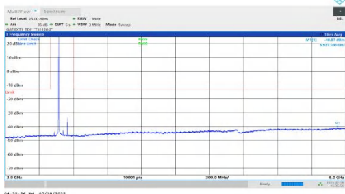
NTNV-n78(3450-3550)-PC1.5-30-80-H-DFT-BPSK-Inner_1RB_Left-3 000-6000-PASS
