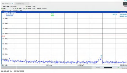
NTNV-n78(3450-3550)-PC1.5-30-90-L-DFT-BPSK-Inner_1RB_Left-0.009-0.15-PASS
