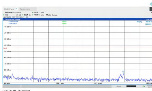
NTNV-n78(3450-3550)-PC1.5-30-90-M-DFT-BPSK-Inner_1RB_Right-0 .009-0.15-PASS
