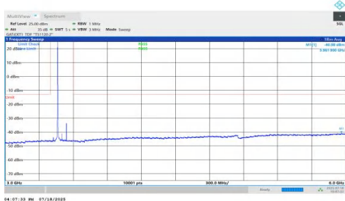
NTNV-n78(3450-3550)-PC1.5-30-80-M-DFT-BPSK-Inner_1RB_Left-3000-6000-PASS
