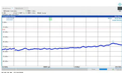
NTNV-n78(3450-3550)-PC1.5-30-80-H-DFT-QPSK-Inner_1RB_Right- 6000-20000-PASS
