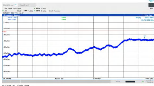
NTNV-n78(3450-3550)-PC1.5-30-80-H-DFT-QPSK-Inner_1RB_Left-2 0000-40000-PASS
