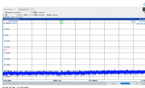
NTNV-n78(3450-3550)-PC1.5-30-80-H-DFT-QPSK-Inner_1RB_Right-3 0-1000-PASS
