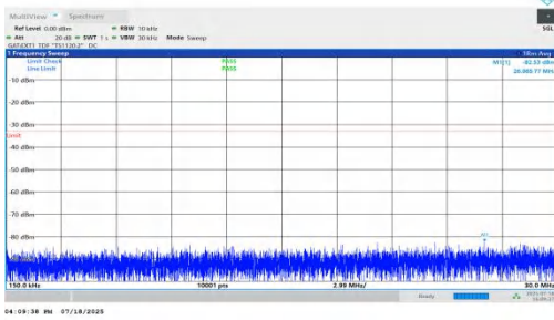
NTNV-n78(3450-3550)-PC1.5-30-80-M-DFT-BPSK-Inner_1RB_Right-0.15-30-PASS
