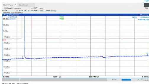
NTNV-n78(3450-3550)-PC1.5-30-90-M-DFT-BPSK-Inner_1RB_Left-3 000-6000-PASS
