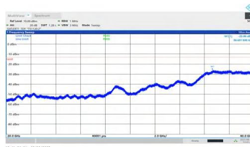
NTNV-n78(3450-3550)-PC1.5-30-70-M-DFT-QPSK-Inner_1RB_Right- 20000-40000-PASS
