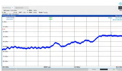
NTNV-n78(3450-3550)-PC1.5-30-90-H-DFT-BPSK-Inner_1RB_Left-20000-40000-PASS
