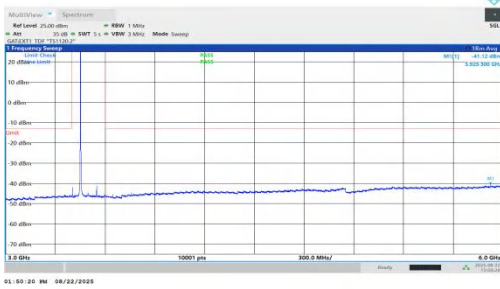
NTNV-n78(3450-3550)-PC1.5-30-100-L-DFT-BPSK-Inner_1RB_Left-3 000-6000-PASS
