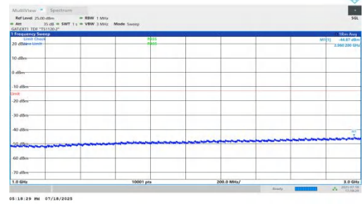
NTNV-n78(3450-3550)-PC1.5-30-90-H-DFT-QPSK-Inner_1RB_Left-10 00-3000-PASS
