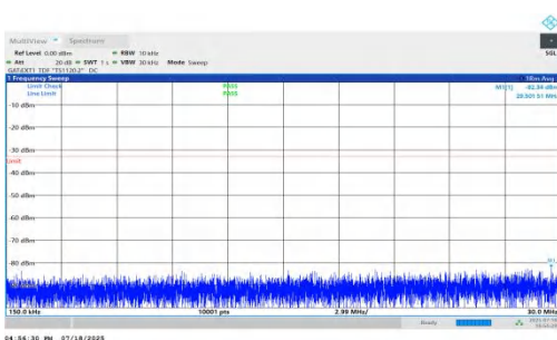
NTV-n78(3450-3550)-PC1.5-30-90-L-DFT-QPSK-Inner_1RB_Right- 0.15-30-PASS
