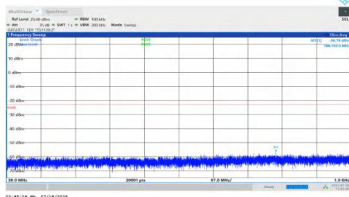
NTNV-n78(3450-3550)-PC1.5-30-70-H-DFT-BPSK-Inner_1RB_Right-3 0-1000-PASS
