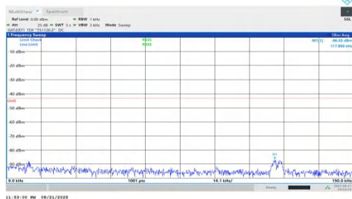
NTNV-n78(3450-3550)-PC1.5-30-90-M-DFT-QPSK-Inner_1RB_Right- 0.009-0.15-PASS
