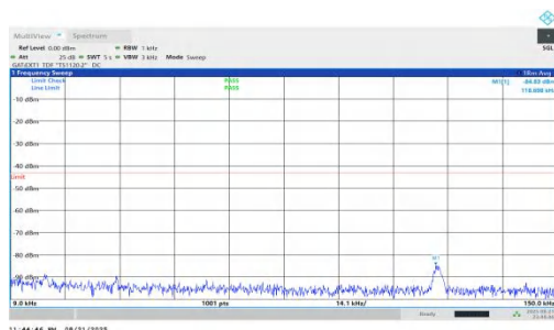
NTNV-n78(3450-3550)-PC1.5-30-80-M-DFT-QPSK-Inner_1RB_Right- 0.009-0.15-PASS
