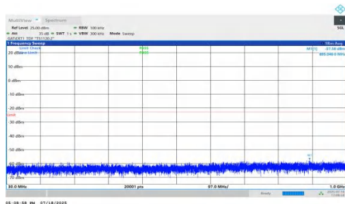
NTNV-n78(3450-3550)-PC1.5-30-90-M-DFT-QPSK-Inner_1RB_Right- 30-1000-PASS
