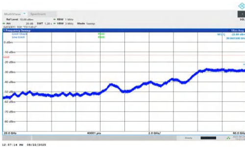
NTNV-n78(3450-3550)-PC1.5-30-90-H-DFT-QPSK-Inner_1RB_Left-2 0000-40000-PASS
