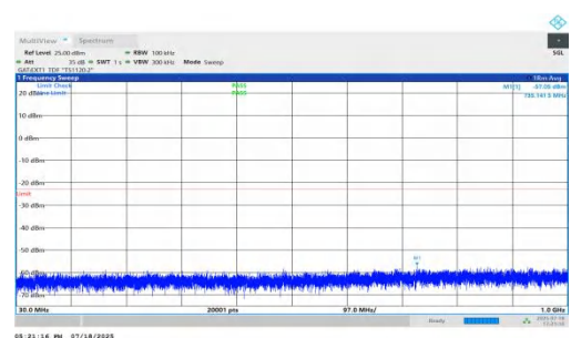
NTNV-n78(3450-3550)-PC1.5-30-90-H-DFT-QPSK-Inner_1RB_Right-3 0-1000-PASS
