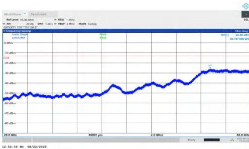
NTV-n78(3450-3550)-PC1.5-30-90-L-DFT-QPSK-Inner_1RB_Left-2 0000-40000-PASS
