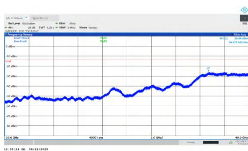
NTNV-n78(3450-3550)-PC1.5-30-90-M-DFT-QPSK-Inner_1RB_Right- 20000-40000-PASS
