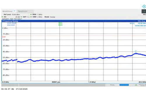
NTVN-n78(3450-3550)-PC1.5-30-80-L-DFT-QPSK-Inner_1RB_Right- 6000-20000-PASS
