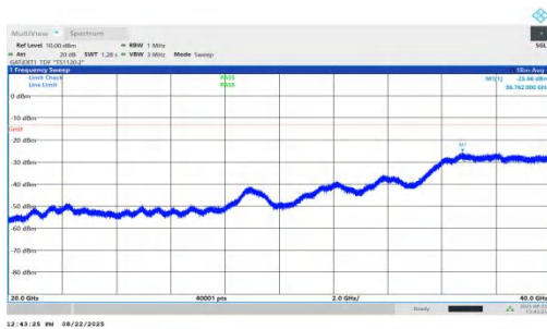
NTNV-n78(3450-3550)-PC1.5-30-70-H-DFT-QPSK-Inner_1RB_Left-2 0000-40000-PASS
