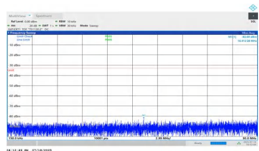
NTNV-n78(3450-3550)-PC1.5-30-80-M-DFT-QPSK-Inner_1RB_Left-0.15-30-PASS
