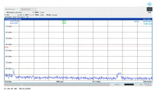
NTNV-n78(3450-3550)-PC1.5-30-70-H-DFT-QPSK-Inner_1RB_Right-0 .009-0.15-PASS
