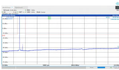
NTVN-n78(3450-3550)-PC1.5-30-80-L-DFT-QPSK-Inner_1RB_Left-3000-6000-PASS
