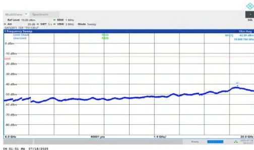
NTNV-n78(3450-3550)-PC1.5-30-90-L-DFT-BPSK-Inner_1RB_Right-6000-20000-PASS
