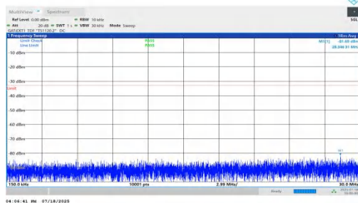
NTNV-n78(3450-3550)-PC1.5-30-80-M-DFT-BPSK-Inner_1RB_Left-0.15-30-PASS
