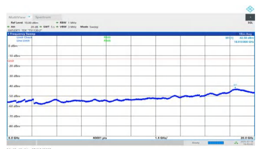
NTNV-n78(3450-3550)-PC1.5-30-80-H-DFT-QPSK-Inner_1RB_Left-6000-20000-PASS
