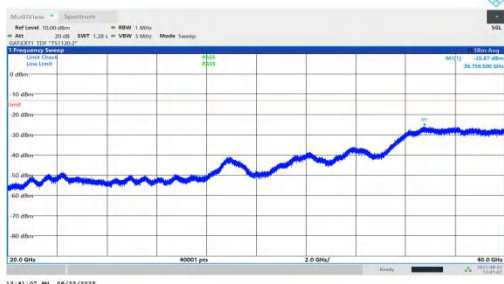
NTNV-n78(3450-3550)-PC1.5-30-70-M-DFT-QPSK-Inner_1RB_Left-2 0000-40000-PASS
