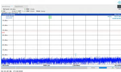
NTVN-n78(3450-3550)-PC1.5-30-80-L-DFT-QPSK-Inner_1RB_Right- 0.15-30-PASS
