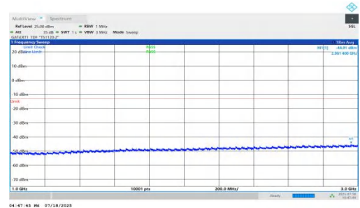
NTNV-n78(3450-3550)-PC1.5-30-90-L-DFT-BPSK-Inner_1RB_Left-1000-3000-PASS
