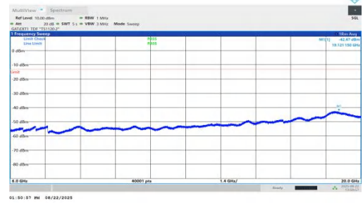
NTNV-n78(3450-3550)-PC1.5-30-100-L-DFT-BPSK-Inner_1RB_Left-6 000-20000-PASS
