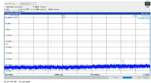
NTNV-n78(3450-3550)-PC1.5-30-80-L-DFT-BPSK-Inner_1RB_Right-3 0-1000-PASS
