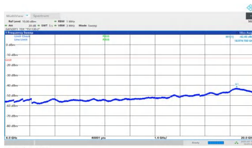
NTVN-n78(3450-3550)-PC1.5-30-80-L-DFT-QPSK-Inner_1RB_Left-6000-20000-PASS
