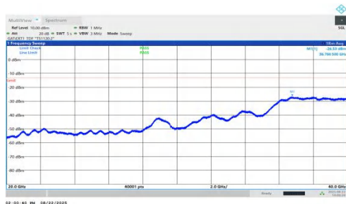
NTNV-n78(3450-3550)-PC1.5-30-100-L-DFT-QPSK-Inner_1RB_Right-20000-40000-PASS
