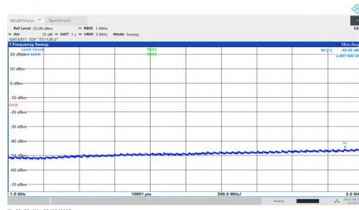
NTNV-n78(3450-3550)-PC1.5-30-100-L-DFT-QPSK-Inner_1RB_Left-1 000-3000-PASS
