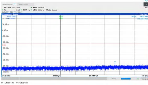
NTNV-n78(3450-3550)-PC1.5-30-90-H-DFT-QPSK-Inner_1RB_Left-3 0-1000-PASS
