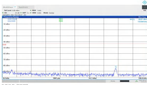
NTNV-n78(3450-3550)-PC1.5-30-100-L-DFT-QPSK-Inner_1RB_Left- 0.009-0.15-PASS
