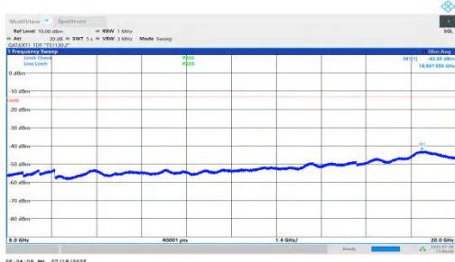
NTNV-n78(3450-3550)-PC1.5-30-90-M-DFT-BPSK-Inner_1RB_Right-6000-20000-PASS
