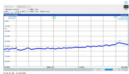
NTNV-n78(3450-3550)-PC1.5-30-70-H-DFT-QPSK-Inner_1RB_Left-60 00-20000-PASS
