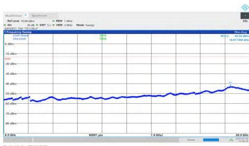
NTNV-n78(3450-3550)-PC1.5-30-70-M-DFT-QPSK-Inner_1RB_Right- 6000-20000-PASS
