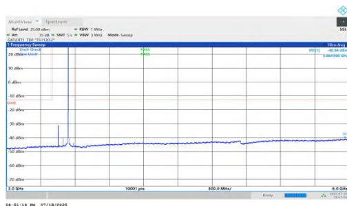
NTNV-n78(3450-3550)-PC1.5-30-90-L-DFT-BPSK-Inner_1RB_Right-3 000-6000-PASS
