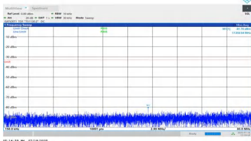
NTNV-n78(3450-3550)-PC1.5-30-90-H-DFT-BPSK-Inner_1RB_Right-0.15-30-PASS
