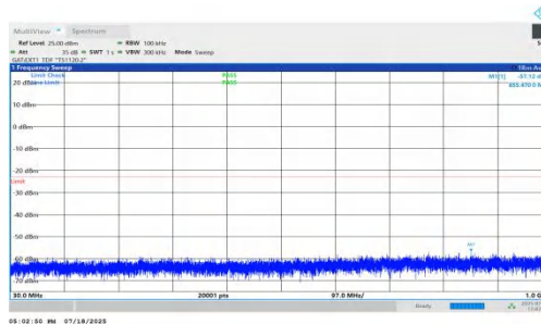
NTNV-n78(3450-3550)-PC1.5-30-90-M-DFT-BPSK-Inner_1RB_Right-3 0-1000-PASS
