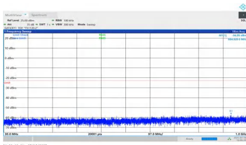
NTVN-n78(3450-3550)-PC1.5-30-80-L-DFT-QPSK-Inner_1RB_Left-30-1000-PASS
