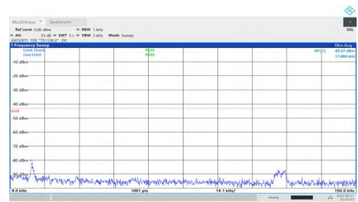
NTNV-n78(3450-3550)-PC1.5-30-90-H-DFT-BPSK-Inner_1RB_Right-0.009-0.15-PASS
