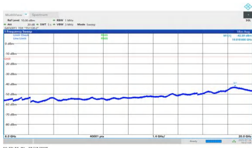
NTNV-n78(3450-3550)-PC1.5-30-90-L-DFT-QPSK-Inner_1RB_Right-6000-20000-PASS
