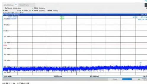
NTNV-n78(3450-3550)-PC1.5-30-80-H-DFT-BPSK-Inner_1RB_Right-3 0-1000-PASS
