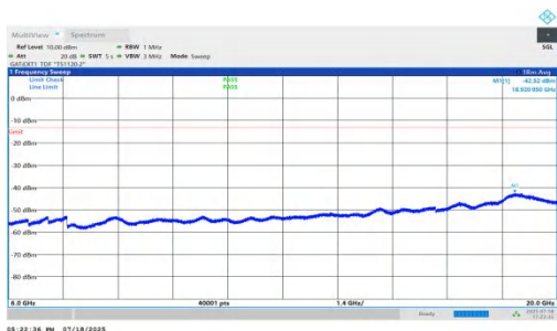
NTNV-n78(3450-3550)-PC1.5-30-90-H-DFT-QPSK-Inner_1RB_Right-6000-20000-PASS
