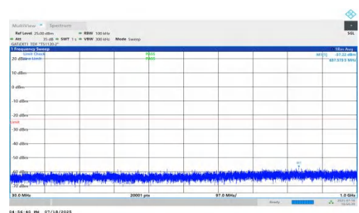
NTV-n78(3450-3550)-PC1.5-30-90-L-DFT-QPSK-Inner_1RB_Right-3 0-1000-PASS
