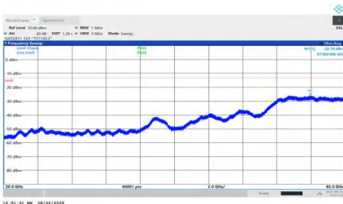
NTNV-n78(3450-3550)-PC1.5-30-90-L-DFT-BPSK-Inner_1RB_Left-20000-40000-PASS
