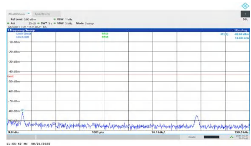
NTNV-n78(3450-3550)-PC1.5-30-90-H-DFT-QPSK-Inner_1RB_Right-0 .009-0.15-PASS
