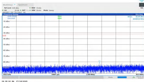
NTNV-n78(3450-3550)-PC1.5-30-80-H-DFT-BPSK-Inner_1RB_Right- 0.15-30-PASS
