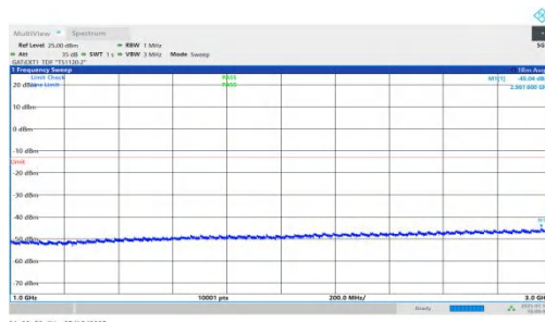
NTVN-n78(3450-3550)-PC1.5-30-80-L-DFT-QPSK-Inner_1RB_Left-1000-3000-PASS
