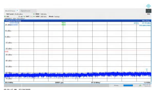
NTNV-n78(3450-3550)-PC1.5-30-70-H-DFT-QPSK-Inner_1RB_Right-3 0-1000-PASS
