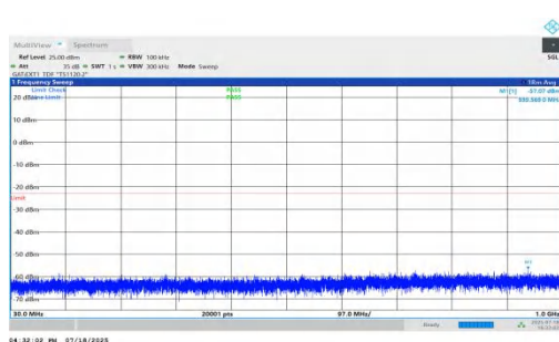
NTNV-n78(3450-3550)-PC1.5-30-80-M-DFT-QPSK-Inner_1RB_Right- 30-1000-PASS
