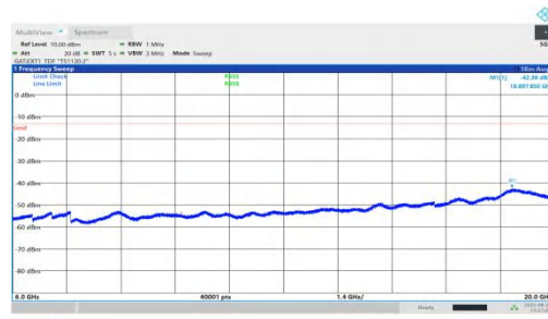
NTNV-n78(3450-3550)-PC1.5-30-100-L-DFT-QPSK-Inner_1RB_Left-6 000-20000-PASS
