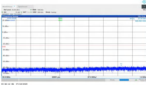
NTNV-n78(3450-3550)-PC1.5-30-70-H-DFT-BPSK-Inner_1RB_Left-3000-1000-PASS
