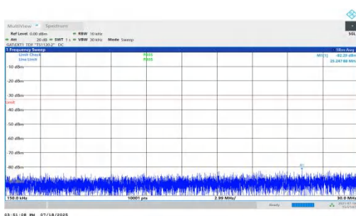
NTNV-n78(3450-3550)-PC1.5-30-70-H-DFT-QPSK-Inner_1RB_Right- 0.15-30-PASS
