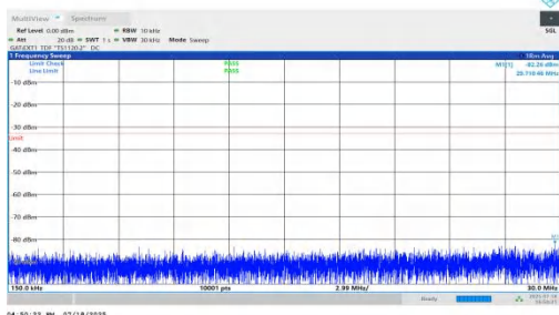
NTNV-n78(3450-3550)-PC1.5-30-90-L-DFT-BPSK-Inner_1RB_Right-0.15-30-PASS
