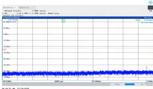
NTNV-n78(3450-3550)-PC1.5-30-80-M-DFT-BPSK-Inner_1RB_Left-30-1000-PASS
