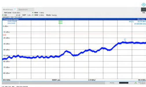
NTNV-n78(3450-3550)-PC1.5-30-80-M-DFT-QPSK-Inner_1RB_Left-2 0000-40000-PASS
