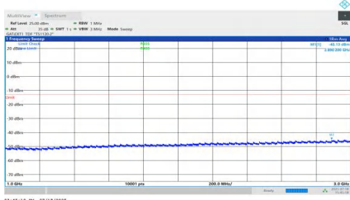
NTNV-n78(3450-3550)-PC1.5-30-70-H-DFT-BPSK-Inner_1RB_Right-1000-3000-PASS
