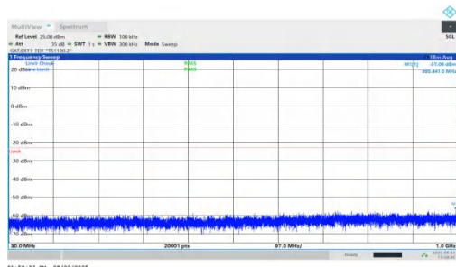
NTNV-n78(3450-3550)-PC1.5-30-100-L-DFT-QPSK-Inner_1RB_Right-30-1000-PASS
