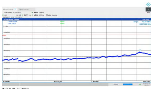
NTNV-n78(3450-3550)-PC1.5-30-80-M-DFT-QPSK-Inner_1RB_Right-6000-20000-PASS
