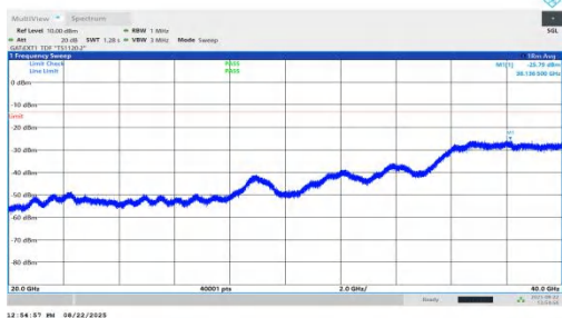
NTNV-n78(3450-3550)-PC1.5-30-90-M-DFT-QPSK-Inner_1RB_Left-2 0000-40000-PASS
